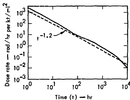
Fig. A-3. Fission-product delay.
