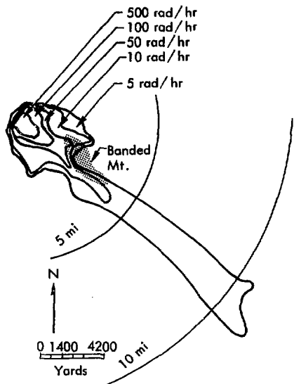
Fig. 15. Fallout pattern for Teapot shot at H+1 hr.
