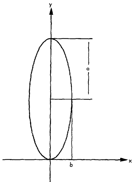
Fig. A-5. Isodose ellipse with focus at origin (ground zero).
