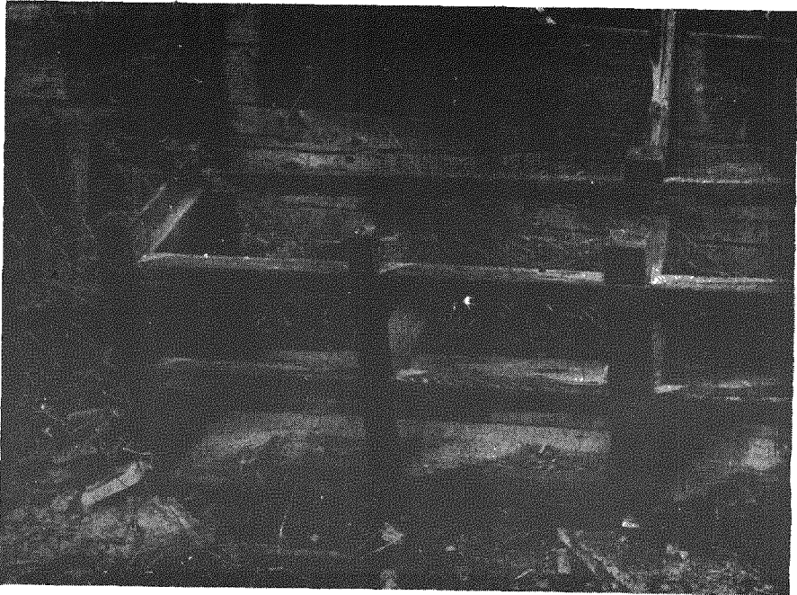
Photo No. 22. NAGASAKI. Timber framing scorched by heat radiation at \frac{1}{3} mile from the centre of damage. The surface is unscorched where it is shielded by the uprights. See paragraph 52.
