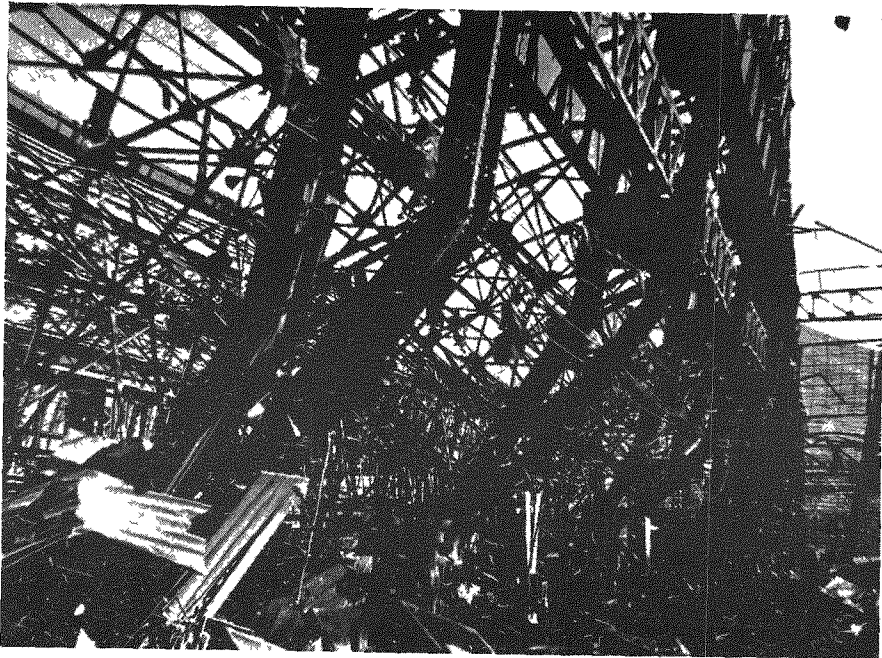
Photo No. 12. NAGASAKI. Large steel framed shed in the Mitsubishi Steel Works, \frac{3}{4} mile from the centre of damage. The steel stanchions have been bent (away from the explosion) and the roof trusses on both sides of these stanchions have collapsed. See paragraphs 22 and 32.
