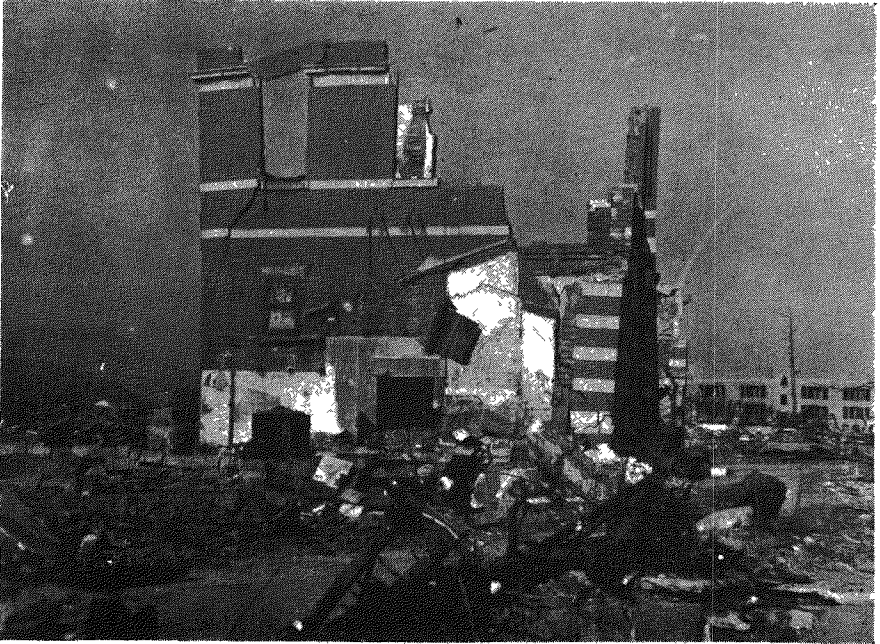
Photo No. 15. HIROSHIMA. Three storey bank building with load bearing brick walls of strong construction and comparable with British standards. This degree of damage to such buildings extends to a radius of \frac{1}{4} mile from centre of damage. Compare with the behaviour of the reinforced concrete framed building in the background. See paragraph 38.
