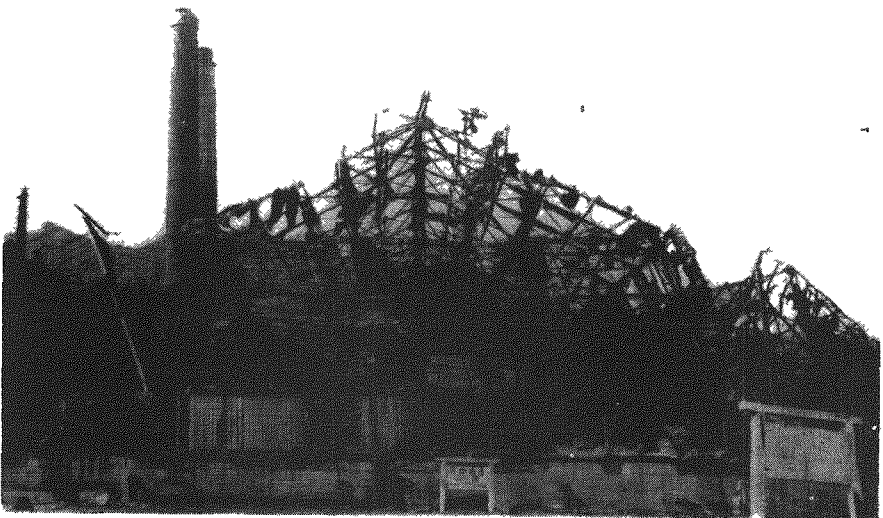
Photo No. 6. NAGASAKI Mass distortion of steel framed shed buildings about half a mile from the centre of damage, which was to the right of the buildings in the photograph. It will be seen that the entire main frame is seriously distorted away from the explosion. See paragraphs 15, 22 and 32.
