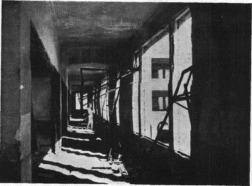
Photo No. 9. HIROSHIMA. Reinforced concrete school 500 yds. from the centre of damage, which is to the right. The frame of this building was of special design (portal) and resisted the lateral forces. The outside walls were of continuous reinforced concrete, and although they were deflected, as seen, they did not fail. See paragraph 27.
