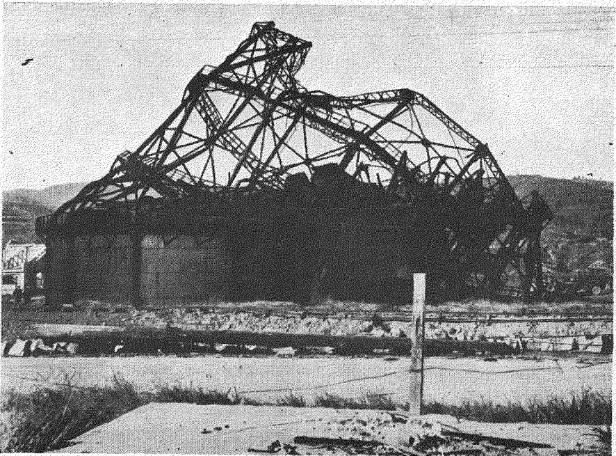
Photo No. 14. NAGASAKI. Blast effect on a gasholder \frac{1}{2} mile from centre of damage. Note the way in which the whole framework has been bent away from the explosion. See paragraph 43.
