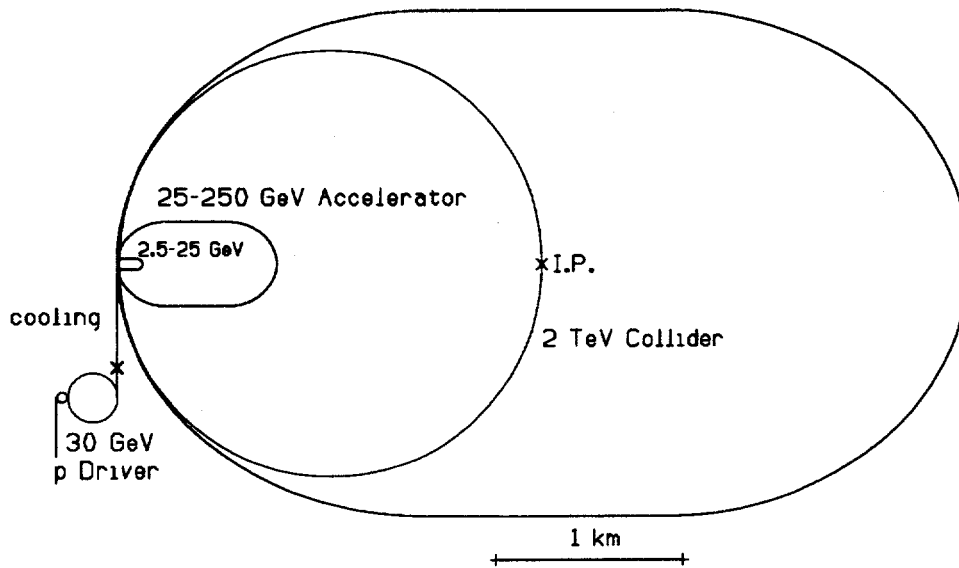
Figure 1: Possible layout of accelerators
