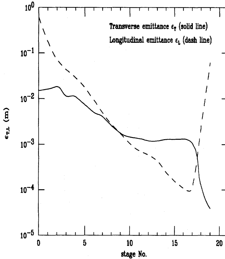
Figure 7: \epsilon_L and \epsilon_T vs stage number in the cooling sequence.
