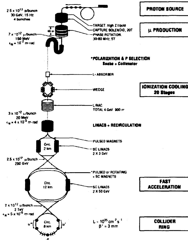
Figure 4: Schematic of a Muon Collider.
