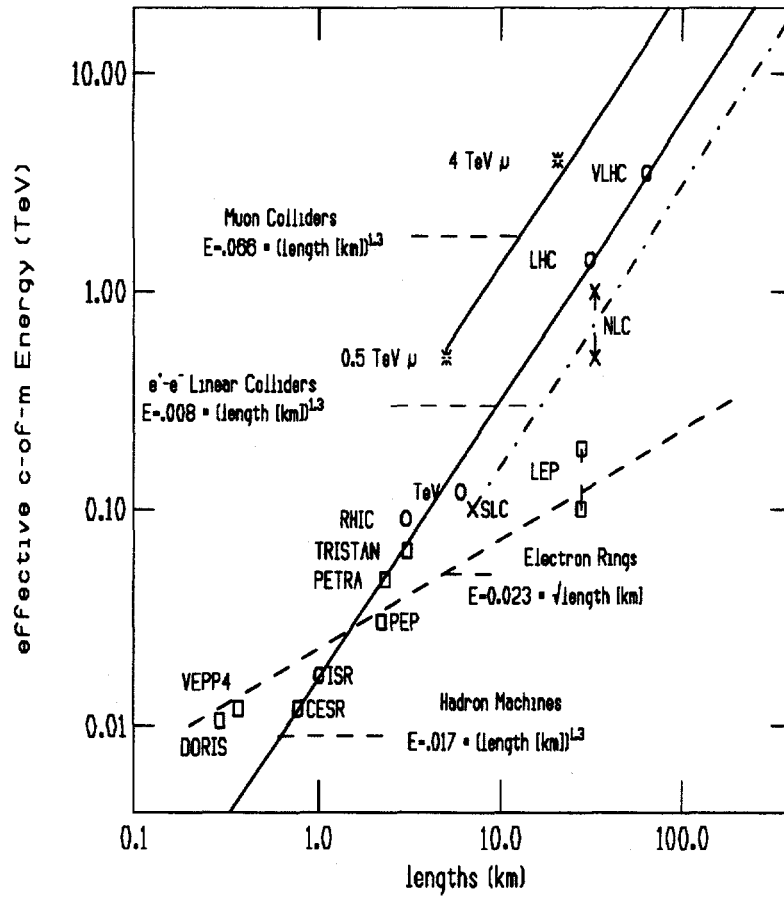
Figure 3: Effective energies of colliders as a function of their total length.
