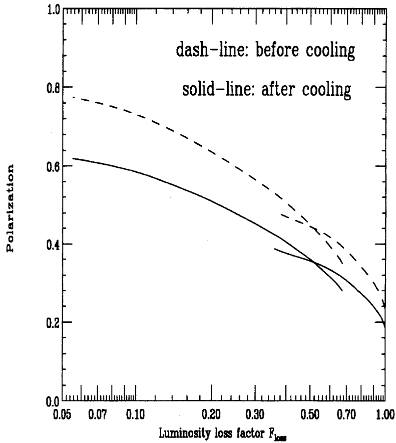
Figure 6: Polarization vs F_{\mu} of muons accepted; the dashed line shows polarization as selected before cooling; the solid line gives the polarization after cooling.
