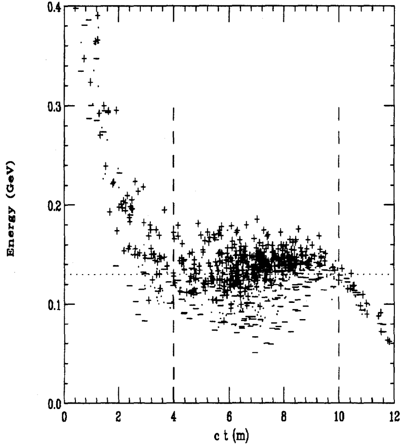
Figure 5: Energy vs ct of muons at end of decay channel with phase rotation. muons with polarization P > \frac{1}{3} , -\frac{1}{3} < P < \frac{1}{3} and P < -\frac{1}{3} are marked by the symbols '+', '.' and '-' respectively.
