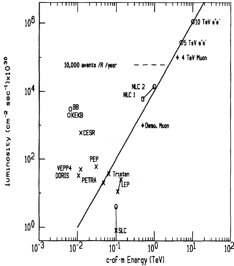
Figure 2: Luminosity of lepton colliders as a function of energy
