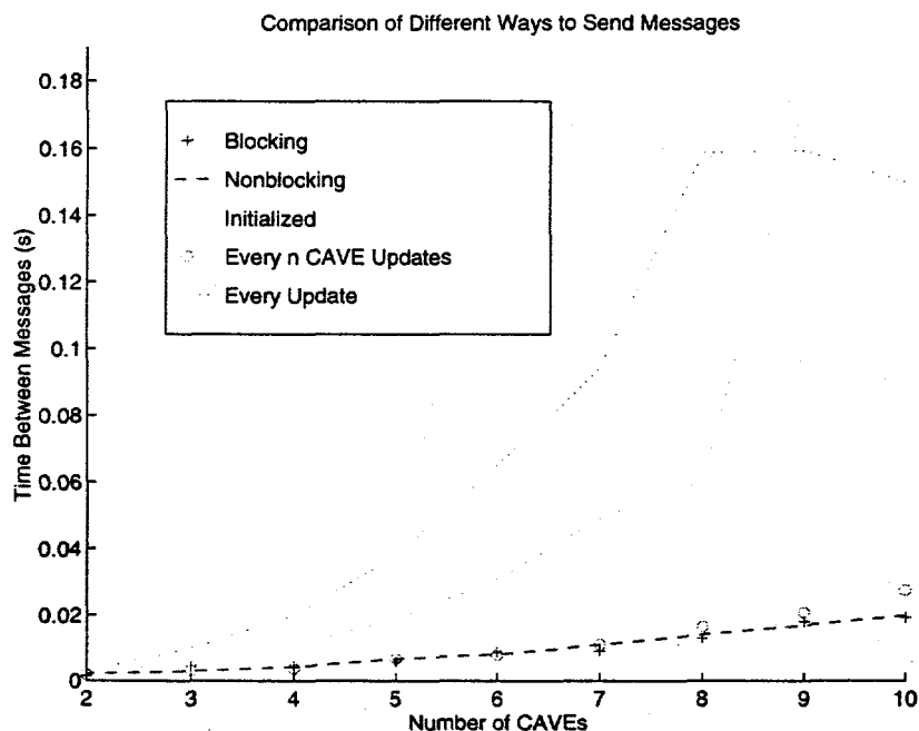
Figure 9: Measurements of time needed to send tracker data using various MPI message sending techniques.
