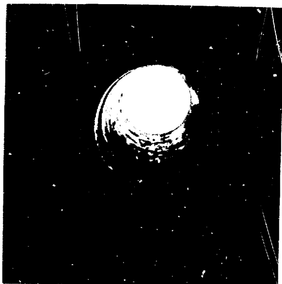
Fig. 1. Glass-lined hole melted in laboratory specimen of tuff.
