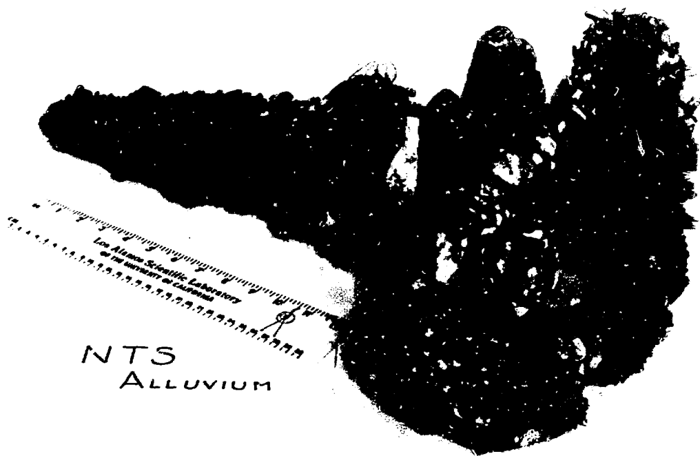
Fig. 8. External surface of glass-lined hole melted in dry alluvium.
