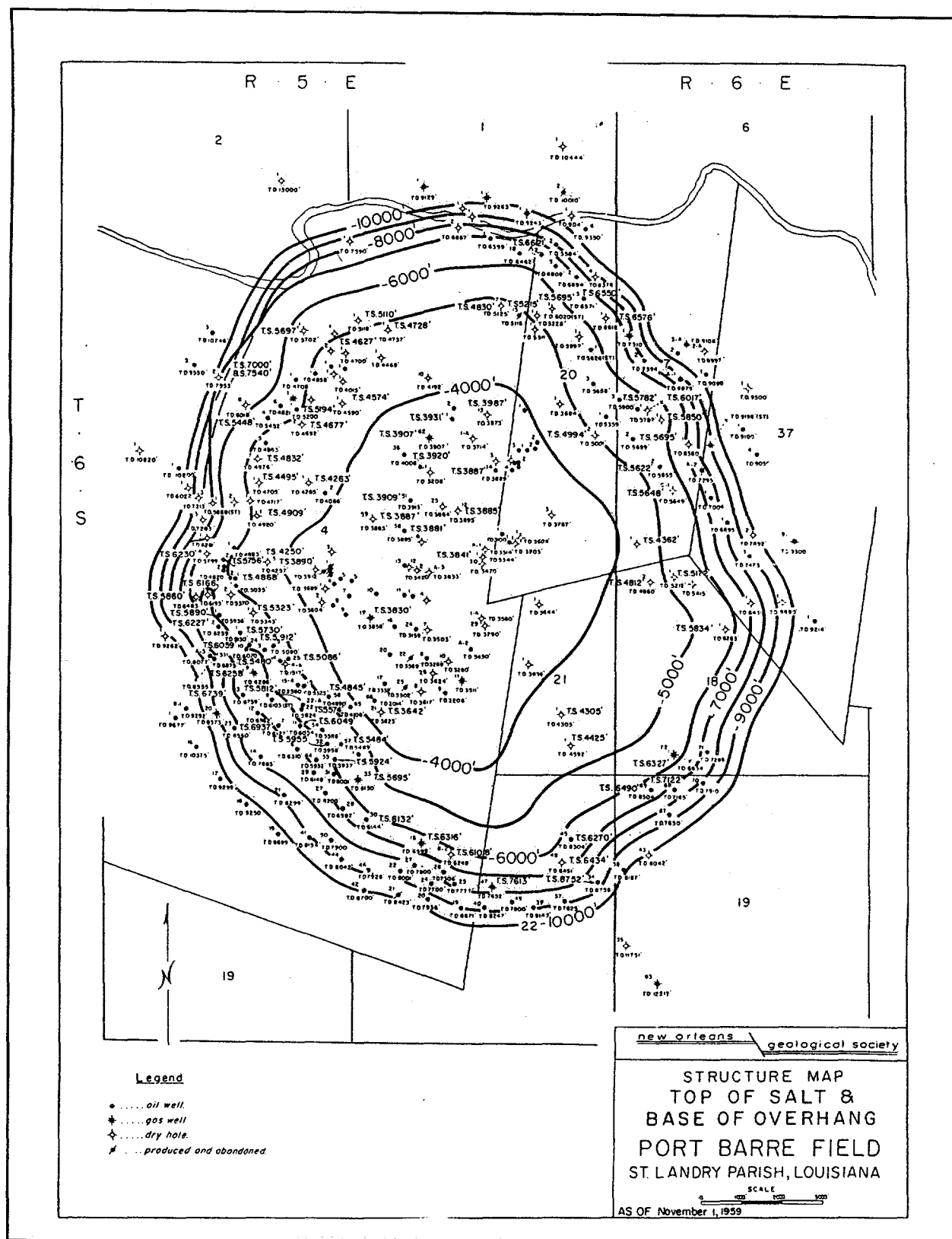
Figure 73. Subsurface map of top of salt found in Port Barre field. (from Stipe 1960)
