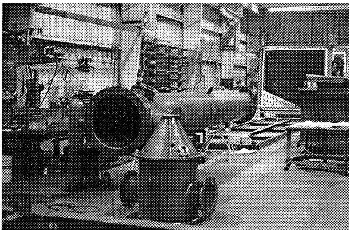
Figure 4. Photograph of collection section taken during fabrication.
