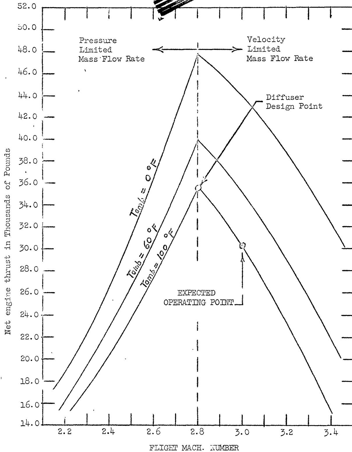
Fig. 1 Tory II-C net engine thrust vs. flight Mach. No., Maximum Fuel Element Wall Temperature = 2500^\circ F , Altitude = 1000 ft.
