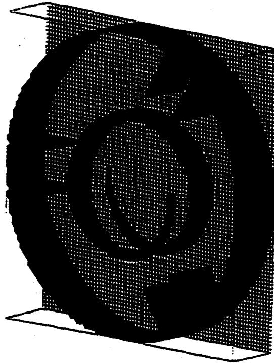
Figure 9. ARGUS structure plot for the helix TWT.
