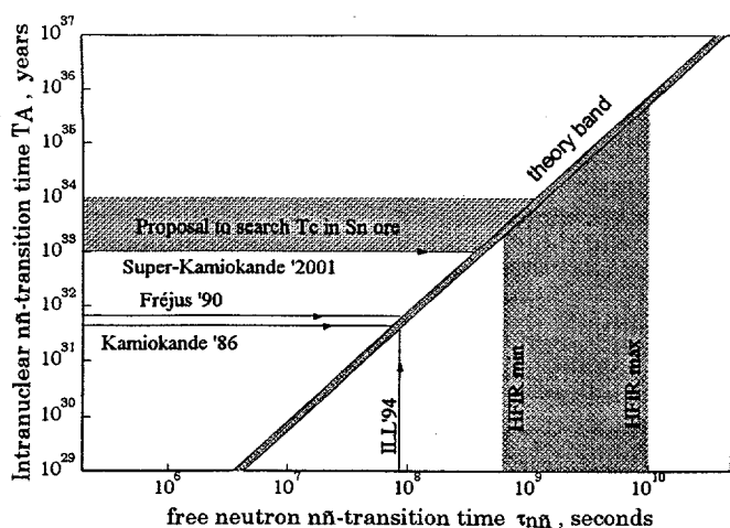
Fig 3. Comparison of n \rightarrow \bar{n} searches in intranuclear transitions ( \tau_A ) to those in free-flying neutron experiments ( \tau_{n-\bar{n}} ). Shaded areas indicate possible improvement in HFIR-based experiment with free neutrons [13-15] and in a new proposed experiment with long-lived isotopes [30].
