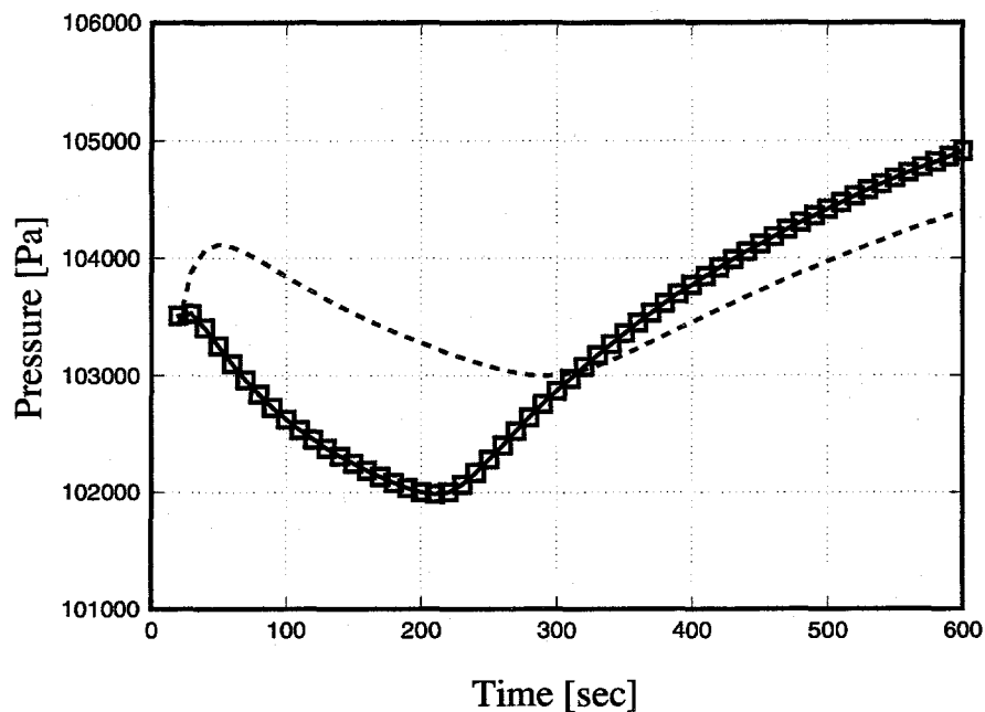
Figure D.4.2. Part 4: Pressure transient at center of column calculated with initial parameter set (dashed line) and after optimization (solid line). Synthetic data are shown as squares.
