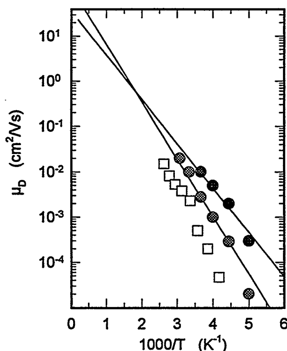
Fig. 7. Semilogarithmic plot of average hole drift mobility \mu as a function of reciprocal temperature 1/T for a displacement/field ratio of L/E = 2 \times 10^{-9} \text{ cm}^2/\text{V} . Two solid lines are a multiple-trapping fit. Open symbols represent the result from an optimized a-Si:H sample.
