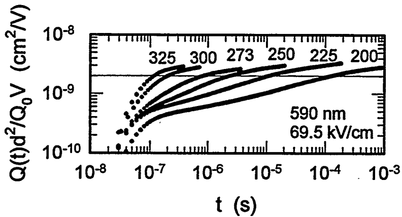
Fig. 6. (upper) Normalized transient photocurrents i(t)d^2/Q_0V for holes measured at \lambda = 590 nm at several temperatures and constant electric field of 69.5 kV/cm. (lower) Logarithmic plot of Q(t)d^2/Q_0V for the same conditions as the transients; for times sufficiently early that carriers have not yet been swept completely across the structure, the charge transient measures the time dependence of L(t)/E of the hole displacement L(t) to the electric field E . The intersection of each curve with the line at 2 \times 10^{-9} cm 2 /V determines the transit times used to calculate a standard drift mobility.
