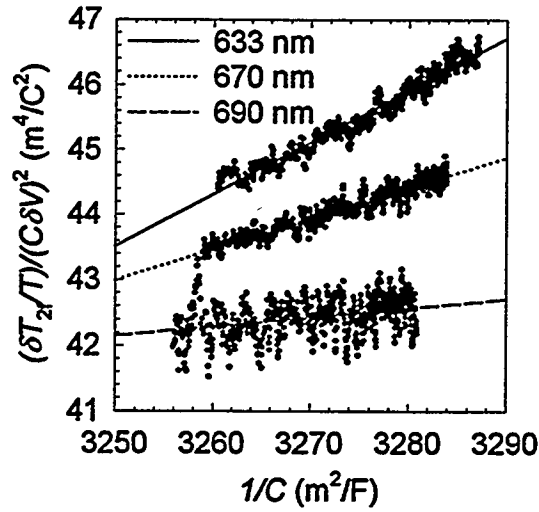
Fig. 4. Plot of the normalized, second harmonic electroabsorption signal \delta T_2/T for three different wavelengths as a function of reciprocal capacitance in the standard cell; the data are generated by varying the reverse bias across the cell.
