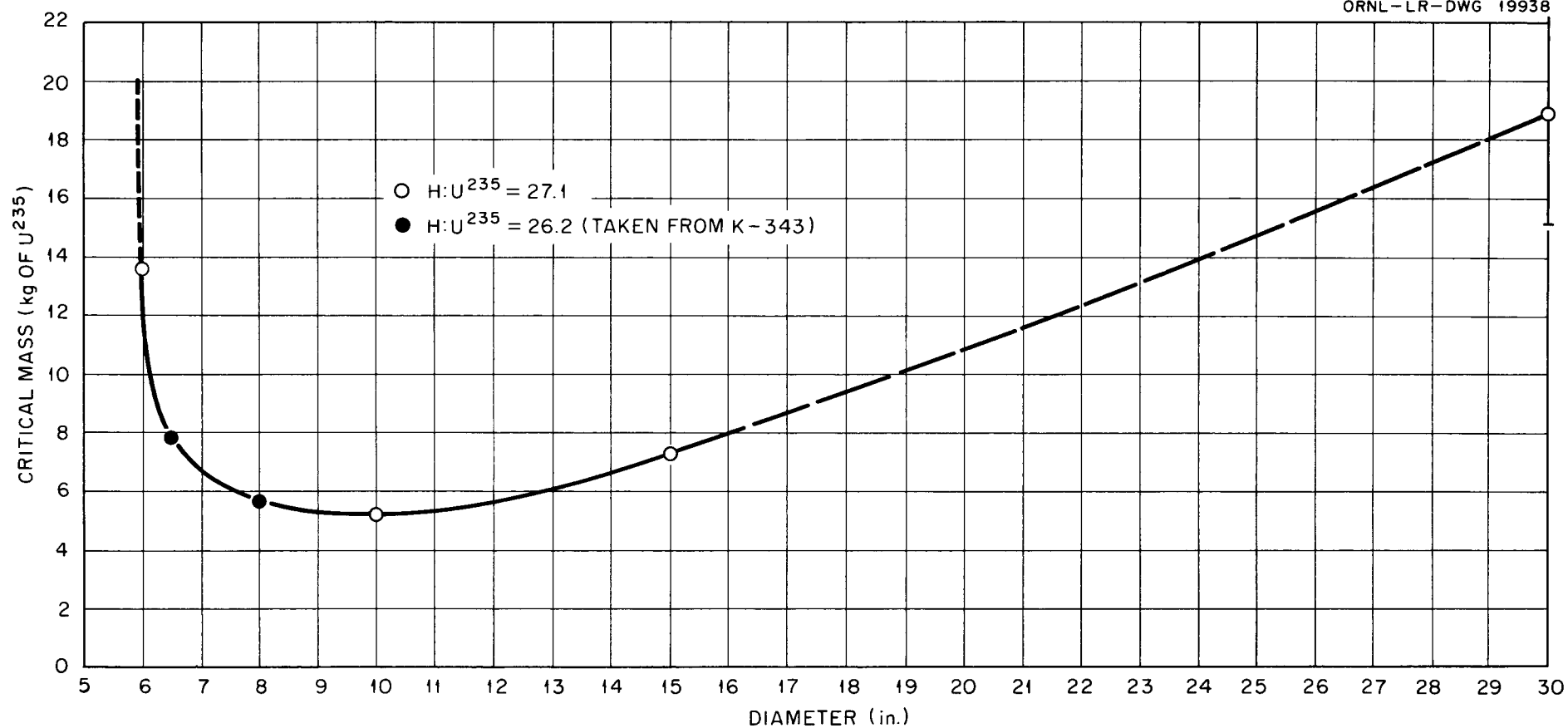
Fig. 11. Critical Mass as a Function of the Diameter of Single Water-Reflected Aluminum Cylinders Containing an Enriched U^{235} Solution.
