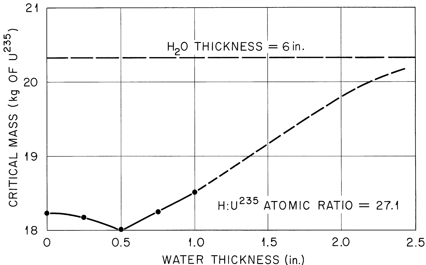
Fig. 23. Critical Mass as a Function of the Thickness of Water Between the Bottom of a 20-in.-dia Cylinder Containing an Enriched U 235 Solution and a 5.5-in.-thick Carbon Reflector .
