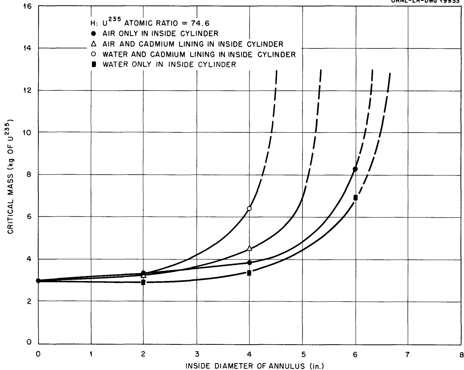
Fig.18. Critical Mass as a Function of the Inside Diameter of a Water-Reflected 10-in.-OD Annulus Containing an Enriched U^{235} Solution; Inside Cylinder Filled with Air, or Water, with and without Cadmium Lining.
