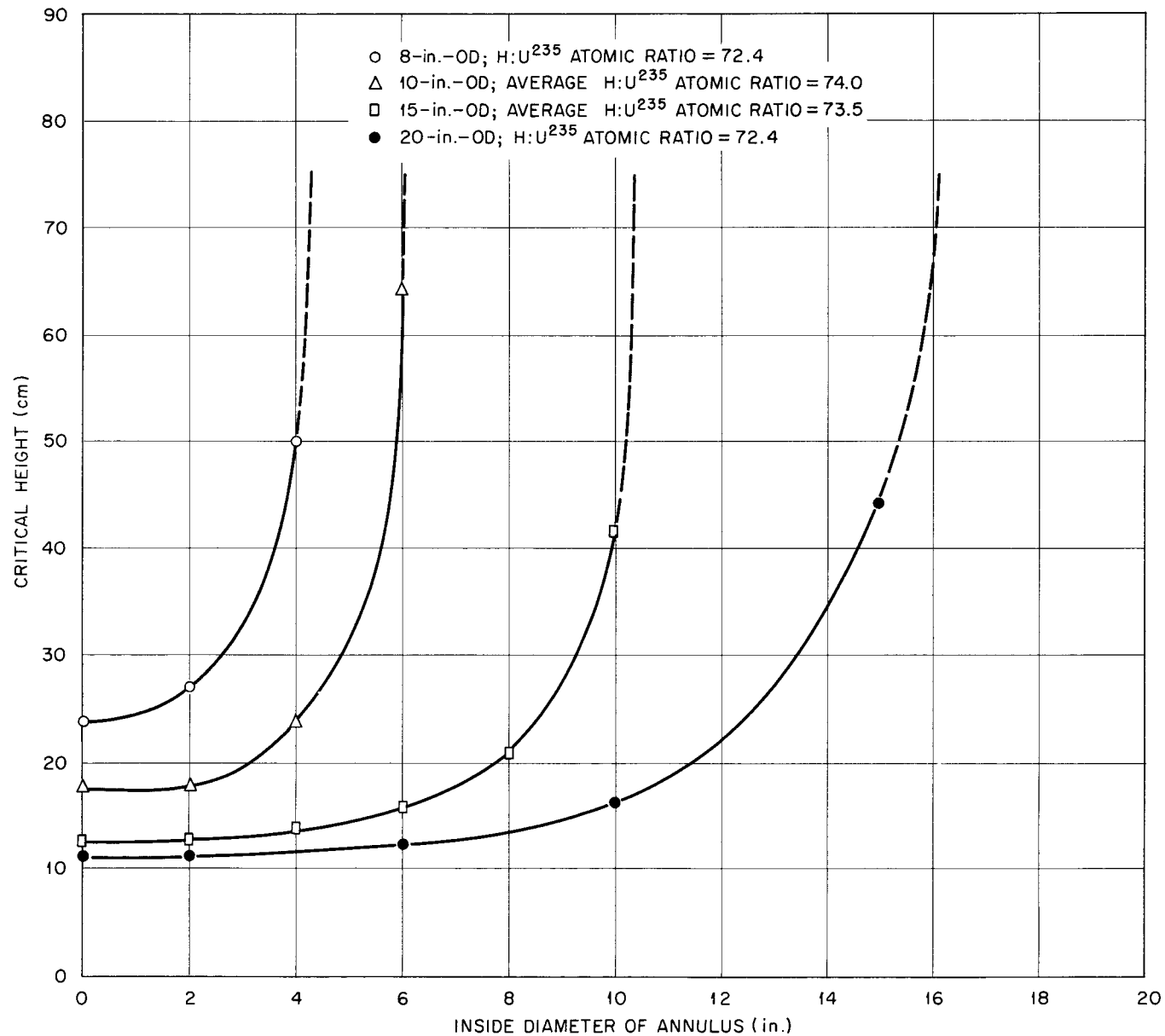
Fig. 17. Critical Height as a Function of the Inside Diameter of Water-Reflected Cylindrical Annuli Containing Enriched U 235 Solutions: Inside Cylinder Filled with Water.
