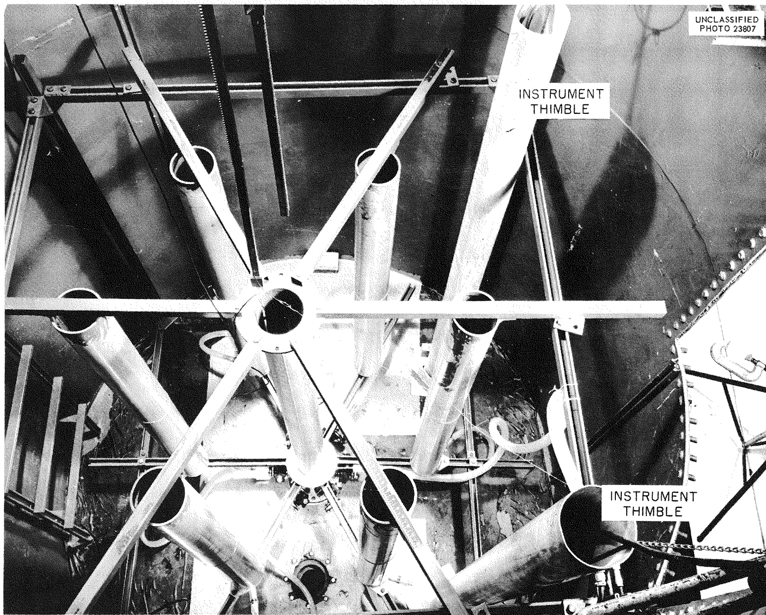
Fig. 1. Typical Arrangement for Critical Experiments with Interacting Arrays of Aluminum Cylinders Containing Enriched U^{235} Solutions.
