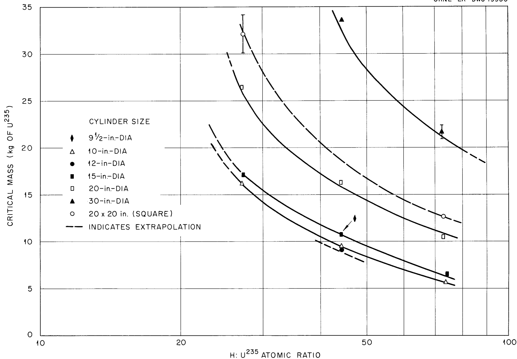
Fig. 15. Critical Mass as a Function of the H: U^{235} Atomic Ratio of Solutions Contained in Single Unreflected Aluminum Cylinders.
