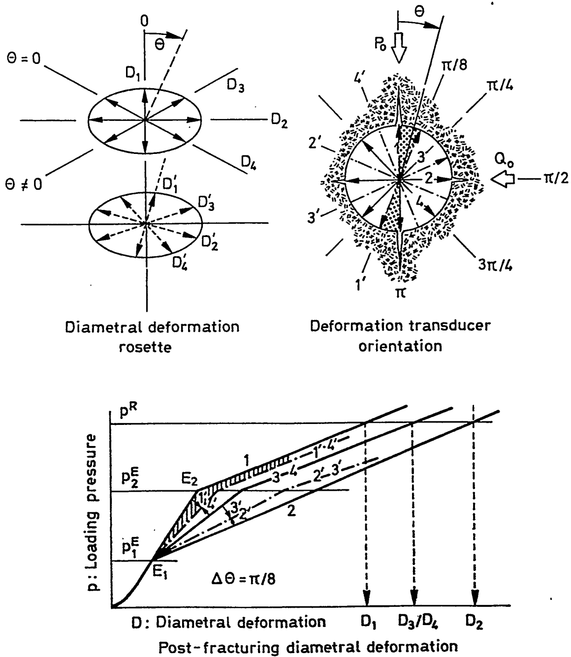
Fig. 4 Two identical deformation rosettes being obtained by double fracture probe set at two different angular orientations, compared with corresponding set of 4 p-D curves monitored by the probe set at \theta = 0 .
