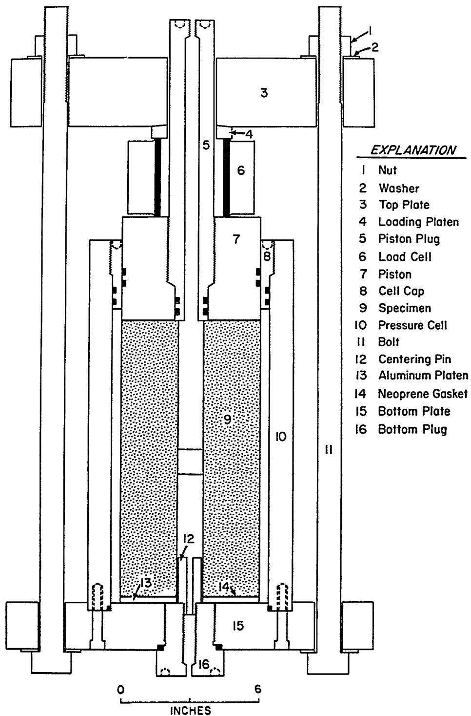
Figure 4. Radial permeameter cell.
