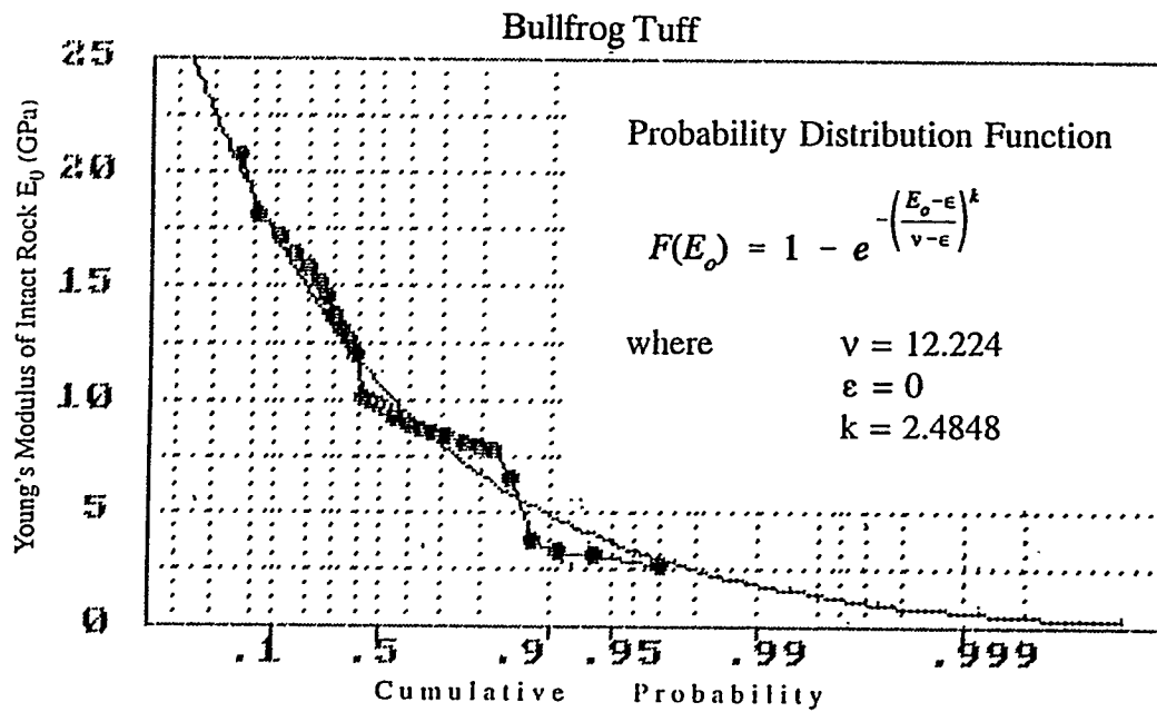
Figure 3. Observed and theoretical extremal distributions of Young's modulus ( E_o ) of Bullfrog Tuff obtained from laboratory core tests
