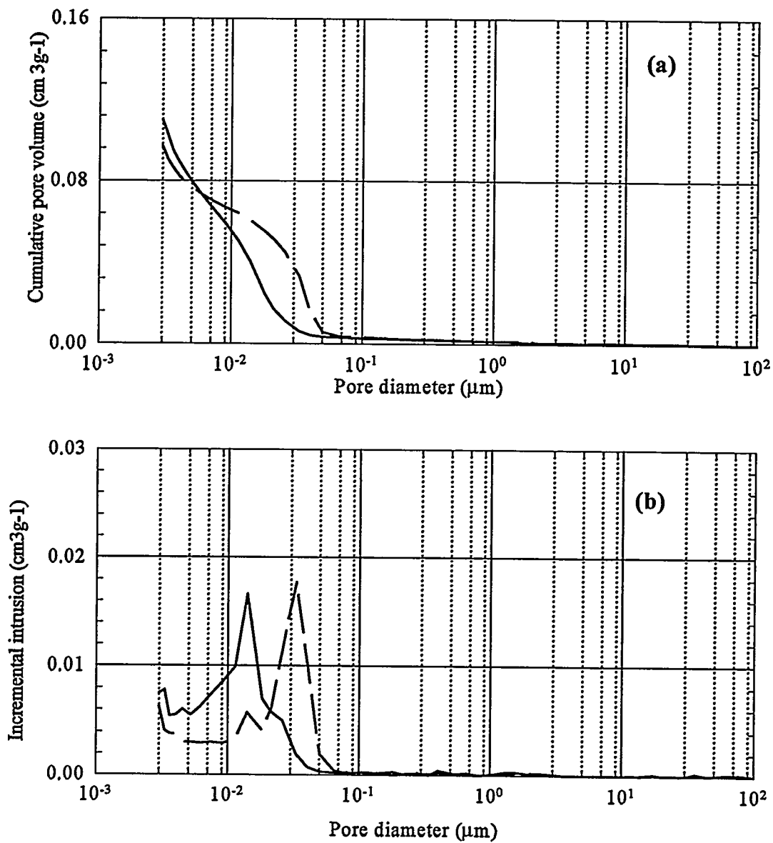
Figure 8. The effect of leaching time (dashed line - after 1 day, continuous line - after 32 days) on the pore size distribution for the reference grout mixed at W/CM = 0.4 and leached in DDW at 10^\circ\text{C} under static conditions.
