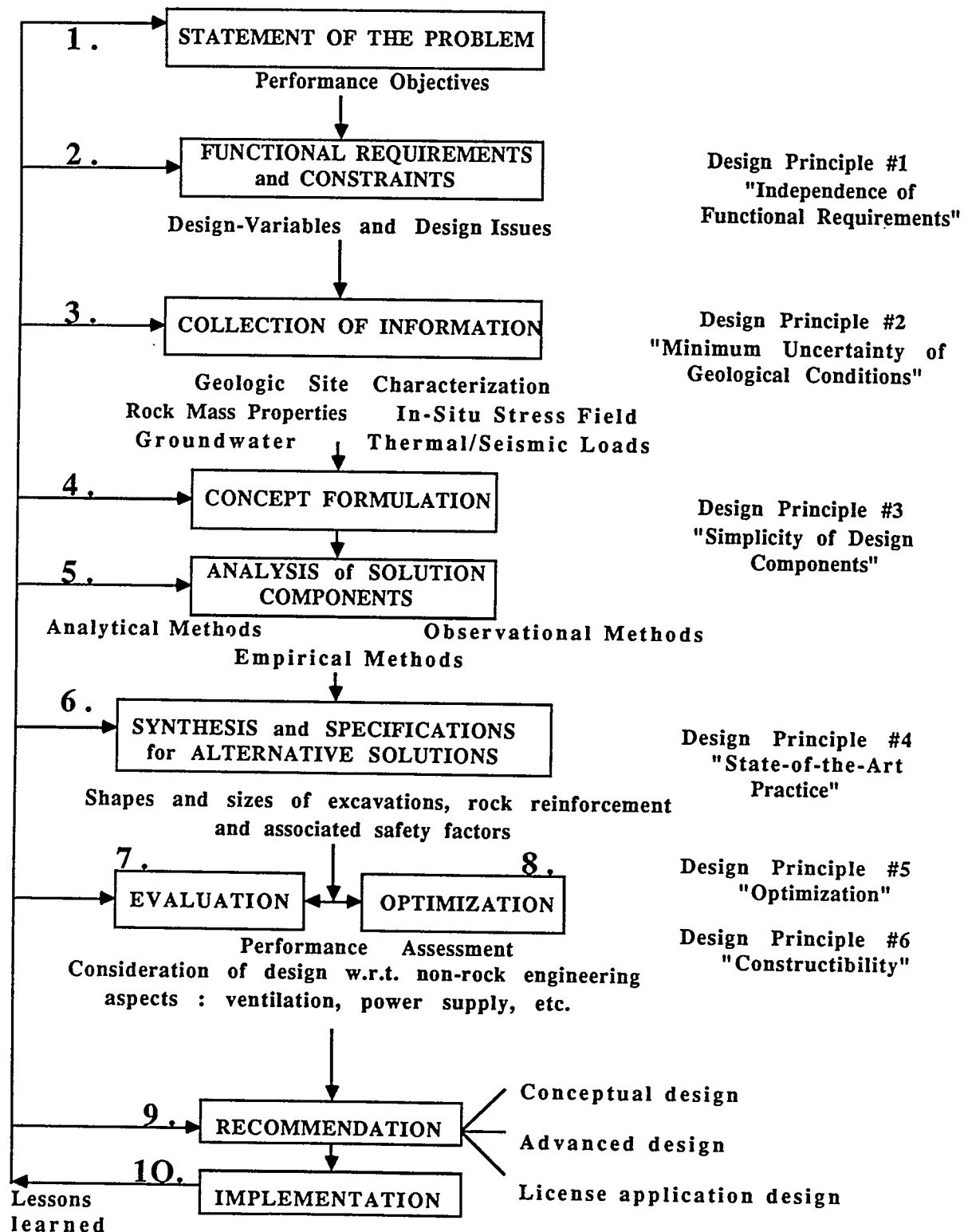
Figure 2 Systems Design Methodology for rock engineering, including the use of design principles (Bieniawski, 1993).
