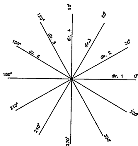
Fig. 2a Directions along which joint roughness measurements and joint shear testing were performed.
