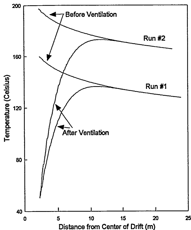
Figure 3 Temperature Profile for Runs #1 and #2.
