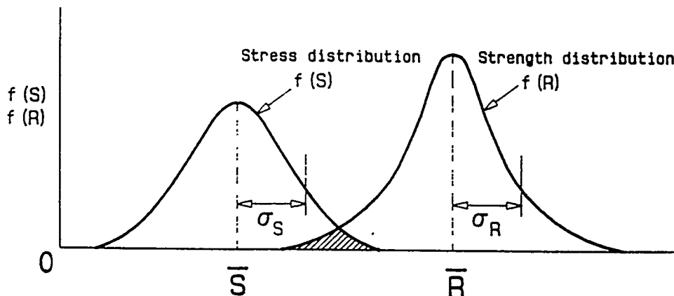
Figure 7. Stress (S) and strength (R) probability distributions (after Haugen, 1968), The overlap between the strength and stress distributions indicates the zone that contributes to the probability of failure.
