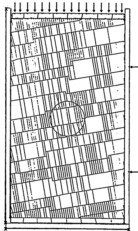
Figure 2 DDA Mesh for Run #4
