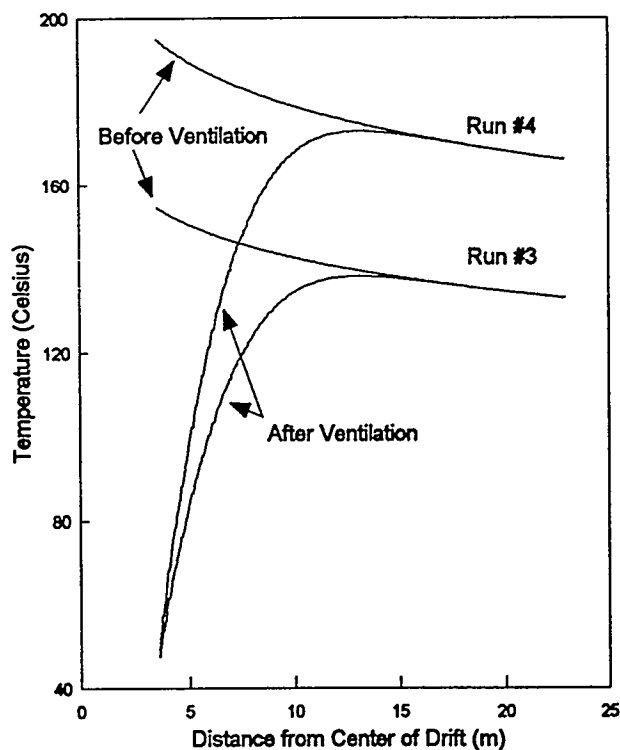
Figure 4 Temperature Profile for Runs #3 and #4.
