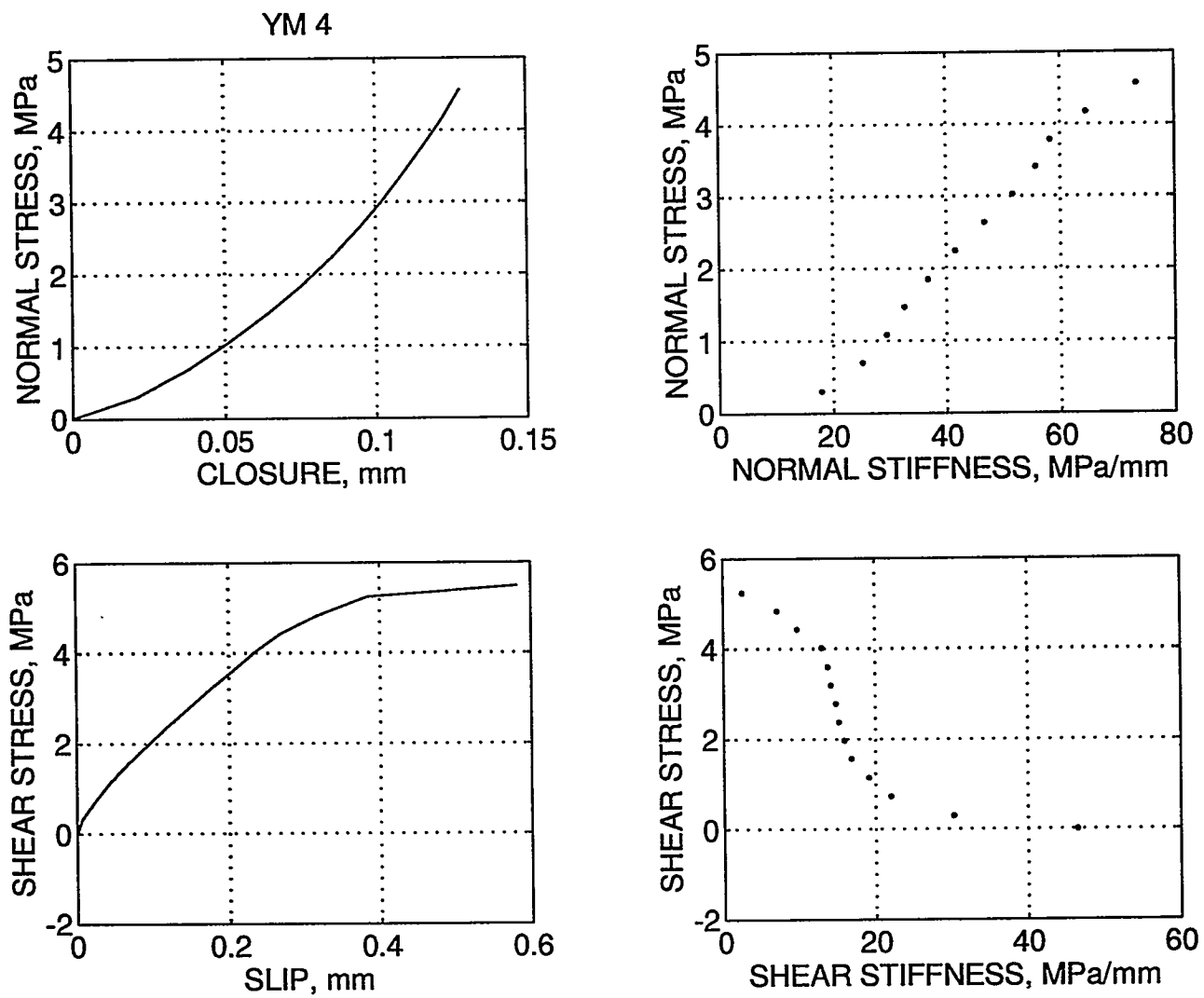
Figure 2: Shear and normal stiffness data for YM 4.
