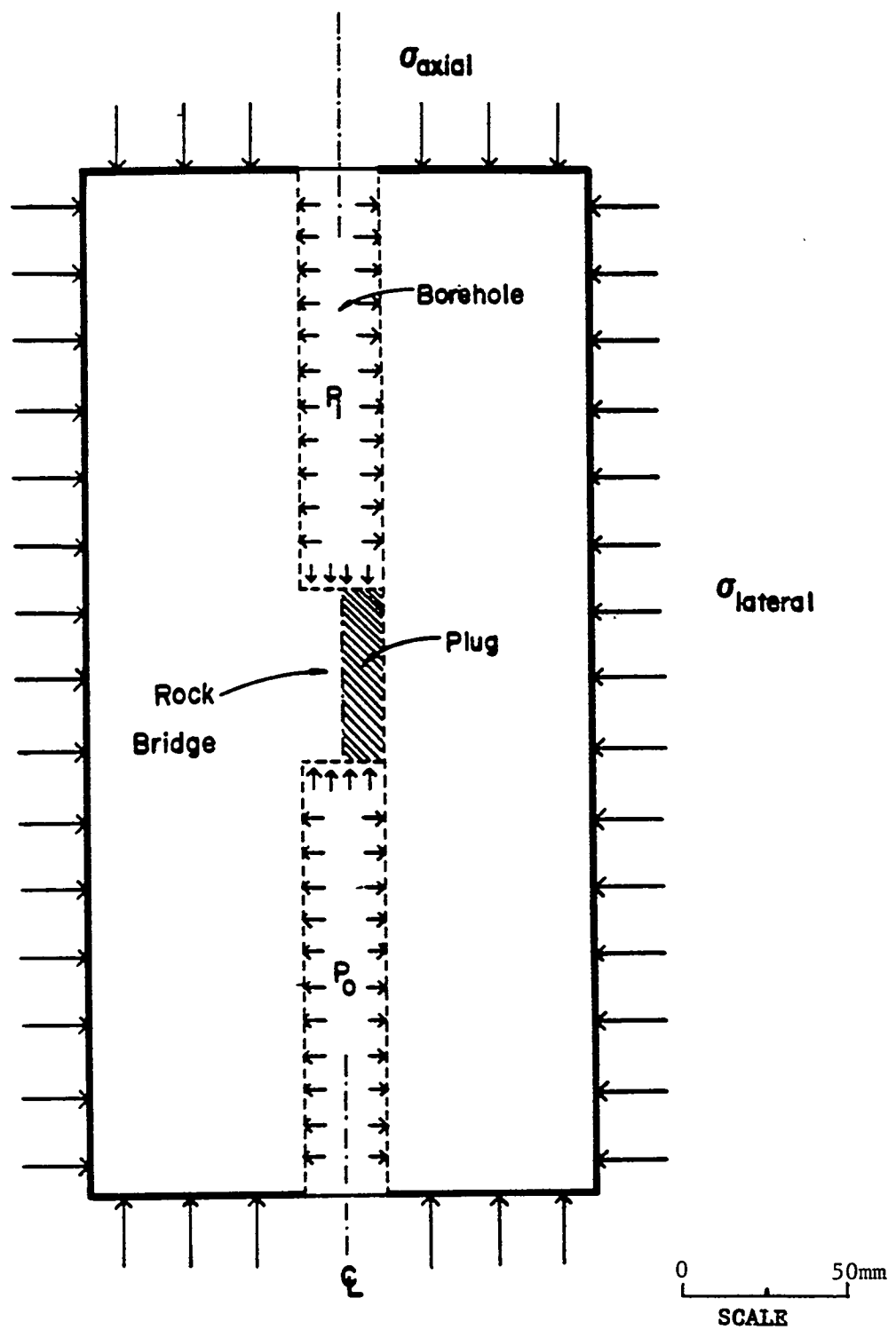
Figure 5. Loading configuration on radial permeameter specimen.
