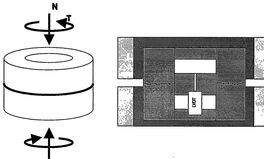
Figure 1: Sample configuration for rotary shear experiments on joints. Left is a perspective view showing applied forces. Right is a cross-section; light grey is aluminum holder, dark grey is potting compound, medium grey is rock sample, white is LVDT body and core, and mounting supports. Setup also included LVDT's mounted diametrically to outside of aluminum ring, measuring across joint. Not to scale.
