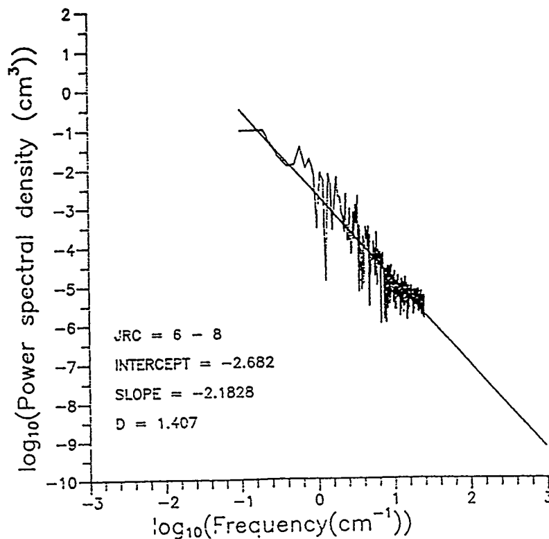
Fig. 4 Spectral analysis results for Barton's profile having JRC = 6 - 8.
