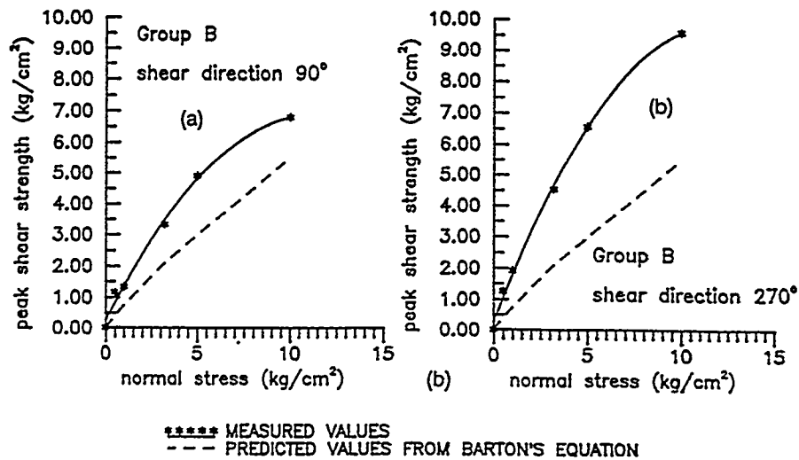
Fig. 3 Typical direct shear test results for group B (a) shear direction 90° (b) shear direction 270°.
