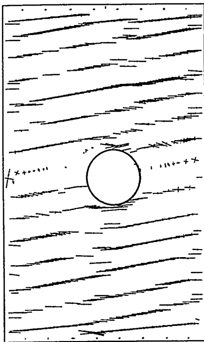
Scale: 100MPa ——— Figure 9 Principal Stresses After Rapid Cooling for Run #4
