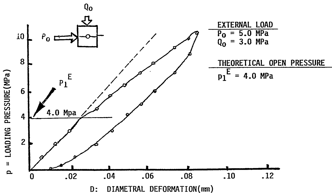
Fig. 14 Laboratory demonstration of detecting reopening pressure p_1^E of single fracture made in uniform property concrete test block (1m x 1m x 1m) subject to initial uniform stress loading, demonstrating stress measurement accuracy for single fracture method to be expected at
