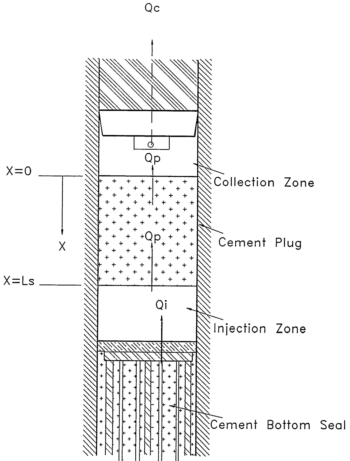
Figure 12. Configuration of in-situ borehole plug prepared for steady state and transient flow testing.
