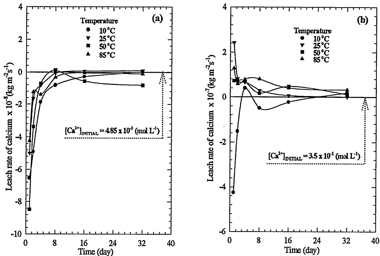
Figure 9. The effect of leaching time and temperature on the leach rate of \text{Ca}^{2+} for the reference grout mixed at W/CM = 0.4 and reacted with: a) WN-1 and b) SCSSS groundwaters under static conditions.
