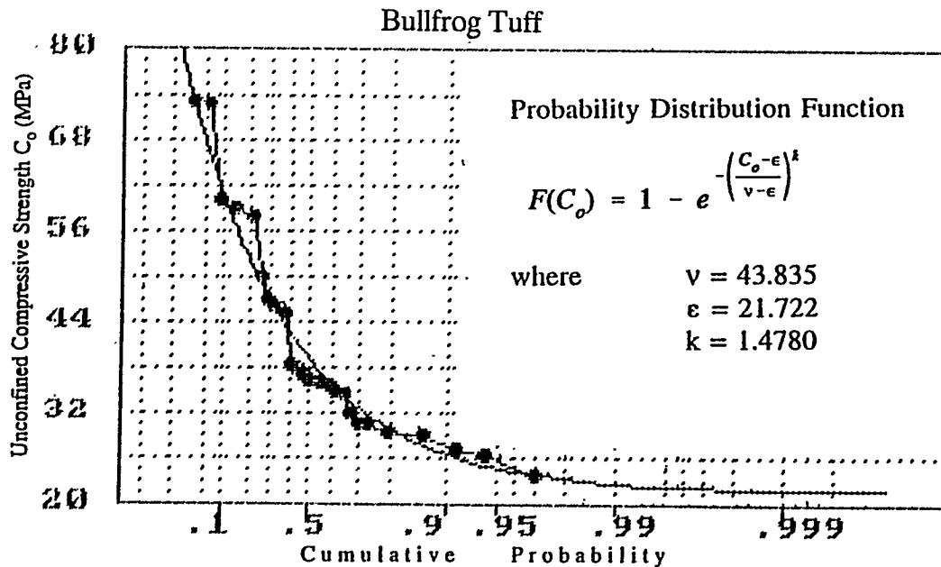
Figure 4. Observed and theoretical extremal distributions of unconfined compressive strength ( C_o ) of Bullfrog Tuff obtained from laboratory core tests
