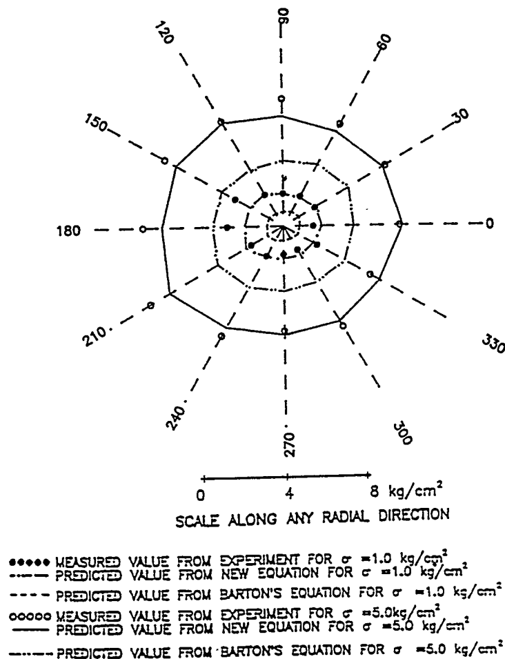
Fig. 5 Comparison between the predicted (based on the new equation and Barton's equation) and measured peak shear strength for group A.
