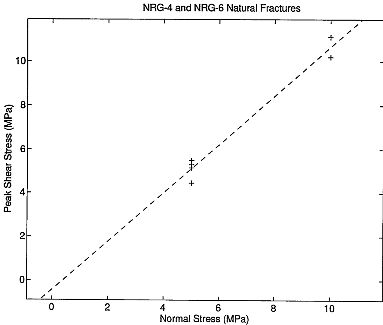
Figure 5: Peak shear stress versus normal stress data for all seven experiments.
