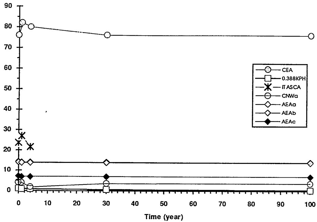
Water flux ( \times 10^{-8} \text{ m}^3 / \text{s} ) across tunnel surface vs. time.
