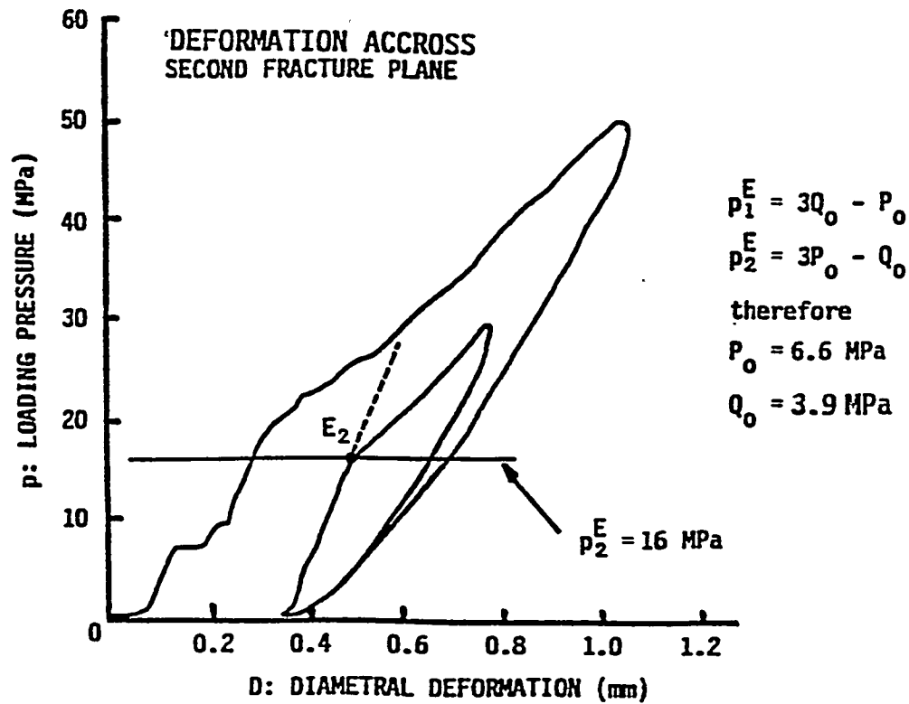
Fig. 3 Typical field observation of pair of p-D diagrams taken in the two mutually perpendicular directions of principal stresses directly disclosing stress state and material properties.
