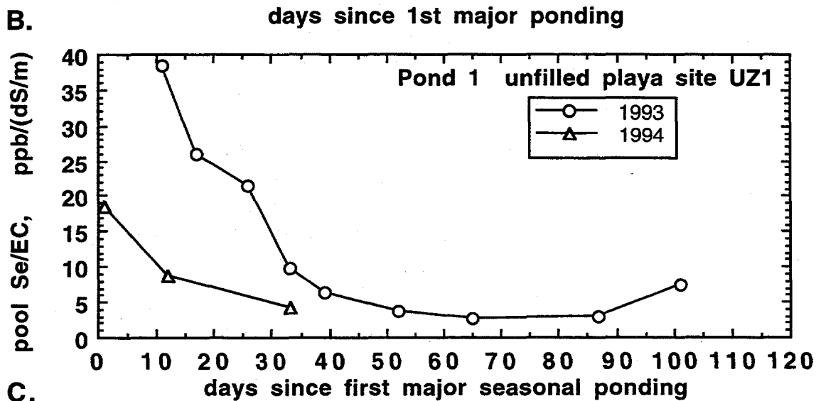
Figure 7.8. Examples of surface water quality in ephemeral pools formed over lowland Kesterson Reservoir soils subject to water table rise (site P1-UZ1). Time trends for (A) selenium concentrations (with surface water quality goal of 5 ppb indicated by the horizontal line), (B) salinity (EC), and (C) [Se]/EC ratios.
