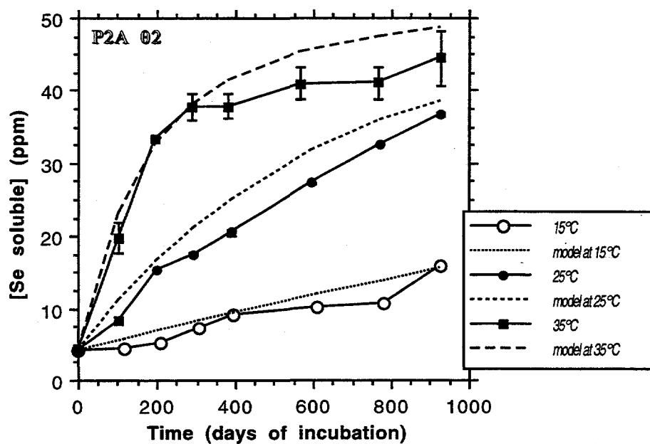
Figure 6.9. Changes in soluble-Se in soil P2A, as a result of incubation at 15°C, 25°C, and 35°C and moisture content 02. Dashed lines correspond to results of modeling as discussed in text.
