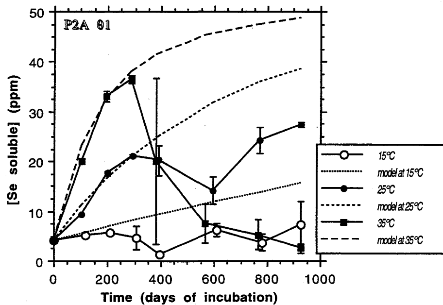
Figure 6.8. Changes in soluble-Se in soil P2A, as a result of incubation at 15°C, 25°C, and 35°C and moisture content 01. Dashed lines correspond to results of modeling as discussed in text.
