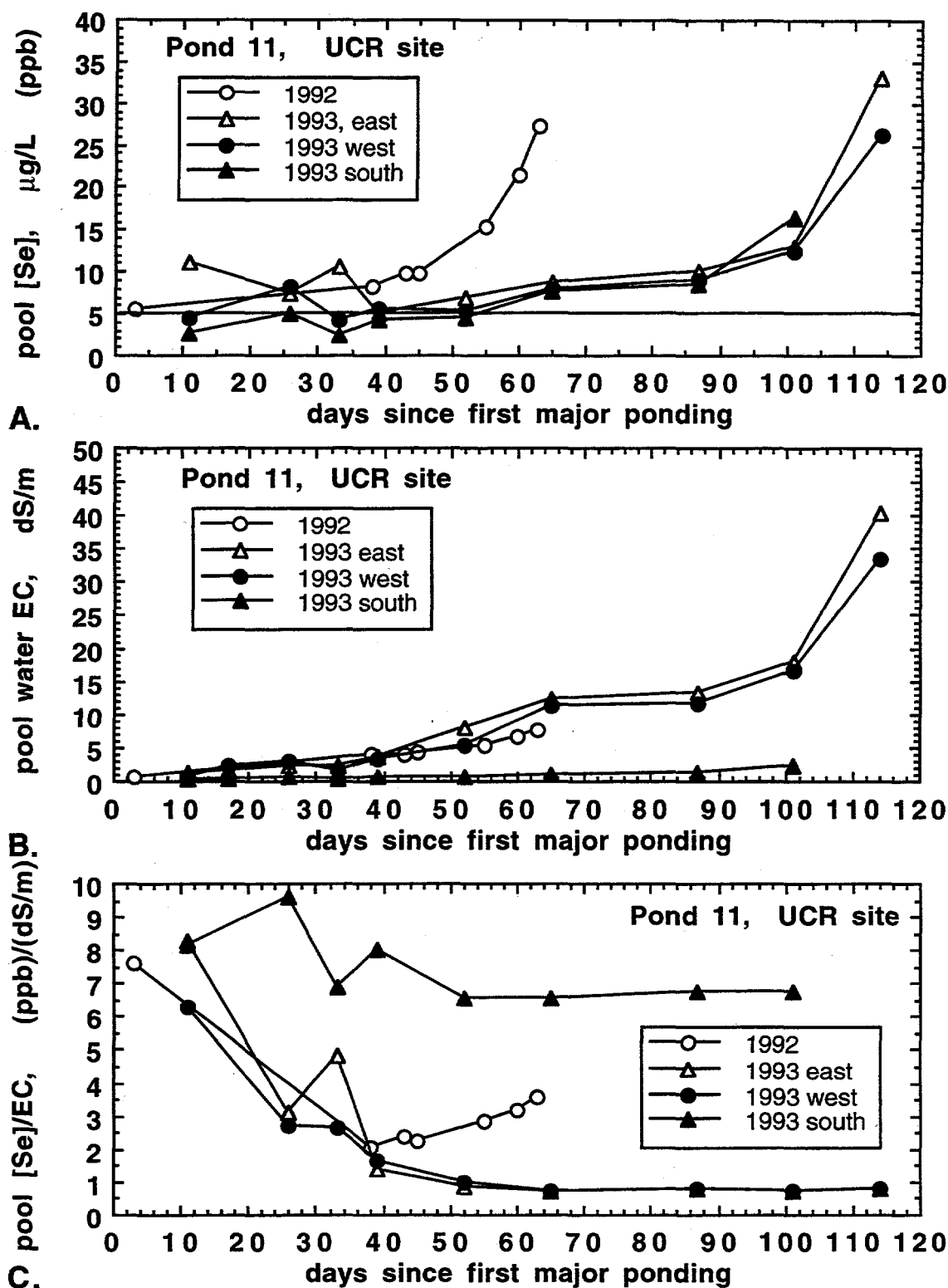
Figure 7.7. Examples of surface water quality in ephemeral pools formed over upland Kesterson Reservoir soils at site P11-UCR. Time trends for (A) selenium concentrations (with surface water quality goal of 5 ppb indicated by the horizontal line), (B) salinity (EC), and (C) [Se]/EC ratios.
