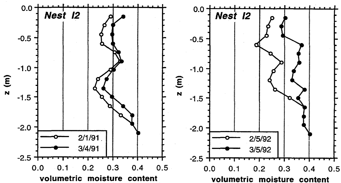
Figure 5.4. Changes in moisture content in treatment I, due to heavy rains over periods of roughly 1 month, as estimated from neutron probe readings.
