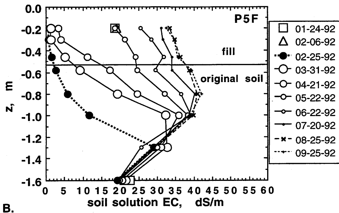
Figure 2.3.1. Soil solution Se concentrations (A), and salinities (B) at the P5F fill monitoring site during 1992, before and after the Feb. 1992 rainstorms.
