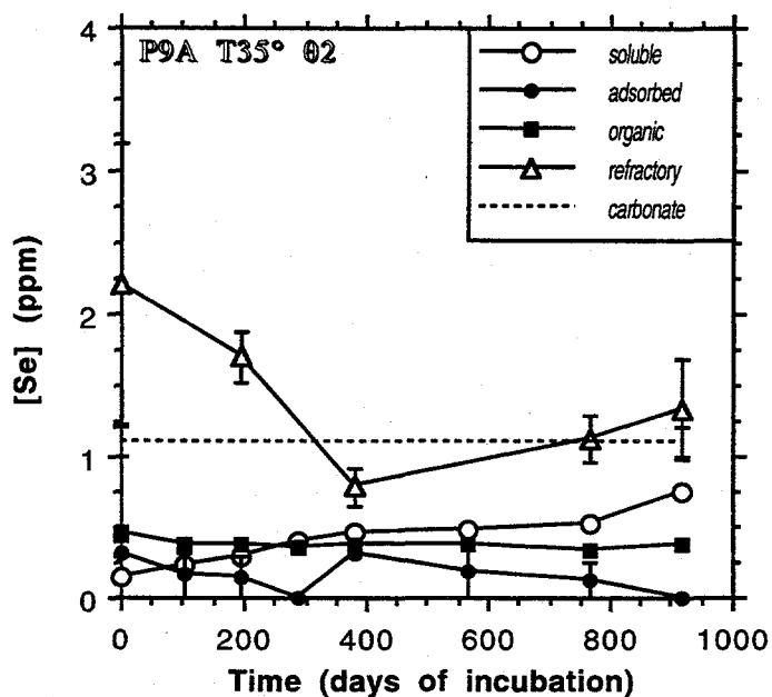
Figure 6.6. Changes in Se fractionation with time as measured in soil P9A, incubated at 35°C and moisture content 0.2. The carbonate-Se concentration is based on an initial and final analysis only.
