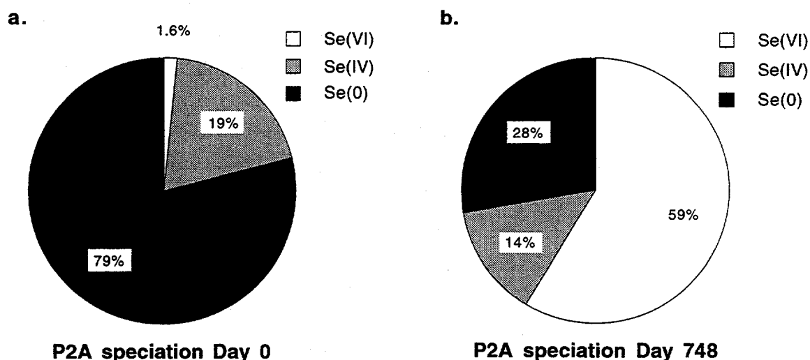
Figure 6.13. Selenium speciation results of x-ray spectroscopy of soil P2A, (a) before incubation and (b) after 748 days at 35°C and moisture content 62.
