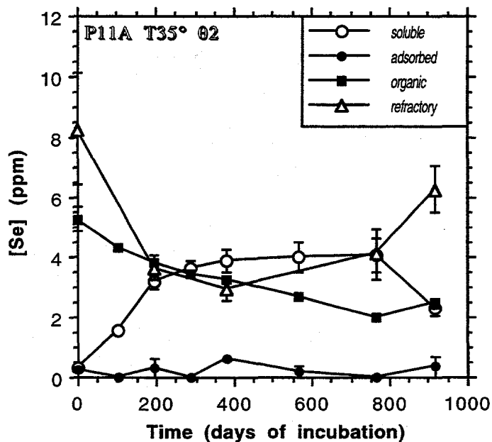
Figure 6.7. Changes in Se fractionation with time as measured in soil P11A, incubated at 35°C and moisture content 0.2.
