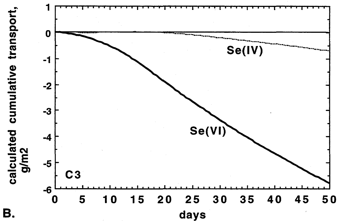
Figure 4.8. Calculated transport rates (A), and cumulative transport (B) of Se(IV) and Se(VI) between ponded waters and unamended sediment.
