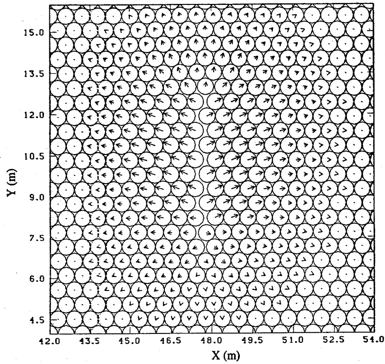
Figure 7: Loading vectors on spheres adjacent to a vertical blasthole. Uplift angle = 20^\circ .
