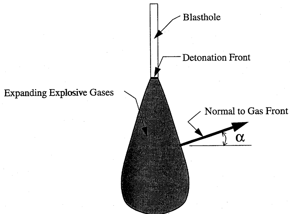
Figure 6: Definition of uplift angle, \alpha .
