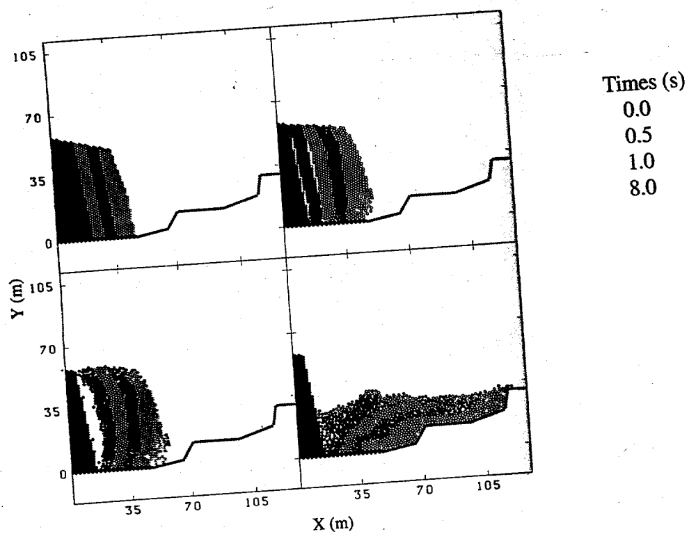
Figure 3: Bench blast simulation as in Figure 1 but with differentiated burdens.
