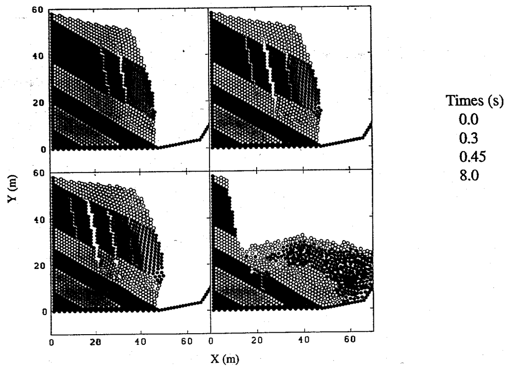
Figure 5: Bench blast simulation as in Figure 1 but with the fourth layer from the top decked-through with inert to prevent explosive loading.
