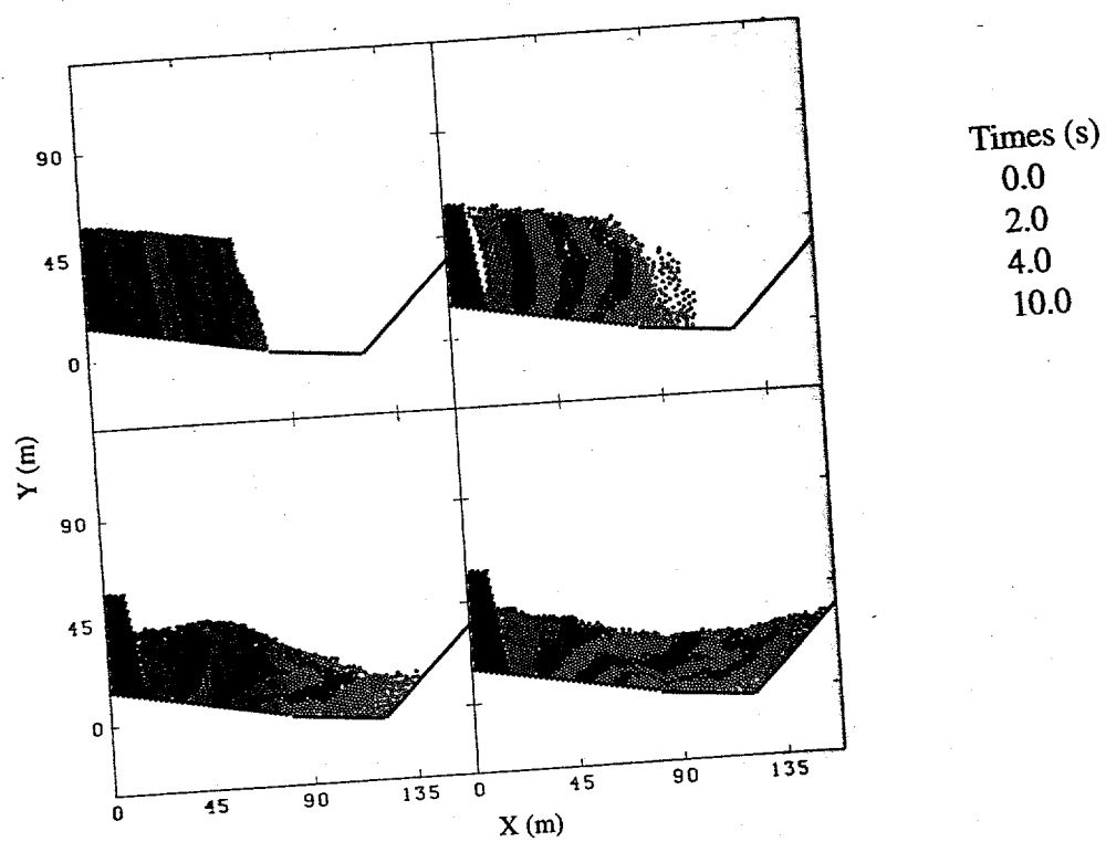
Figure 4: Bench blast simulation as in Figure 2 but with differentiated burdens.
