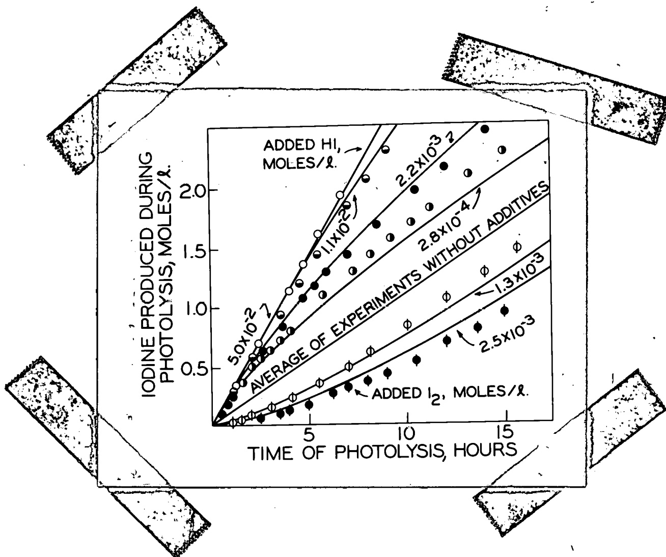
Fig. 1 Effect of added HI and I_2 on the photolysis of ethyl iodide at 25°. Points are from experimental data; curves are calculated.
