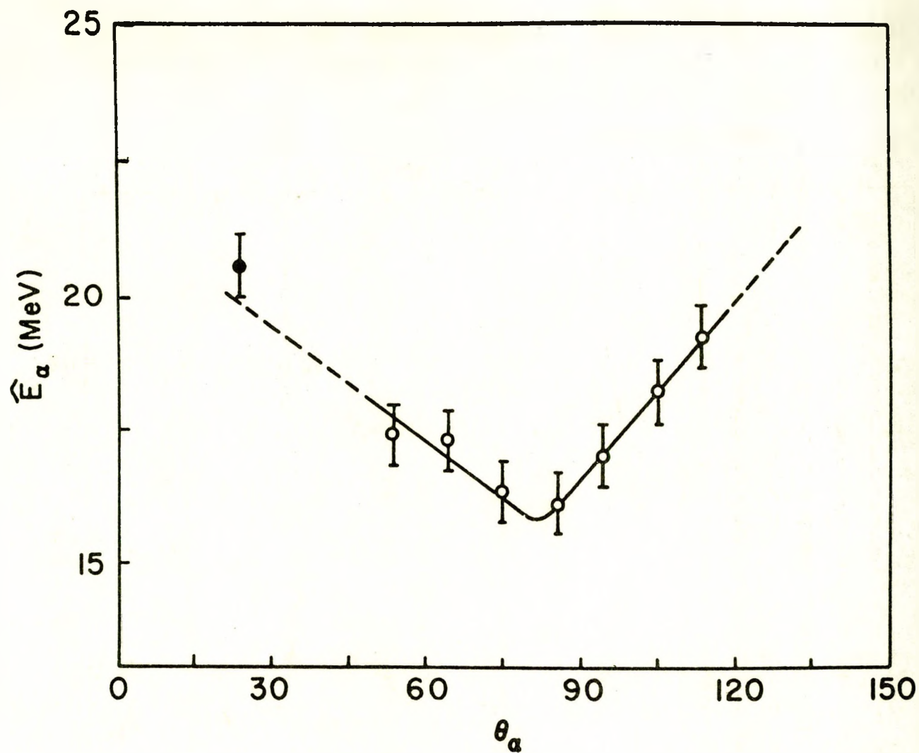
Fig. 3. Dependence on angle of emission on mean energy of long-range \alpha -particles. Solid point represents present experiment.
