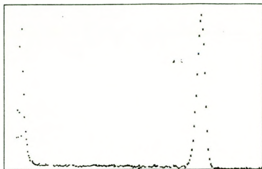
FIG 2A SPECTRA WITH BEAM CENTERED ON THE 1.25-INCH LONG ANODE OF THE PROTON-RECOIL TUBE
