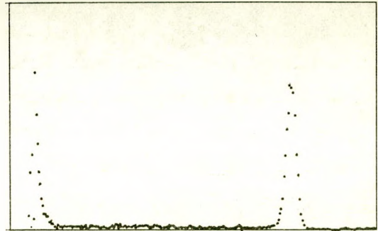
FIG 3B ^{14}\text{N}(\text{n,p})\text{C}^{14} PULSE-HEIGHT DISTRIBUTION FOR 2350 VOLTS BIAS
