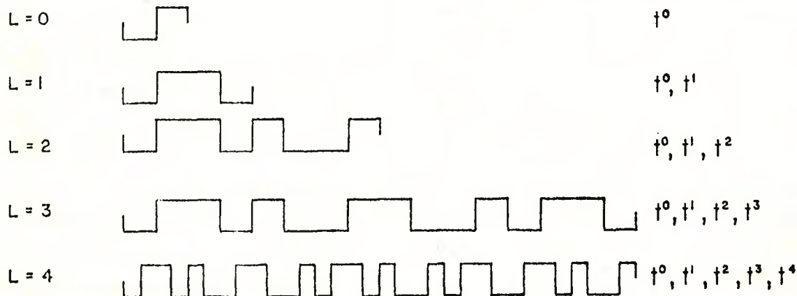
Fig. 1. Switching patterns from zeroeth to fourth order.
