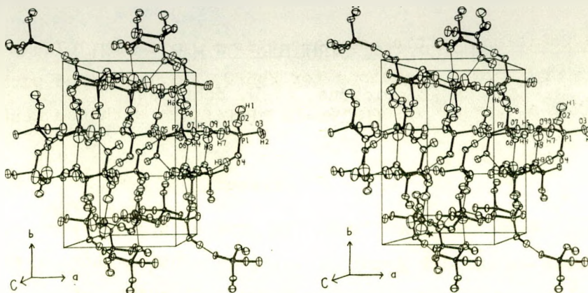
Fig. 1. Stereographic illustration of the crystal structure of \text{H}_3\text{PO}_4 \cdot 1/2\text{H}_2\text{O} . The water molecule oxygen and the P of one of the two crystallographically discrete \text{H}_3\text{PO}_4 molecules are both shaded.
