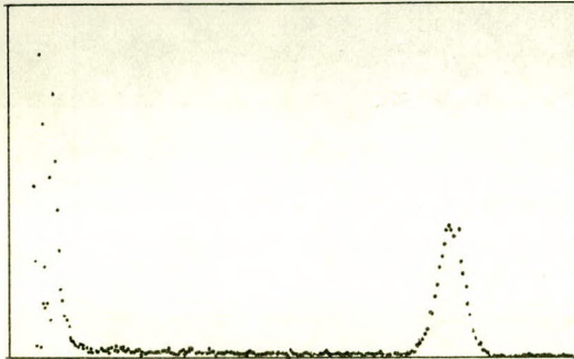
FIG 3A ^{14}\text{N}(\text{n,p})\text{C}^{14} PULSE-HEIGHT DISTRIBUTION FOR 2000 VOLTS BIAS
