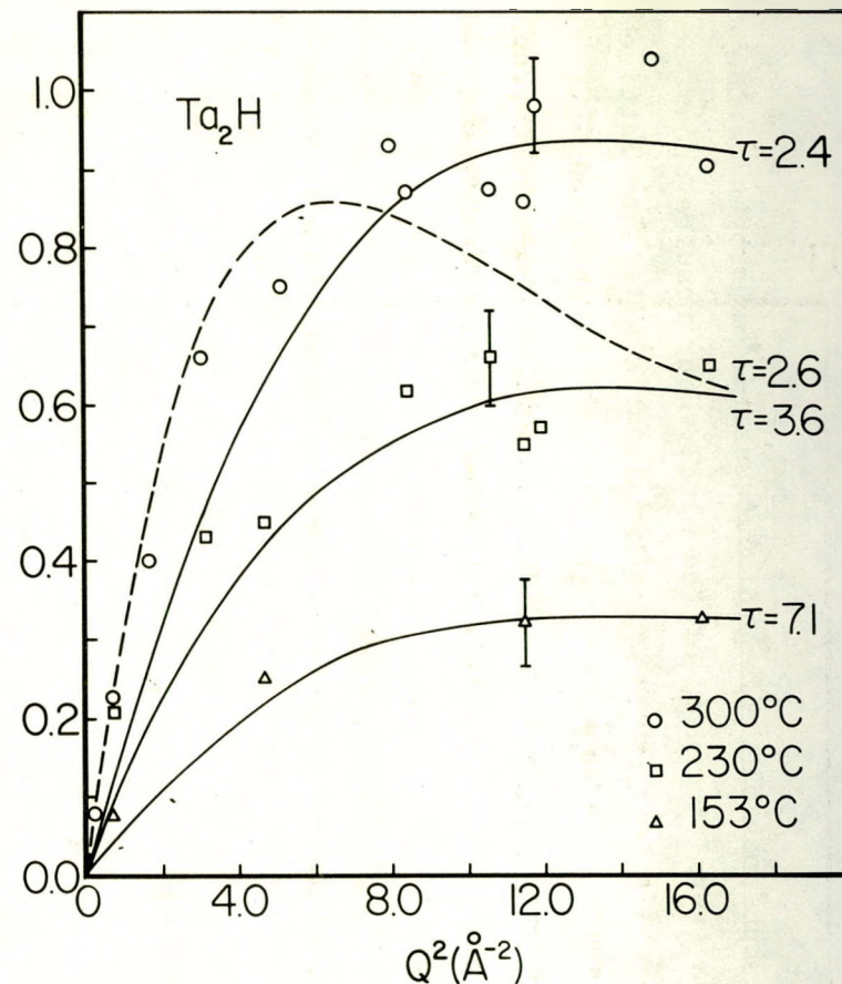
Fig. 1. The full widths at half-maximum ( \Delta\omega_{1/2}^L ) of single Lorentzians obtained for \text{TaH}_{0.15} and \text{Ta}_2\text{H} by deconvoluting the experimental quasielastic peaks into a Gaussian (resolution function) and a broadened Lorentzian. The solid and dashed lines are the theoretical widths predicted for instantaneous jumps between the tetrahedral and octahedral models, respectively. The \tau values derived from the best fit to the tetrahedral model at various temperatures are also shown.
