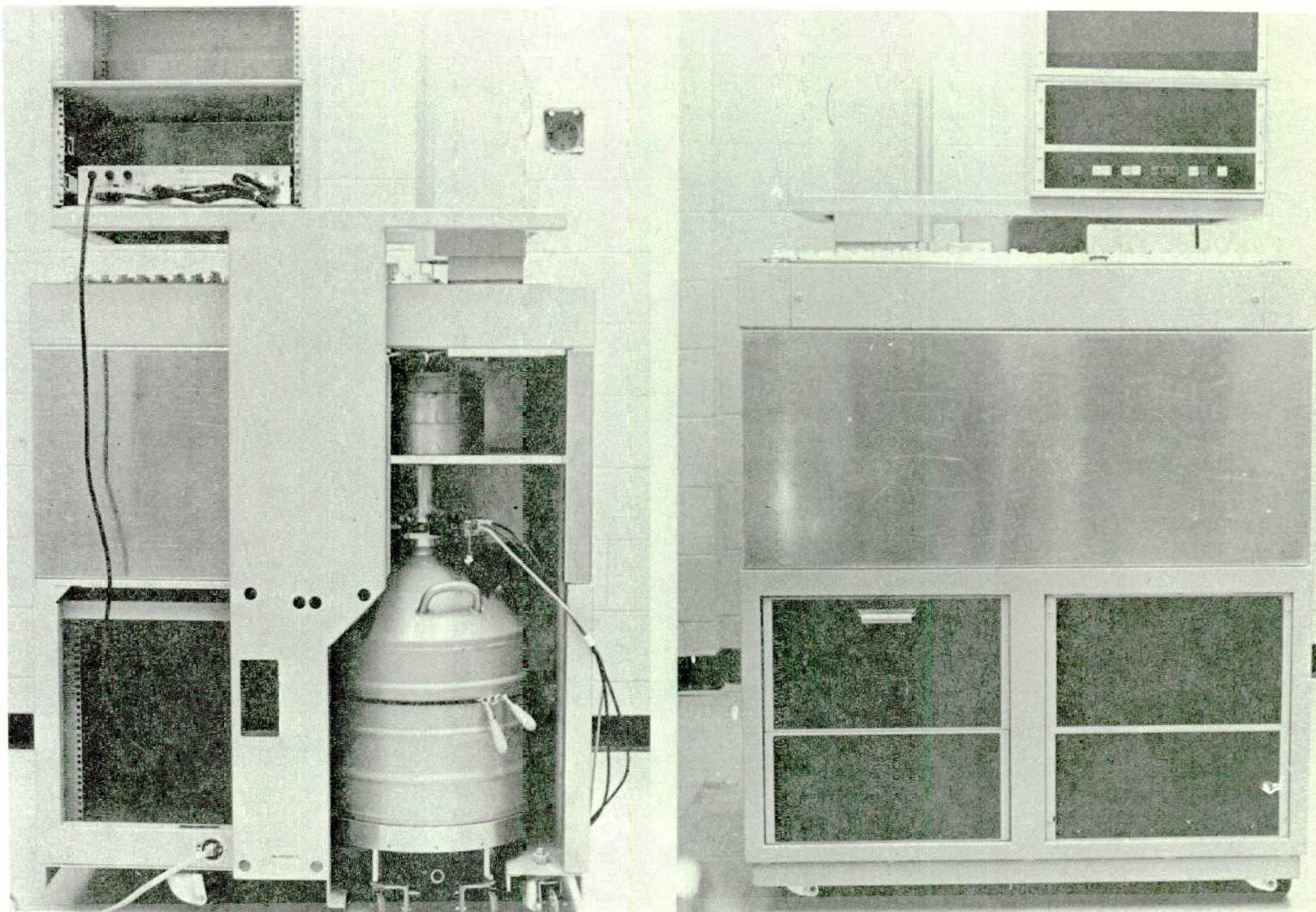
Fig. 1. Left: Rear view of sample changer with Ge(Li) detector in place. Right: Front view of sample changer showing steel insert in cabinet.
