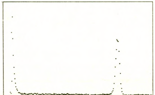
FIG 3D ^{14}\text{N}(\text{n,p})\text{C}^{14} PULSE-HEIGHT DISTRIBUTION FOR 2800 VOLT BIAS
