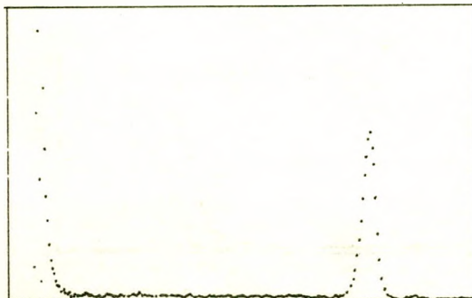
FIG 3C ^{14}\text{N}(\text{n,p})\text{C}^{14} PULSE-HEIGHT DISTRIBUTION FOR 2650 VOLT BIAS
