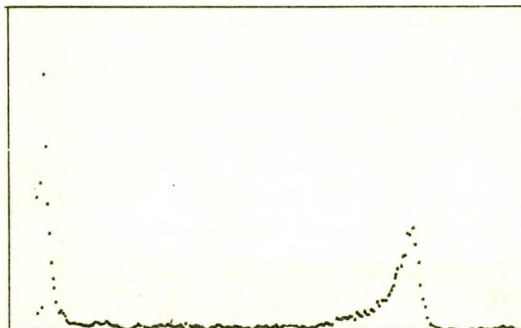
FIG 3E ^{14}\text{N}(\text{n,p})\text{C}^{14} PULSE-HEIGHT DISTRIBUTION FOR 3100 VOLTS BIAS
