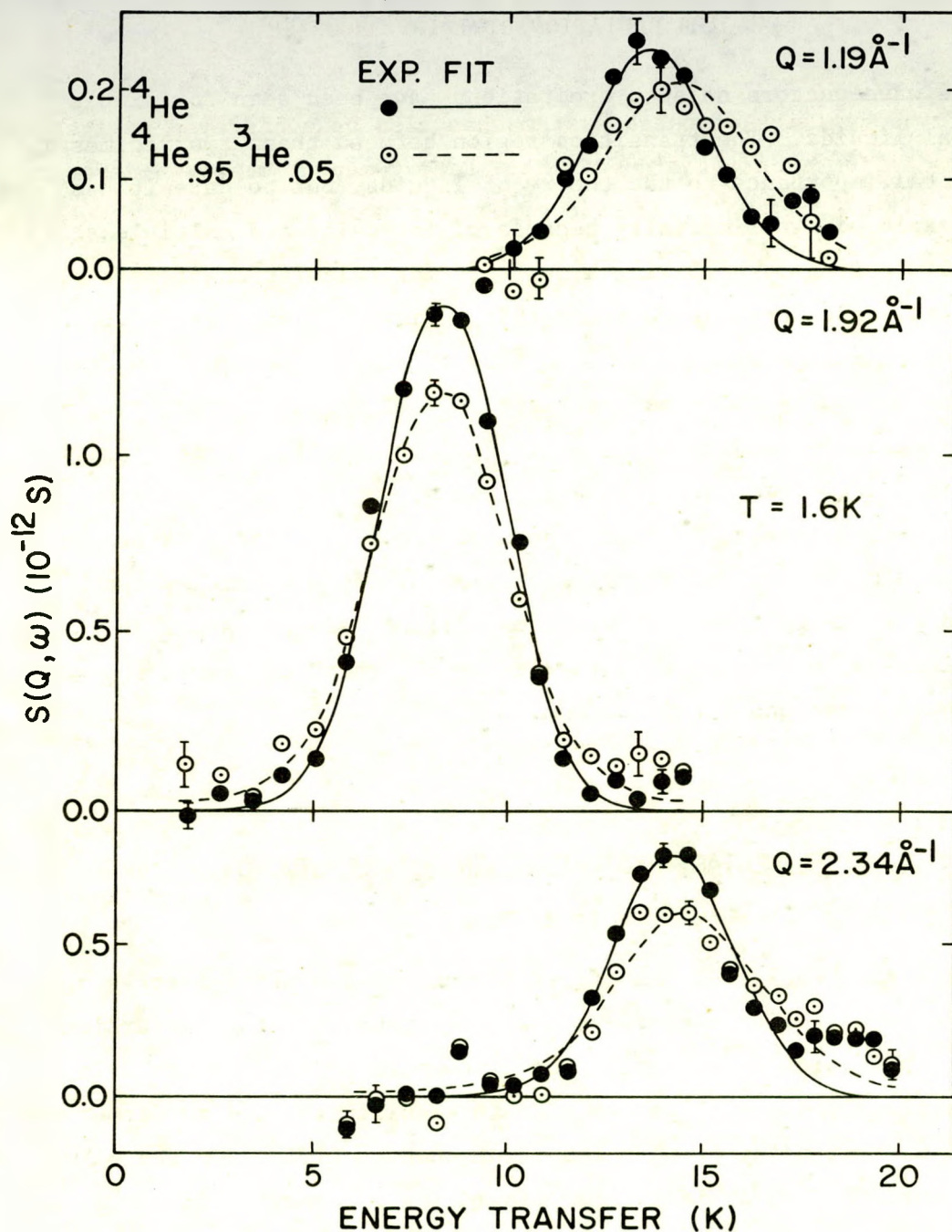
Fig. 1. The experimental scattering law data for ^4\text{He}(\bullet) and the ^4\text{He}_{.95}^3\text{He}_{.05}(0) liquids at three selected angles of scattering for a temperature of 1.6K. The solid and broken lines represent fits to the data which will not be discussed here. The value of wave vector transfer Q shown is determined at the energy corresponding to the peak.
