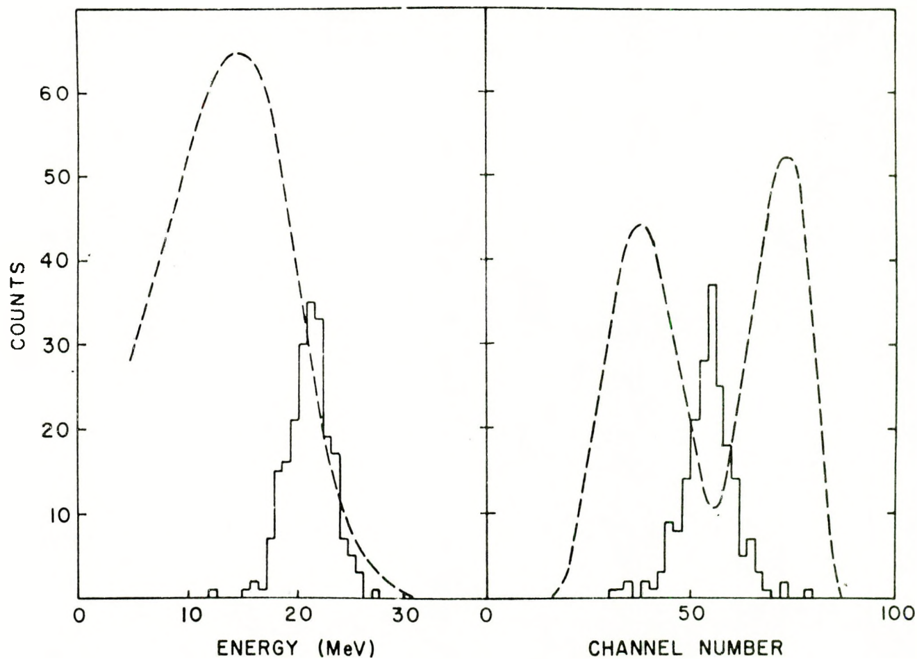
Fig. 2. Solid line represents A) Energy distribution of extreme-angle \alpha -particles B) Energy distribution of fission fragments associated with the emission of extreme-angle \alpha -particles. Broken lines represent corresponding distribution associated with normal emission of \alpha -particles.
