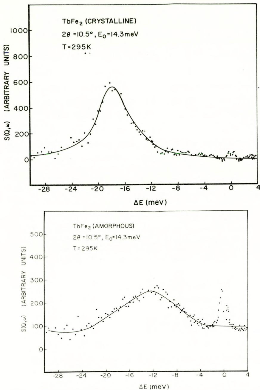
Fig. 1. Corrected time-of-flight spectra for polycrystalline (a) and amorphous (b) \text{TbFe}_2 at room temperature.
