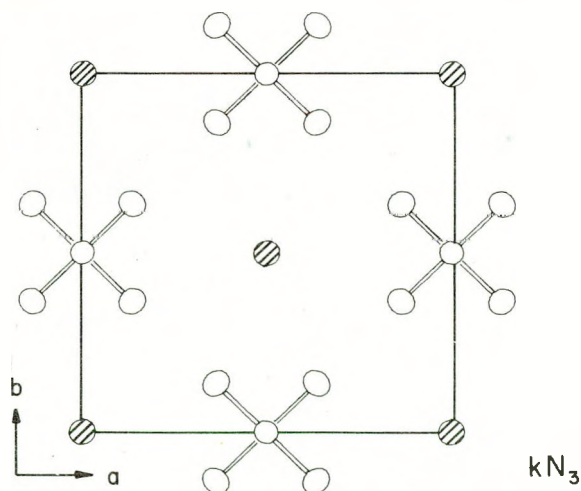
Fig. 1. Crystal structure of \text{KN}_3 projected along c-axis.
