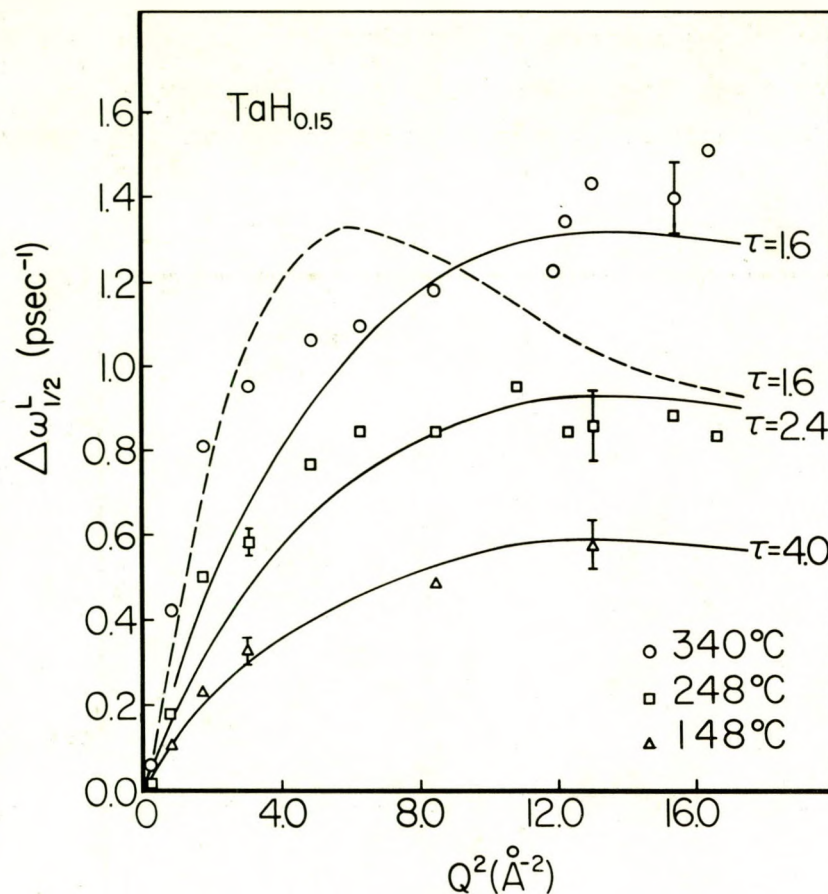
Fig. 1. The full widths at half-maximum ( \Delta\omega_{1/2}^L ) of single Lorentzians obtained for \text{TaH}_{0.15} and \text{Ta}_2\text{H} by deconvoluting the experimental quasielastic peaks into a Gaussian (resolution function) and a broadened Lorentzian. The solid and dashed lines are the theoretical widths predicted for instantaneous jumps between the tetrahedral and octahedral models, respectively. The \tau values derived from the best fit to the tetrahedral model at various temperatures are also shown.
