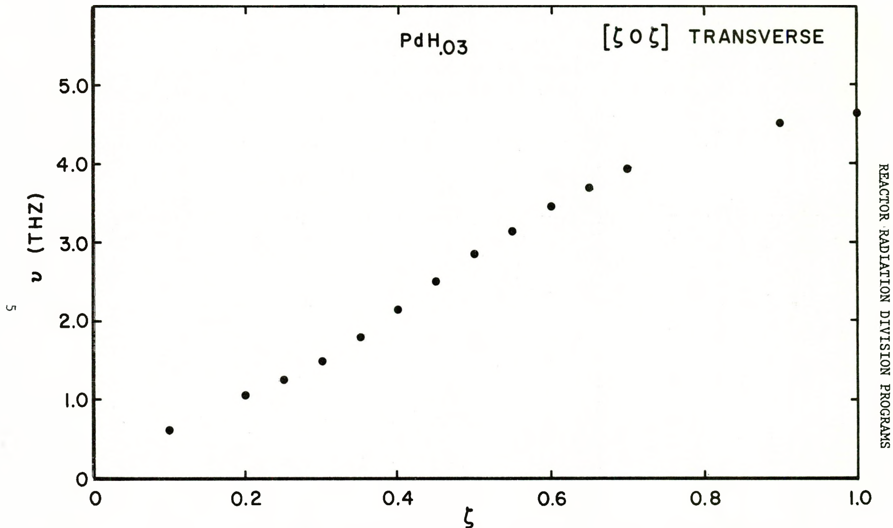
Fig. 2. The frequency vs wave-vector dispersion relation for the \text{PdH}_{0.03} transverse ( T_1 ) branch propagating in the [110] direction. The results for pure palladium are not shown, as they would be indistinguishable from the \text{PdH}_{0.03} result on this scale.
