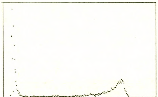
FIG 3F ^{14}\text{N}(\text{n,p})\text{C}^{14} PULSE-HEIGHT DISTRIBUTION FOR 3300 VOLTS BIAS
