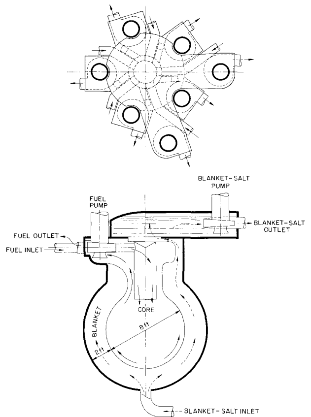
Fig. 1.1.5. MSR Layout with Fuel Return Ducts at the Same Place as the Fuel Discharge Ducts.
