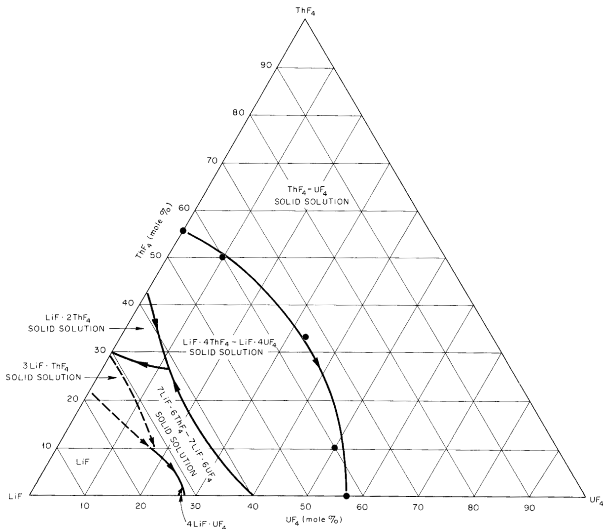
Fig. 2.3.10. The Primary-Phase Fields in the System \text{LiF}-\text{ThF}_4-\text{UF}_4 .
