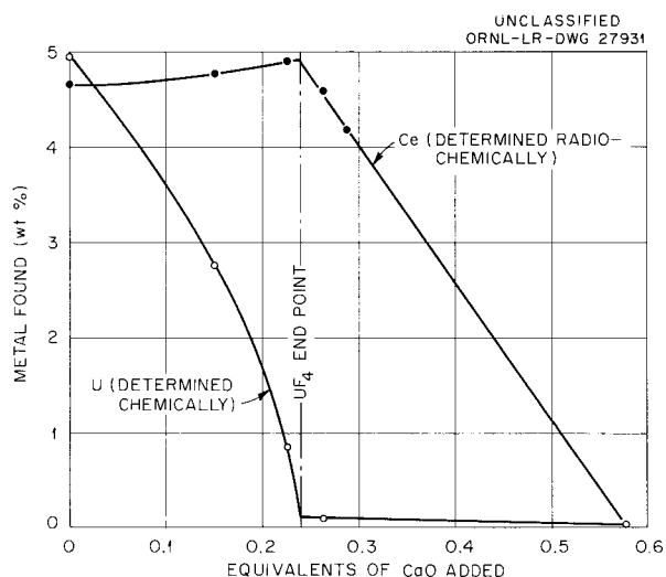
Fig. 2.3.22. Titration of \text{CeF}_3 and \text{UF}_4 with \text{CaO} in \text{LiF-KF} (50-50 Mole %).
