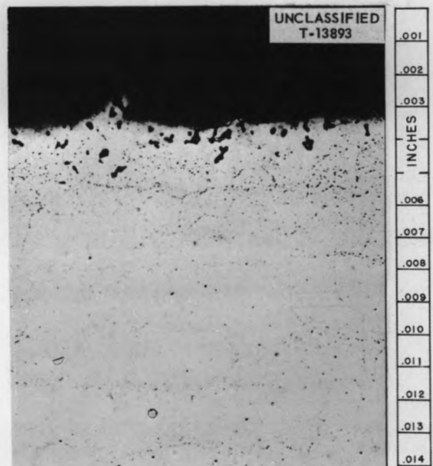
Fig. 2.1.5. Specimen Taken from Hot Leg of Inconel Thermal-Convection Loop 1171 at Point of Maximum Loop Temperature. 250X.
