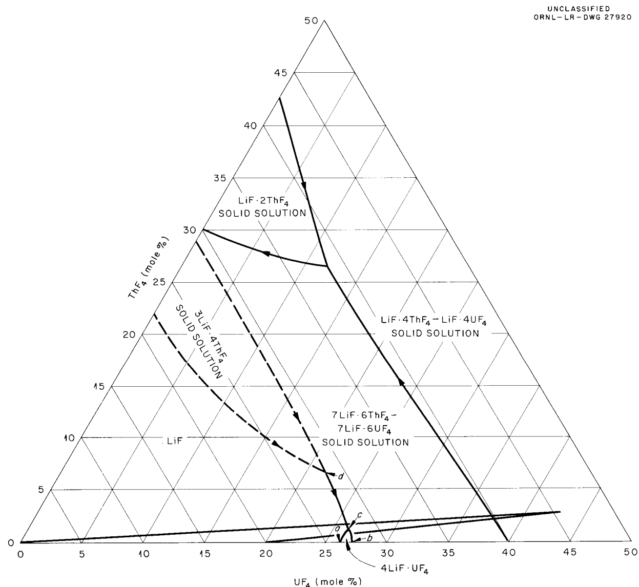
Fig. 2.3.11. Primary-Phase Fields in the System LiF-ThF 4 -UF 4 for the Region Representing Mixtures Containing 50 to 100 Mole % LiF.
