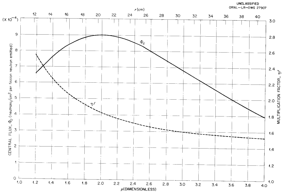
Fig. 1.4.5. Central Flux and Multiplication Factor as Functions of Shell Radius of Idealized Flux Trap Reactor with a BeO Moderator.
