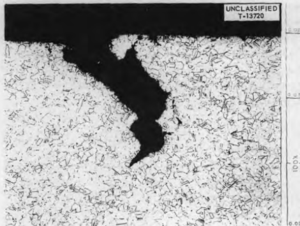
Fig. 2.1.38. Specimen Showing a Crack Found in Weld Area of Weld drawn INOR-8 Tubing. Etchant: aqua regia. 100X. Reduced 31%.
