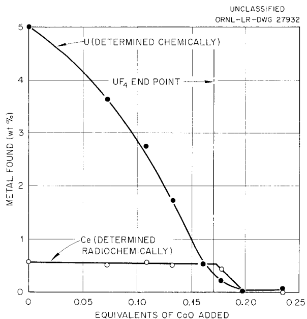
Fig. 2.3.23. Titration of \text{CeF}_3 and \text{UF}_4 with \text{CaO} in \text{LiF-KF} (50-50 Mole %).
