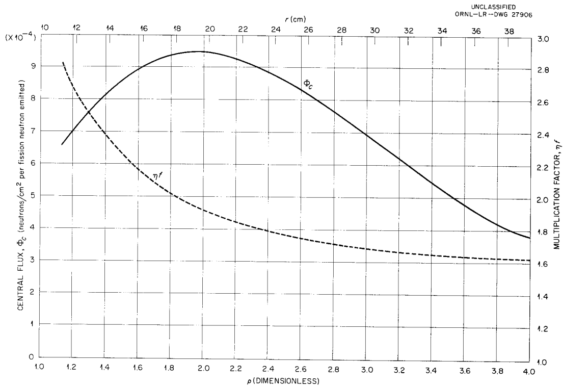
Fig. 1.4.4. Central Flux and Multiplication Factor as Functions of Shell Radius of Idealized Flux Trap Reactor with a Be Moderator.
