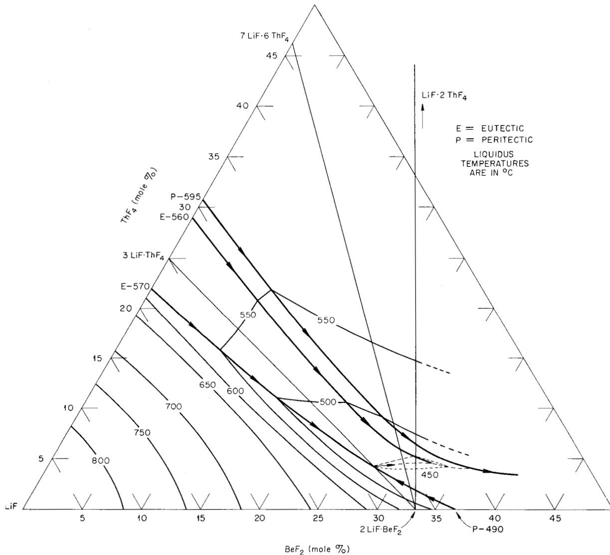
Fig. 2.3.1. Partial Phase Diagram of the System \text{LiF} - \text{BeF}_2 - \text{ThF}_4 for the Region Representing Mixtures Containing 50 to 100 Mole % \text{LiF} .
