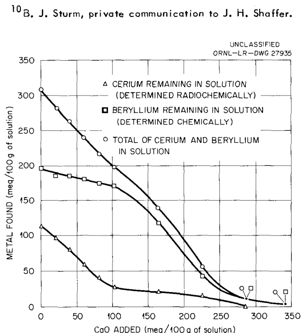
Fig. 2.3.26. Titration of \text{CeF}_3 and \text{BeF}_2 with \text{CaO} in \text{LiF-KF} (50-50 Mole %).
