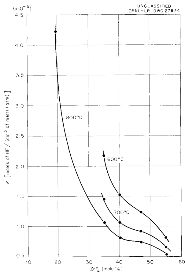
Fig. 2.3.15. Henry's Law Constants for HF Solubility in NaF- \text{ZrF}_4 Mixtures as a Function of Solvent Composition.
