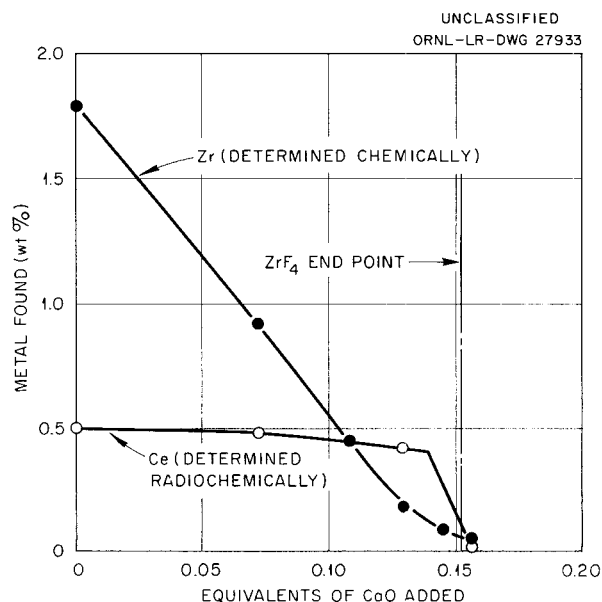
Fig. 2.3.24. Titration of \text{CeF}_3 and \text{ZrF}_4 with \text{CaO} in \text{LiF-KF} (50-50 Mole %).
