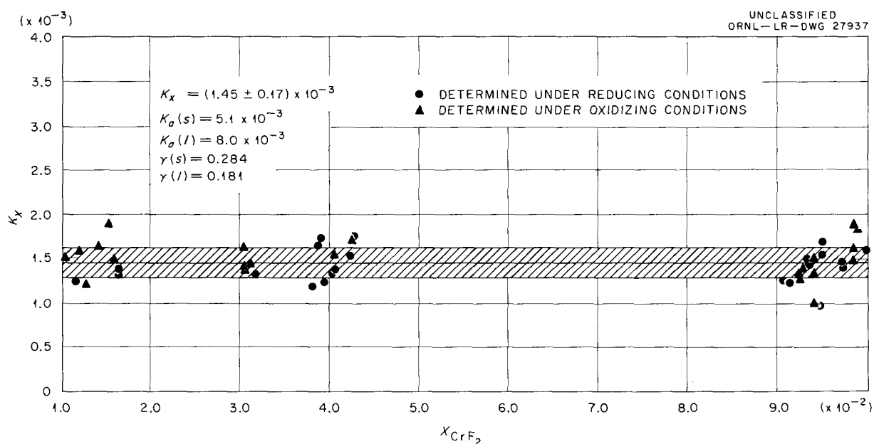
Fig. 2.3.28. Equilibrium Quotients at 850°C of the Reaction \text{CrF}_2(d) + \text{H}_2(g) \rightleftharpoons \text{Cr}(s) + 2\text{HF}(g) in \text{NaF-ZrF}_4 (53-47 Mole %).
