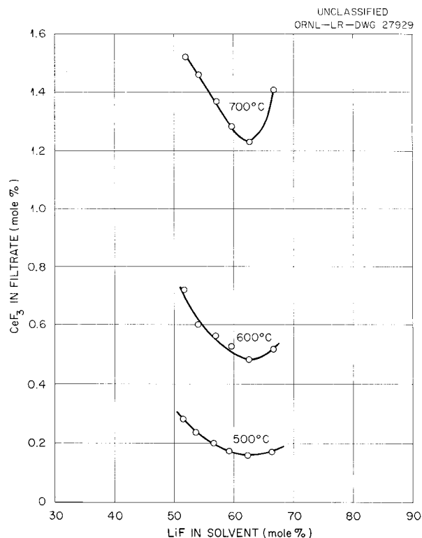
Fig. 2.3.20. Solubility of CeF 3 in Various LiF·BeF 2 Solvents.
