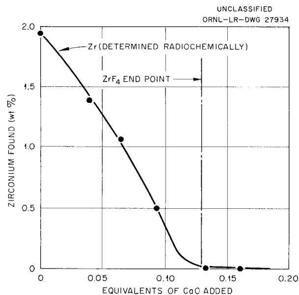
Fig. 2.3.25. Titration of \text{ZrF}_4 in the Presence of \text{CeF}_3 with \text{CaO} in \text{LiF-KF} (50-50 Mole %).
