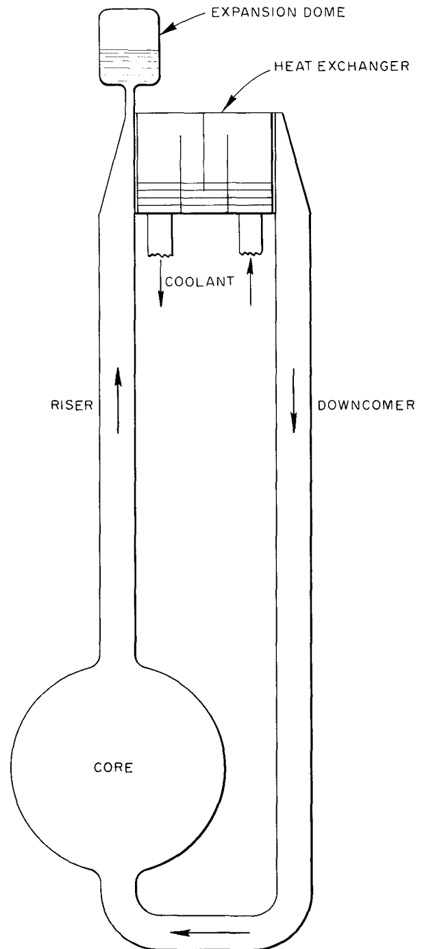
Fig. 1.4.1. Schematic Diagram of a Molten Salt Natural-Convection Reactor.
