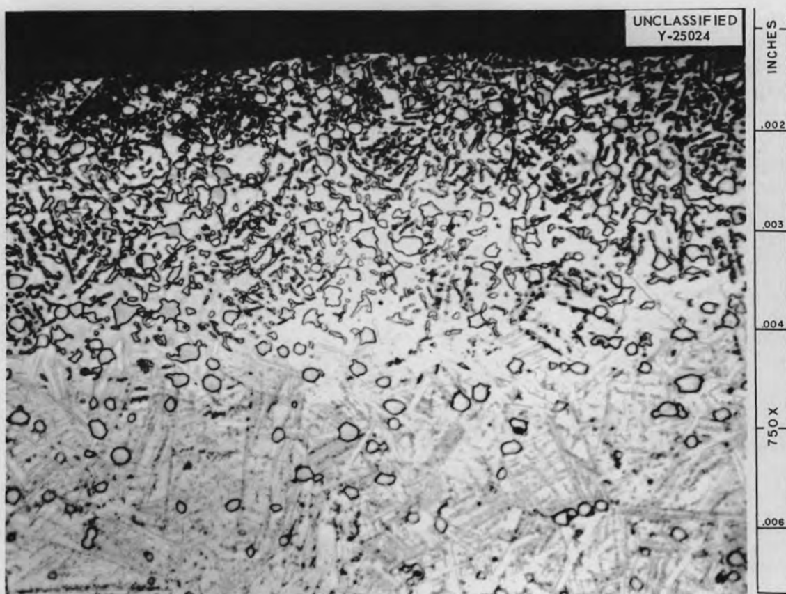
Fig. 2.1.8. Hastelloy B After Exposure to Fuel 30 Containing 25 wt % Graphite at 1500°F for 500 hr. Etchant: chromic and hydrochloric acids. 750X.
