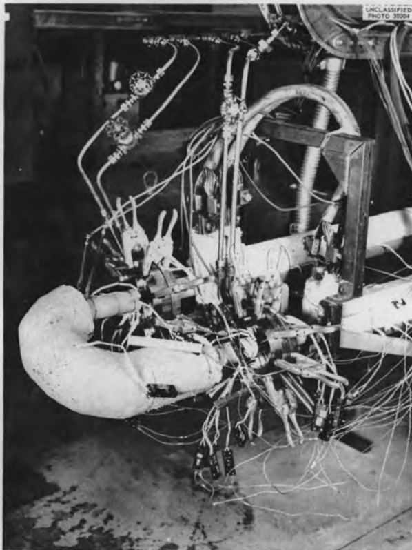
Fig. 1.2.3. Freeze-Flange Joints in Test Loop.
