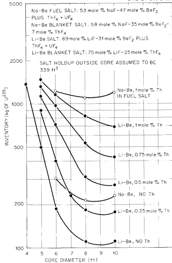
Fig. 1.1.9. Clean, Critical Inventory of U 235 for 600-Mw Reactors Fueled with Lithium-Beryllium- or with Sodium-Beryllium-Base Salts.
