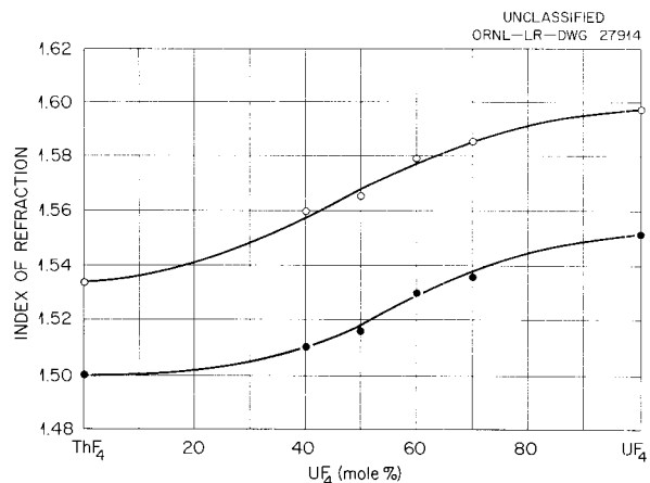
Fig. 2.3.5. Indices of Refraction in the System ThF 4 -UF 4 .
