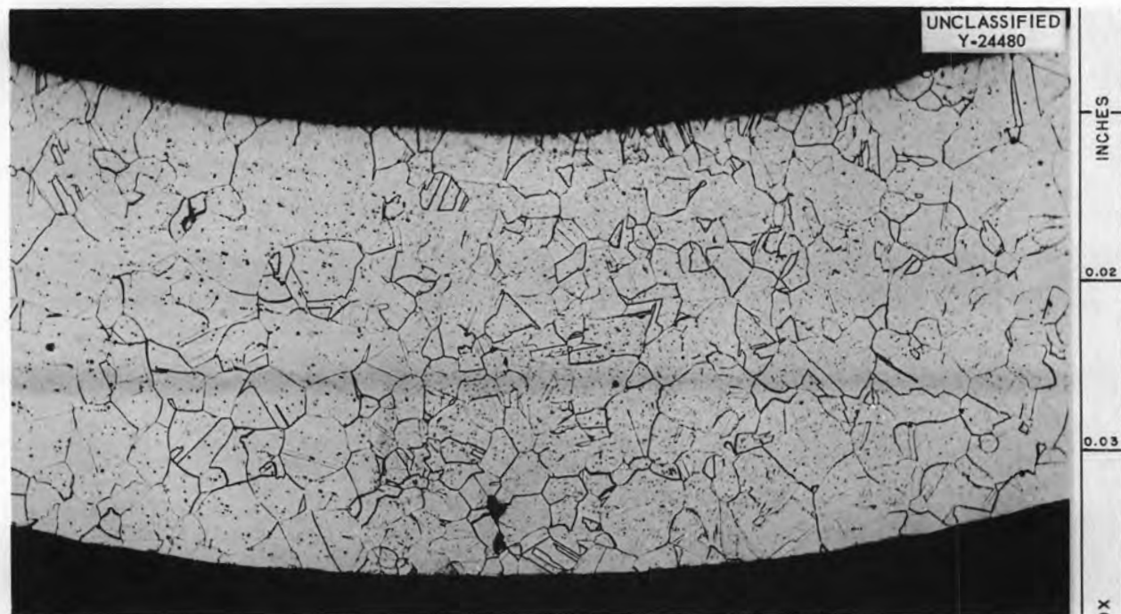
Fig. 2.1.36. Subsurface Void Found by Immersed Ultrasound Inspection of \frac{1}{2} -in.-OD, 0.045-in.-Wall INOR-8 Tubing. Etchant: chromic and hydrochloric acids. 100X.
