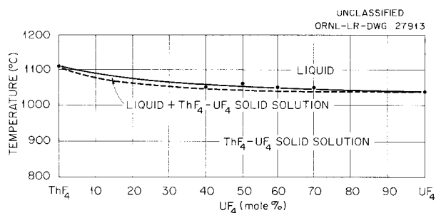
Fig. 2.3.4. The System ThF 4 -UF 4 .
