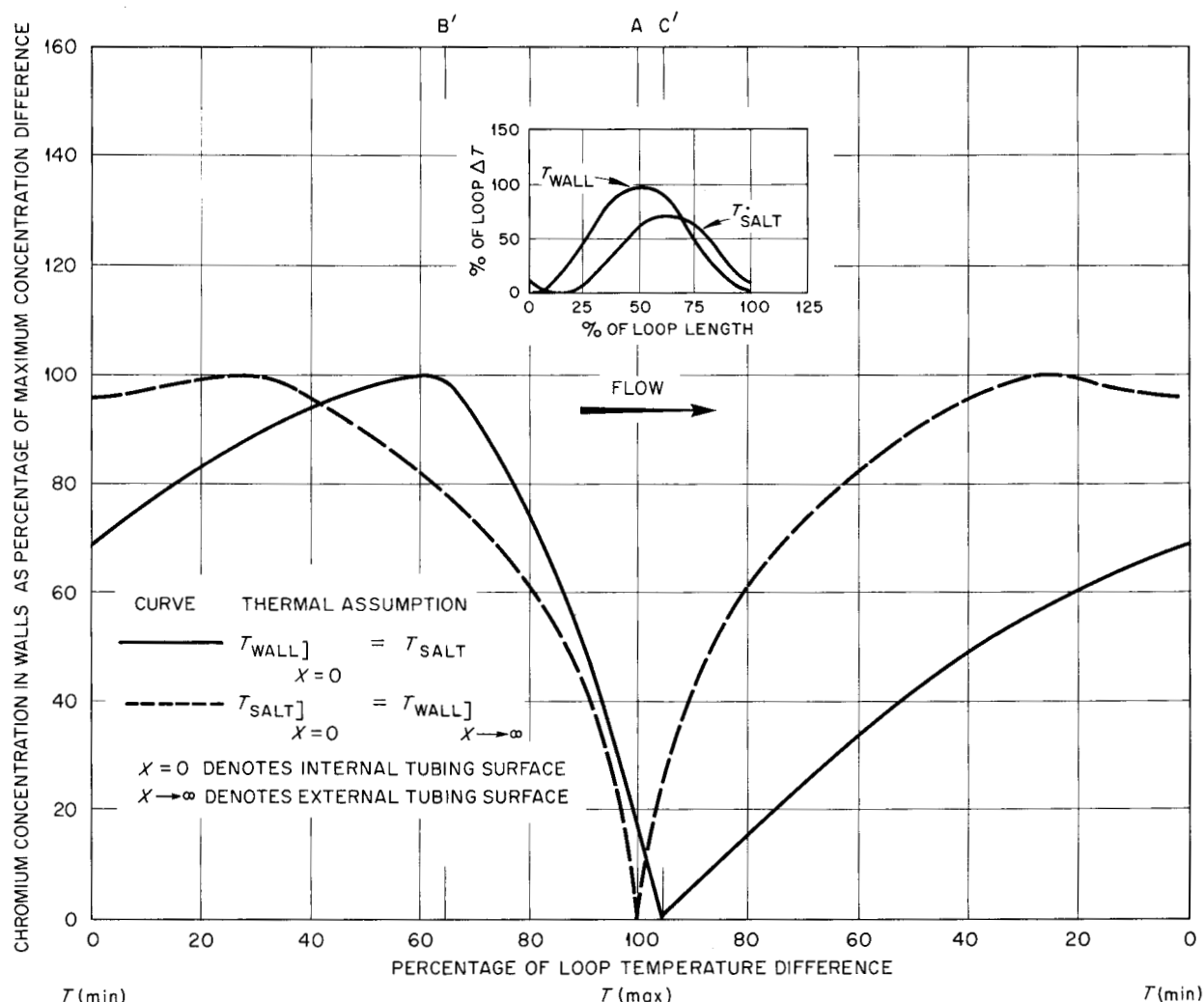
Fig. 2.3.31. Calculated Loop Wall Distribution of Chromium After Diffusion-Controlled UF_4 - UF_3 Corrosion of Inconel.
