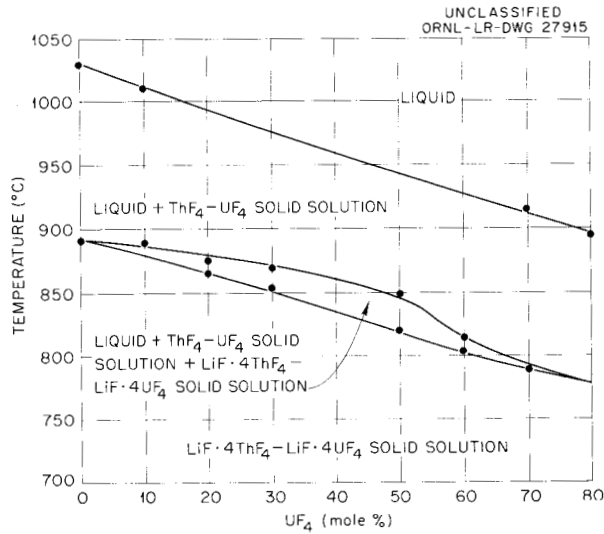
Fig. 2.3.6. The Join \text{LiF} \cdot 4\text{ThF}_4 - \text{LiF} \cdot 4\text{UF}_4 .
