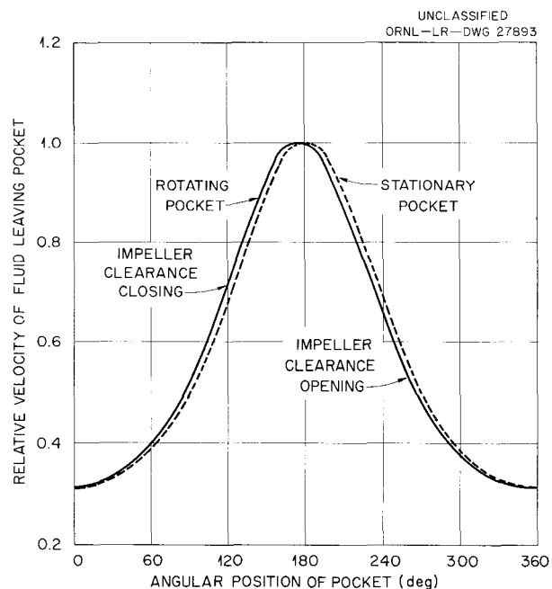
Fig. 1.1.11. Comparison of Velocities of Fluid Leaving Pockets of Stationary and Rotating Hydrostatic Bearing Systems.
