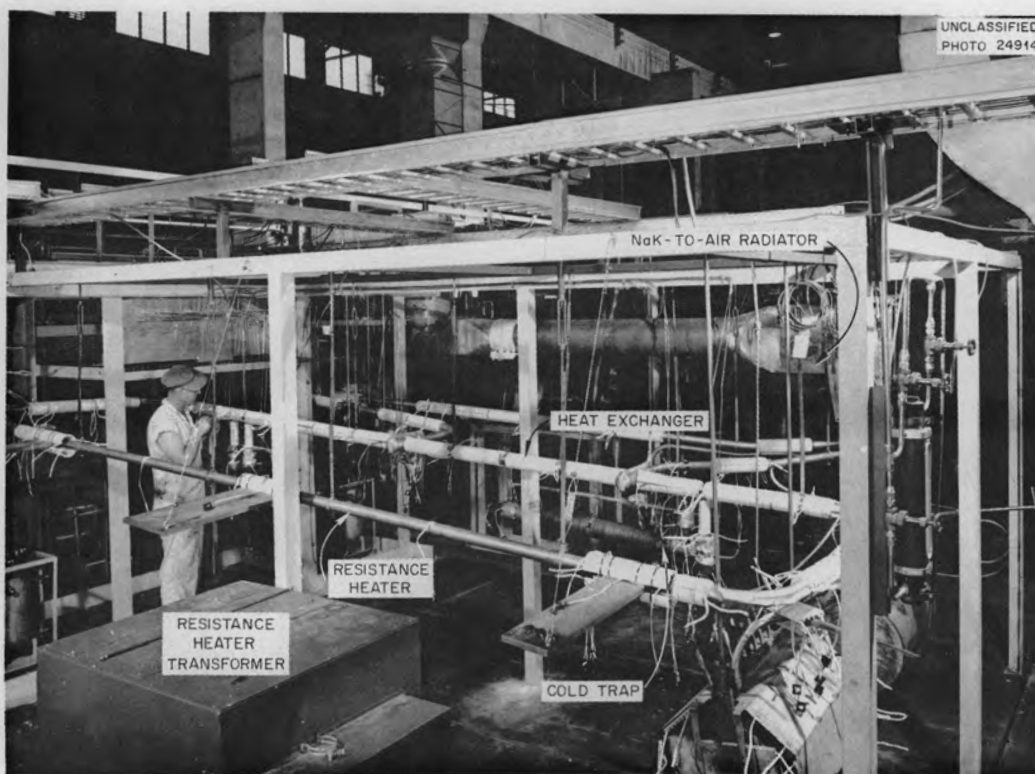
Fig. 1.2.14. Piping Arrangement of Small Heat Exchanger Test Stand C.
