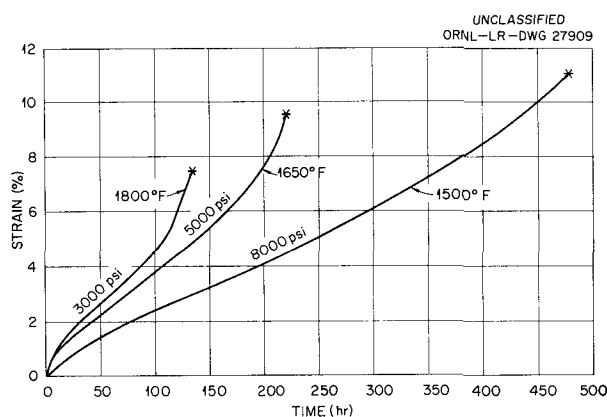
Fig. 2.1.16. Creep Curves for Solution-Annealed INOR-8 Tested in Fuel 107 at Various Temperatures and Stresses.
