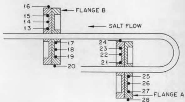
Fig. 1.2.4. Locations of Thermocouples on Freeze-Flange Joints.
