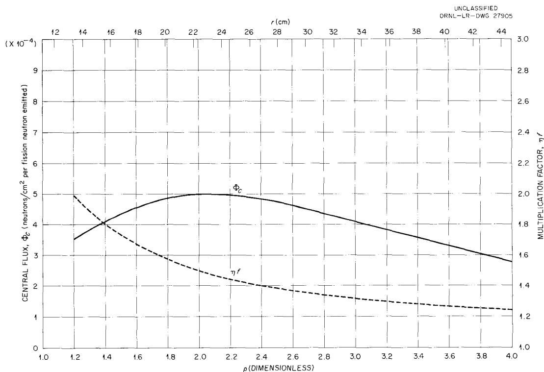
Fig. 1.4.3. Central Flux and Multiplication Factor as Functions of Shell Radius of Idealized Flux Trap Reactor with a D 2 O Moderator.
