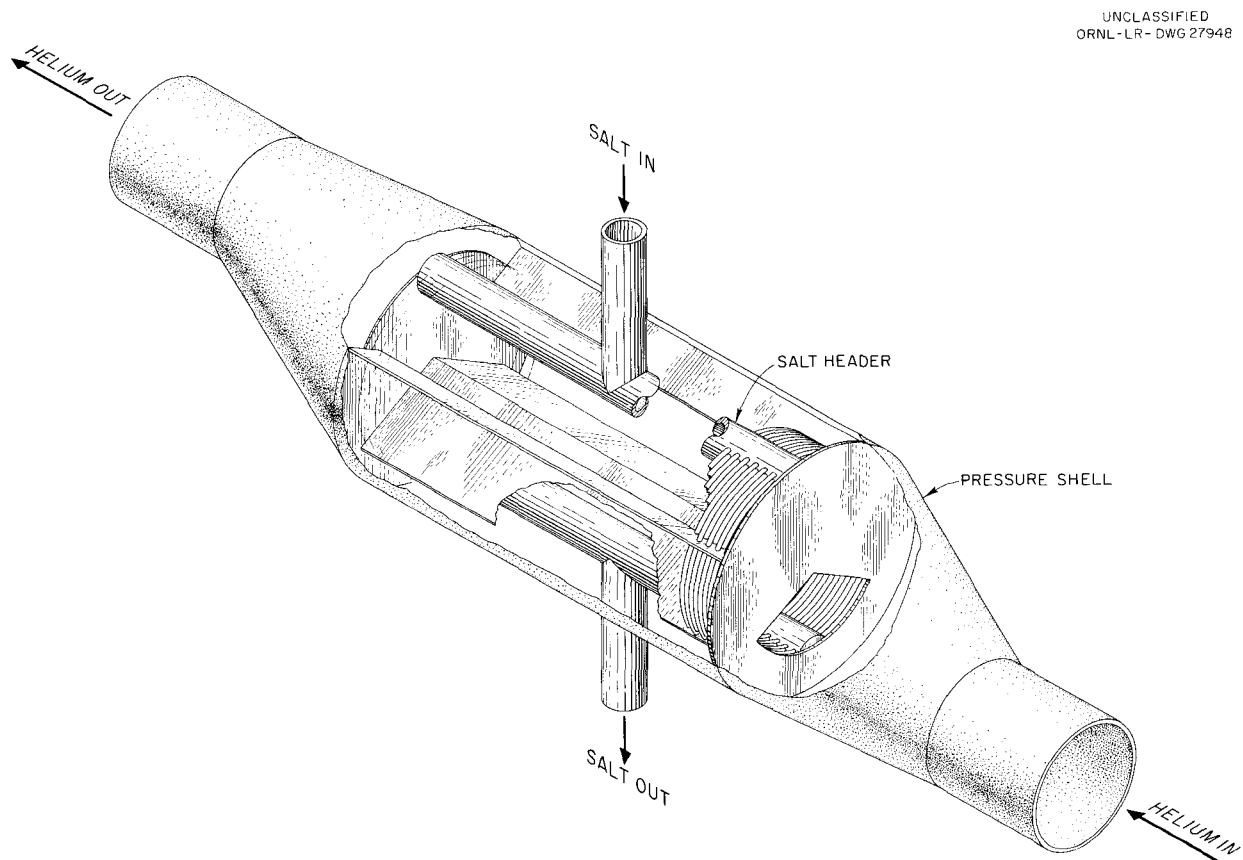
Fig. 1.4.2. Schematic Diagram of a Possible Fuel-Salt-to-Helium Heat Exchanger with Three Gas Passes.
