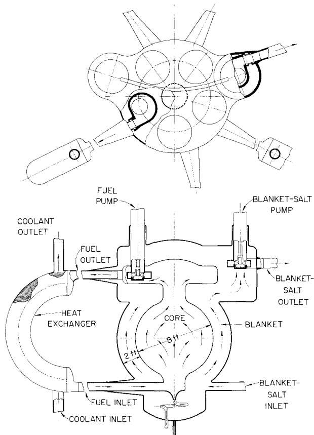
Fig. 1.1.4. Single-Pass MSR Layout.
