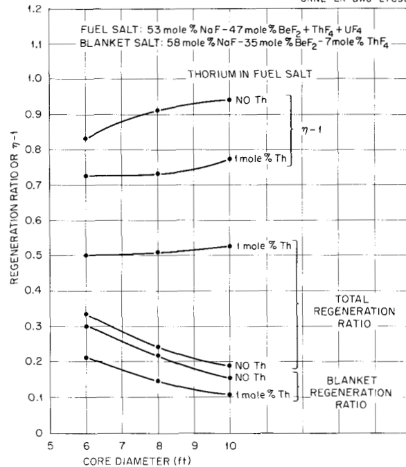
Fig. 1.1.10. Initial Regeneration Characteristics of Molten Salt Reactors Fueled with Sodium-Beryllium-Base Salts Containing U 235 .
