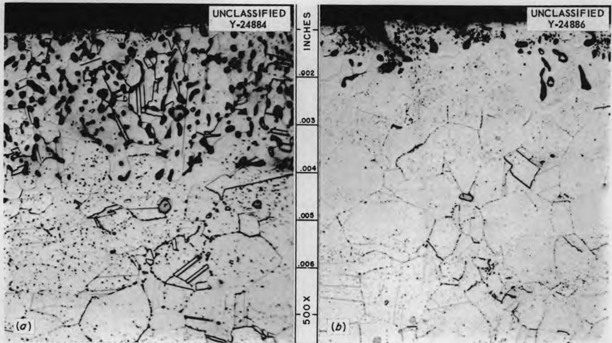
Fig. 2.1.11. (a) Specimen from Position 17 of Loop 30; (b) Specimen from Position 17 of Loop 39. Etchant: aqua regia. 500X.
