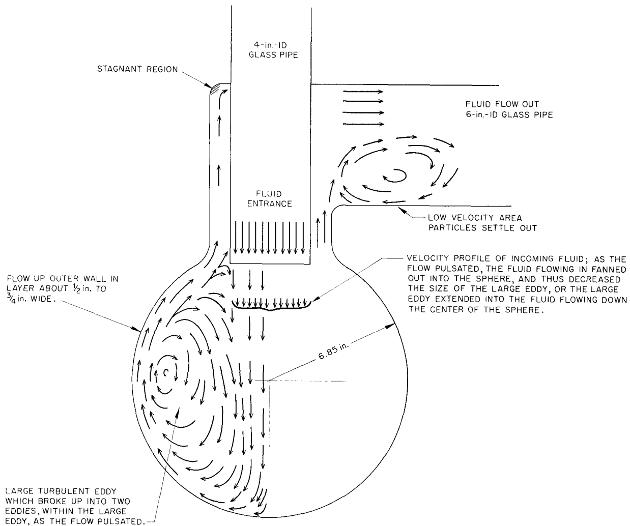
Fig. 1.3.3. Flow Patterns Observed Within an Illuminated Plane of the Concentric Entrance-Exit Core Model with Fluid Entering Through Inner Pipe.
