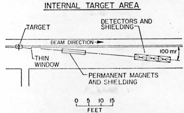
Fig. 1. Layout of the apparatus in the Internal Target Laboratory at NAL to study photon production in proton-proton collisions.
