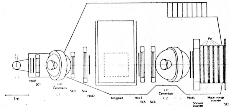
Fig. 8. Layout of the British-Scandinavian spectrometer at the ISR for the study of particle composition at intermediate transverse momentum.
