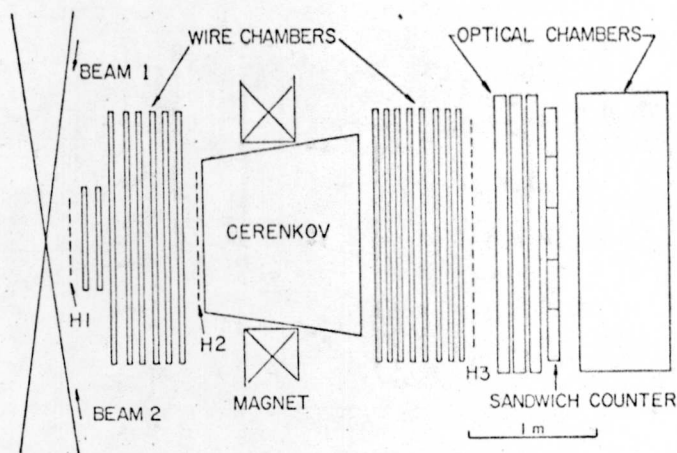
Fig. 10. Experimental layout of the Saclay-Strasbourg spectrometer at the ISR to study large transverse momentum particle production.
