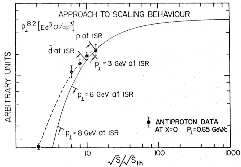
Fig. 20. The function F(p_1/\sqrt{s}) = p_1^{8.2} E(d^3 \sigma/dp^3) is shown as the solid curve versus \sqrt{s}/\sqrt{s_{th}} where \sqrt{s_{th}} = 2p_1 . The data points are for antiproton production and have been normalized to the curve at the highest energy. In this case \sqrt{s_{th}} is the center-of-mass threshold energy for antiproton production. The dashed curve is a guide to the eye through the antiproton data points.
