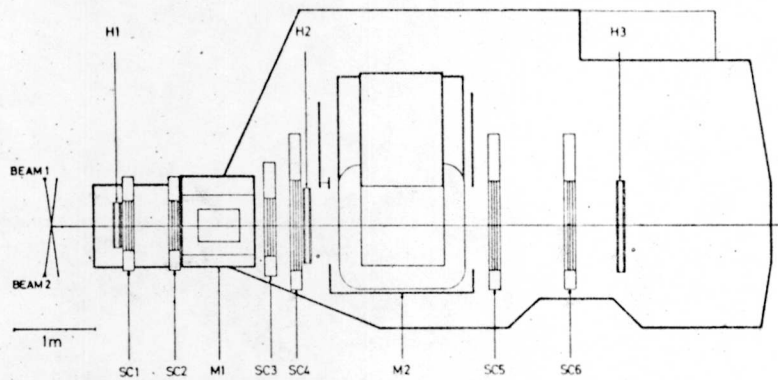
Fig. 5. Layout of the British-Scandinavian spectrometer at the ISR for the study of particle production at high transverse momentum.
