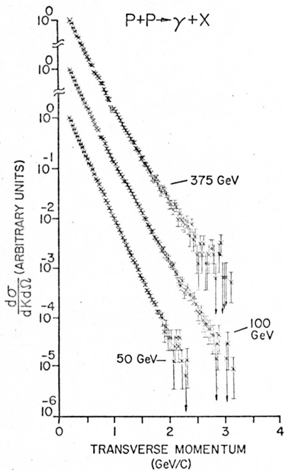
Fig. 3. Single photon inclusive cross section d\sigma/d\Omega dk versus transverse momentum for 50, 100, and 375 GeV incident protons.
