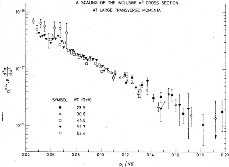
Fig. 16. The function F(p_{\perp}/\sqrt{s}) = p_{\perp}^n E (d^3\sigma/dp^3) , as deduced from the measurements, using the best fit value n = 8.24 . The errors are statistical only.
