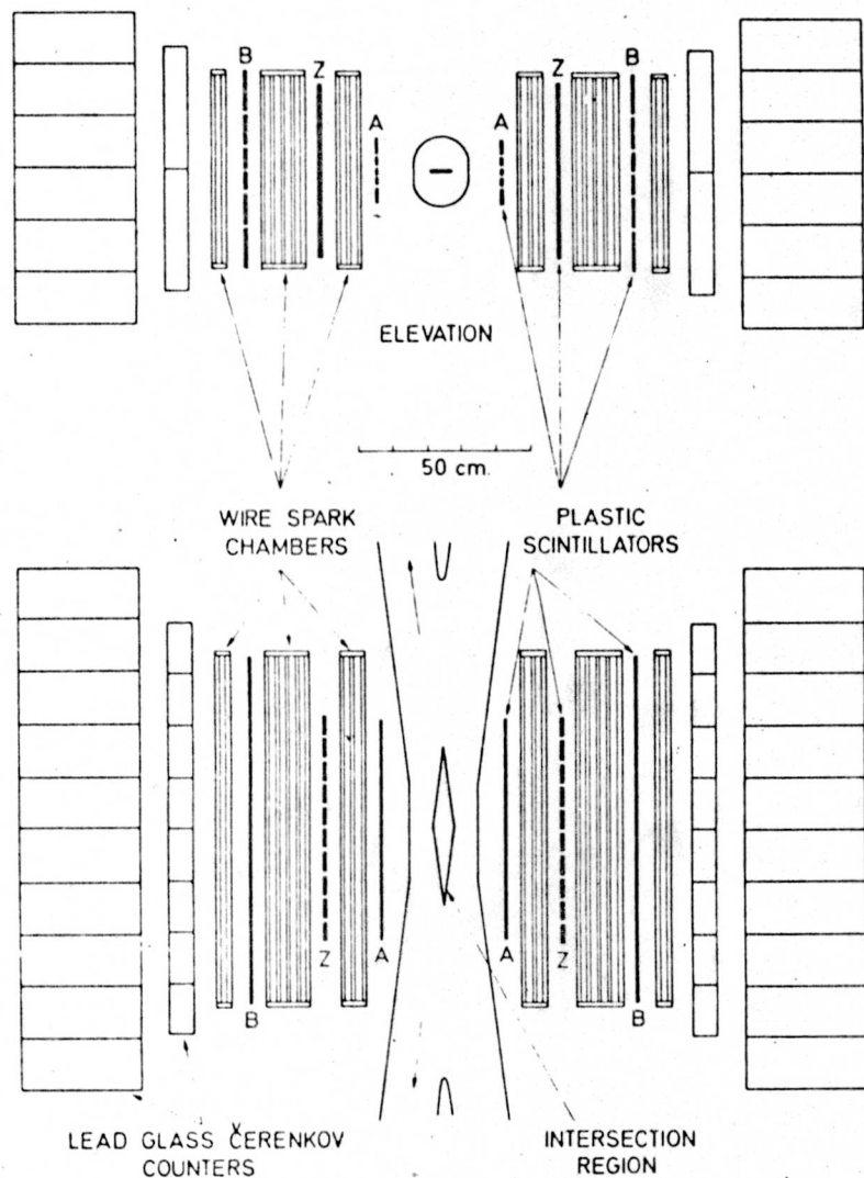
Fig. 14. Schematic of the CERN-Columbia-Rockefeller apparatus at the ISR.
