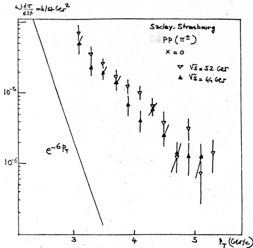
Fig. 11. Charged pion distribution at large p_T .
