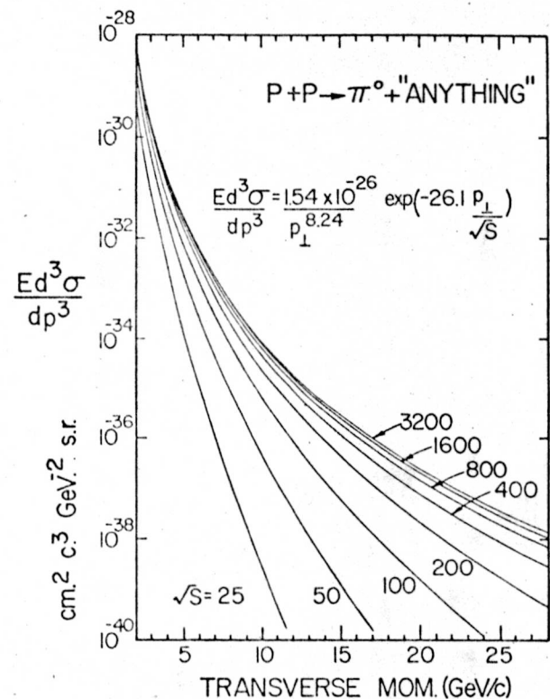
Fig. 17. The transverse momentum dependence of the \pi^0 inclusive invariant cross section at various center-of-mass energies using the CCR fitted function.
