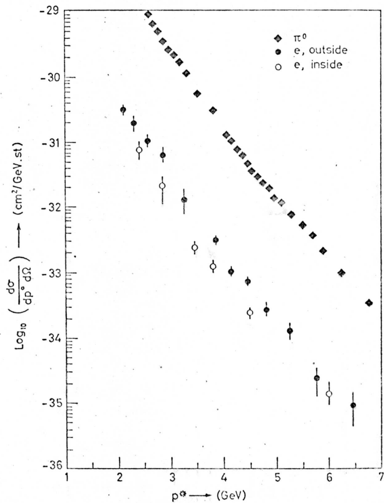
Fig. 18. Cross section for single electron production deduced from the two spectrometers. The \pi^0 cross section is also shown for comparison purposes.
