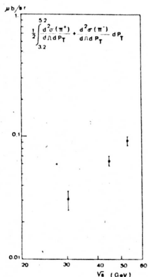
Fig. 13. Integrated pion yield 3.2 < p_{\perp} < 5.2 GeV/c at 90^\circ as a function of center-of-mass energy.
