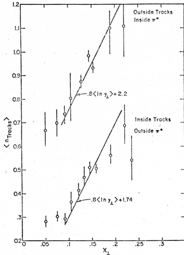
Fig. 22. The associated mean charged track multiplicity of the "jet" opposite the detected \pi^0 as a function of \pi^0 normalized transverse momentum. The curves are predictions of a parton model.
