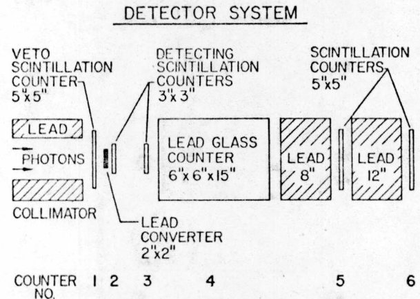
Fig. 2. Schematic of the photon detection apparatus.
