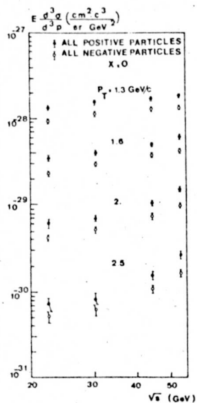
Fig. 12. Invariant charged pion cross sections at different p_{\perp} as a function of center-of-mass energy.
