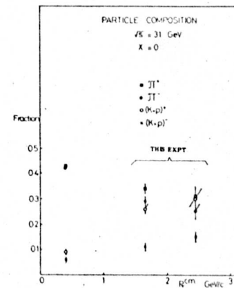
Fig. 9. Particle composition as a function of transverse momentum.
