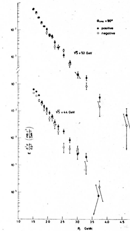
Fig. 6. Inclusive charge particle spectra at 90^\circ in the center of mass for \sqrt{s} = 44 and 53 GeV.
