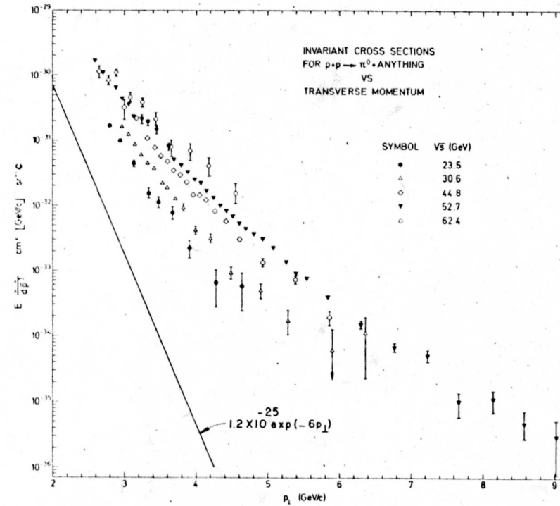
Fig. 15. The transverse momentum dependence of the \pi^0 inclusive invariant cross section at five center-of-mass energies. The errors are statistical only.
