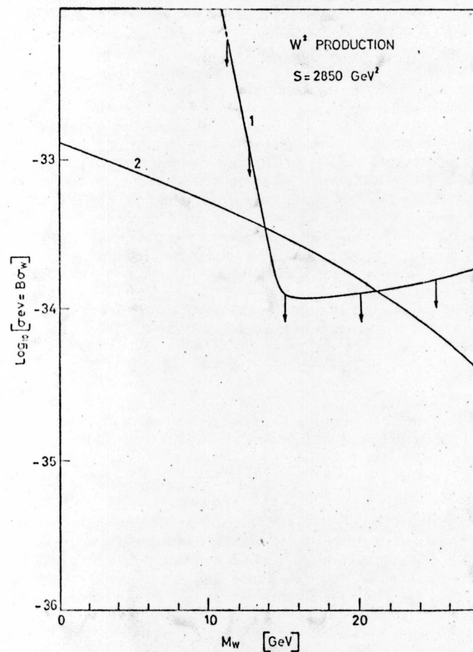
Fig. 19. Curve 1 is the cross section upper limit for charged intermediate bosons. Curve 2 is a possible lower bound prediction for charged intermediate boson production.
