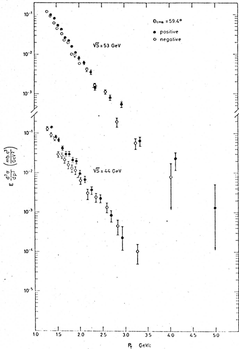
Fig. 7. Inclusive charge particle spectra at 59.4^\circ in the center of mass for \sqrt{s} = 44 and 53 GeV.
