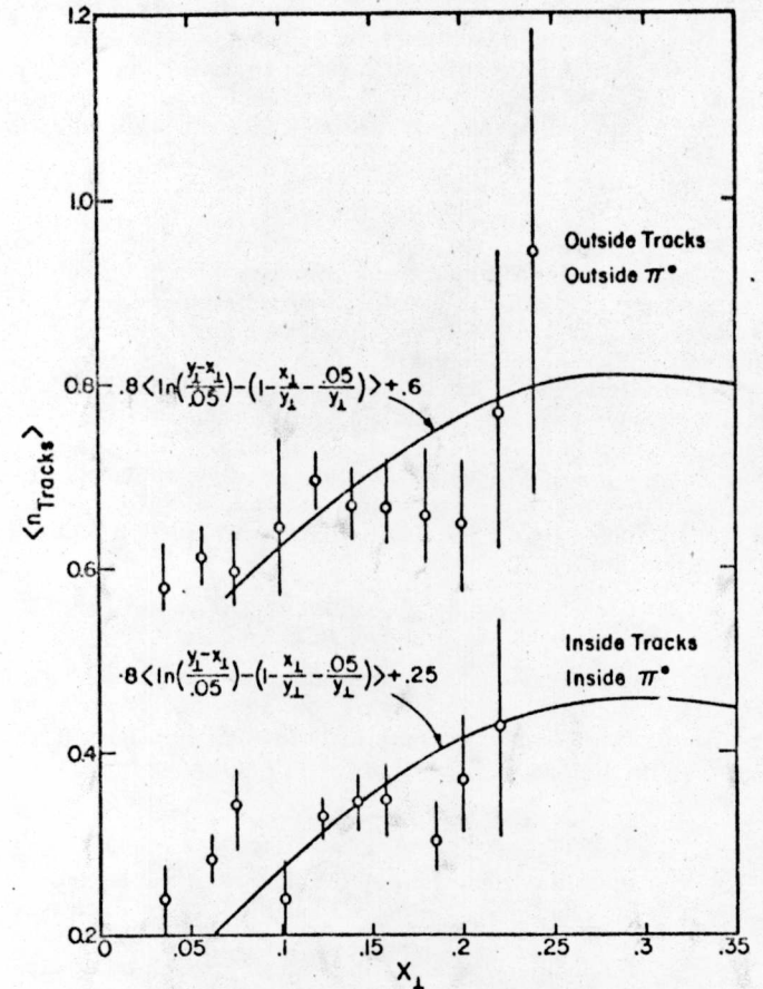
Fig. 23. The associated mean charged track multiplicity of the "jet" in the same direction as the detected \pi^0 as a function of \pi^0 normalized transverse momentum. The curves are predictions of a parton model.
