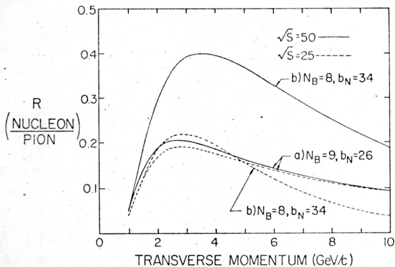
Fig. 21. The predicted general form of the baryon to pion ratio of inclusive cross sections at large momentum transfer. The different curves are for two different values of the parameters N_B and b_N at two different center-of-mass energies.
