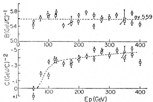
Fig. 4. Values of the parameters B and C for the photon cross sections. The circles and squares are for the hydrogen and carbon target data respectively.
