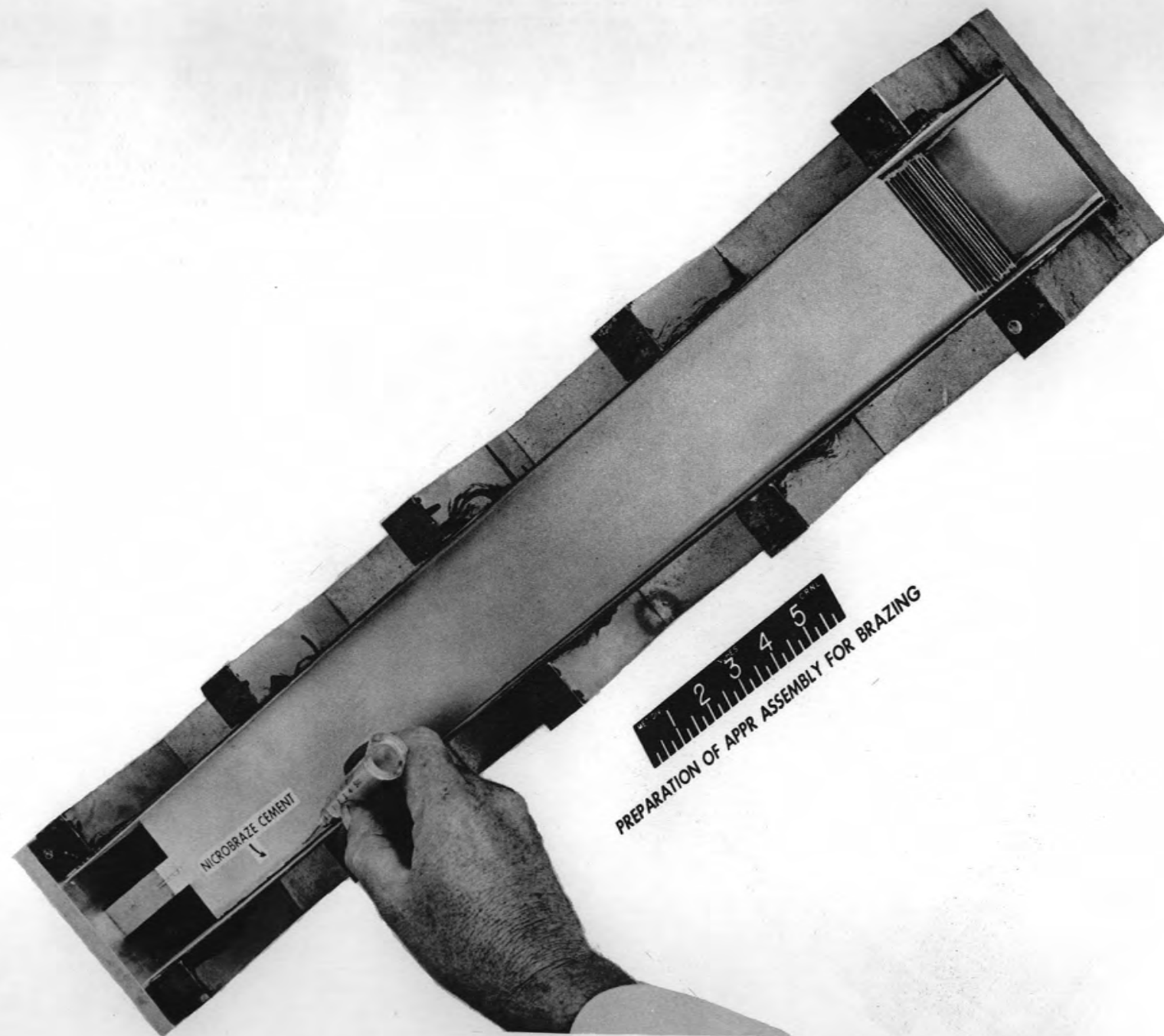
Fig. 23 (Y-25952) Application of Microbrazing Cement.
