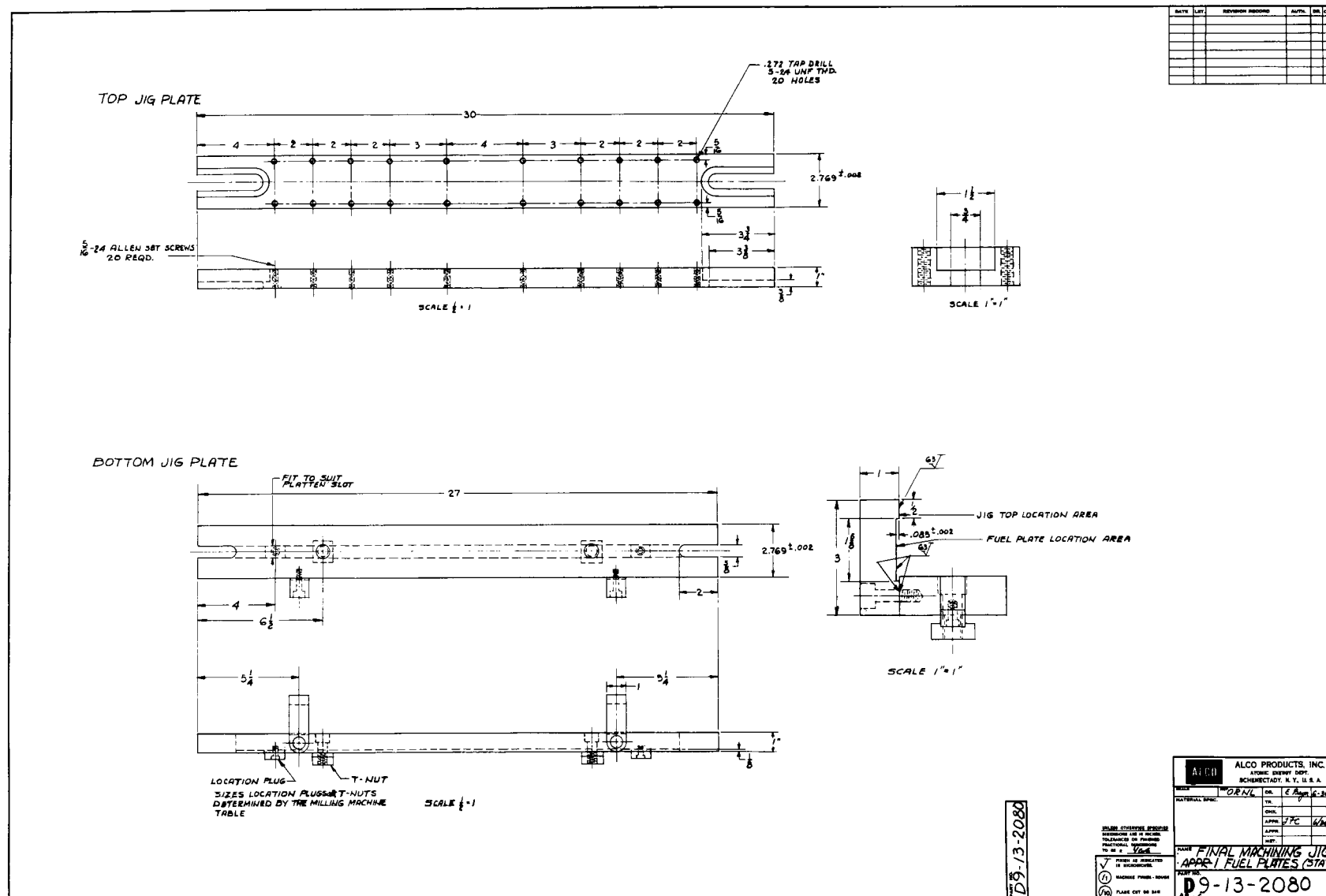
Fig. 15 (Alco-Dwg D9-13-2080) Fuel Plate Machining Fixture.
