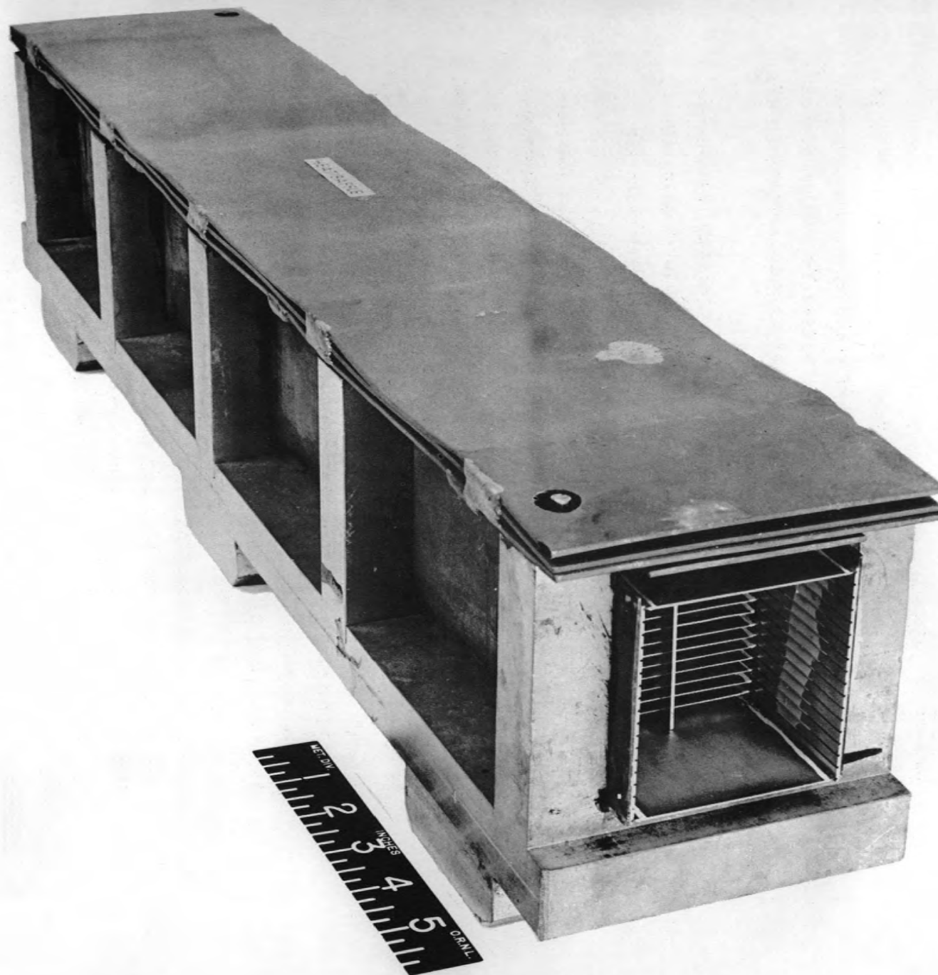
Fig. 25 (Y-25957) APPR Fuel Assembly Ready for Brazing.
