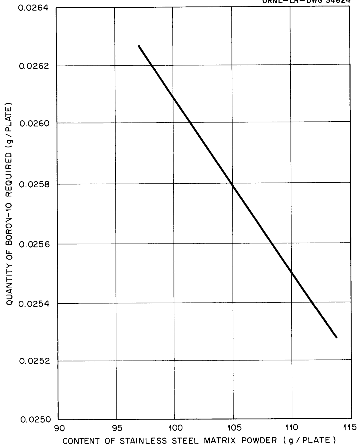
Fig.7. Variation in Boron-10 Content Required Per Plate as a Function of Stainless Steel Matrix Powder. Based on a Constant U^{235} Loading of 28.62 g / Plate.
