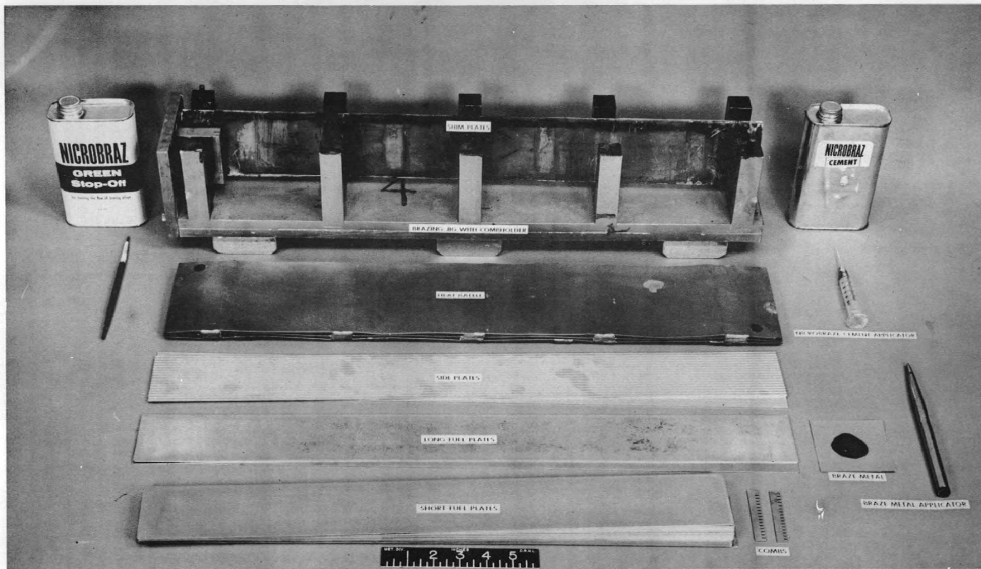
Fig. 21 (Y-25949) Components for Brazing APPR Fuel Element Assembly.
