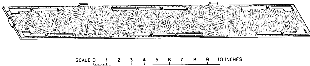
Fig. 17 Final Inspection Template for APPR Short Stationary Fuel Plate.
