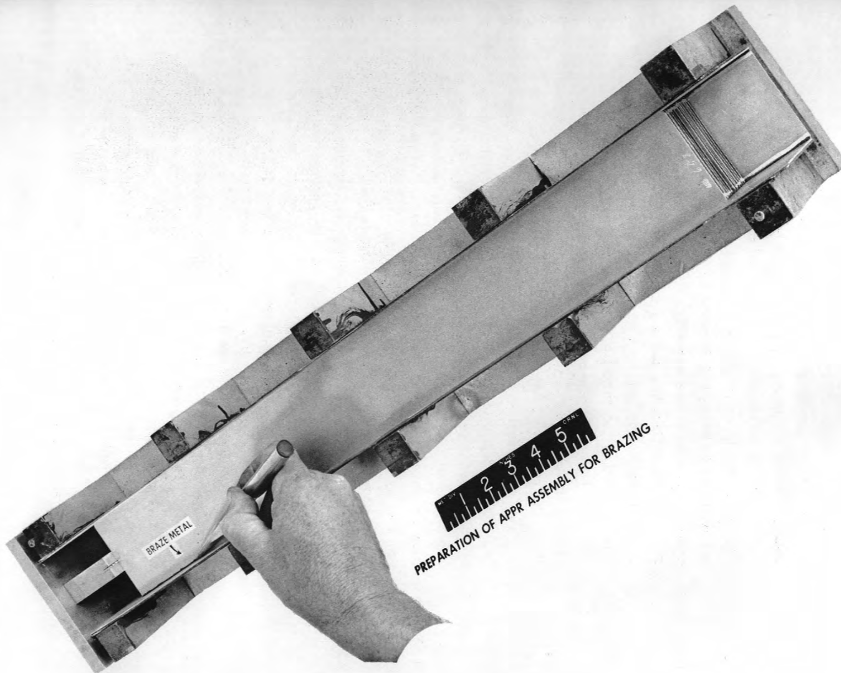
Fig. 22 (Y-25951) Application of Braze Metal.
