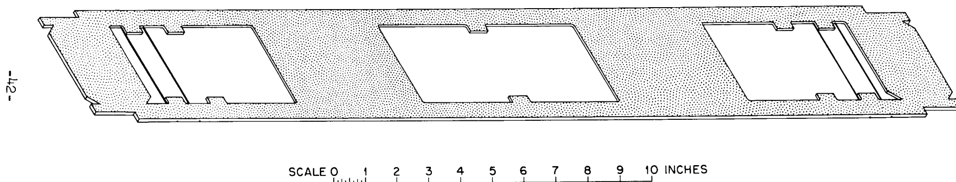
Fig. 14 Final Shearing Template for Either APPR Short or Long Stationary Fuel Plate.
