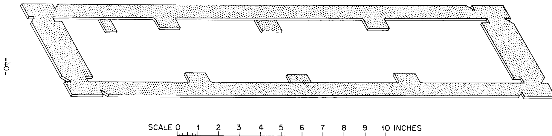
Fig. 13 Rough Shearing Template for APPR Stationary Fuel Plate.
