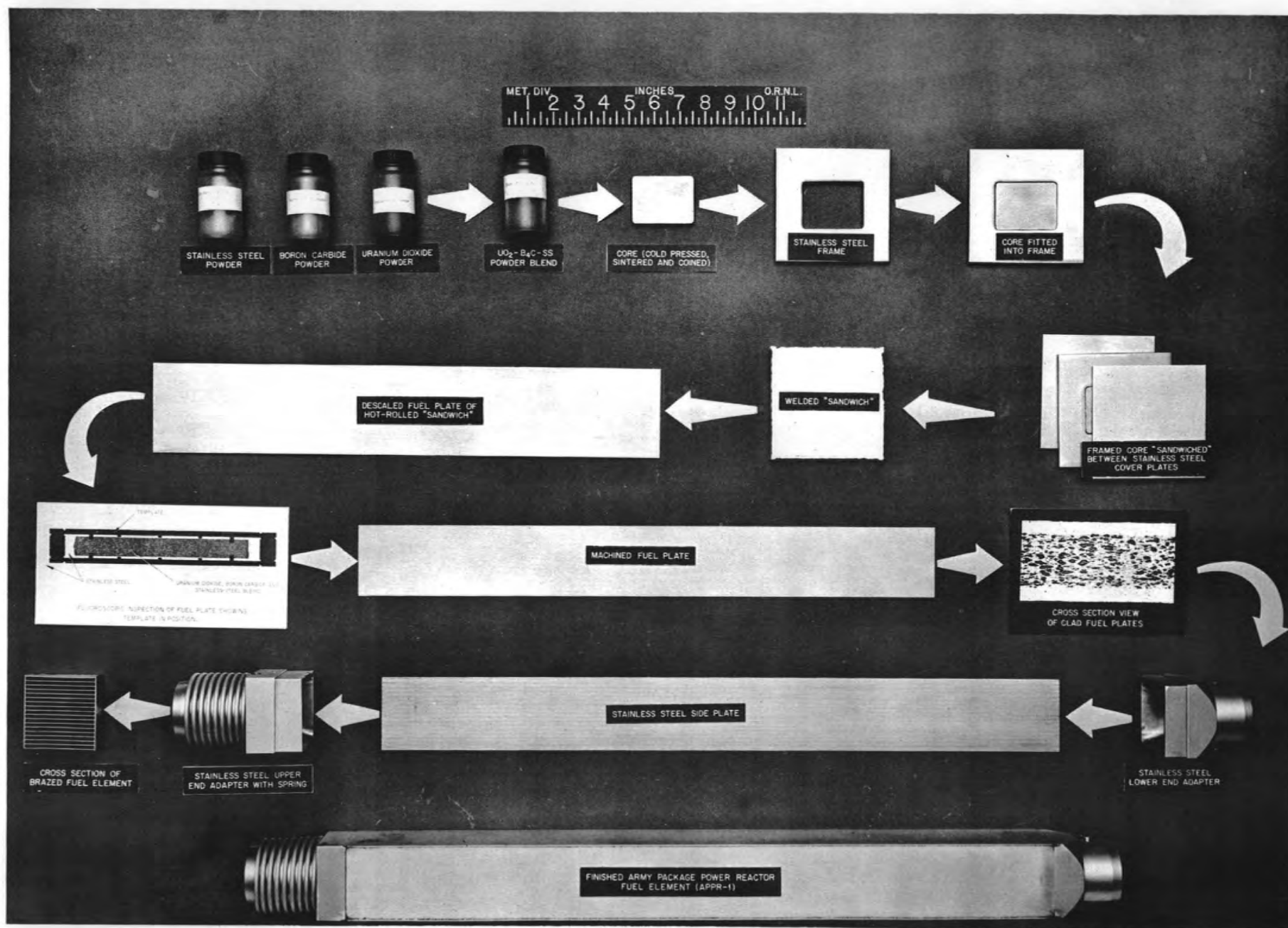
Fig. 6 (Y-25687) Fabricational Procedure for Manufacturing APPR Fuel Components.
