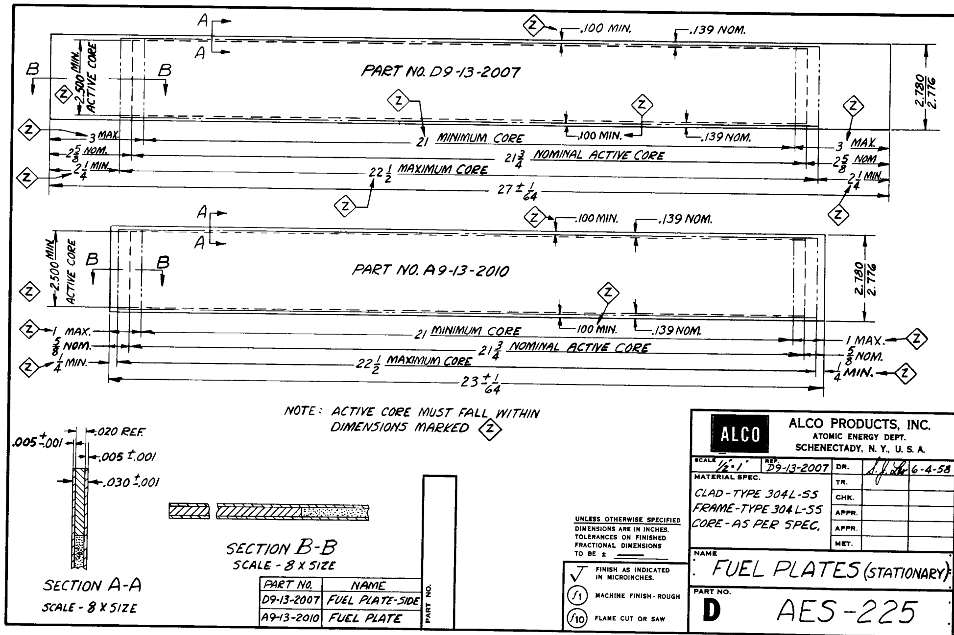
Fig. 16 Stationary Fuel Plates.
