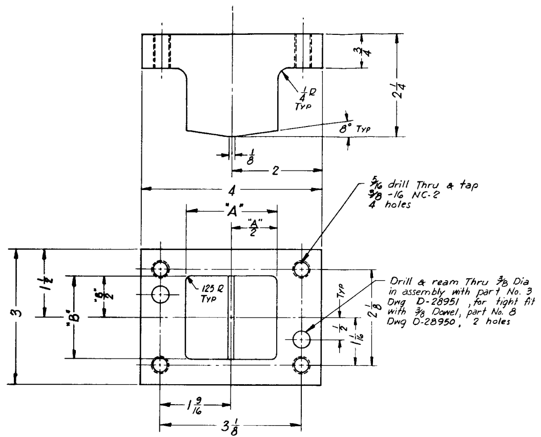
⑦ PUNCH MATL: Tool Steel, Ontario, Harden & Draw to Rockwell "C" 60-62 1 REQD
