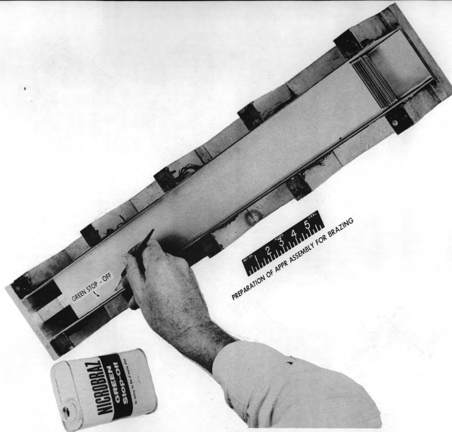
Fig. 24 (Y-25953) Application of Microbraz Green Stop-Off.
