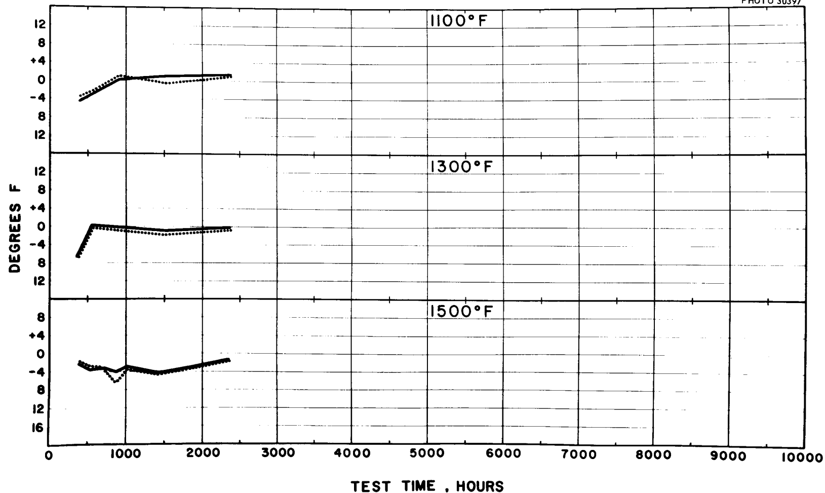
Figure 28. Typical Drift of Well-Type Thermocouple Assembly with Chromel P-Alumel Wires ( \pm 3/8\% 530°F to 2300°F) in NaK. (Note double curves represent the two couples contained in the assembly.)
