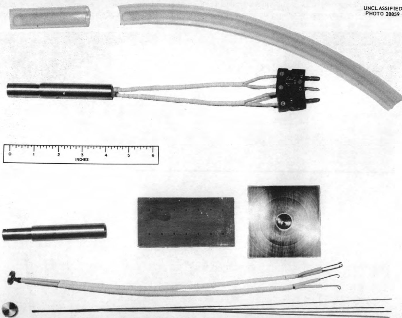
Figure 25. Disassembled and Assembled Views of Well-Type Thermocouple for NaK Piping Showing Copper Block for Fabrication of Inconel-Coated Thermocouple Junction, Jig for Attachment Weld to Well Bottom and Plastic Tubing for Protection of the Assembly During Handling.
