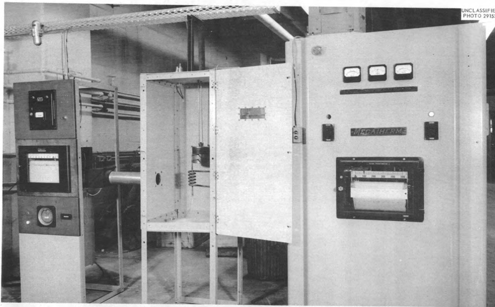
Figure 17. Induction Heating Facility for Rapid Heating of 0.250-in.-O.D. Inconel-Sheathed Thermocouples Showing Instrument Control Cabinet on the Left, Test Cabinet in the Center and Main Control Cabinet on the Right.
