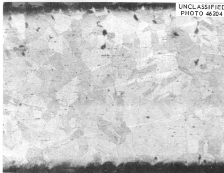
Figure 21 (9) . Cross-Section of Chromel P Wire Taken from Ceramic Beaded Assembly in One Foot, 0.250-in.-O.D. Inconel Protection Tube After 5000 hr at 1800°F. UT Sample No. 123. Etchant: \text{CuCl}_2 - aqua regia solution. 100X
