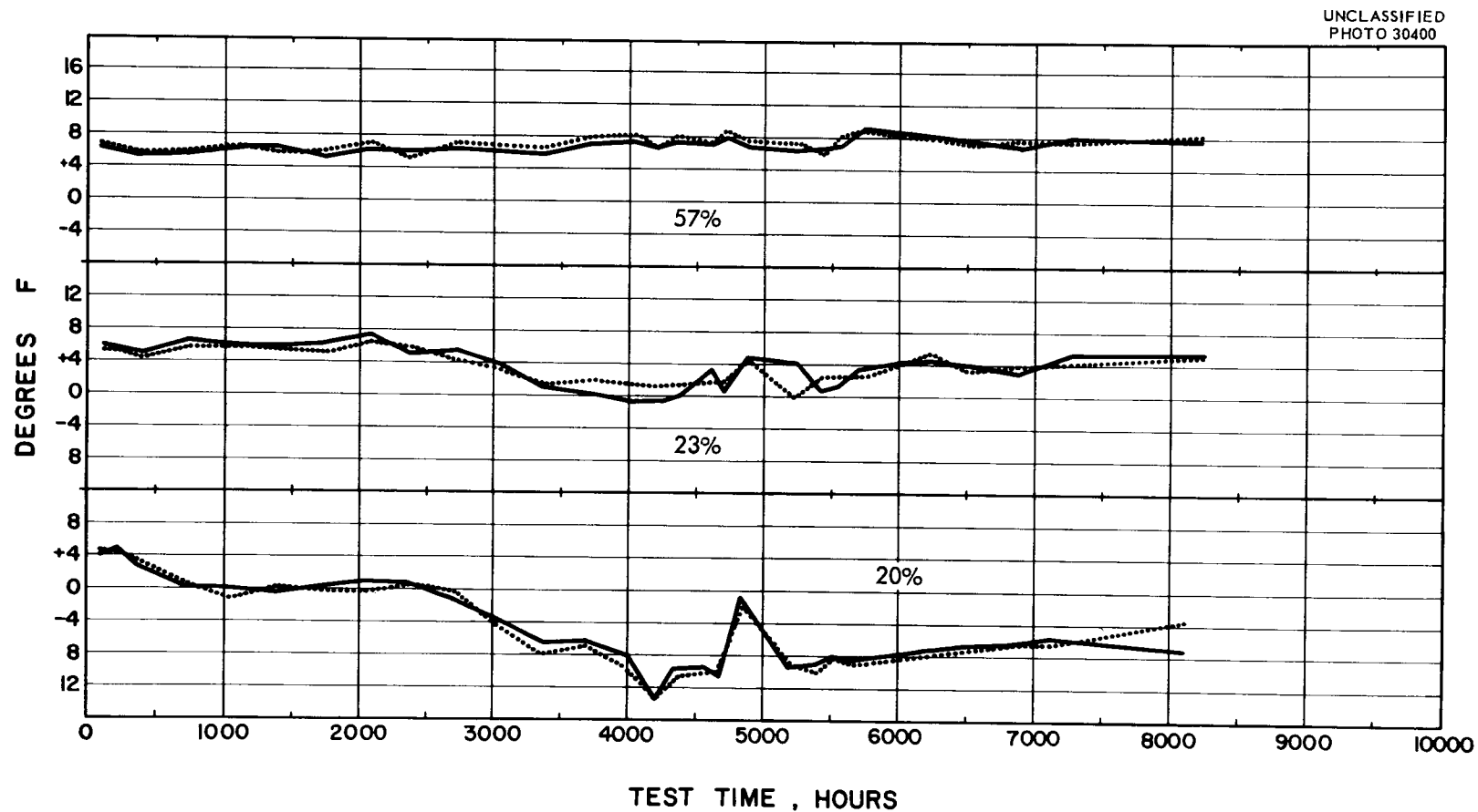
Figure 6. Typical Drift of 24-hr Soaked 0.250-in.-O.D. Inconel-Sheathed Chromel P-Alumel Thermocouple Material in Sodium and Fluoride Salt at 1500°F. (Note double curves represent the two couples contained in the sheath.)
