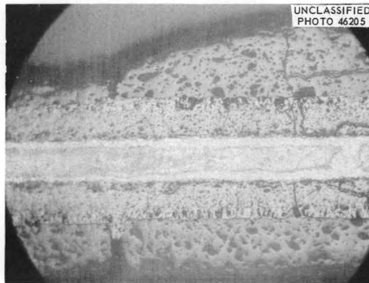
Figure 22 (9) . Cross-Section of Alumel Wire (With Adhering Heavy Layer of Alumel Oxide and Ceramic Bead) Taken from Ceramic Beaded Assembly in One Foot, 0.250-in.-O.D. Inconel Protection Tube After 5000 hr at 1800°F. (Note oxide growth at the refractory break, unusual wire surface effects and the unusual oxide appearance.) UT Sample No. 122. Etchant: Chromic Acid Solution - \text{CuCl}_2 - aqua regia solution. 30X.
