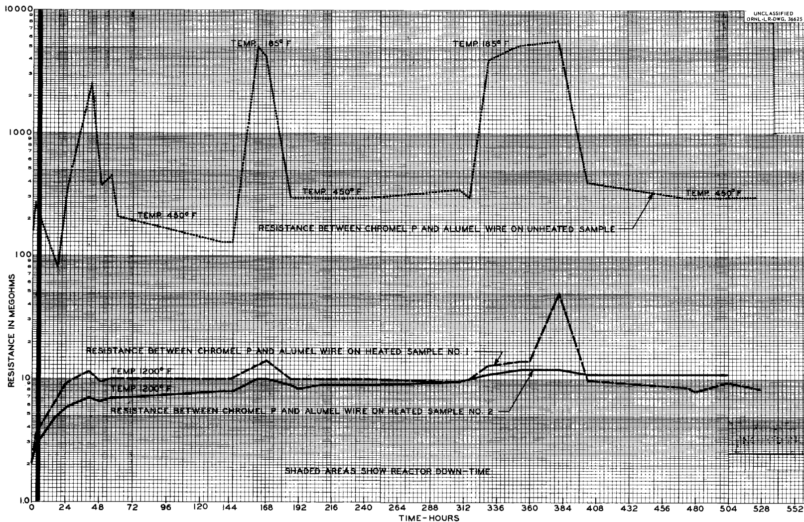
Figure 18 (7) . Magnesium Oxide Insulation Resistance of 0.250-in.-O.D. Inconel-Sheathed Thermocouple Material vs Irradiation Time in HB-3 of the LTR.
