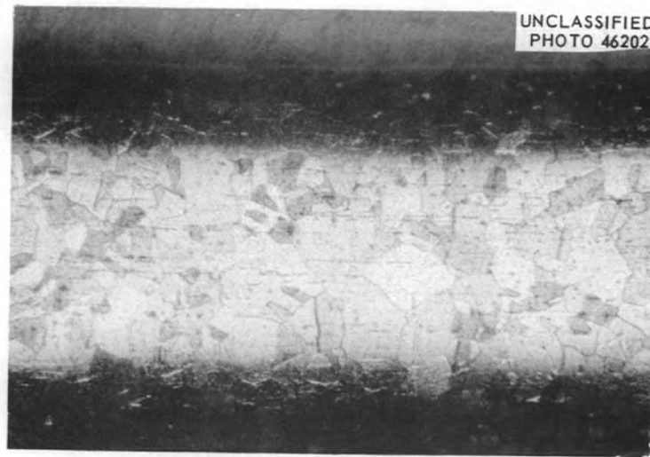
Figure 13 (9) . Cross-Section of Chromel P Wire from 0.250-in.-O.D. Inconel-Sheathed Thermocouple After 5000 hr at 1800°F. UT Sample No. 125. Etchant: \text{CuCl}_2 - aqua regia solution. 100X.
