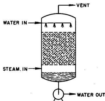
PACKED TOWER
