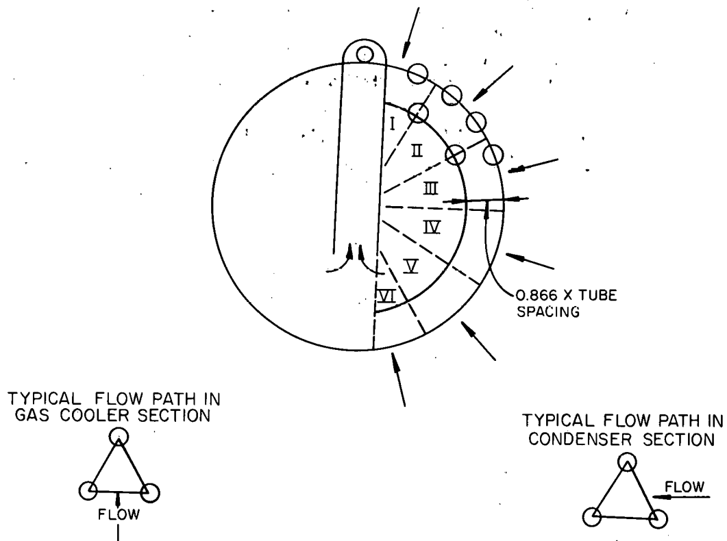
Fig. 1. Typical Condenser Geometries.
