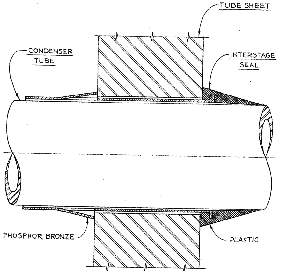
Fig. 16. Seal Design 2. Tube diameter, 0.750 in.; hole diameter, 0.875 in.
