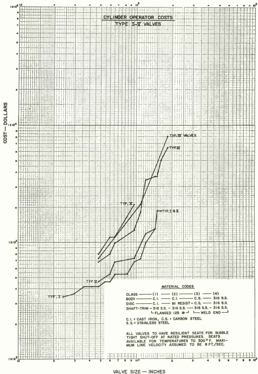
Fig. 34. Cylinder Operator as a Function of Size. Types I-V valves.
