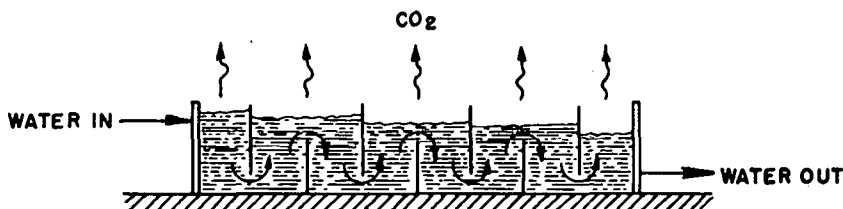
BAFFLES AND WEIR TYPE POND
