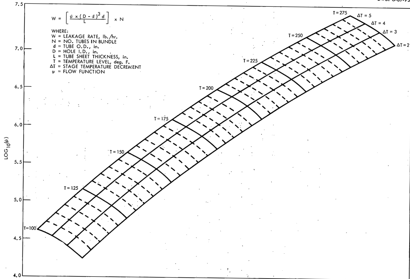
Fig. 11. Interstage Leakage vs Temperature, Temperature Decrement, and Annulus Geometry.
