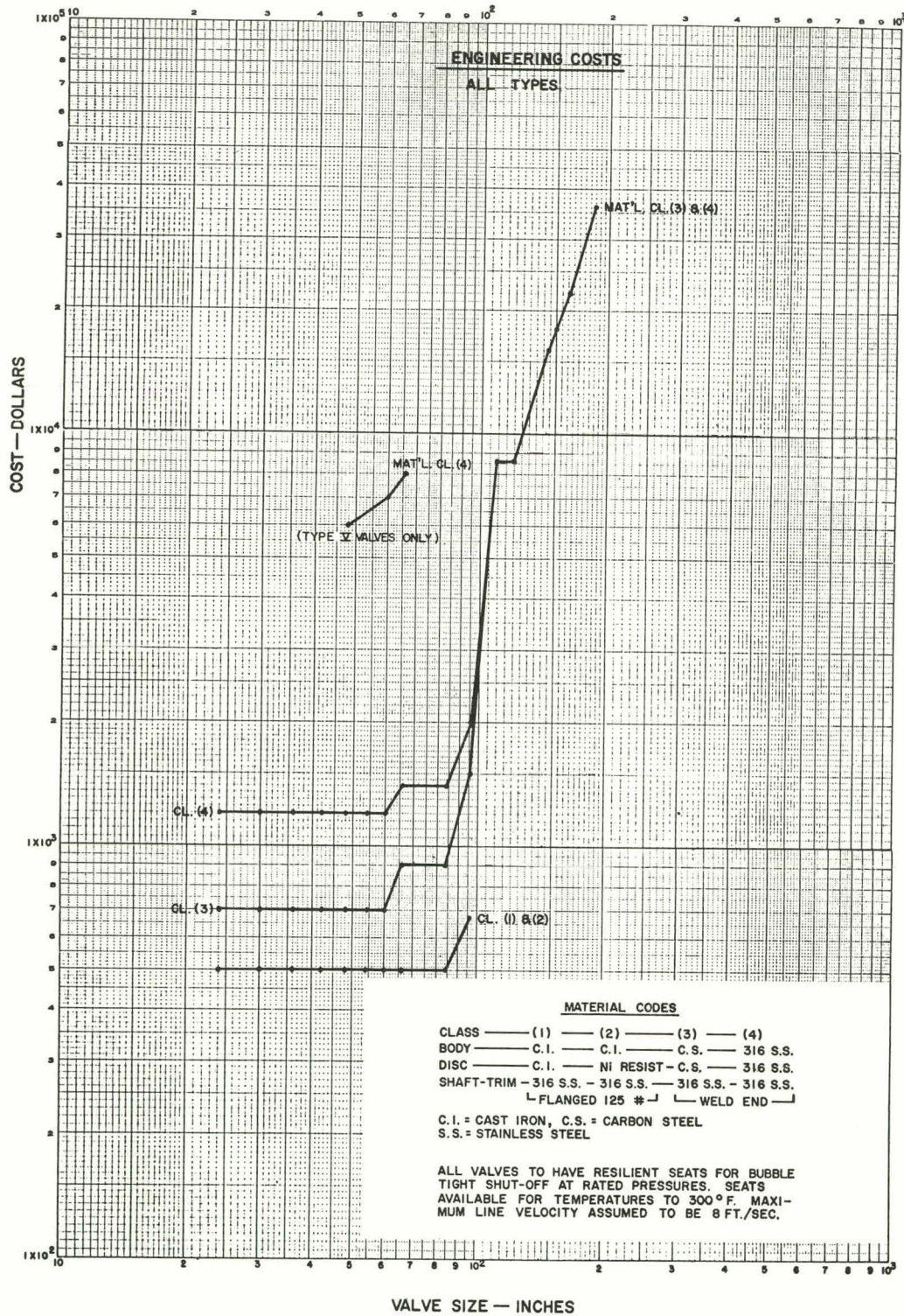
Fig. 35. Engineering Costs as a Function of Size. Types I-V valves.
