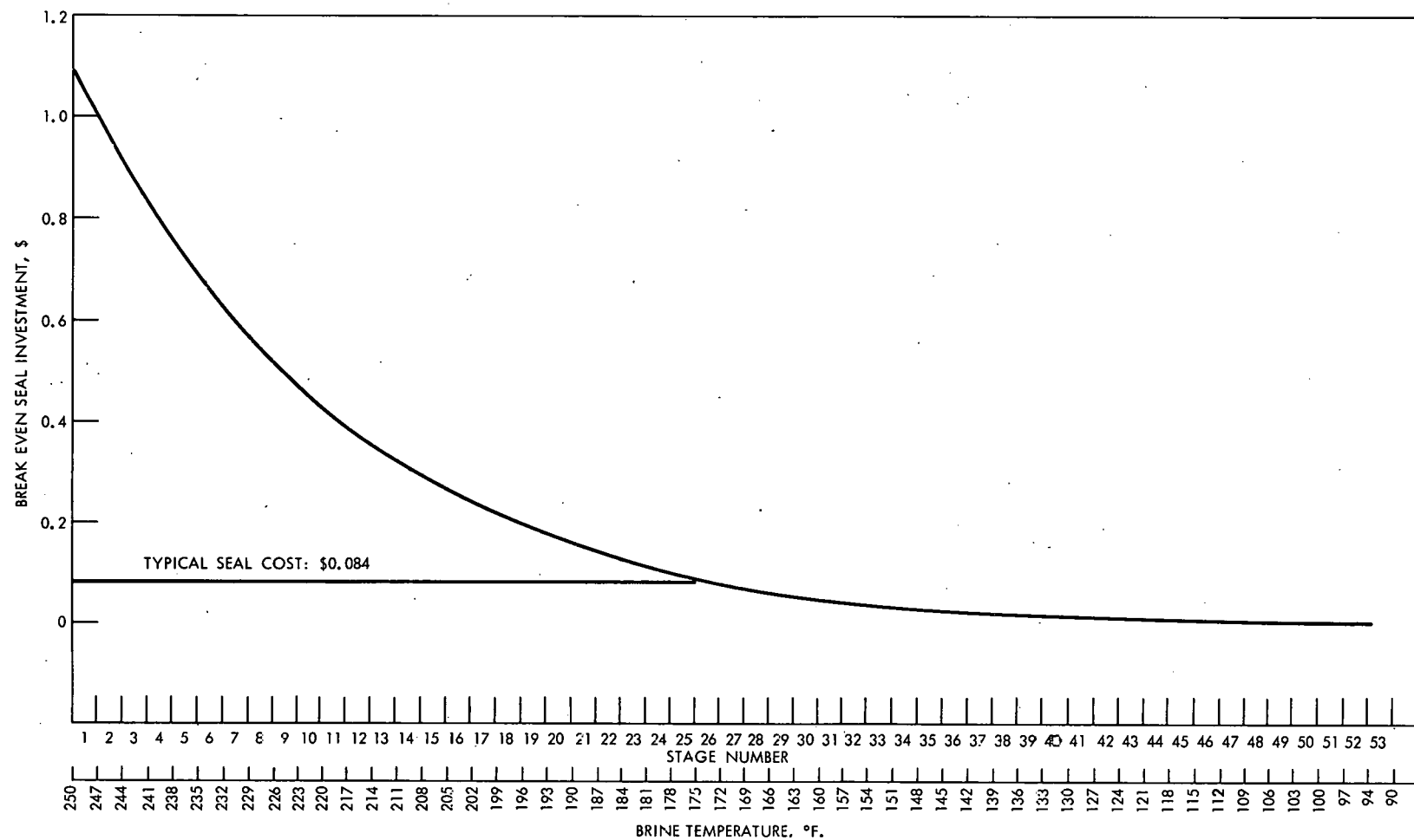
Fig. 13. Break-Even Sealing Investment.
