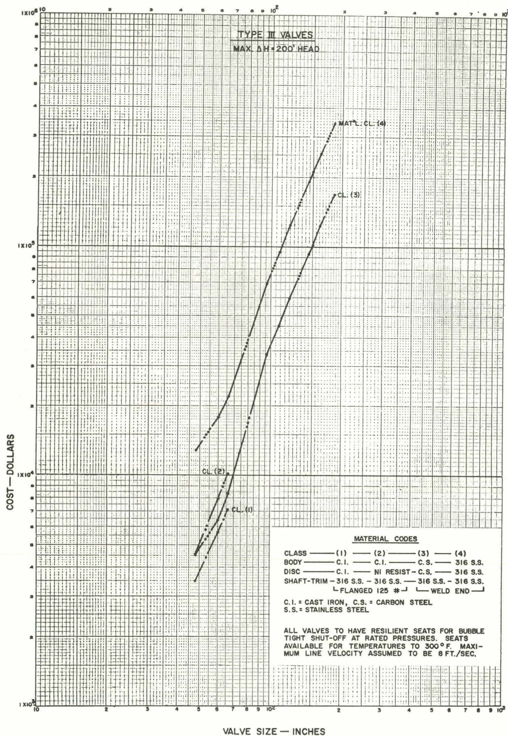
Fig. 31. Valve Costs as a Function of Size. Type III valves. Maximum \Delta H = 200 ft head.
