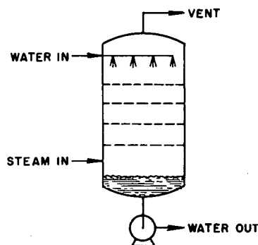
PLATE OR TRAY TOWER
