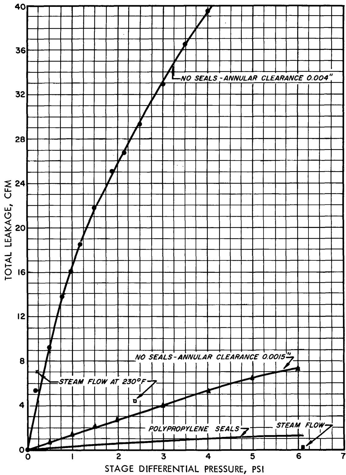
Fig. 14. Leak Tests for a 40-Tube Array of 0.75-in. Tubes.
