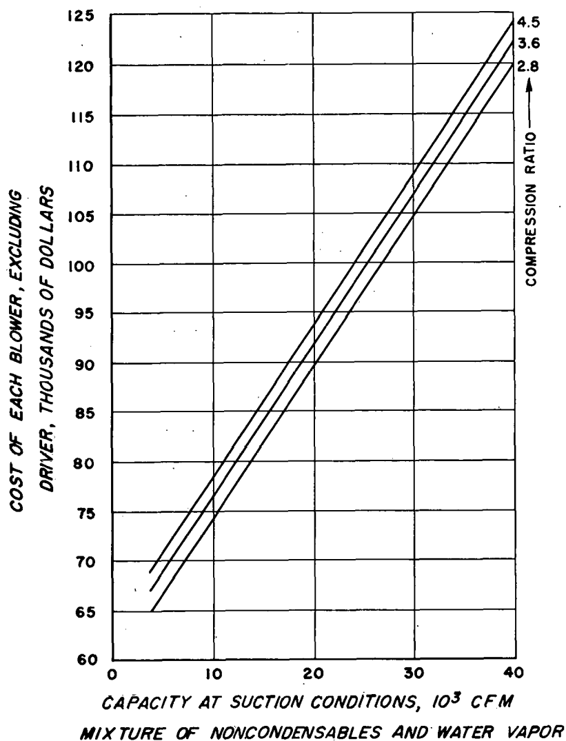
Fig. 19. Capacity vs Blower Cost. Cast iron with 3% nickel.
