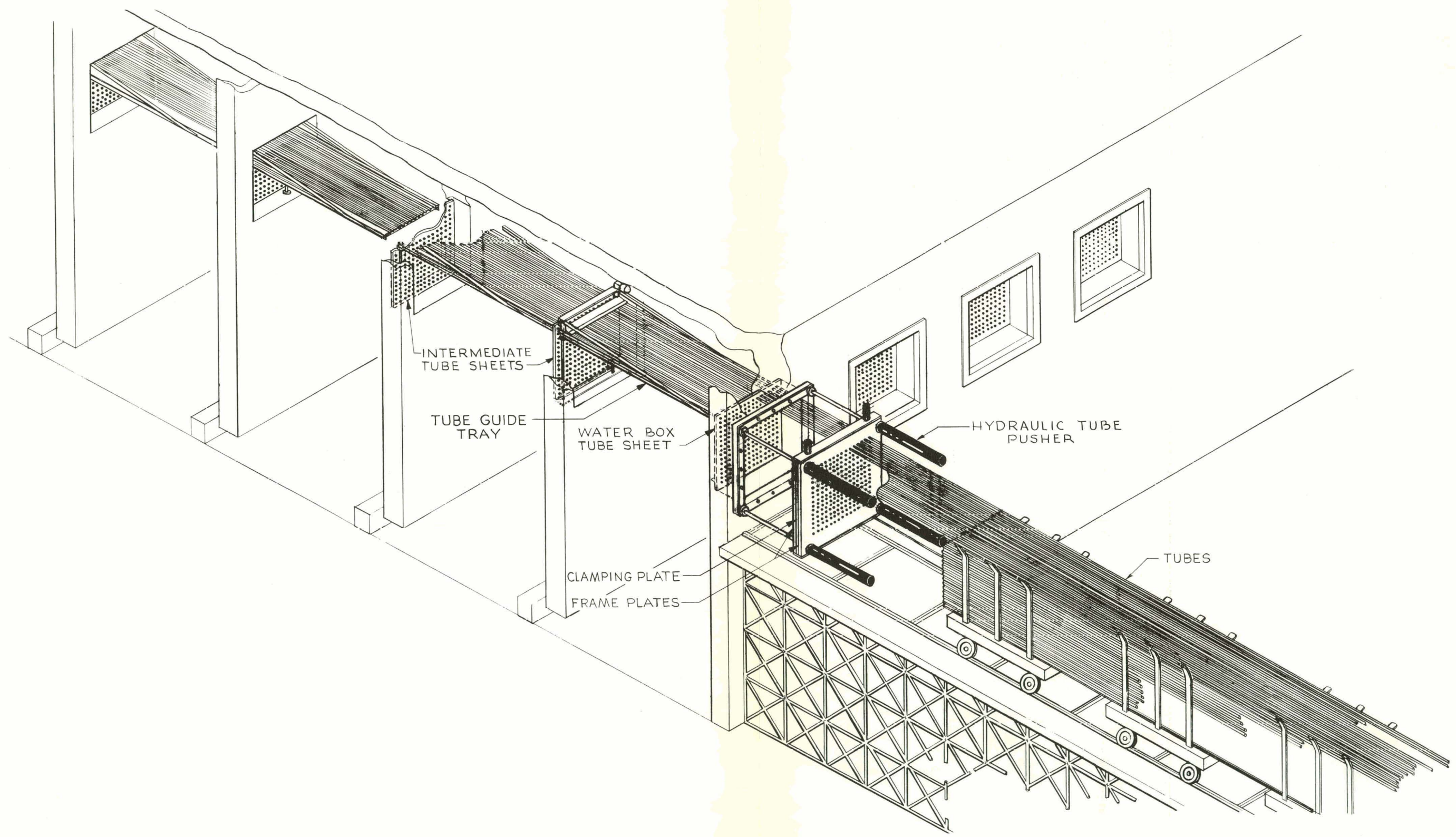
Fig. 9. Insertion of Full-Length Tubes in Evaporator.
