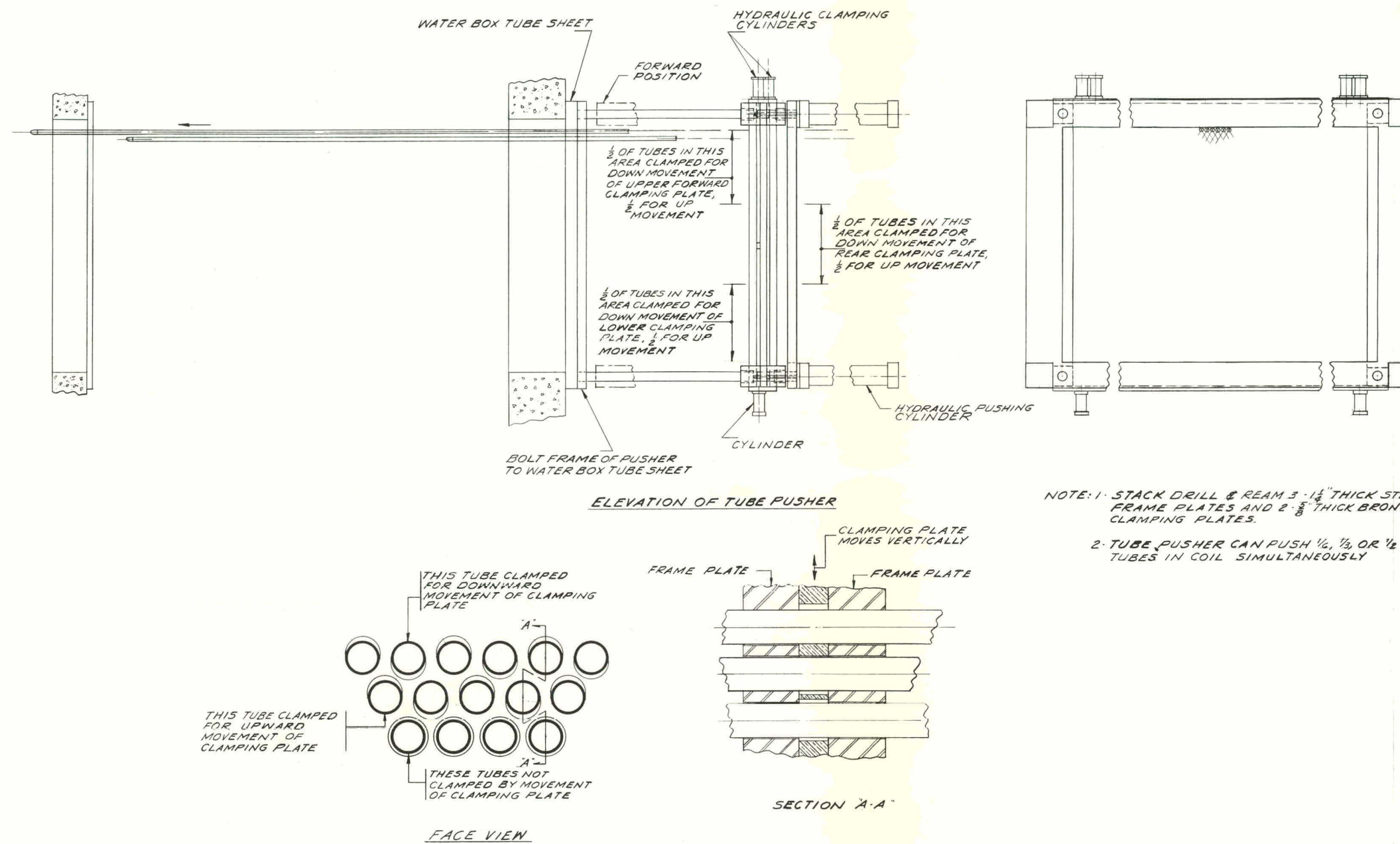
Fig. 8. Tube Pusher.
