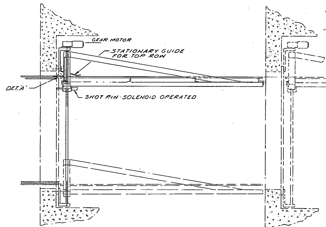
ELEVATION TYPICAL STAGE
