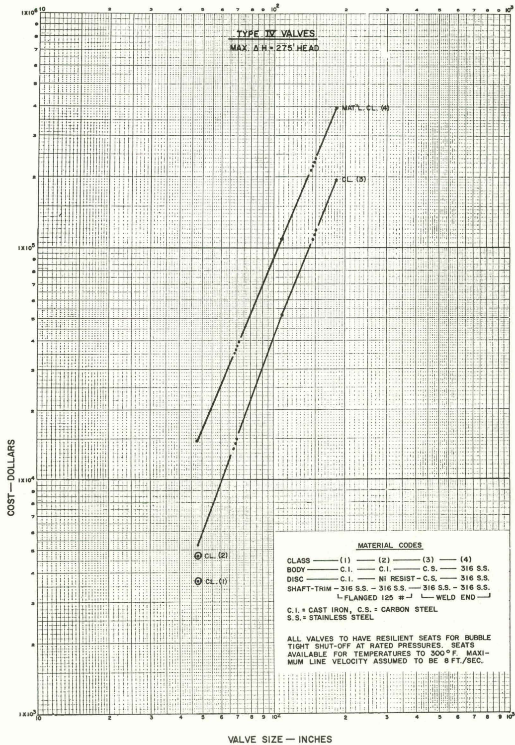
Fig. 32. Valve Costs as a Function of Size. Type IV valves. Maximum \Delta H = 275 ft head.
