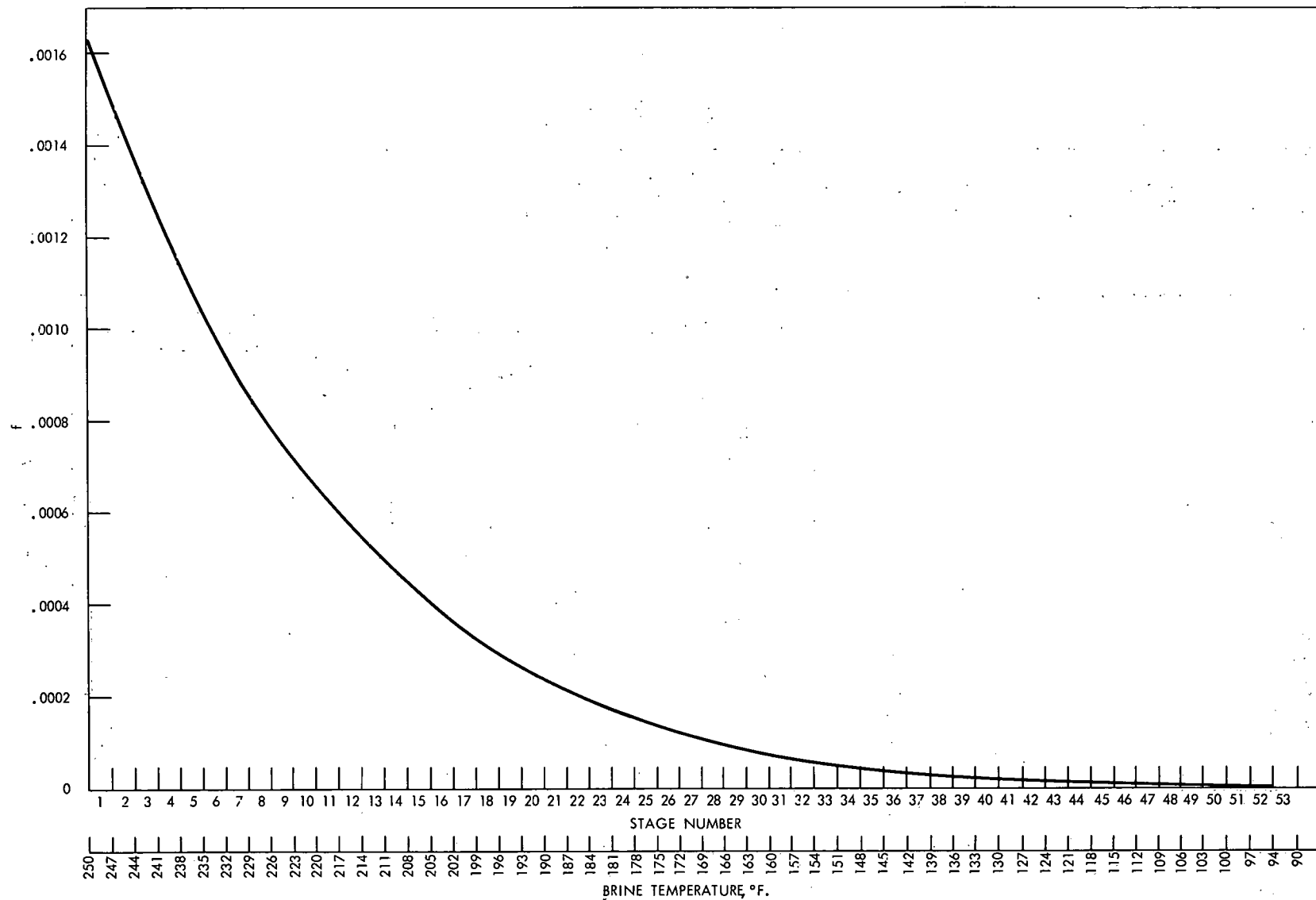
Fig. 12. Steam Availability Loss in Each Stage.
