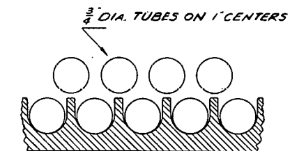
TYPICAL SECTION OF TRAY
