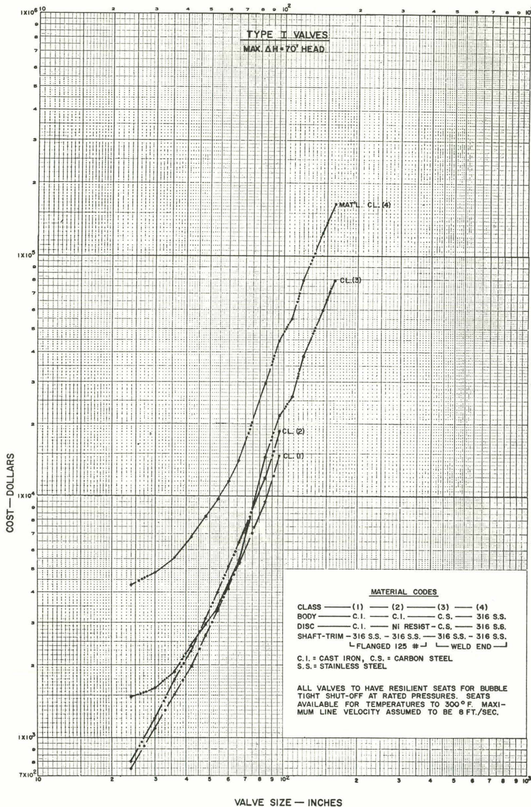
Fig. 29. Valve Costs as a Function of Size. Type I valves. Maximum \Delta H = 70 ft head.
