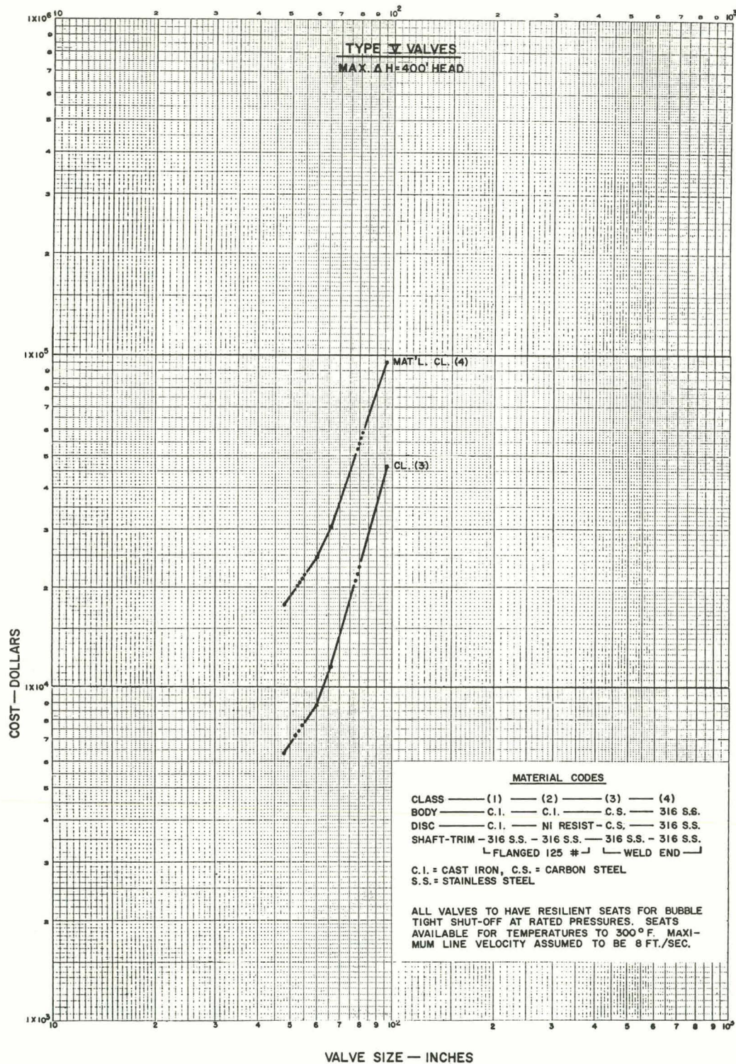
Fig. 33. Valve Costs as a Function of Size. Type V valves. Maximum \Delta H = 400 ft head.
