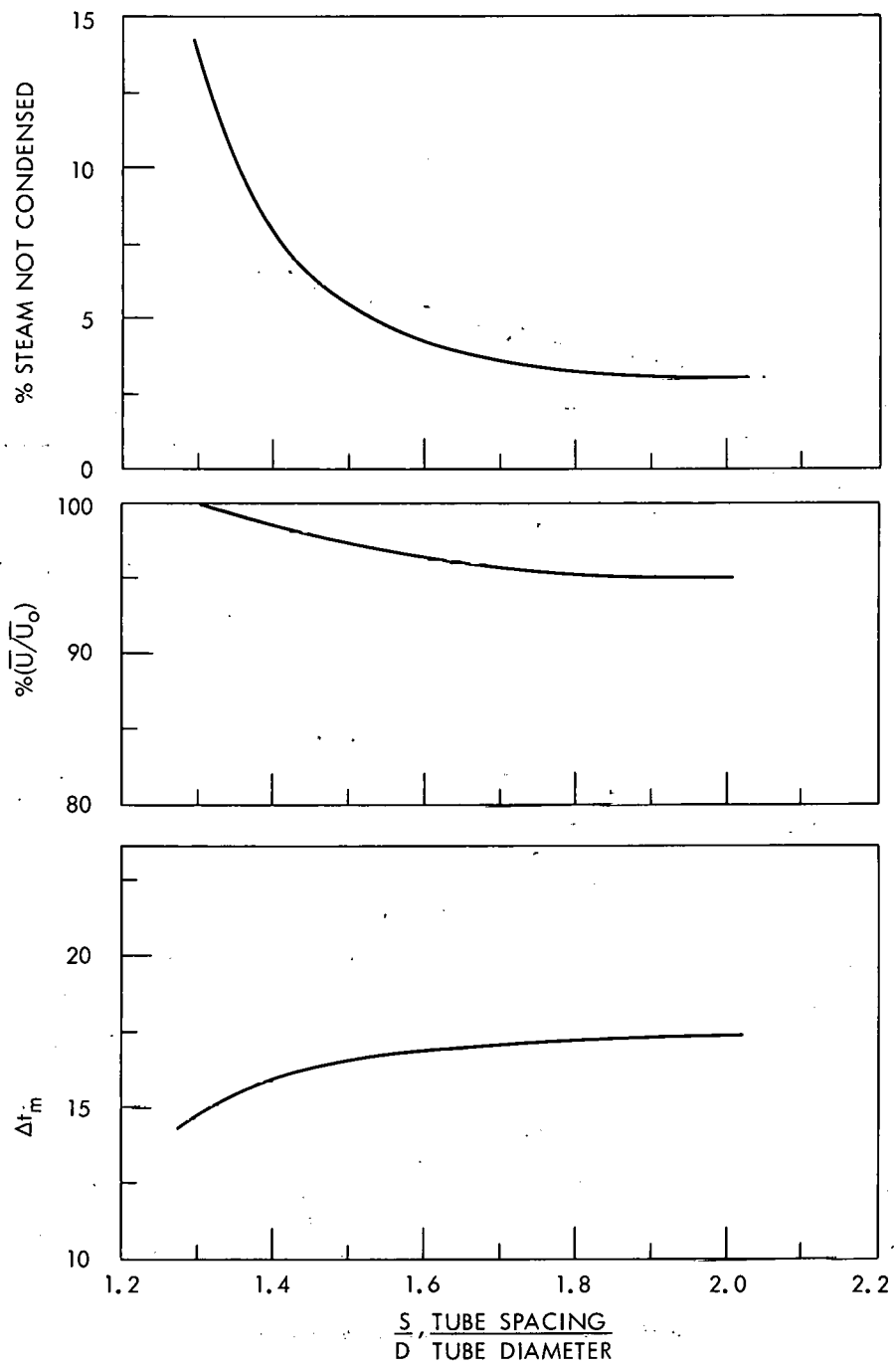
Fig. 3. Effect of Tube Spacing Ratio upon Condenser Performance in the Condenser of Fig. 2.
