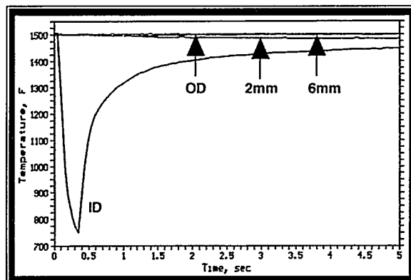
Figure 3. Radial Temperature Profile Through the Wall of the Alumina/Mullite Candle Filter During Pulse Cycling
