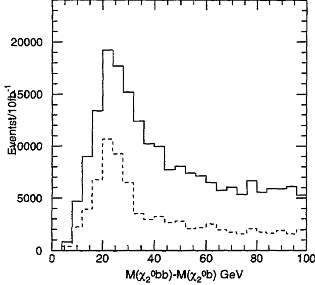
Figure 11: Distribution of mass difference ( m_{\tilde{g}} - m_{\tilde{0}_L} ). This is the y-projection of the scatter plot in Fig. 9.
