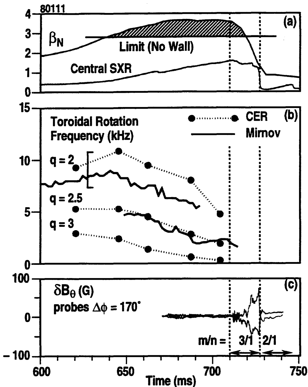
Fig. 4. The temporal evolution of discharge 80111, showing the correlation between the rotation, and the growth of the unstable mode. (a) normalized beta, \beta_N , and central SXR, (b) toroidal rotation frequencies at several rational surfaces from magnetic (Mirnov) oscillations and CER spectroscopy; and (c) measurement of \delta B_\theta from two magnetic probes separated toroidally by 170^\circ , the separation of the two signals at t \sim 712 ms indicates the growth of an n=1 mode.
