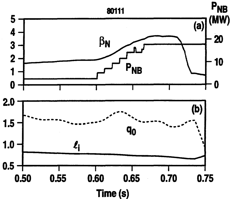
Fig.1. Temporal evolution of wall stabilized discharge. (a) normalized plasma beta, \beta_N = \beta_T / (I/aB) \% \cdot m \cdot T/MA , and injected neutral beam power, P_{NB} (b) calculated internal inductance l_i and measured central safety factor, q(0)
