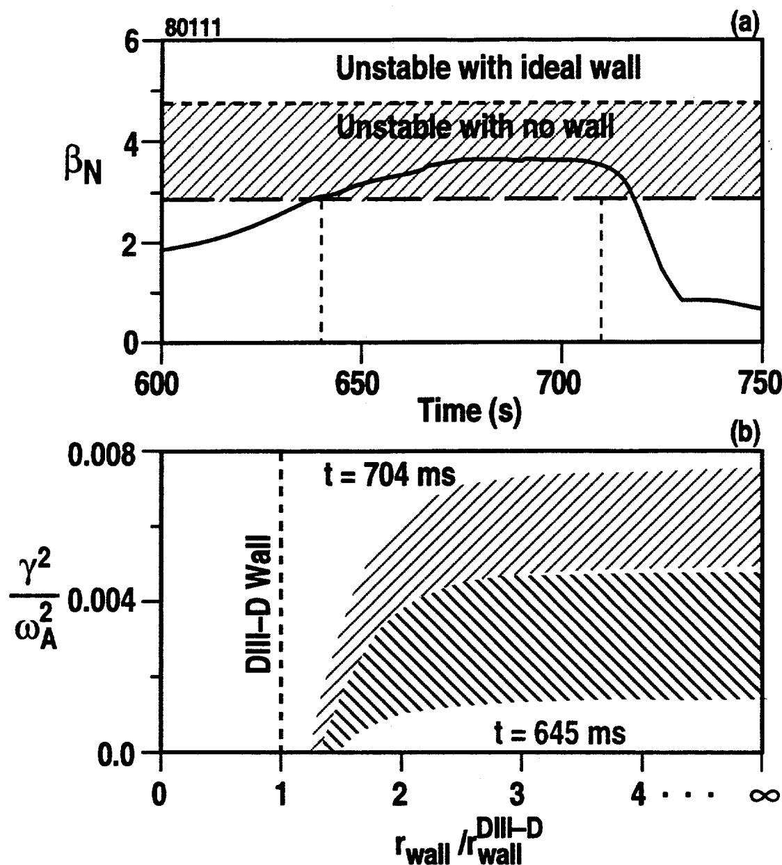
Fig. 3. Calculated ideal kink mode limits (a) normalized beta, \beta_N , dashed line is the maximum achievable beta with no wall stabilization, dotted line is the maximum achievable beta with an ideal wall and the location of the DIII-D vessel. (b) Variation of normalized growth rate, \gamma^2/\omega_A^2 , with wall position for the reconstructions of discharge 80111 at t = 645 ms and at t = 704 ms.
