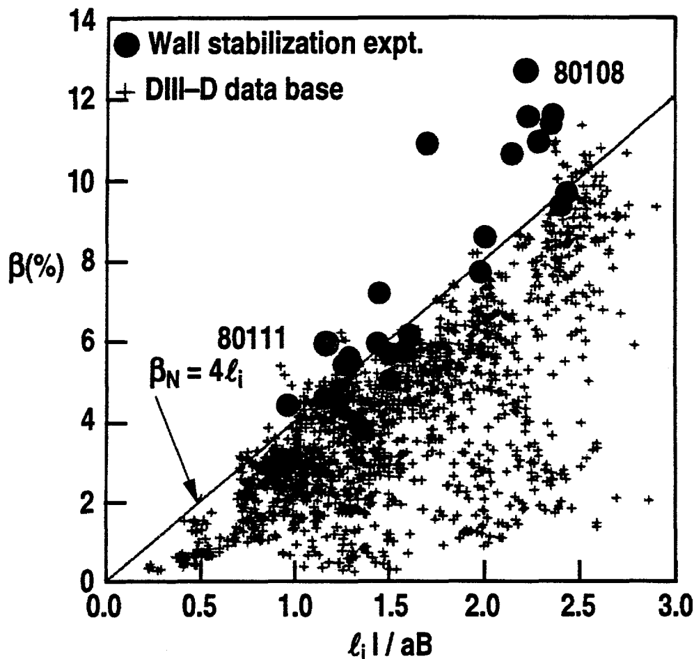
Fig. 2. Scaling of the DIII-D beta limit with \ell_i and normalized current, including the recent high beta experiments, solid circles.
