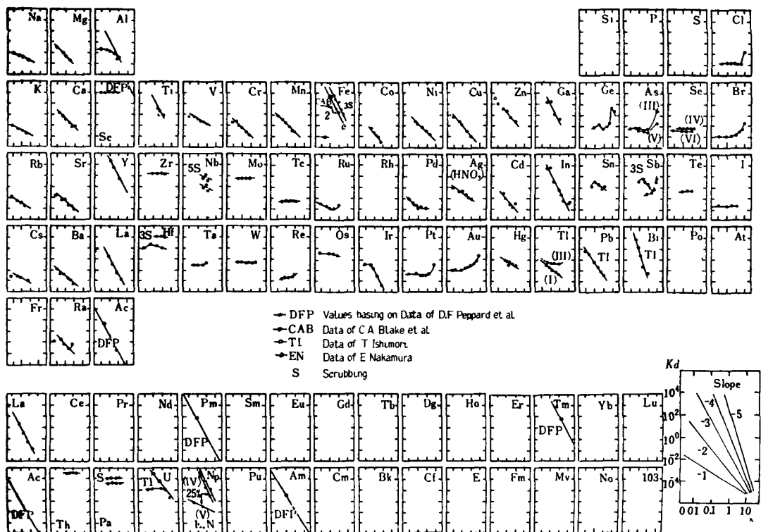
Figure 7. Extraction of Elements from HCl Solution by 50% HDEHP in Toluene as a Function of Acid Concentration. 178
