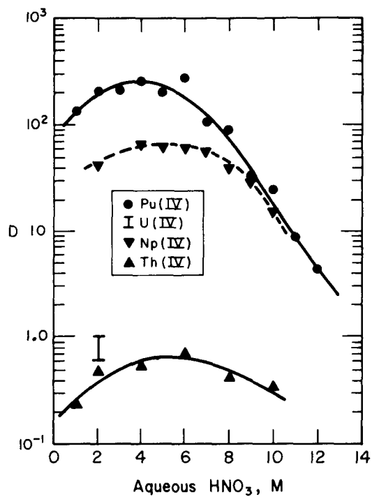
Figure 11. The Extraction of the Quadravalent Actinide Nitrates by 10 vol % TOA in Xylene. 190
