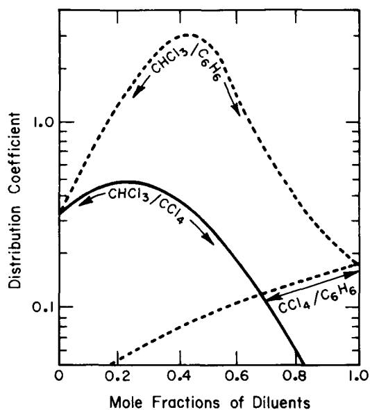
Figure 17. Distribution Coefficients for Np(IV) Extraction with 10^{-2} M Tetrabutyl-Ammonium Nitrate from 3M \text{HNO}_3 Using Mixtures of Different Diluents. 203
