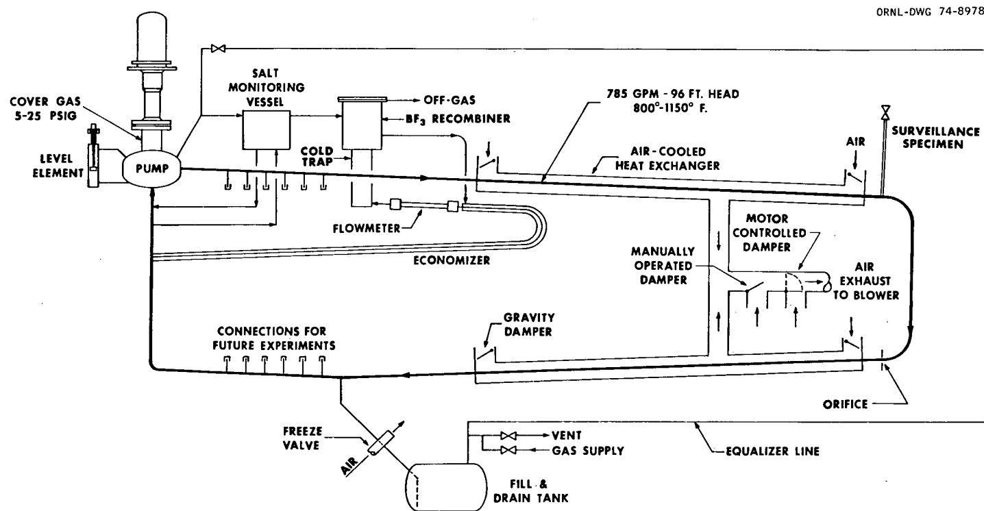
Fig. 10.5.4. CSTF schematic.
