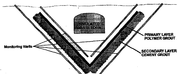
Figure 1. Schematic of Close-Coupled Barrier Demonstration.
