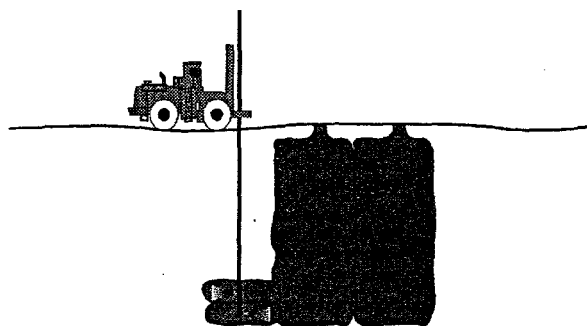
Figure 2. Conventional column jet grouting.
