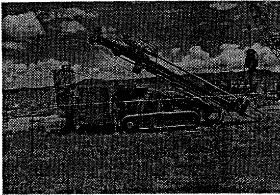
Figure 5. Casa Grande Jet Grouting Rig to be used at Hanford Demonstration.
