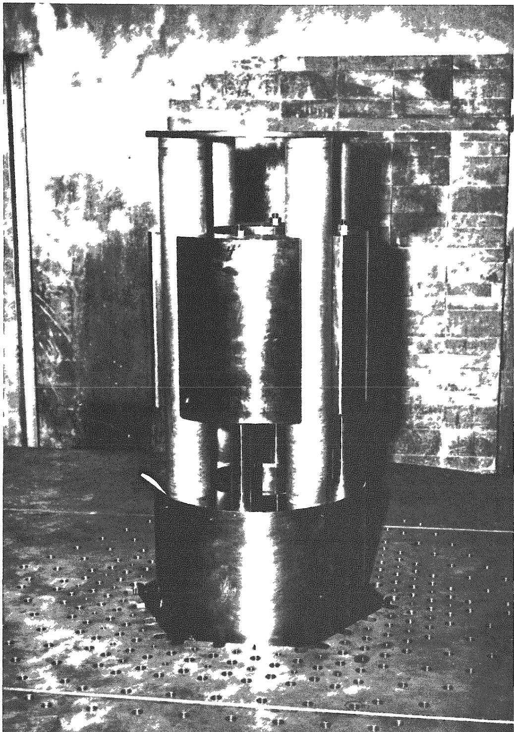
Fig. 2.25 Shim assembly.
