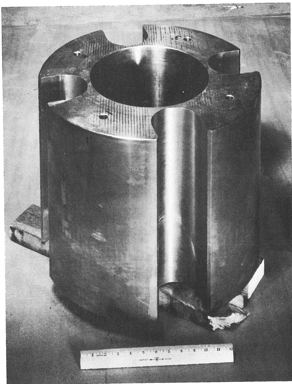
Fig. 2.23 Control shim.
