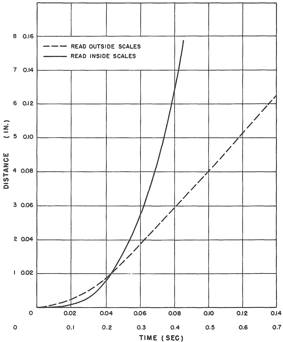
Fig. 2.28 Shim position vs time after scram signal.
