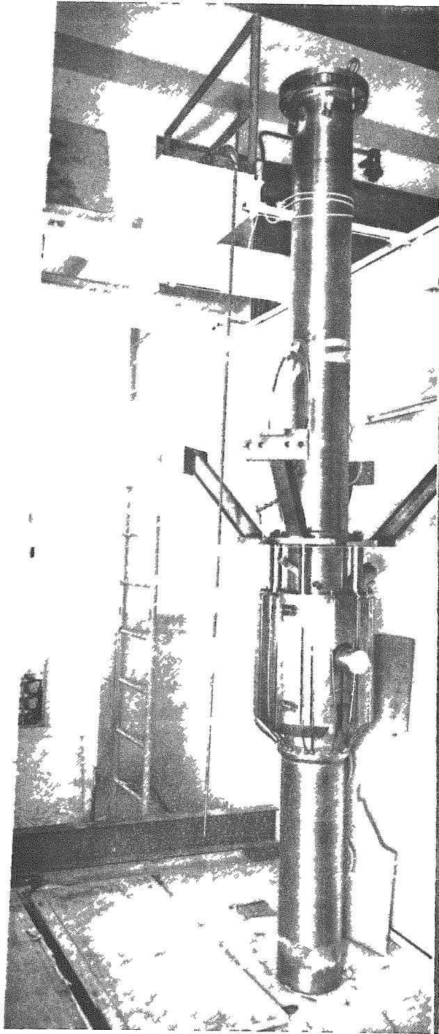
Fig. 2.13 Fuel element suspended beside vessel.
