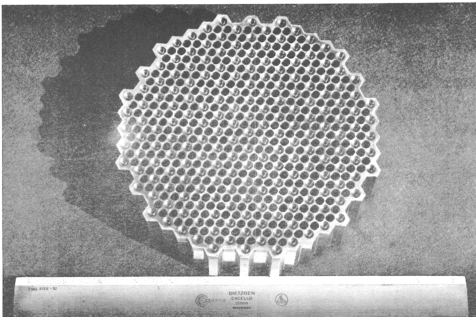
Fig. 2.8 Capsule locator plate.
