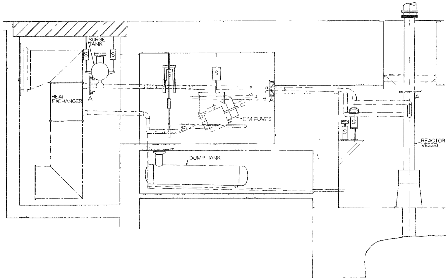
Fig. 2.19 Elevation of sodium system.
