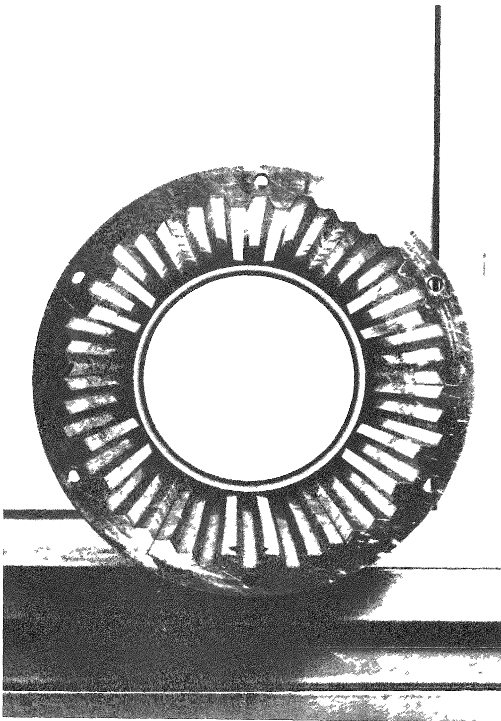
Fig. 2.7 Flow divider.
