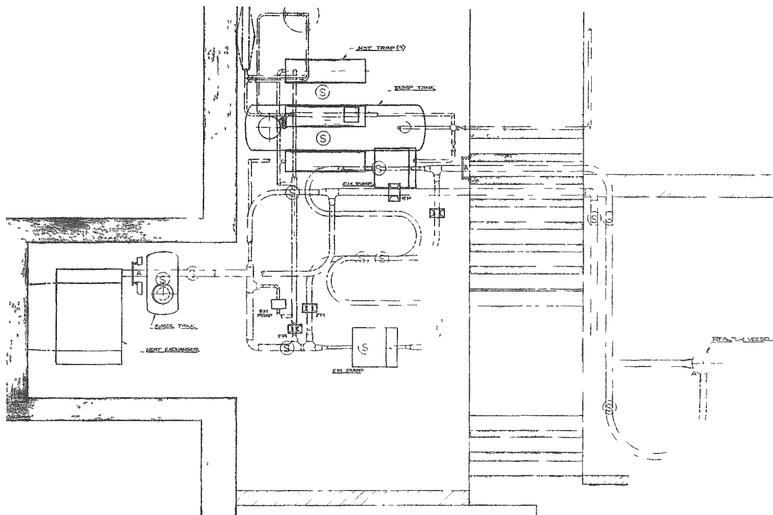
Fig. 2.16 Plan view of sodium system showing main components, support, and anchor points.
