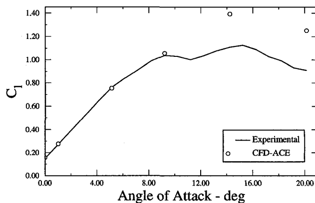
Figure 10. Lift Coefficients
