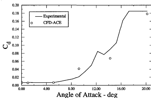
Figure 11. Drag Coefficients
