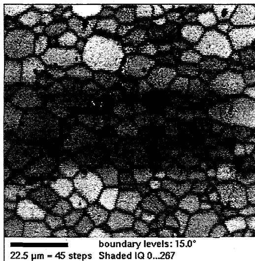
Figure 9. The OIM image of the 10 \mu\text{m} , 99.99% alumina sample and the points across the crack that were used to determine the distribution of misorientations along a crack.
