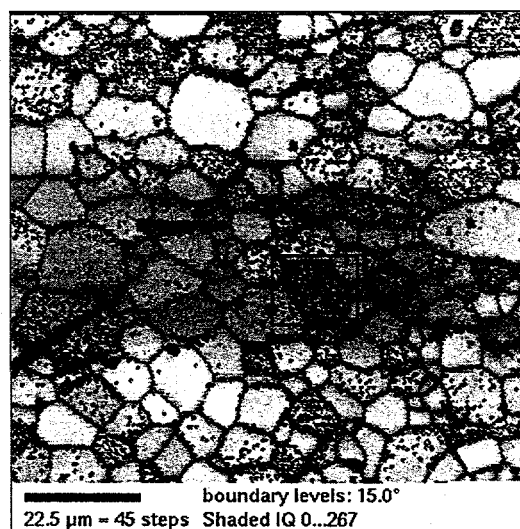
Figure 3. The OIM image of the 10 \mu\text{m} 99.99% alumina with the addition of grain boundaries, which are drawn for misorientations between neighboring measurements of greater than 15^\circ .
