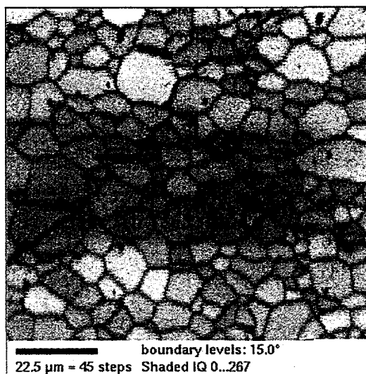
Figure 2. Image quality map for the 10 \mu\text{m} , 99.99% alumina sample with darker pixels representing a lower image quality.
