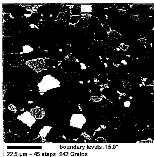
Figure 4. The OIM image of the 10 \mu\text{m} , 99.99% alumina sample after a clean-up procedure was used to minimize the presence of ambiguous patterns. The shades in this image are only used to help delineate the grains.
