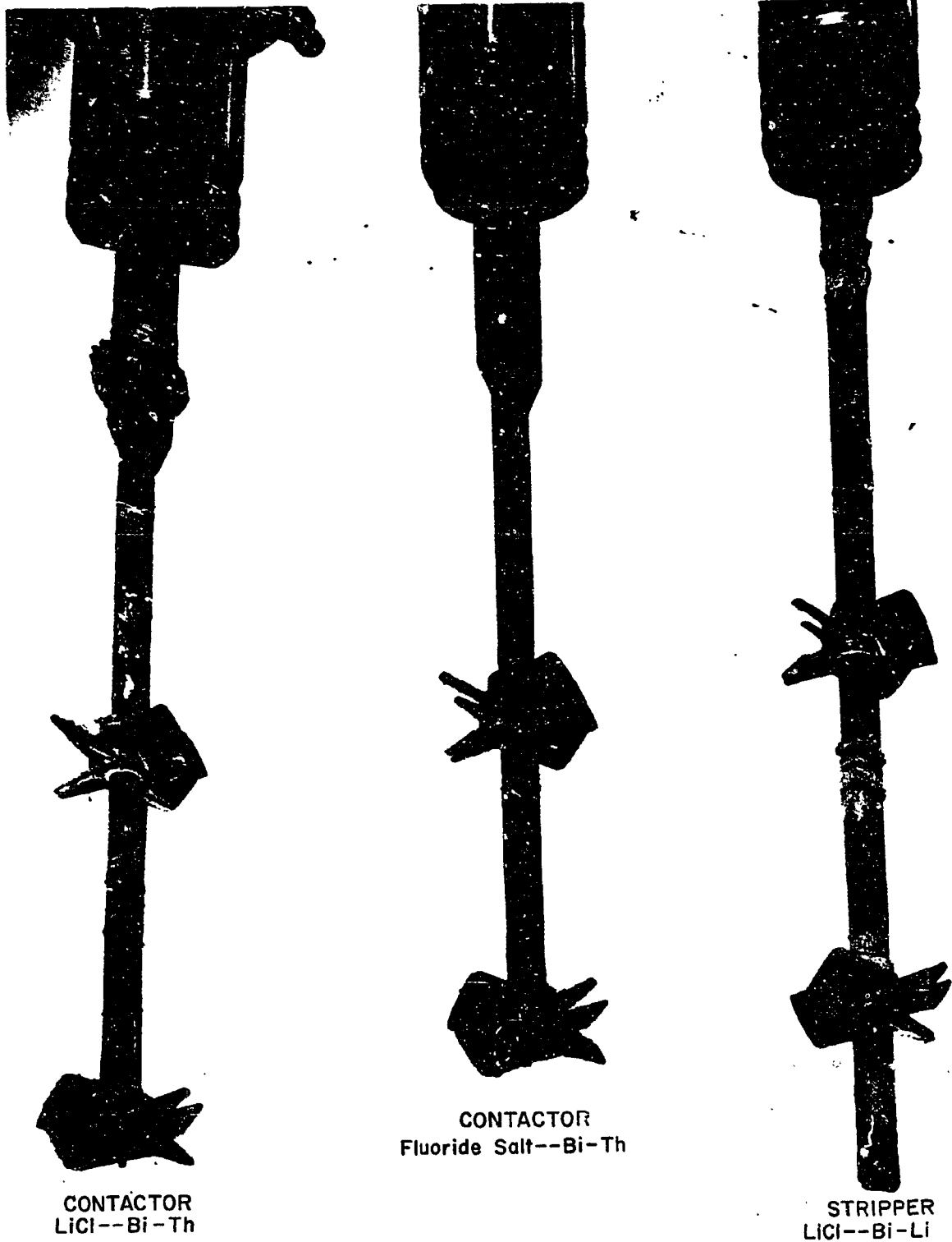
Fig. 7. Photograph of agitator shafts removed from MTE-3.
