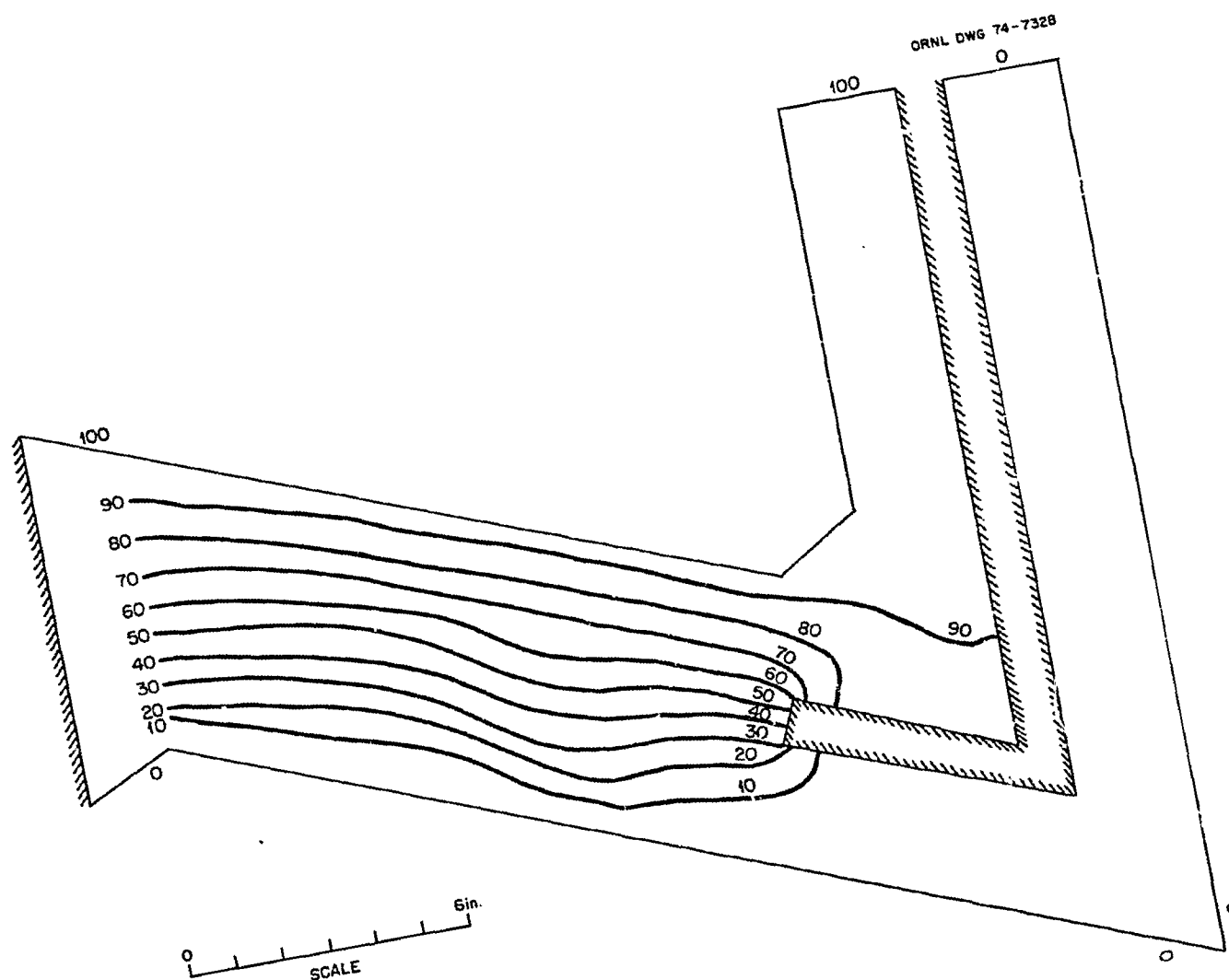
Fig. 16. Calculated current distribution in the electrode sidearm using a new electrode design. The percentage of the total current flowing between two stream lines is equal to the difference between the numbers on the stream lines.
