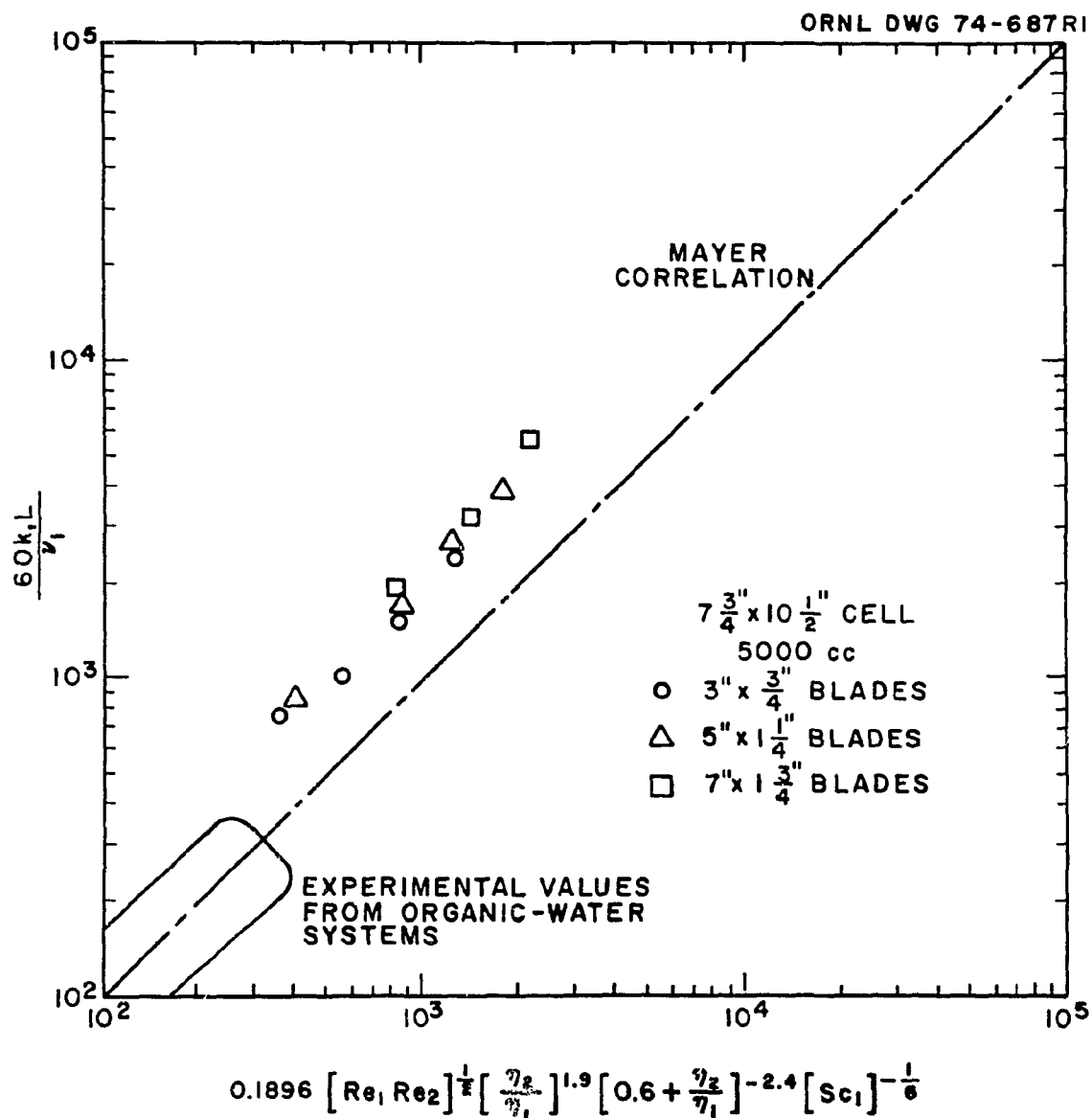
Fig. 3. Selected experimental results as compared with the Mayer correlation for the water-mercury system.
