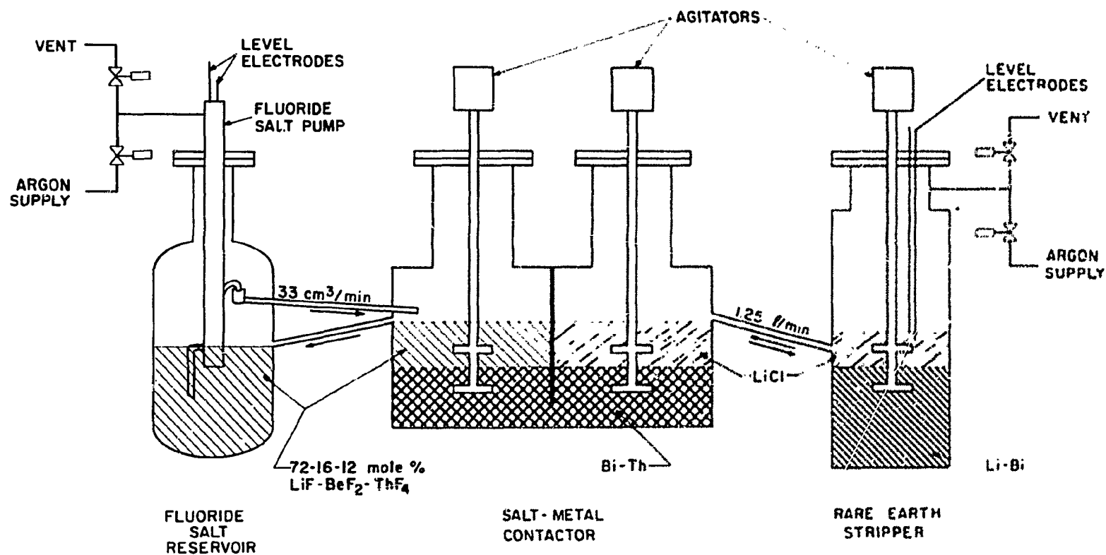
Fig. 6. Flow diagram for metal transfer experiment MTH-3.
