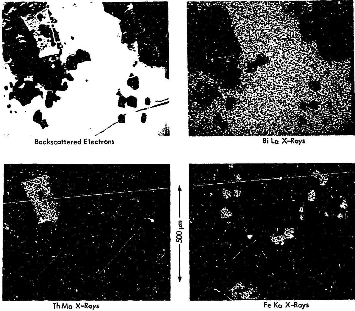
Fig. 13. Electron beam scanning images of elements in the Li-Bi phase from the stripper at the LiCl salt interface in experiment MTE-3.
