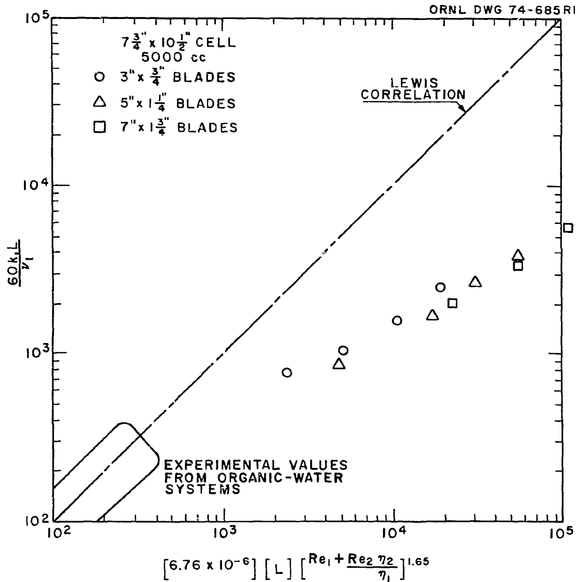
Fig. 1. Selected experimental results as compared with the Lewis correlation for the water-mercury system.
