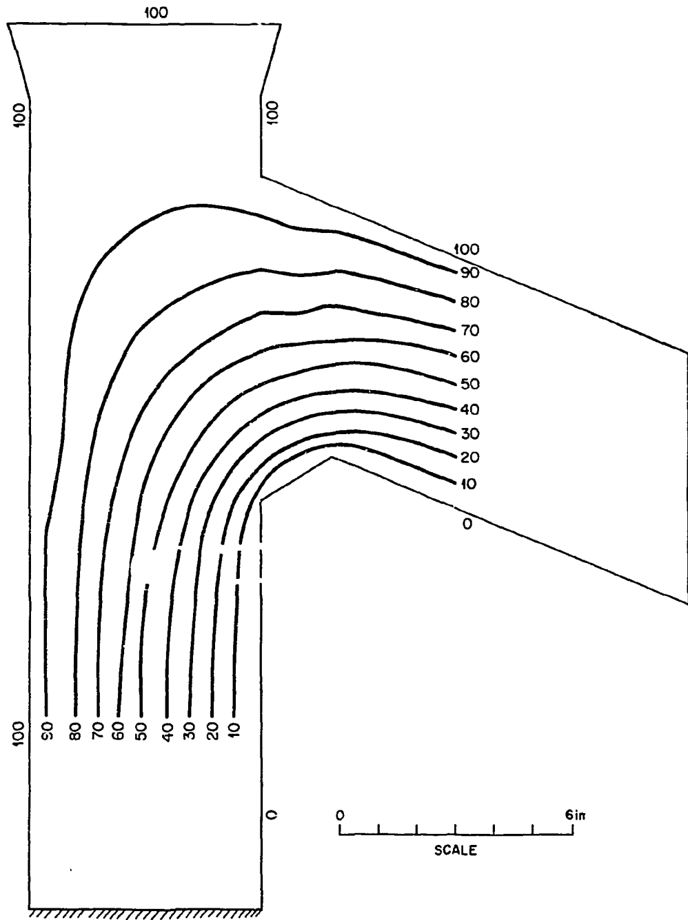
Fig. 15. Calculated current distribution at the junction of the electrode sidearm and the flucration section in autoresistance heating test AHT-3. The percentage of total current flowing between two stream lines is equal to the difference between the numbers on the stream lines.
