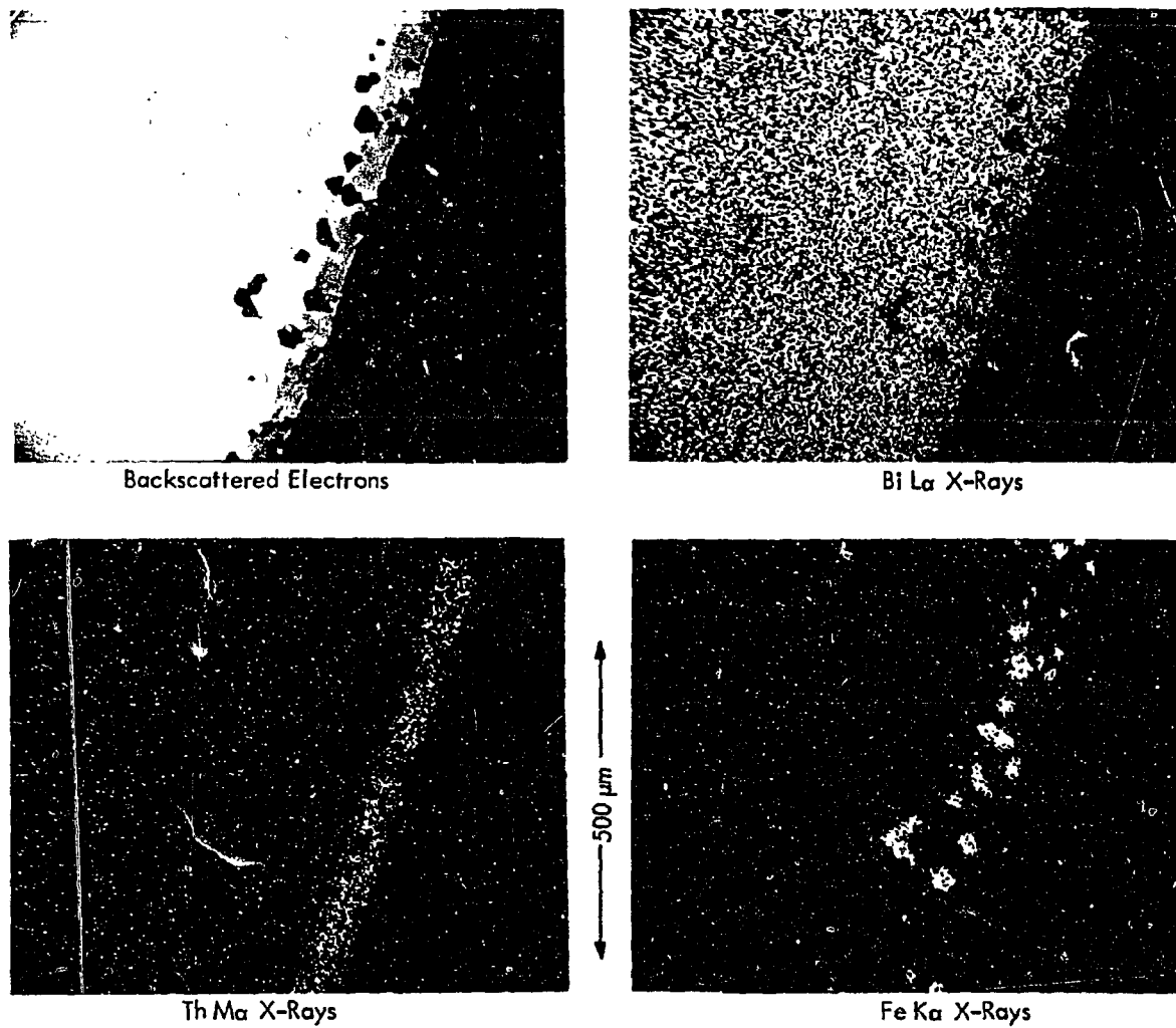
Fig. 11. Electron beam scanning images of elements in the Bi-Th phase from the contactor at the fluoride salt interface in experiment MTE-3.
