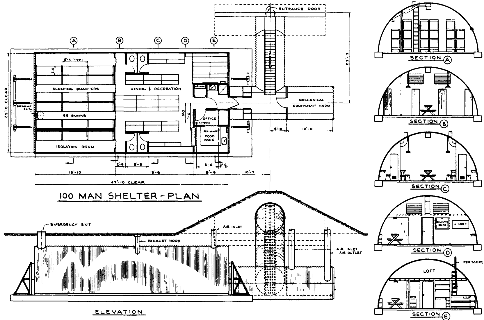
Fig. 2 —Plan and elevation of group shelter.
