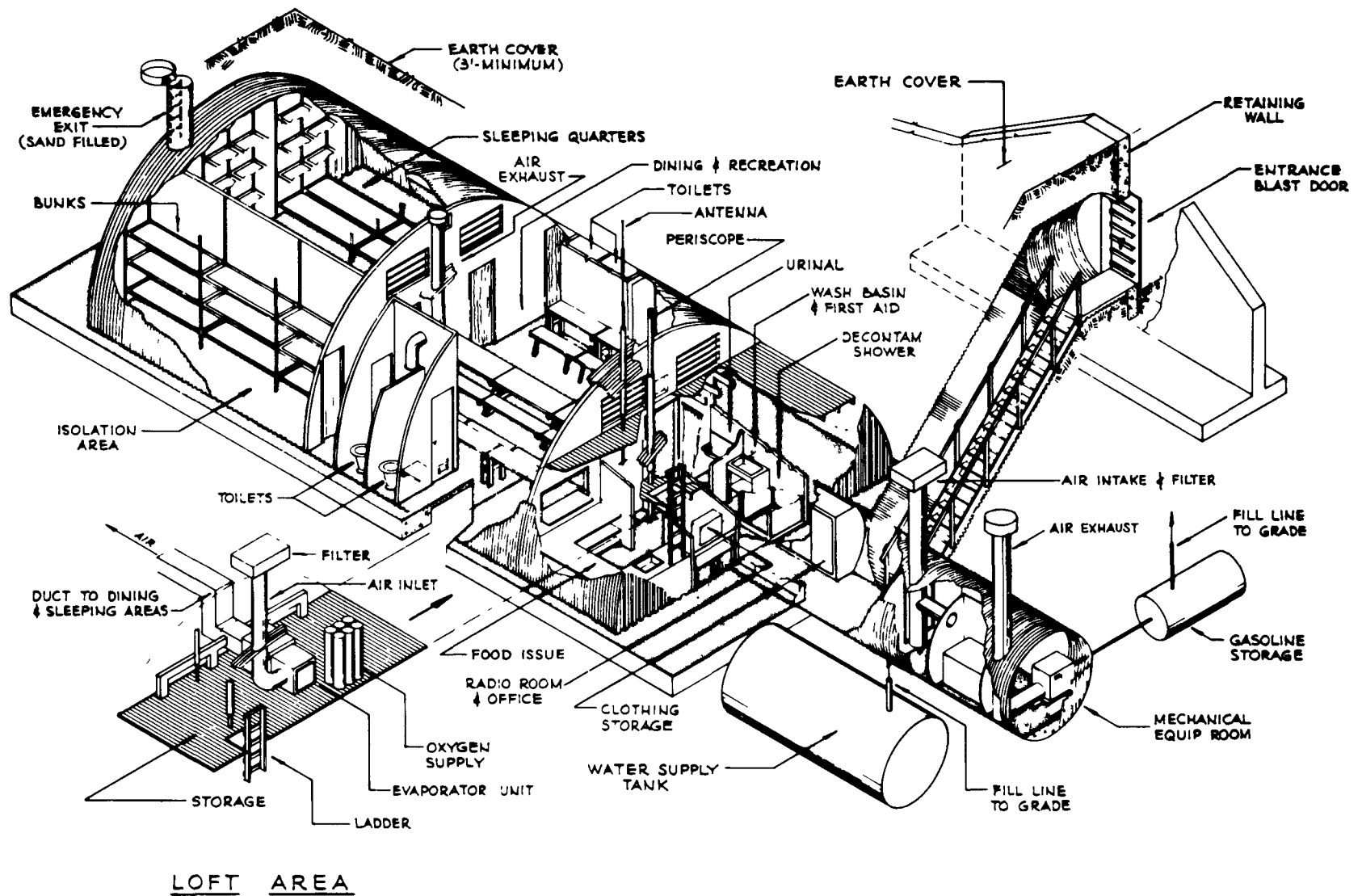
Fig. 1—Cutaway view of group shelter.
