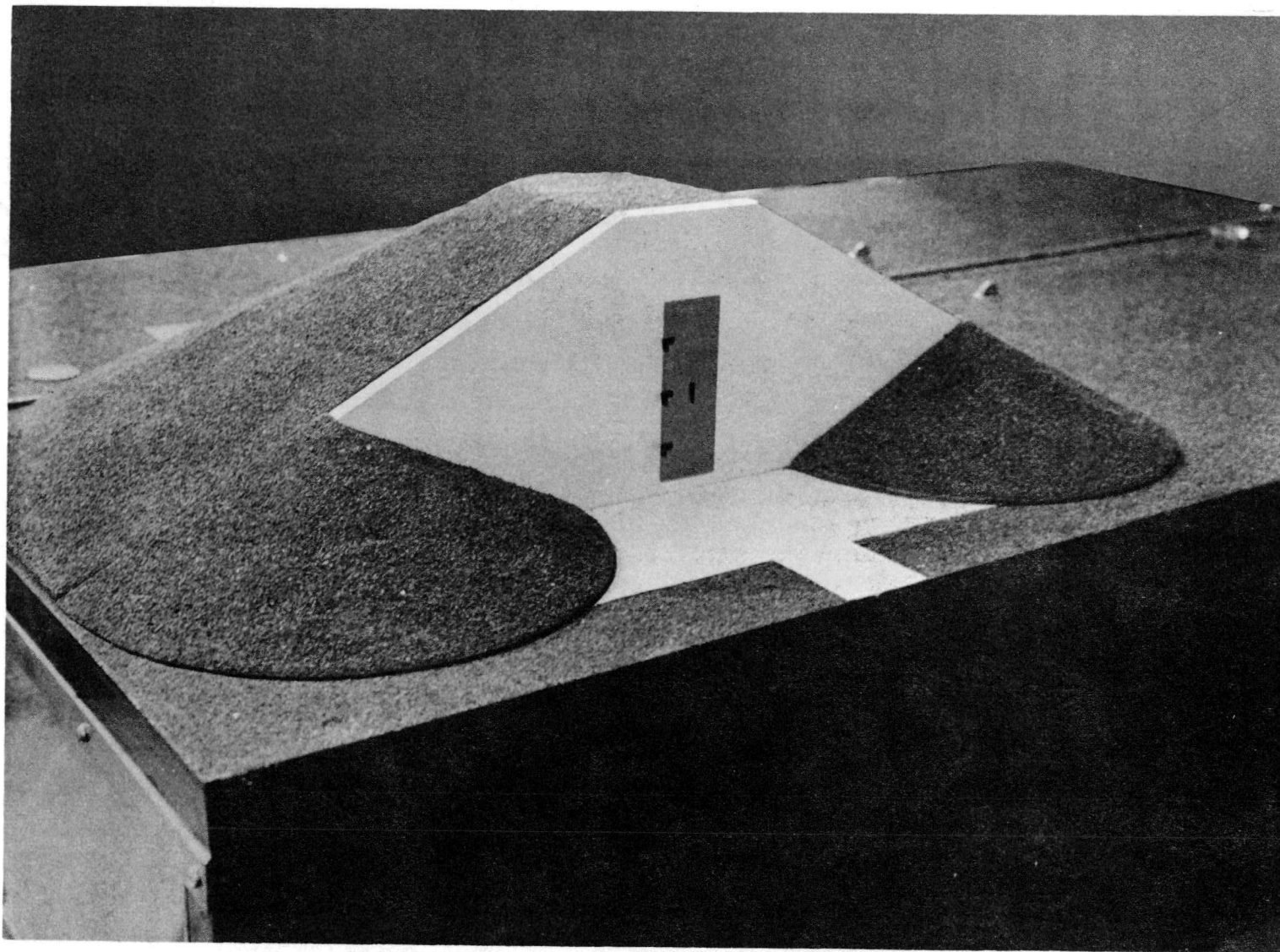
Fig. 4—Photograph of shelter model, cover in place.
