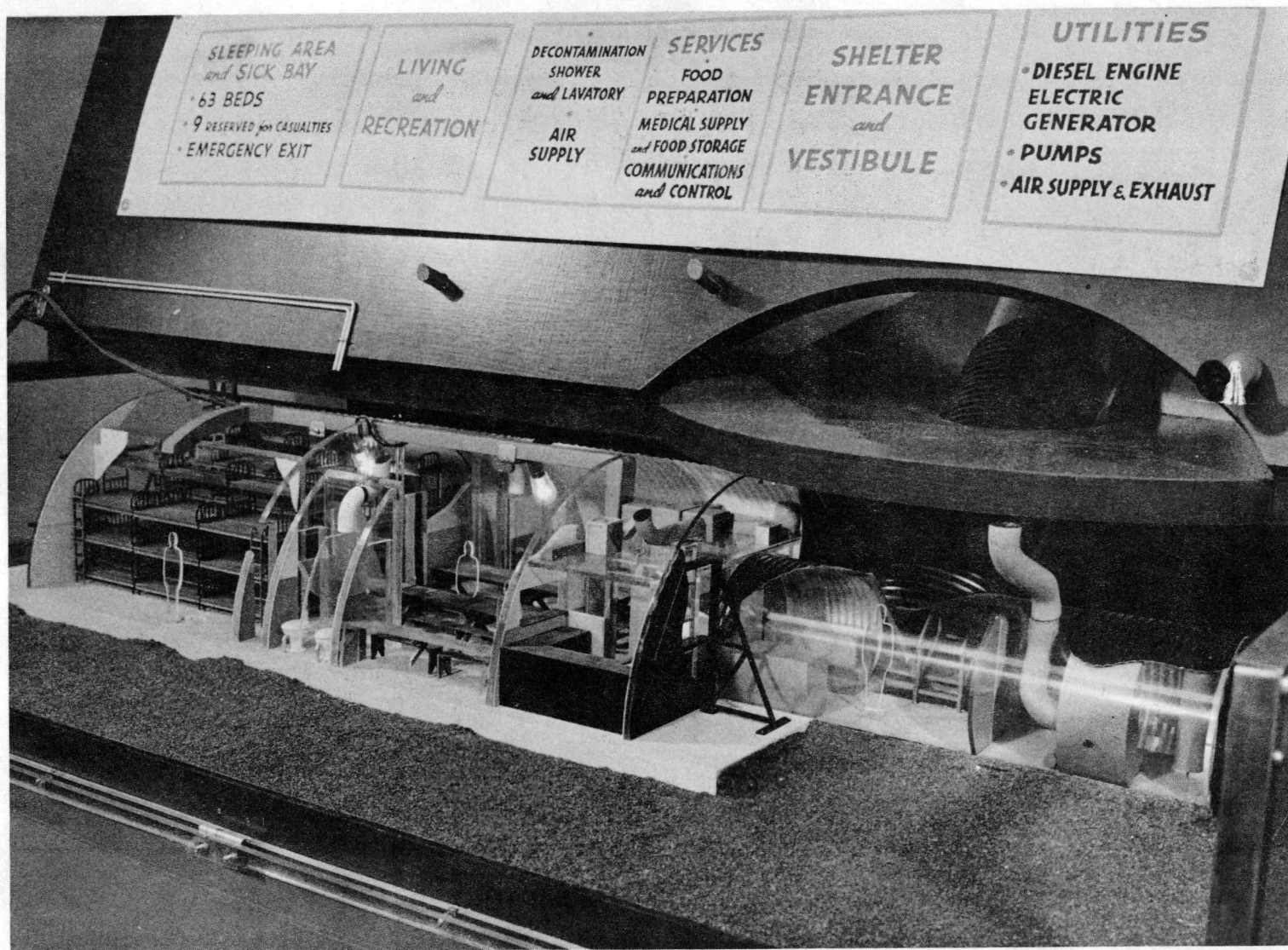
Fig. 7— Photograph of shelter model, cover removed.
