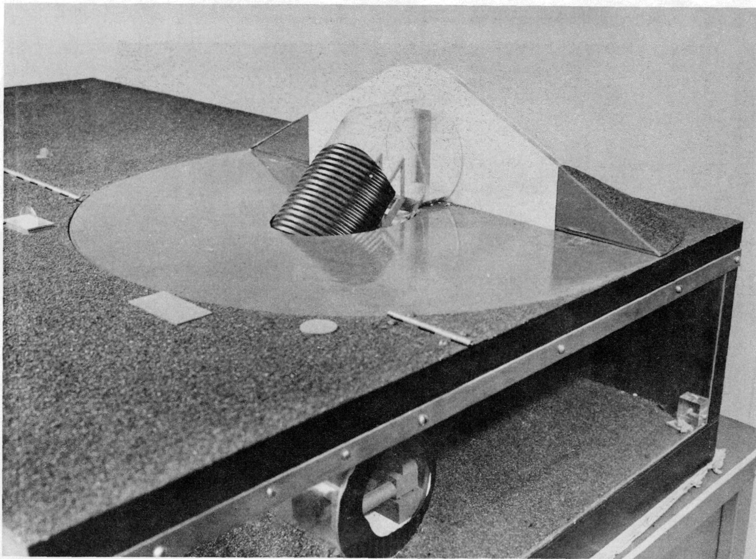
Fig. 5— Photograph of shelter model, part of cover removed.
