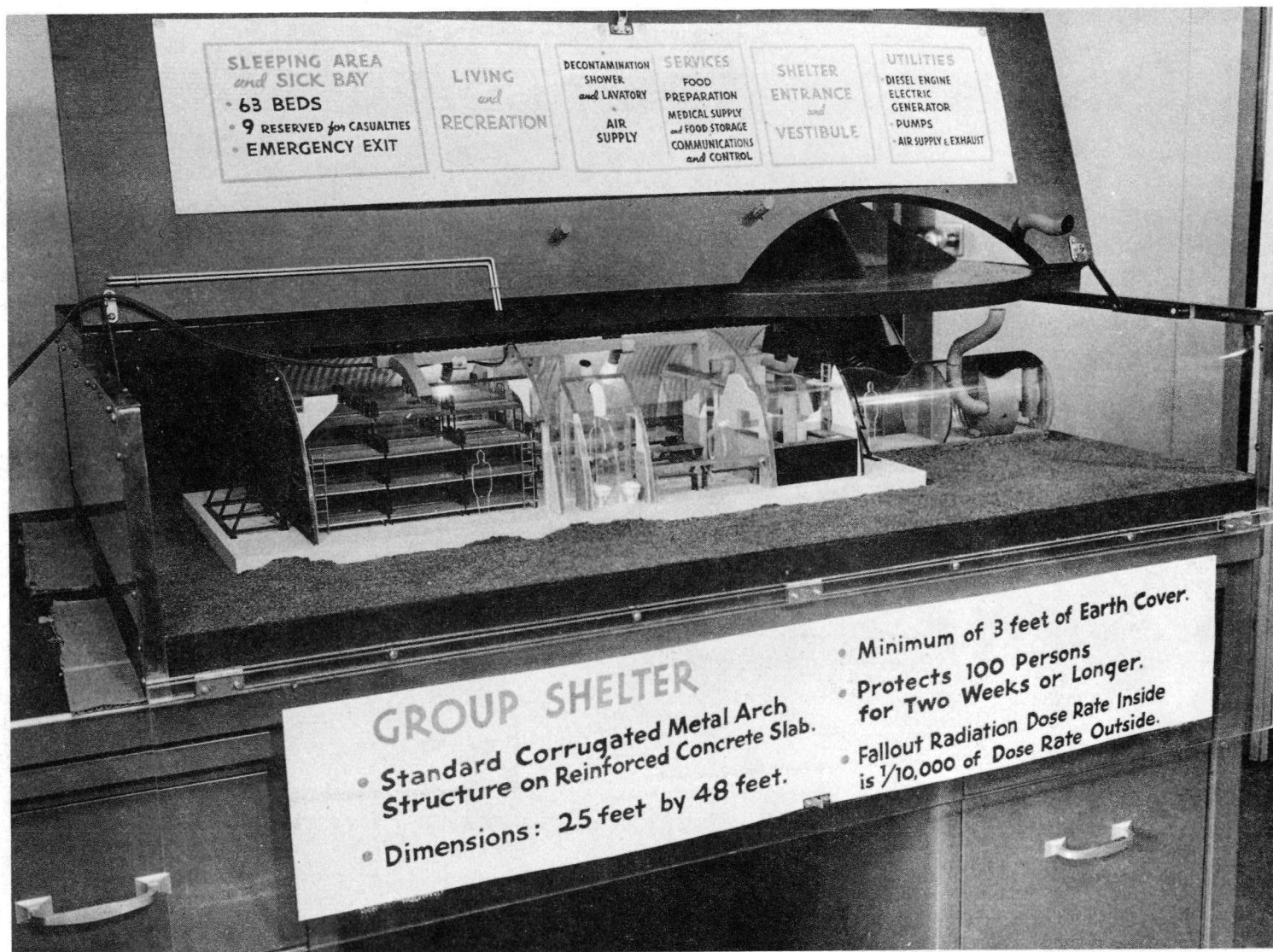
Fig. 6 — Photograph of shelter model, cover removed.
