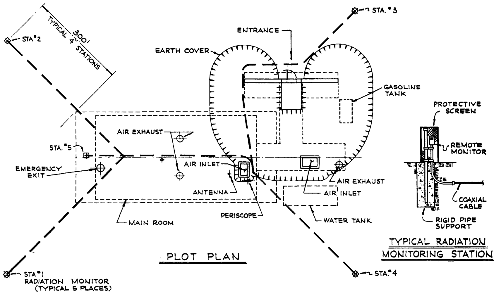
Fig. 3—Plot plan, showing position of monitoring stations.
