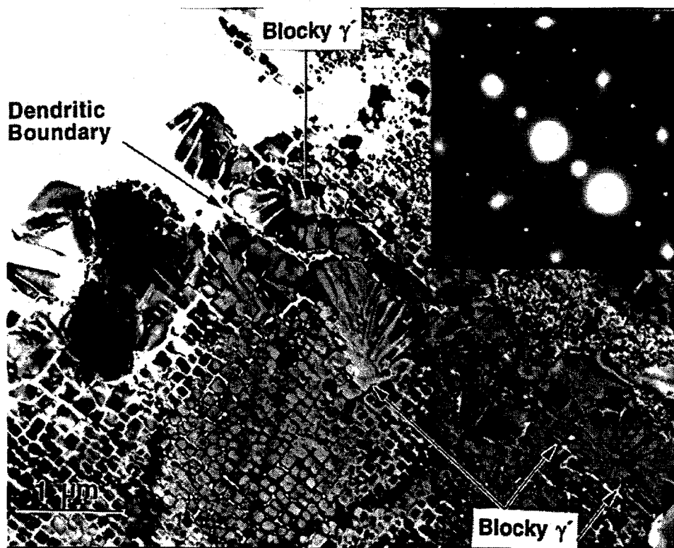
Fig. 9. Transmission electron micrograph of the PWA-1480 weld metal region in the as-welded condition showing dendritic boundary and eutectic \gamma' precipitate (marked by an arrow) along the dendritic boundary. The electron diffraction pattern (inset), taken near to the [001]_{\gamma} zone, shows the superlattice reflections from \gamma' precipitates.
