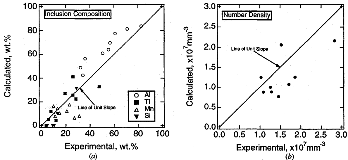
Fig. 7. Comparison of experimental inclusion characteristics measured by Kluken and Grong [50] and the calculated inclusion characteristics by the present inclusion model: (a) inclusion composition and (b) inclusion number density.
