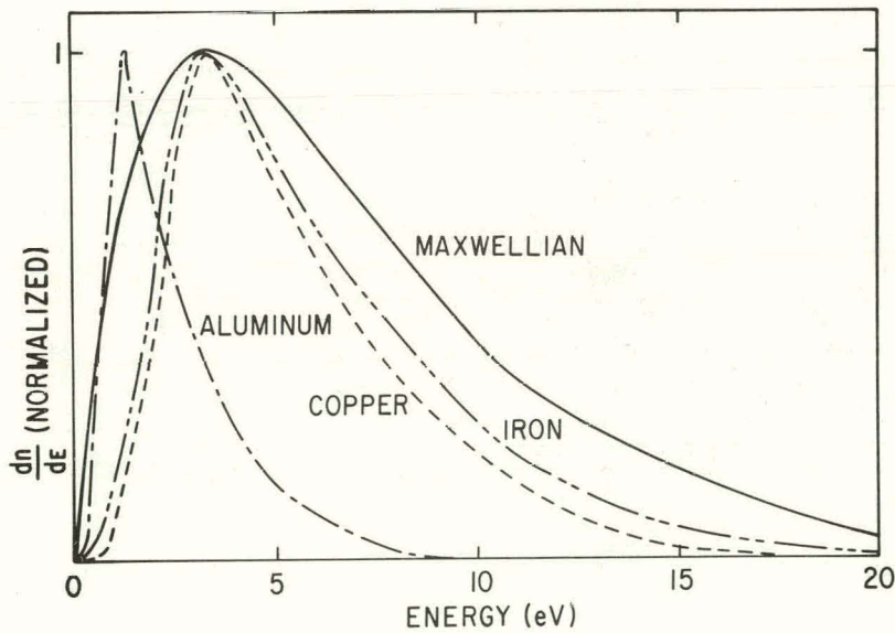
Fig. 4. Energy distributions, dn/dE , for copper, iron, and aluminum. The Maxwellian distribution has a temperature of 3.3 eV.
