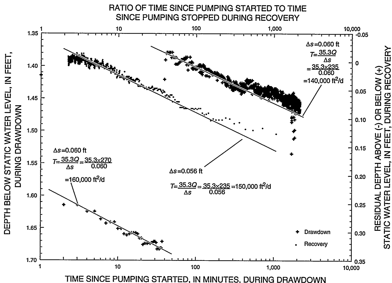
Figure 9. Analysis of water-level drawdown and recovery during aquifer test at well JF-3, Jackass Flats, Nevada, March 4-5, 1992. Water levels are corrected for effects of atmospheric pressure.
