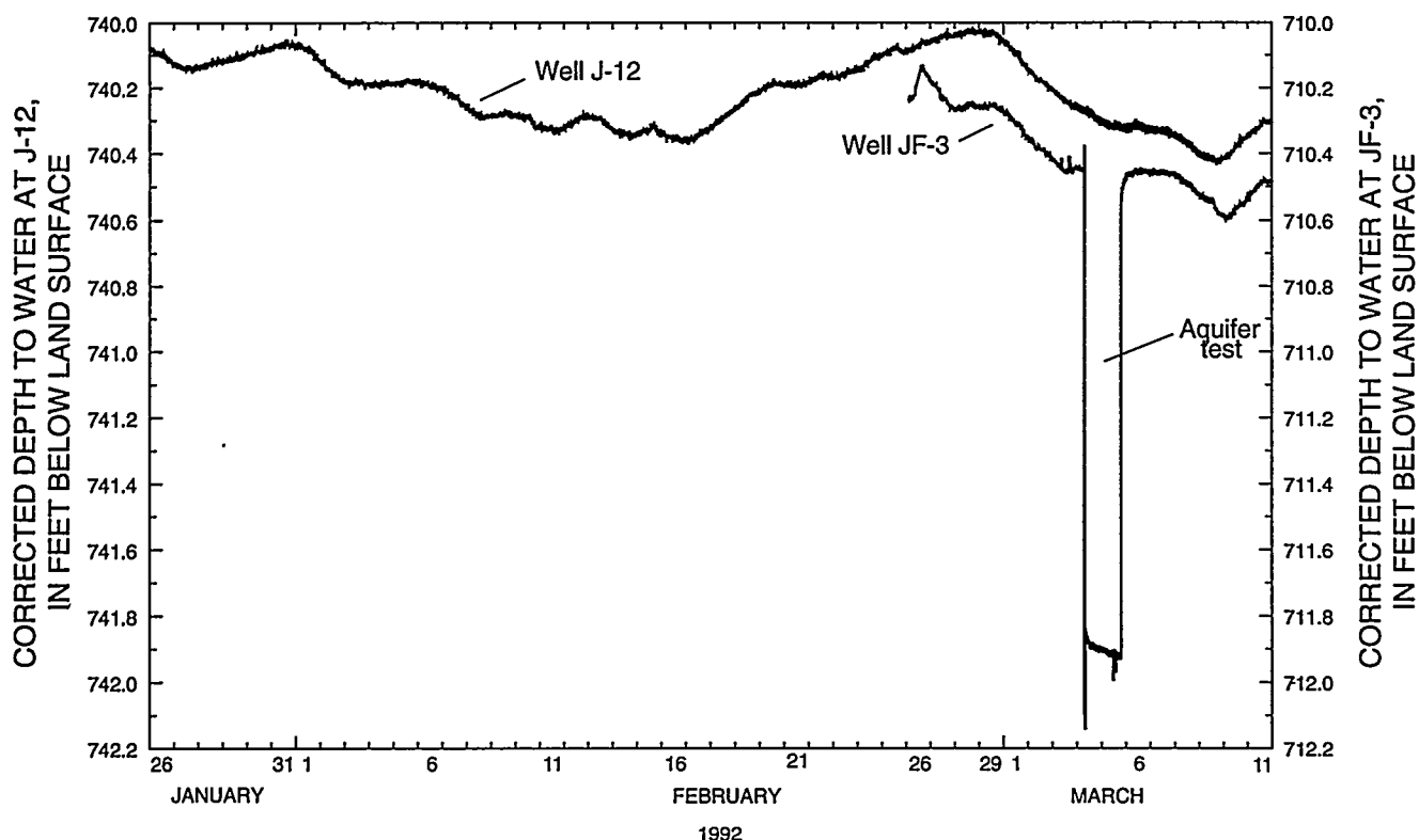
Figure 7. Depth to water at wells J-12 and JF-3, Jackass Flats, Nevada, corrected for effects of atmospheric pressure, January 26-March 11, 1992.
