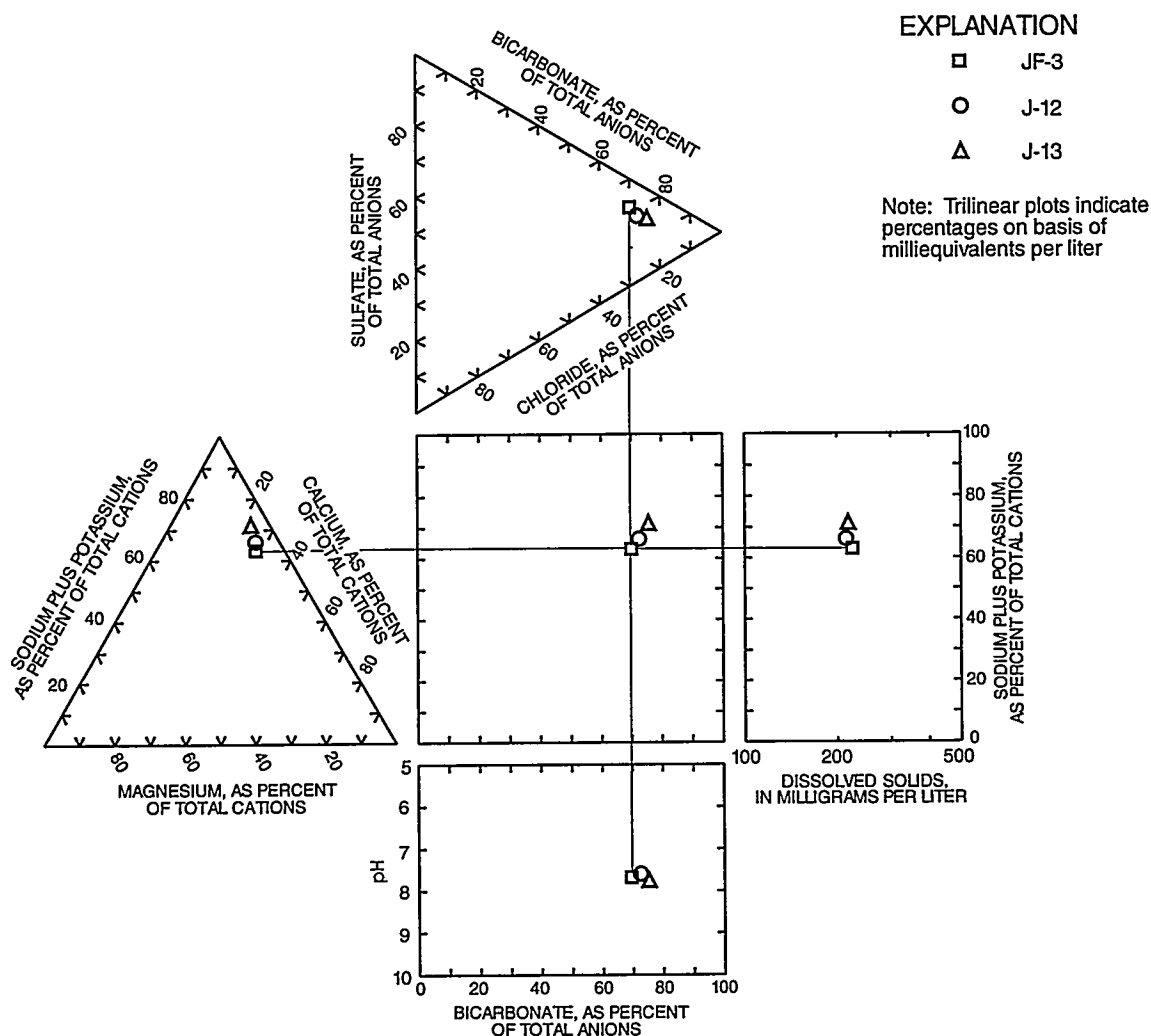
Figure 10. General chemical quality of ground water at wells JF-3, J-12, and J-13, Jackass Flats, Nevada. Data from La Camera and Westenburg (1994, p. 121-123).
