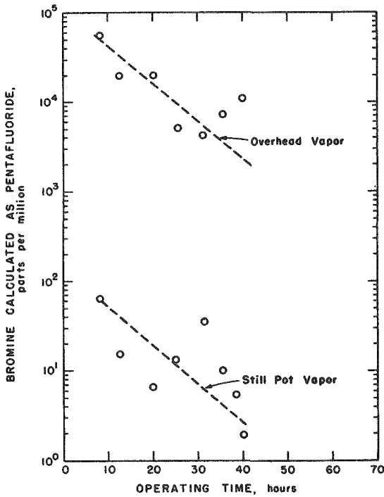
FIGURE 12. URANIUM HEXAFLUORIDE-BROMINE PENTAFLUORIDE DISTILLATION. Run C-5
