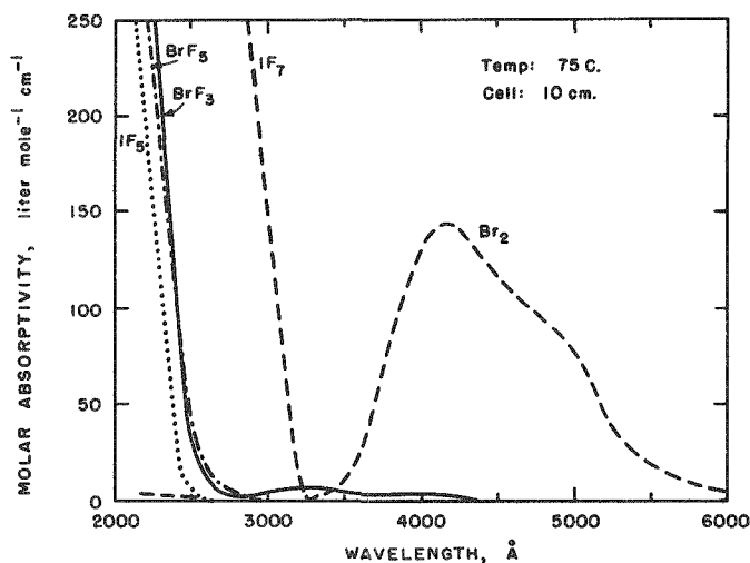
FIGURE 9. ABSORPTION SPECTRA OF \text{Br}_2 , \text{BrF}_3 , \text{BrF}_5 , \text{IF}_5 , AND \text{IF}_7 .
