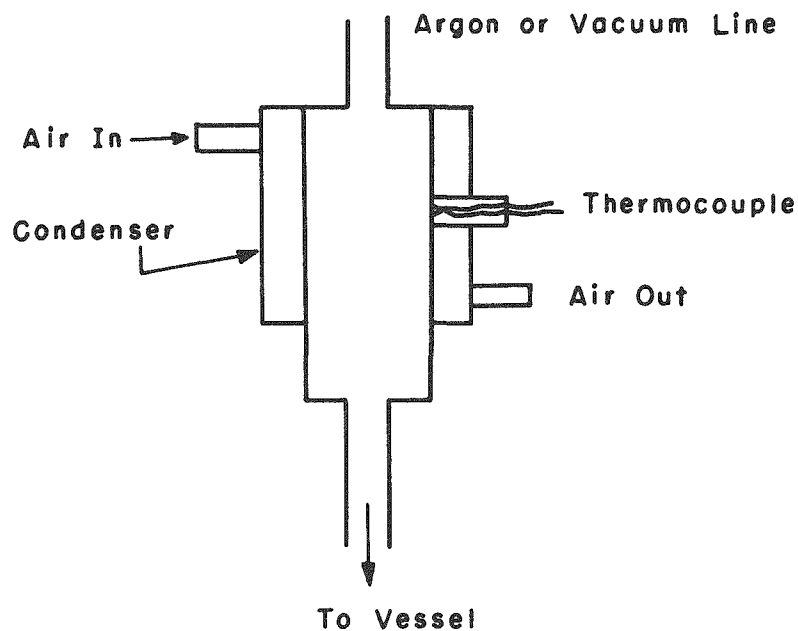
Figure 40 Vapor Pressure Trap
