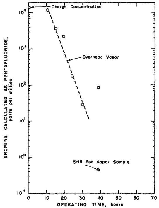
FIGURE 13. URANIUM HEXAFLUORIDE-BROMINE PENTAFLUORIDE DISTILLATION. Run C-6 (Continuous Fluorine Bleed)
