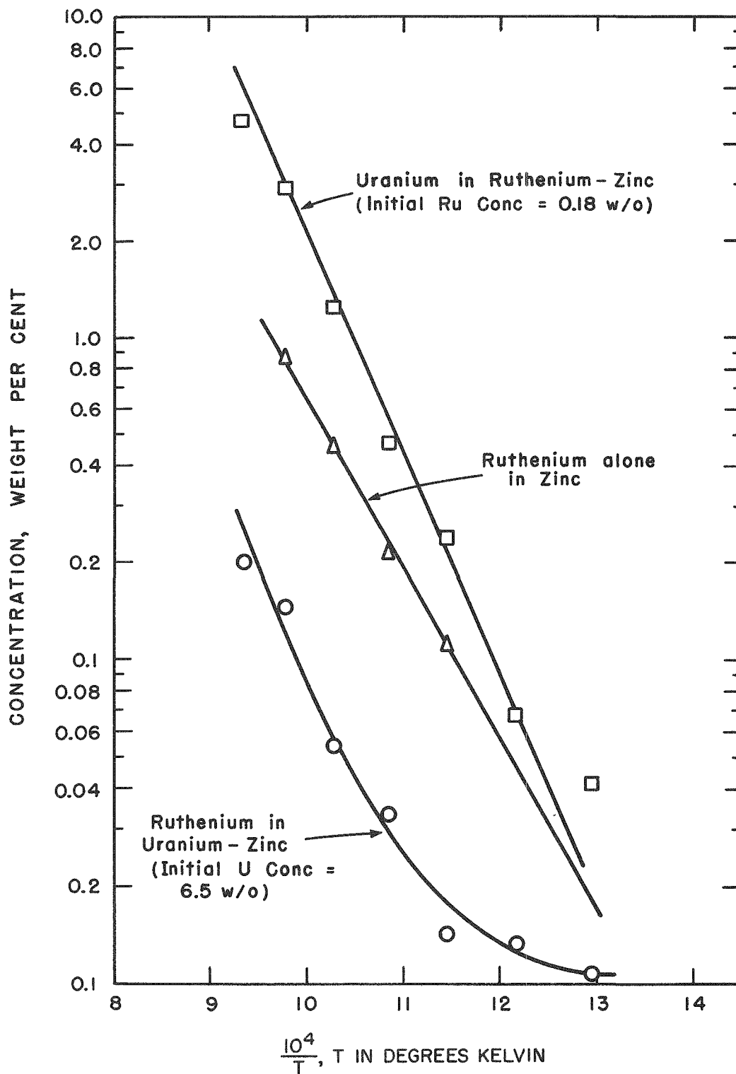
FIGURE 38. RUTHENIUM AND URANIUM SOLUBILITIES IN THE SYSTEM URANIUM - RUTHENIUM - ZINC.
