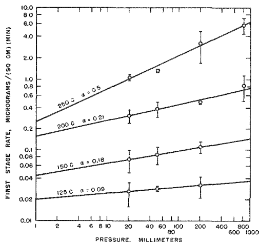
FIGURE 21 FIRST STAGE PRESSURE DEPENDENCE. -\frac{dw}{dt} = kP^a
