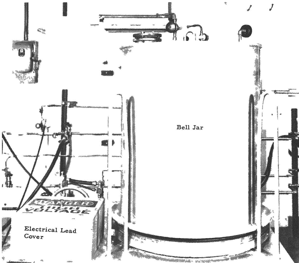
Bell Jar Cover in Position
