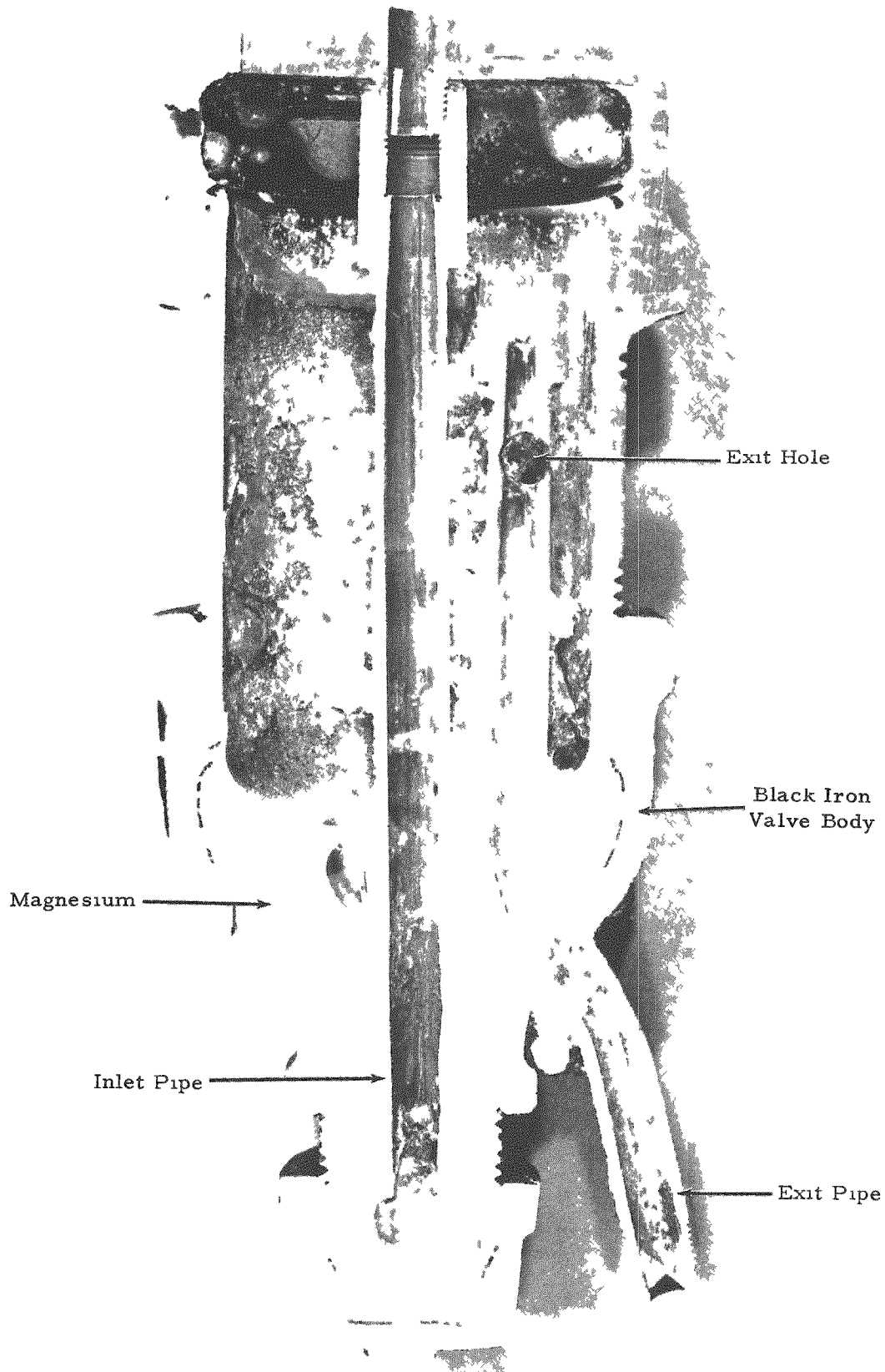
Figure 42 Sectioned Magnesium Freeze Valve
