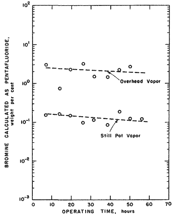
FIGURE 13. URANIUM HEXAFLUORIDE-BROMINE PENTAFLUORIDE DISTILLATION. Run C-6 (Continuous Fluorine Bleed)
