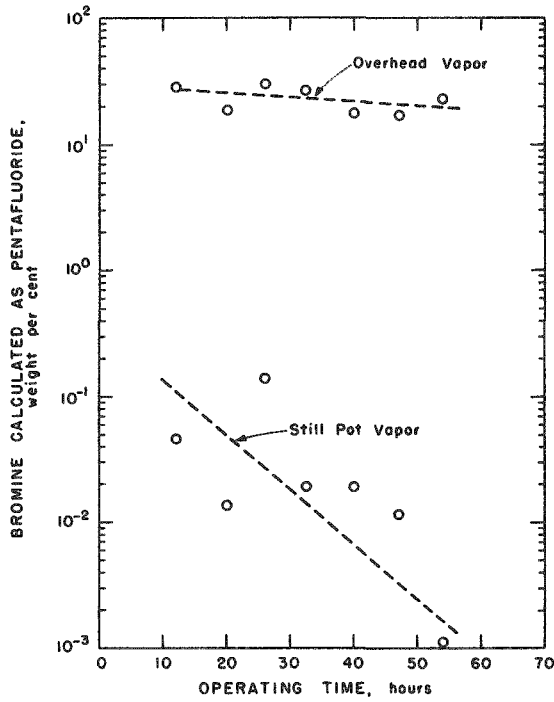
FIGURE 10. URANIUM HEXAFLUORIDE-BROMINE PENTAFLUORIDE DISTILLATION. Run C-3
