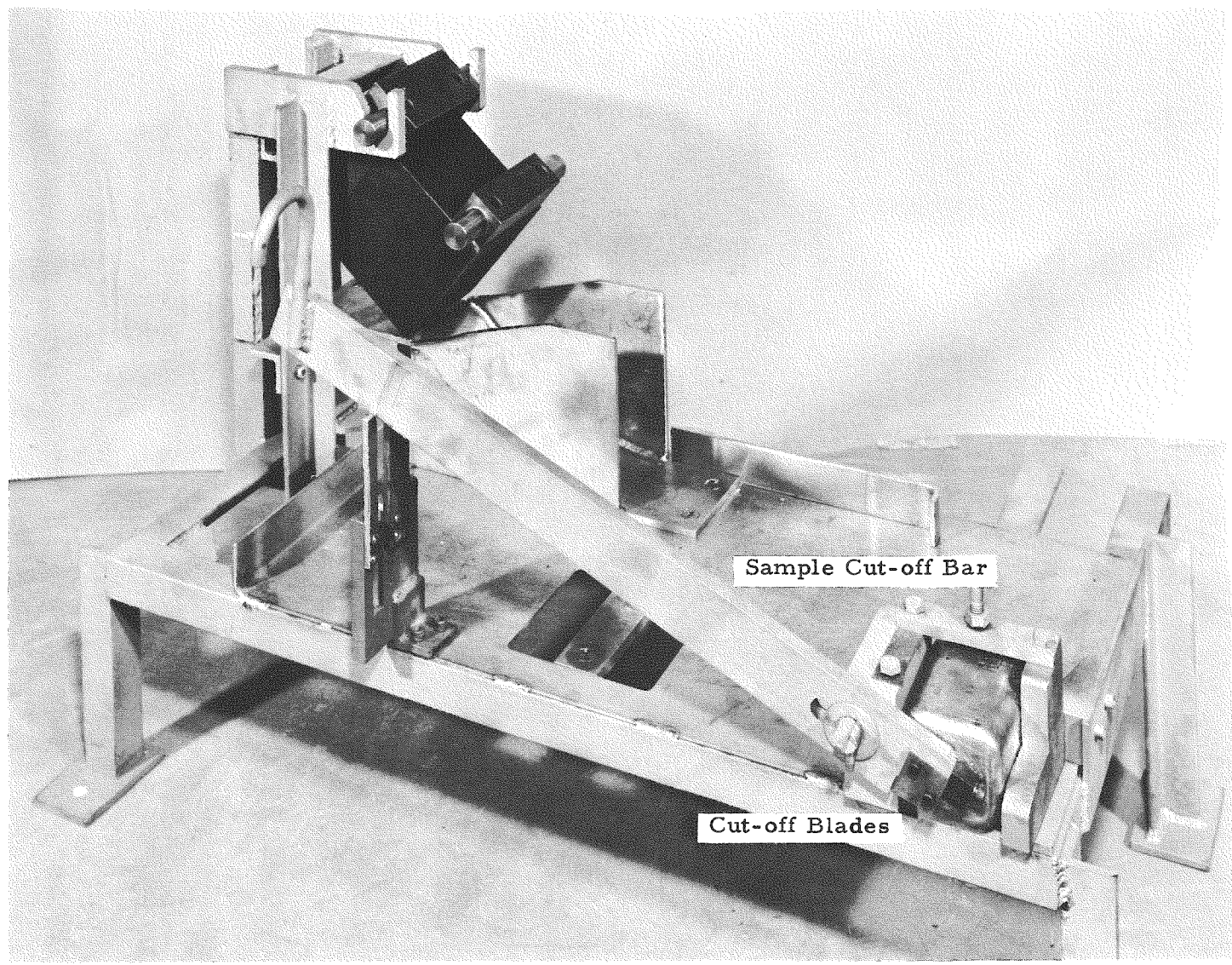
Ingot Remover and Sampler
