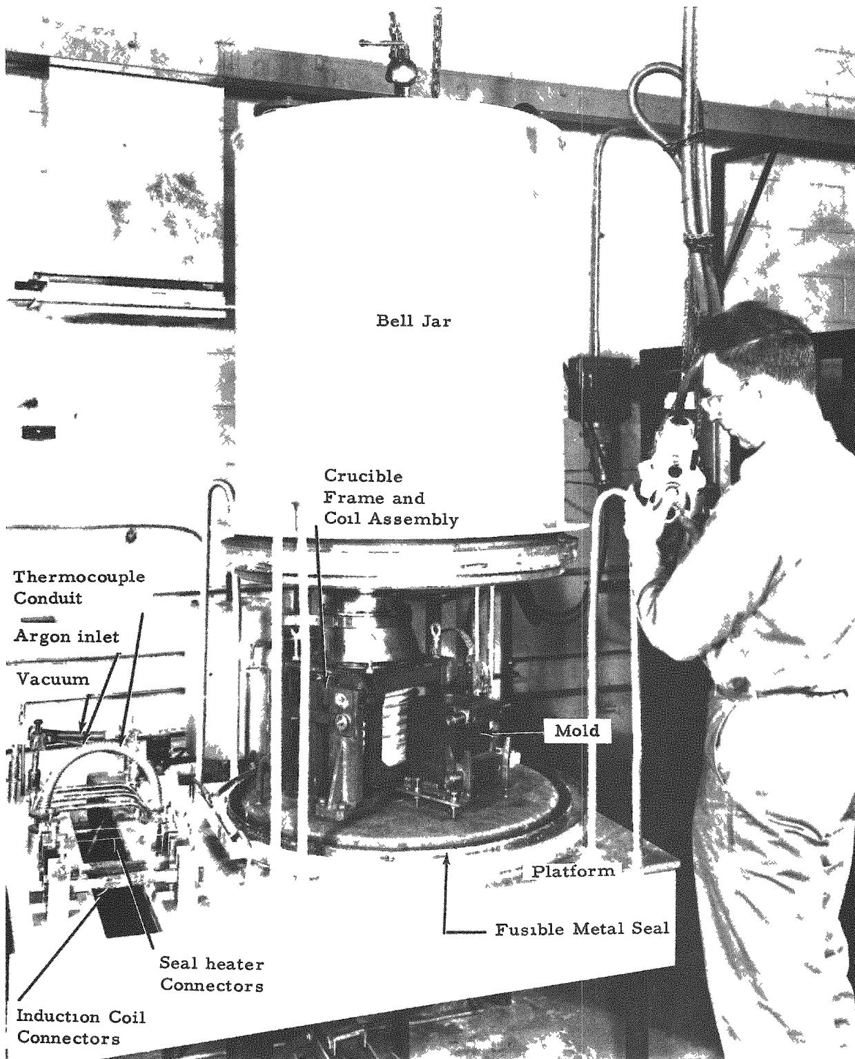
Uranium Melting Furnace - Bell Jar Partially Removed.
