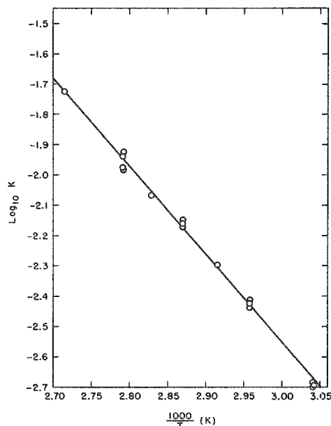
FIGURE 6. DETERMINATION OF THE ACTIVATION ENERGY FOR THE REACTION IF_5 + F_2 \rightarrow IF_7 .
