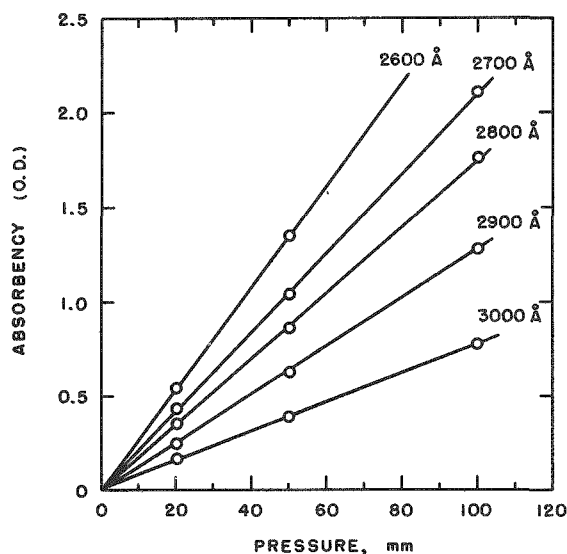
FIGURE 7. BEER'S LAW BEHAVIOR OF IODINE HEPTAFLUORIDE. Optical Path of Cell: 10 cm Temperature: 25 C.
