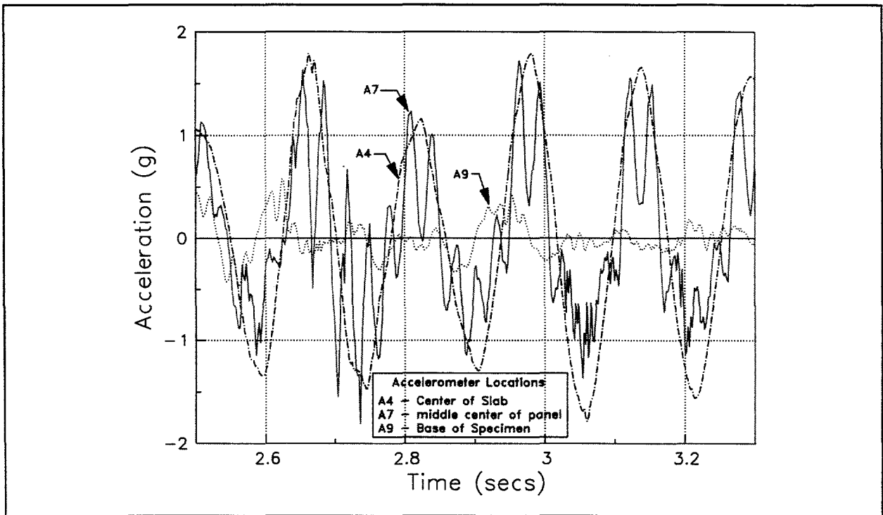
Figure 3: Accelerometer readings from the third seismic test
