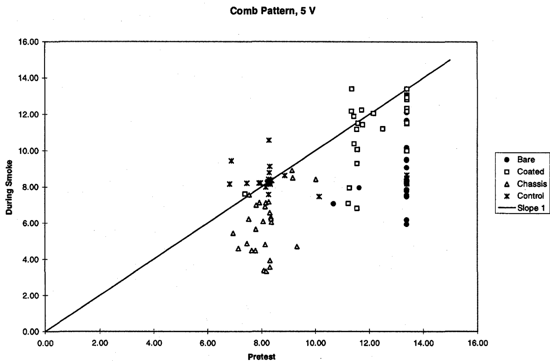
Figure 28. Comb Pattern, 5 V, \text{Log}_{10}(R) Pretest vs. During smoke
