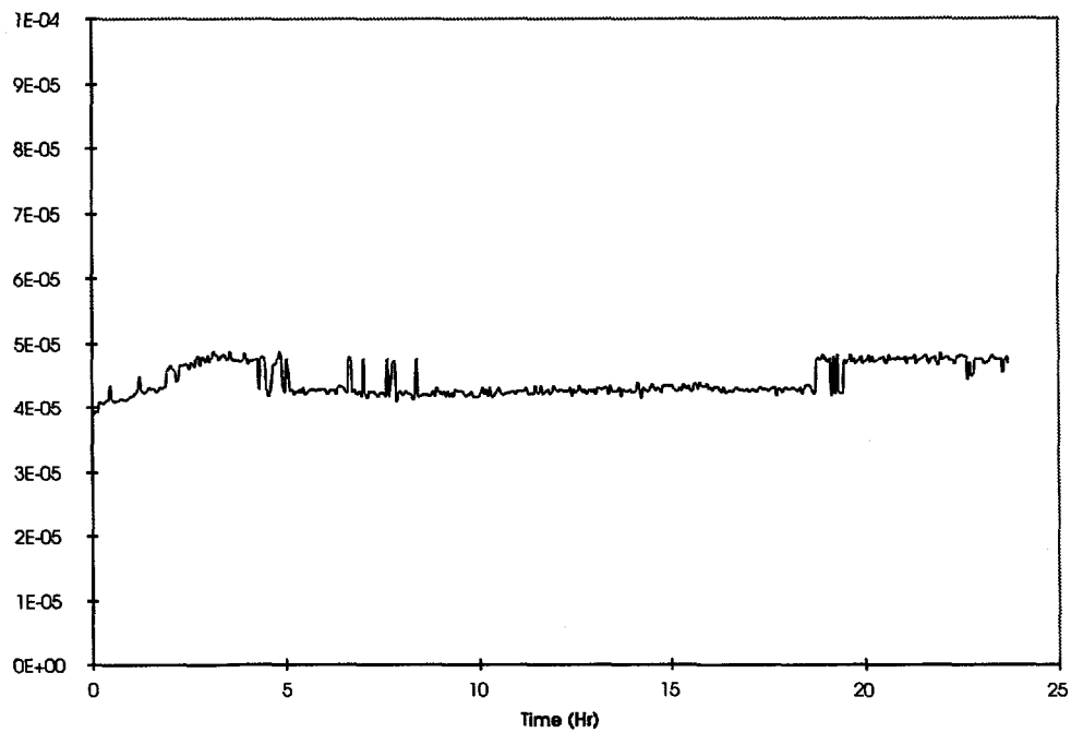
Figure 17. Optical isolator rise time from test 5
