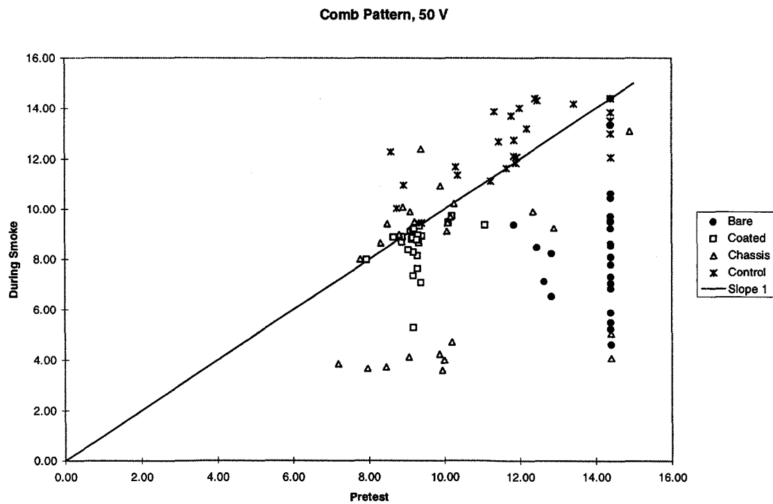
Figure 25. Comb Pattern, 50 V, \log_{10}(R) Pretest vs. During smoke
