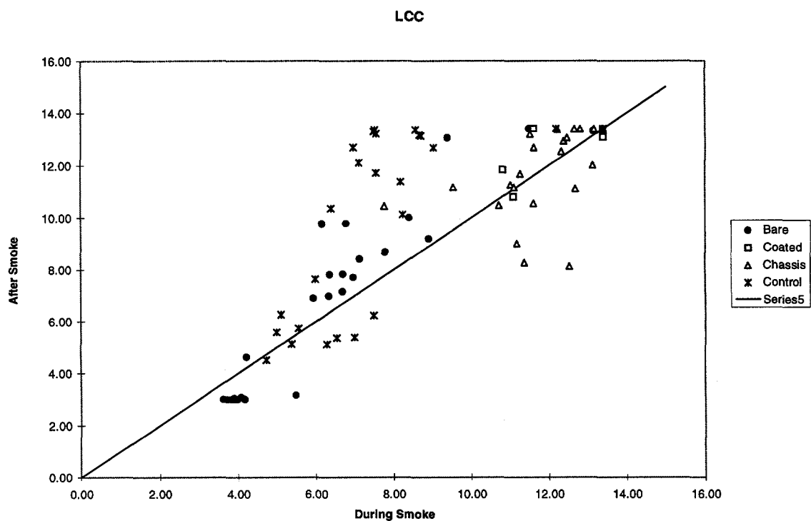
Figure 3. Leadless Chip Carrier \log_{10}(R) During Smoke vs. After Smoke
