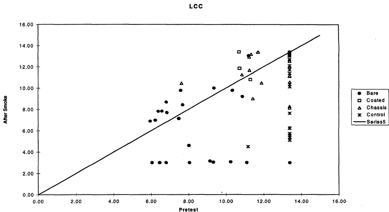
Figure 2. Leadless Chip Carrier \log_{10}(R) Pretest vs. After Smoke
