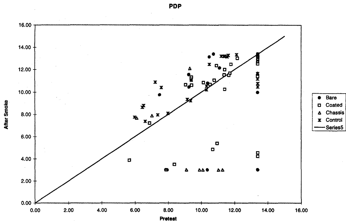
Figure 20. Plastic DIP Log 10 (R) Pretest vs. After smoke
