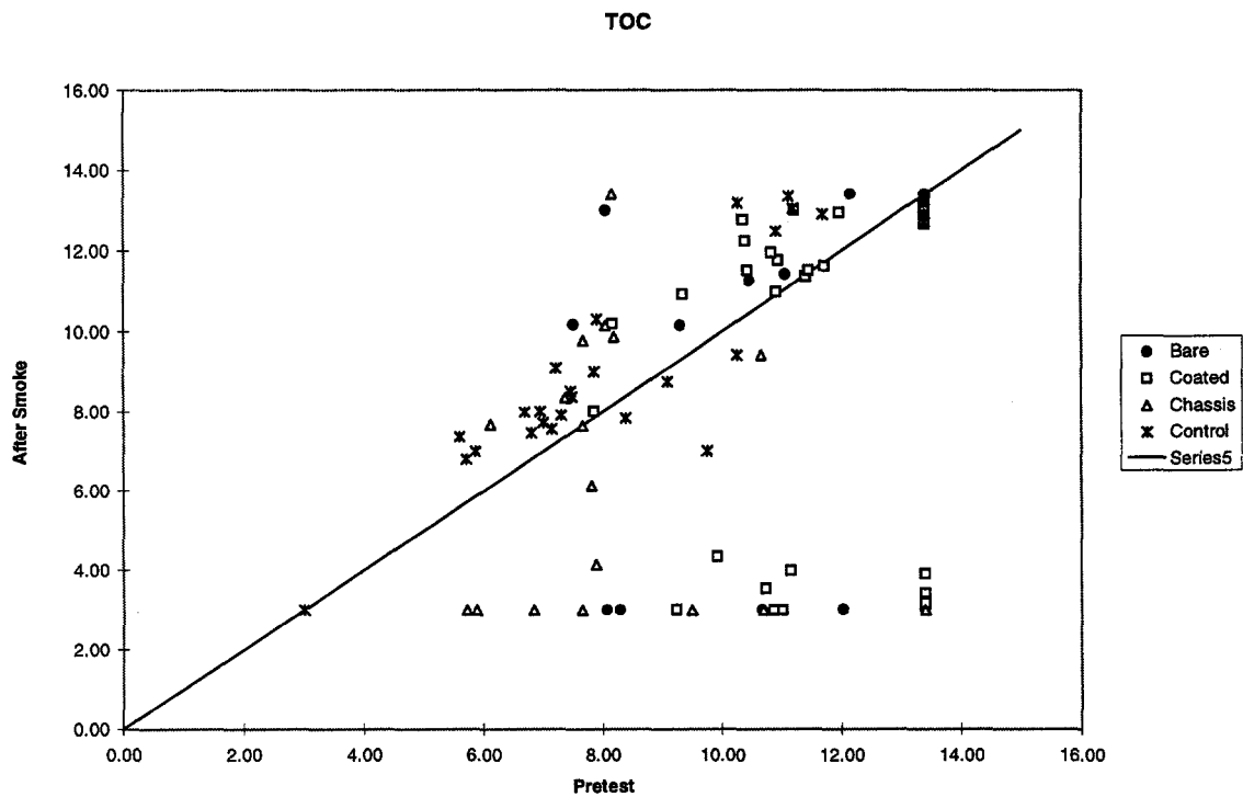
Figure 11. Transistor Outline Can \log_{10}(R) Pretest vs. After smoke
