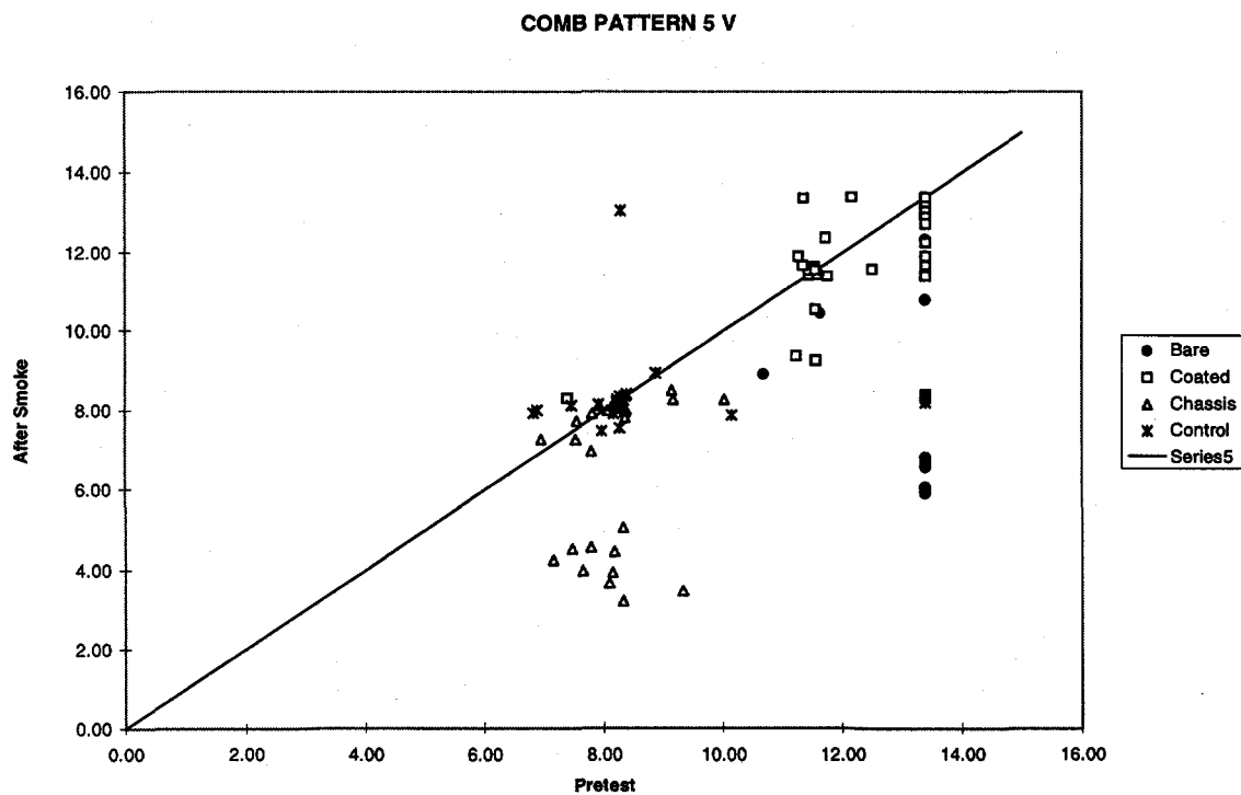
Figure 29. Comb Pattern, 5 V, \text{Log}_{10}(R) Pretest vs. After smoke
