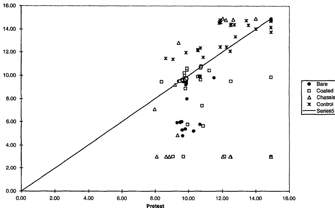
Figure 11. \text{Log}_{10}(R) after exposure compared with pretest for 160 V comb patterns.
