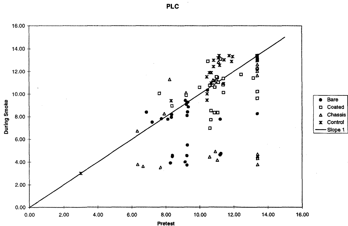
Figure 13. Plastic Leaded Chip Carrier \text{Log}_{10}(\text{R}) Pretest vs. During smoke
