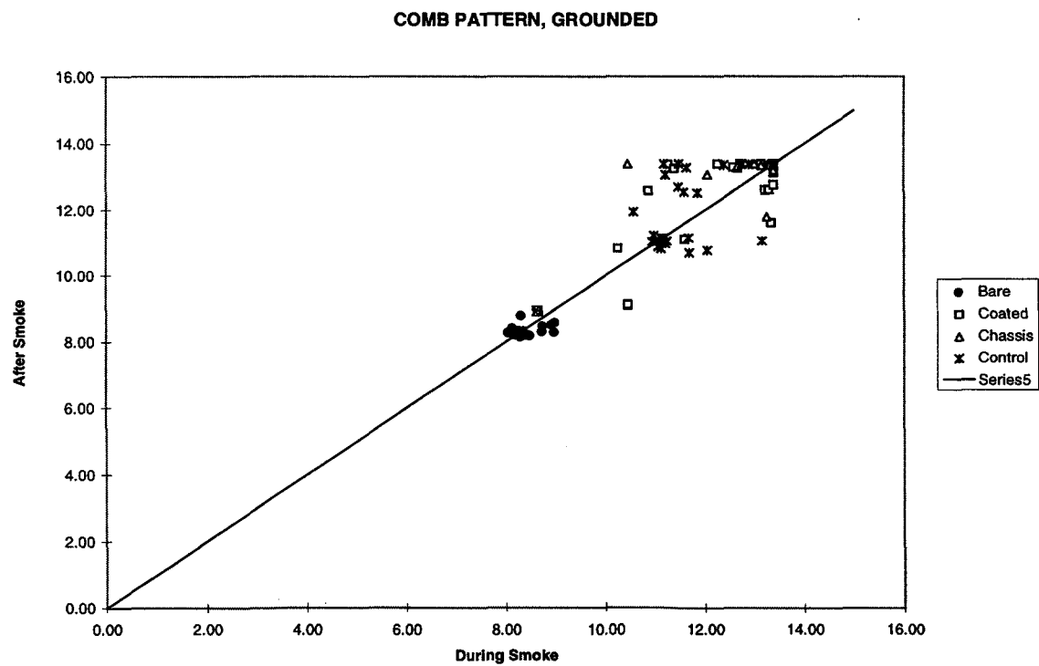
Figure 33. Comb Pattern, Grounded, \text{Log}_{10}(R) During smoke vs. After smoke
