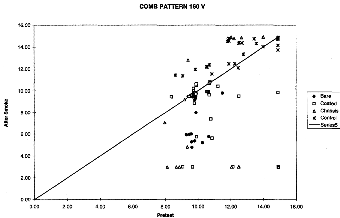
Figure 23. Comb Pattern, 160 V, \log_{10}(R) Pretest vs. After smoke
