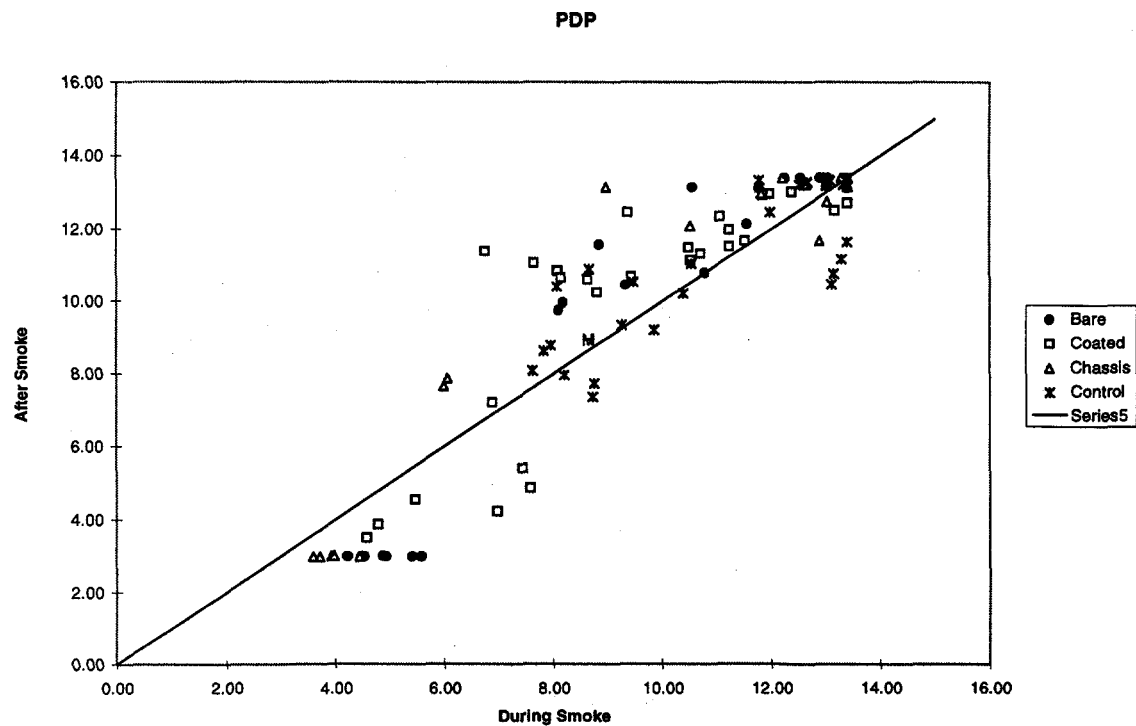
Figure 21. Plastic DIP Log 10 (R) During smoke vs. After smoke
