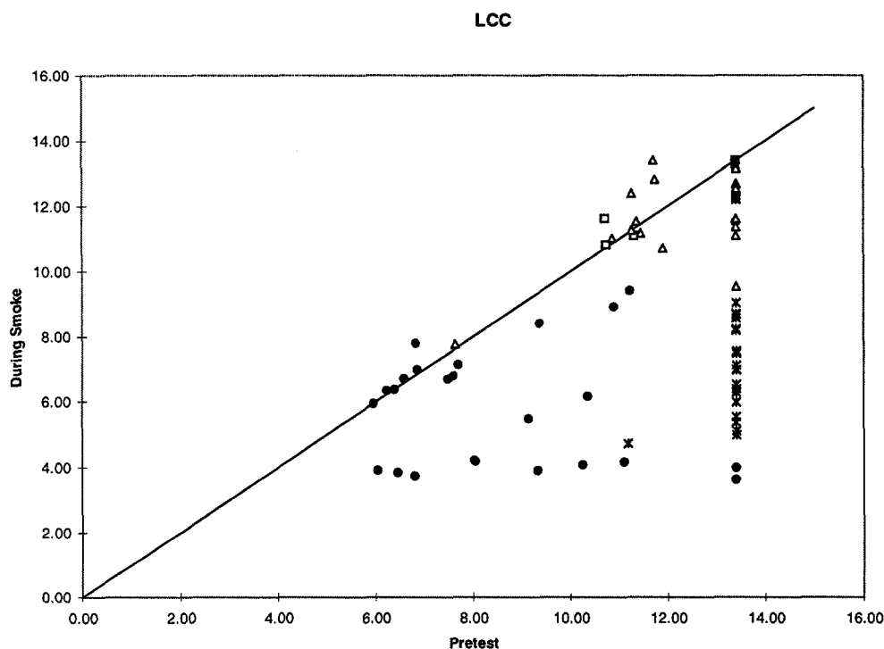
Figure 1. Leadless Chip Carrier \log_{10}(R) Pretest vs. During Smoke
