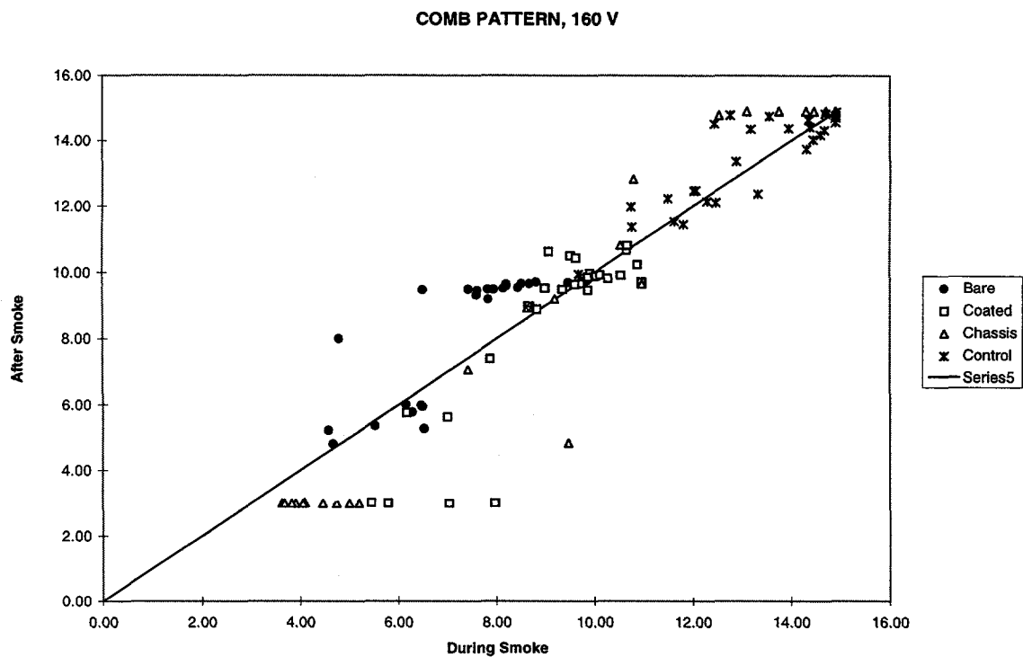
Figure 24. Comb Pattern, 160 V, \log_{10}(R) During smoke vs. After smoke
