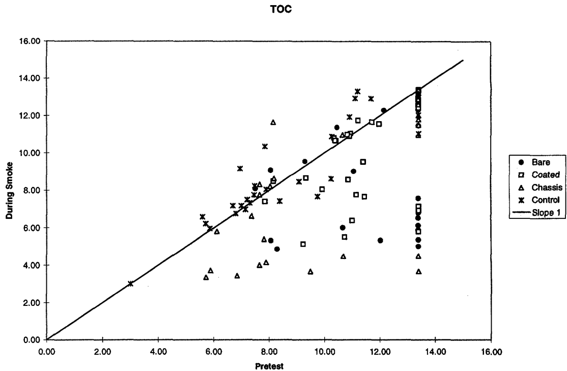
Figure 10. Transistor Outline Can \log_{10}(R) Pretest vs. During smoke
