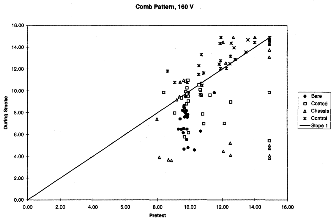
Figure 22. Comb Pattern, 160 V, \log_{10}(R) Pretest vs. During smoke
