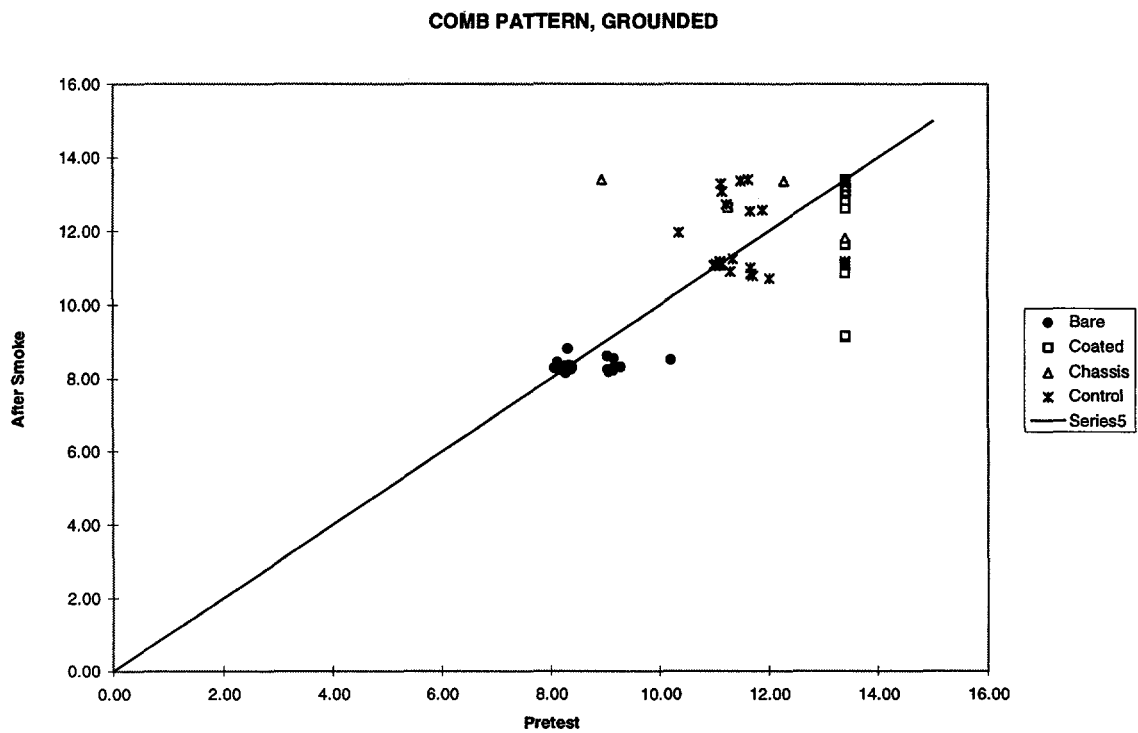
Figure 32. Comb Pattern, Grounded, \text{Log}_{10}(R) Pretest vs. After smoke
