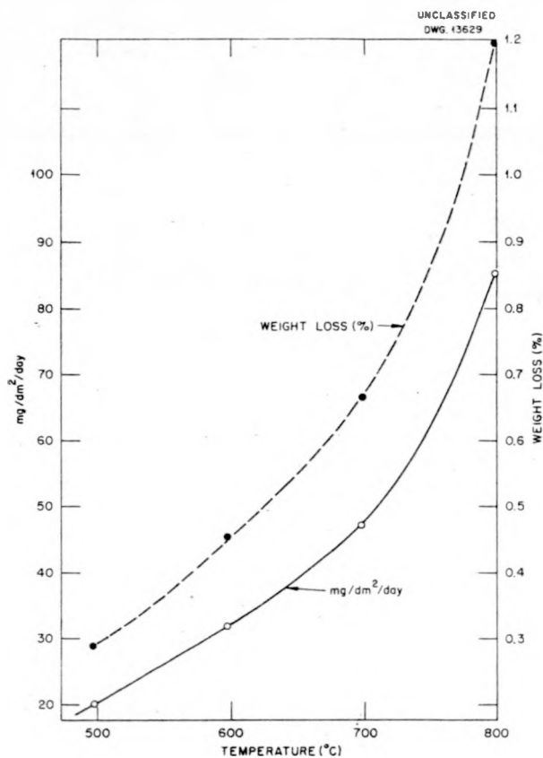
Fig. 11.11. Weight Loss of Inconel Specimen in Potassium Hydroxide for 100 hr as a Function of Temperature.
