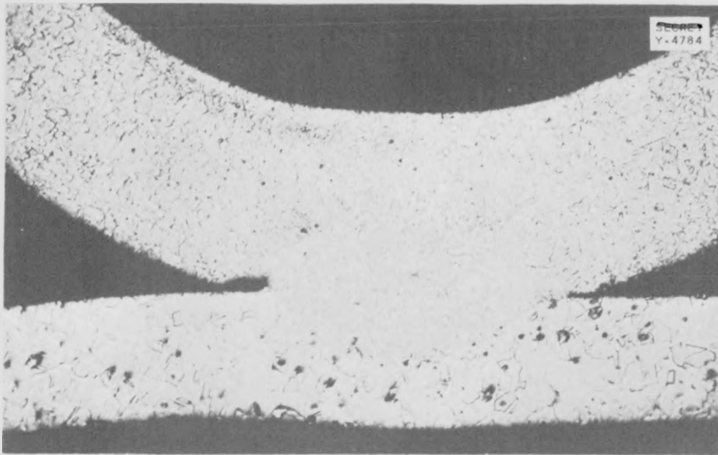
Fig. 13.5. Transverse Section of a 0.015-in.-Thick Inconel Sheet Spot Welded to an 0.188-in.-o.d. Inconel Tube of 0.025-in. Wall Thickness. Etchant, aqua regia and glycerin. 175X.
