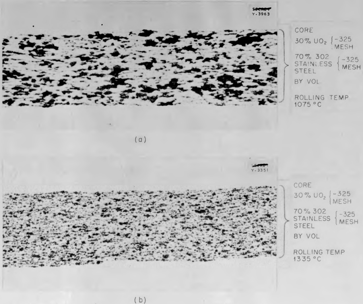
Fig. 13.2 a, b. Effect of Rolling Temperature on UO 2 Distribution. 175X.
