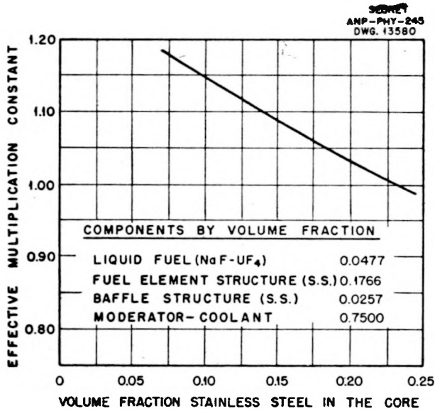
Fig. 3.16. Effective Multiplication Constant as a Function of Volume Fraction of Stainless Steel in the Core for the 2½-ft-Diameter-Core NaOH-Moderated and -Cooled Reactor.
