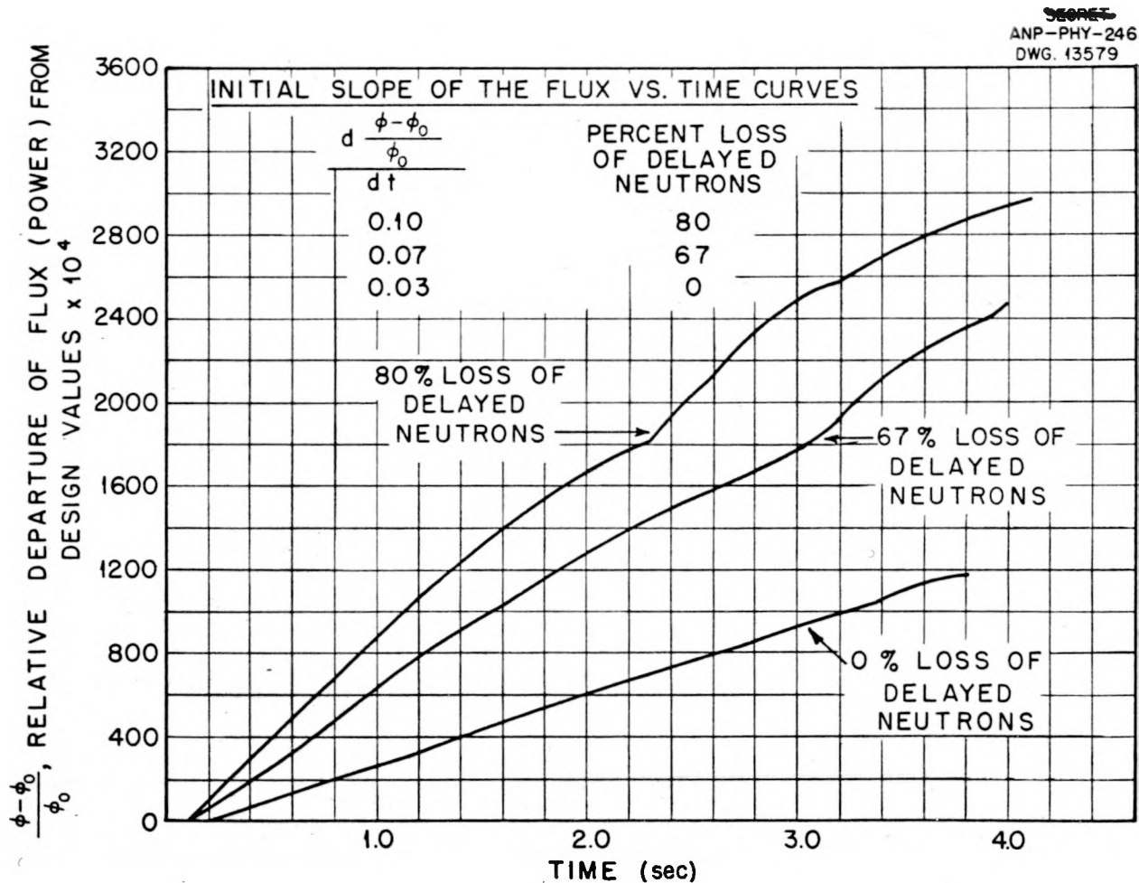
Fig. 3.15. Fractional Change in Neutron Flux as a Function of Time for 0, 67, and 80% Decrease in Delayed Neutrons.
