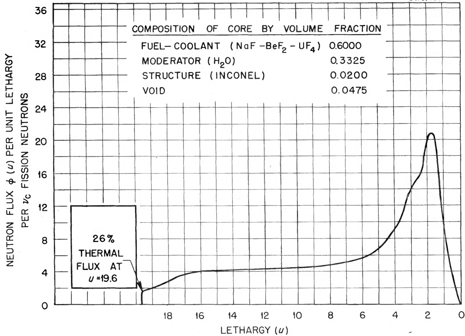
Fig. 3.13. Neutron Flux Spectrum vs. Lethargy for the H 2 O-Moderated Circulating-Fuel Reactor with 3-ft-Diameter Core.
