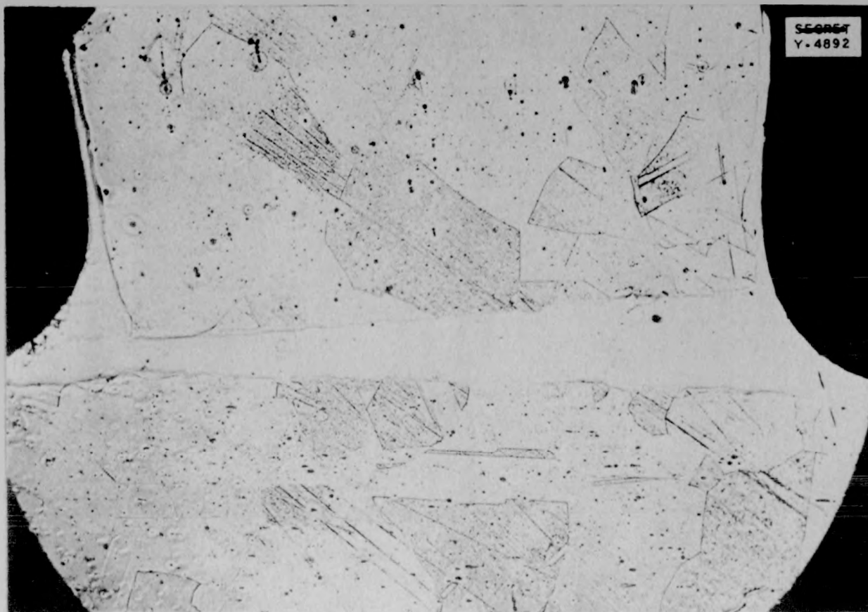
Fig. 13.9. Transverse Section of an Inconel Tube-to-Header Joint Brazed with a 60% Pd - 40% Ni Alloy in Dry Hydrogen at 1270°C for 20 min. Etchant, aqua regia and glycerin. 75X.
