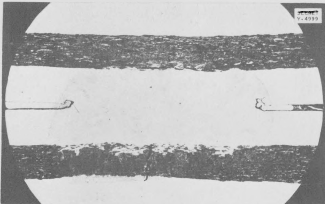
Fig. 13.6. Section of a Spot Weld Joining Two Stainless Steel—Clad Fuel Plates. Etchant, aqua regia and glycerin. 60X.
