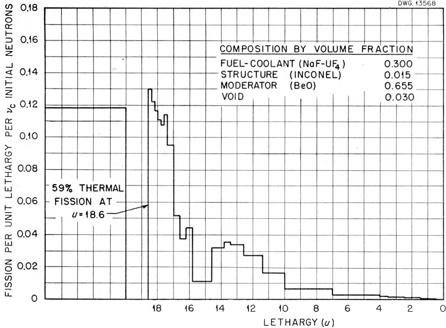
Fig. 3.4. Fission Spectrum vs. Lethargy for the BeO-Moderated Circulating-Fuel Reactor with a 3½-ft-Diameter Core.
