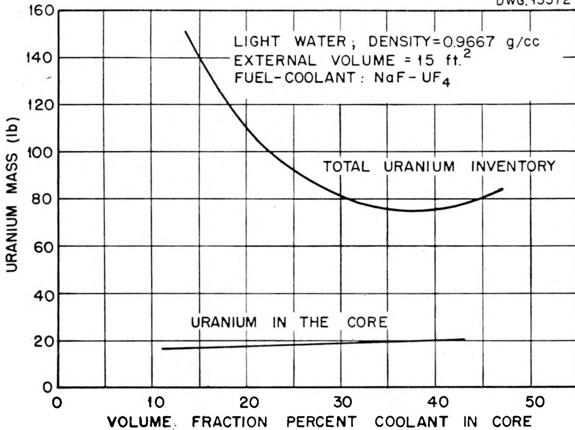
Fig. 3.8. Total Uranium Inventory and Uranium in the Core as a Function of the Volume Fraction Fuel-Coolant in the 3-ft-Diameter-Core Water-Moderated Reactor with NaF-UF 4 Fuel-Coolant.
