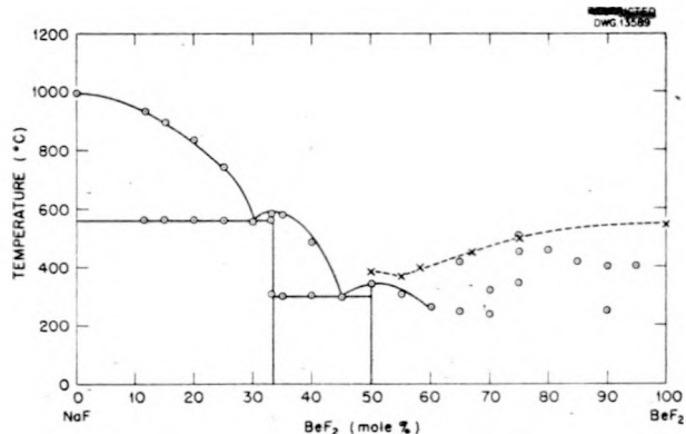
Fig. 10.3. The System NaF-BeF 2 .
