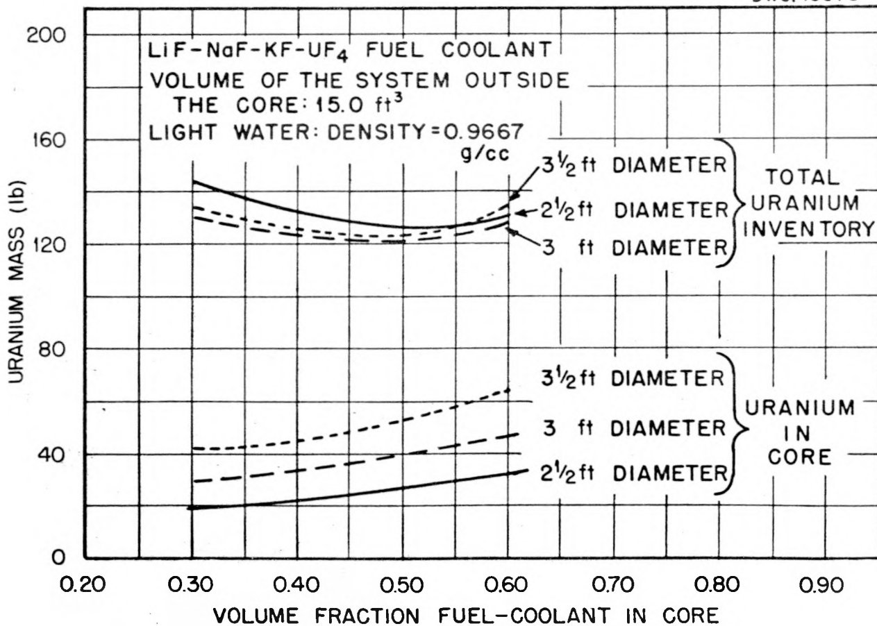
Fig. 3.14. Total Uranium Inventory and Uranium in Core as a Function of Volume Fraction Fuel-Coolant in the Core for H 2 O-Moderated Circulating-Fuel Reactors with 2½-, 3-, and 3½-ft-Diameter Cores and LiF-NaF-KF-UF 4 Fuel-Coolant.
