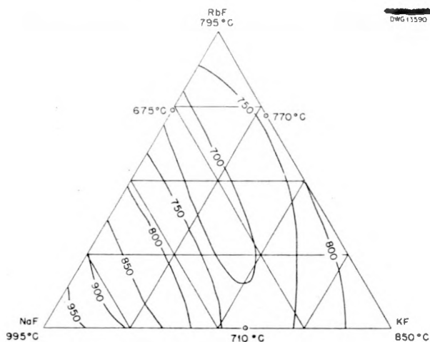
Fig. 10.4. The System NaF-KF-RbF.
