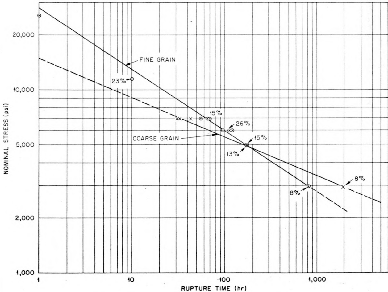
Fig. 13.10. Stress-Rupture Time for Inconel Sheet.
