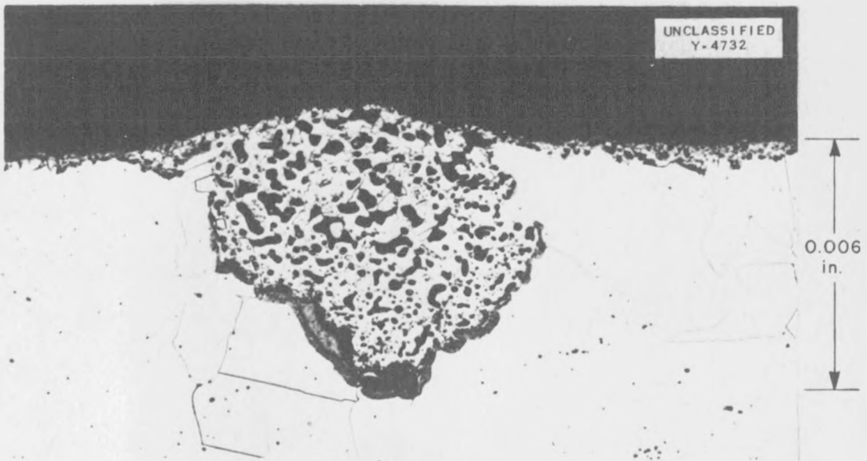
Fig. 11.4. Surface of Nickel Z Specimen after 100 hr of Exposure to Barium Hydroxide at 816°C.
