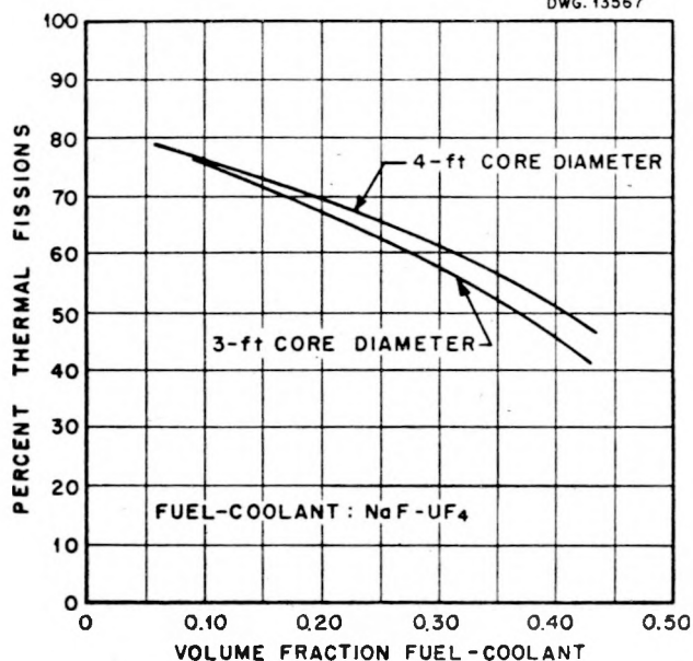
Fig. 3.3. Percent Thermal Fissions as a Function of the Fuel-Coolant Volume Fraction in the 3- and 4-ft-Diameter Cores of the BeO-Moderated Circulating-Fuel Reactor.
