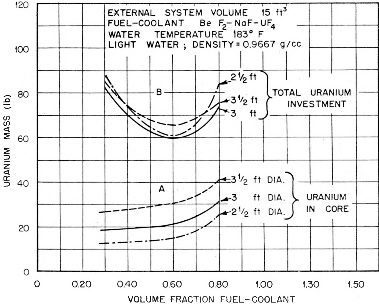
Fig. 3.9. Total Uranium Inventory and Uranium in Core as a Function of the Volume Fraction Fuel-Coolant in the Core for the Water-Moderated Circulating-Fuel Reactor with 2½-, 3-, and 3½-ft-Diameter Cores.
