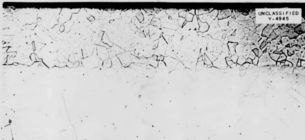
Fig. 11.14. Nickel-Clad Inconel (Nickel Powder) after 100 hr of Exposure to Sodium Hydroxide at 816°C. 100X
