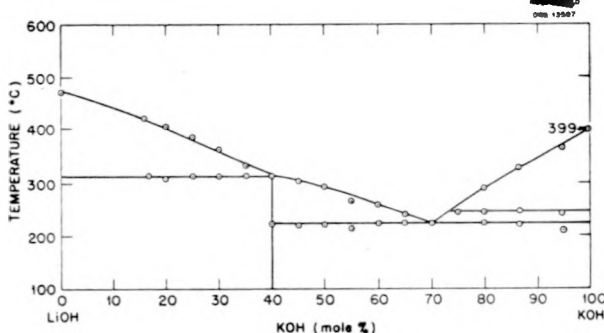
Fig. 10.1. The System KOH-LiOH.
