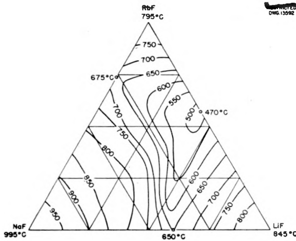
Fig. 10.6. The System NaF-LiF-RbF.
