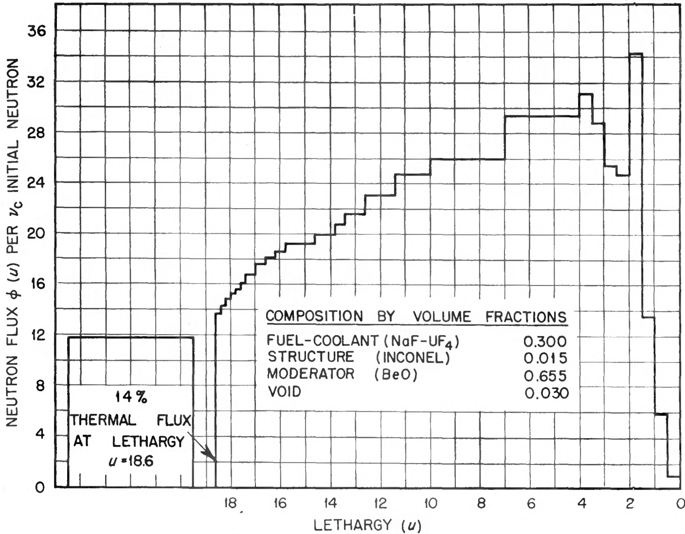
Fig. 3.7. Neutron Flux Spectrum vs. Lethargy for the BeO-Moderated Circulating-Fuel Reactor with a 3½-ft-Diameter Core.
