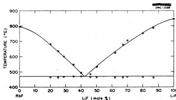
Fig. 10.2. The System RbF-LiF.
