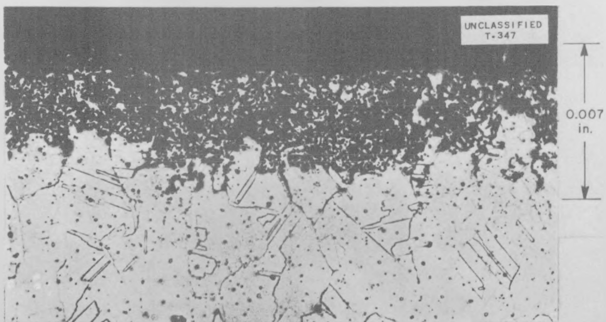
Fig. 11.7. Surface of Inconel Specimen after 100 hr of Exposure to Rubidium Hydroxide at 800°C.
