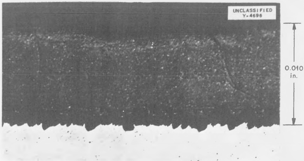
Fig. 11.1. Surface of 304 Stainless Steel after 100 hr of Exposure to Barium Hydroxide at 816°C.
