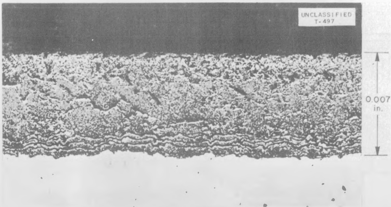
Fig. 11.6. Surface of Inconel Specimen after 100 hr of Exposure to Lithium Hydroxide at 800°C.
