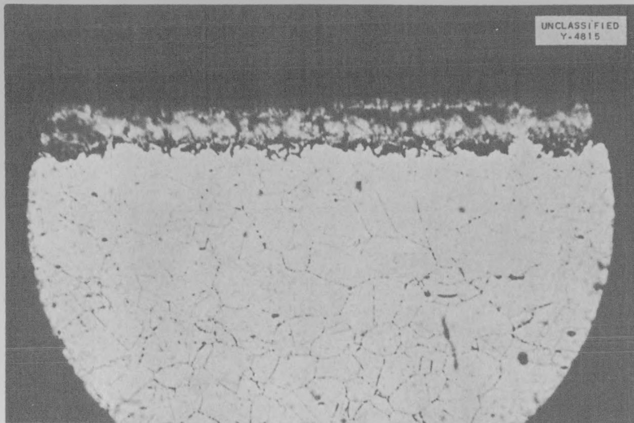
Fig. 11.12. Surface of 304 Stainless Steel Coated with 3-mil Nickel Electroplate after 100 hr of Exposure to Barium Hydroxide at 816°C. Original magnification 500X; reduced to 96%.
