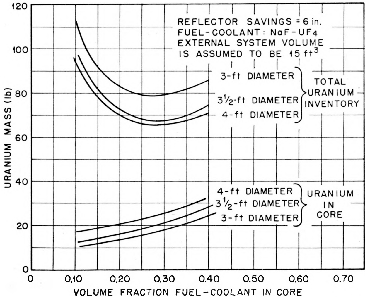
Fig. 3.1. Total Uranium Inventory and Uranium in Core as a Function of the Volume Fraction Fuel Coolant in the Core for BeO-Moderated Circulating-Fuel Reactors with 3-, 3½-, and 4-ft-Diameter Cores.
