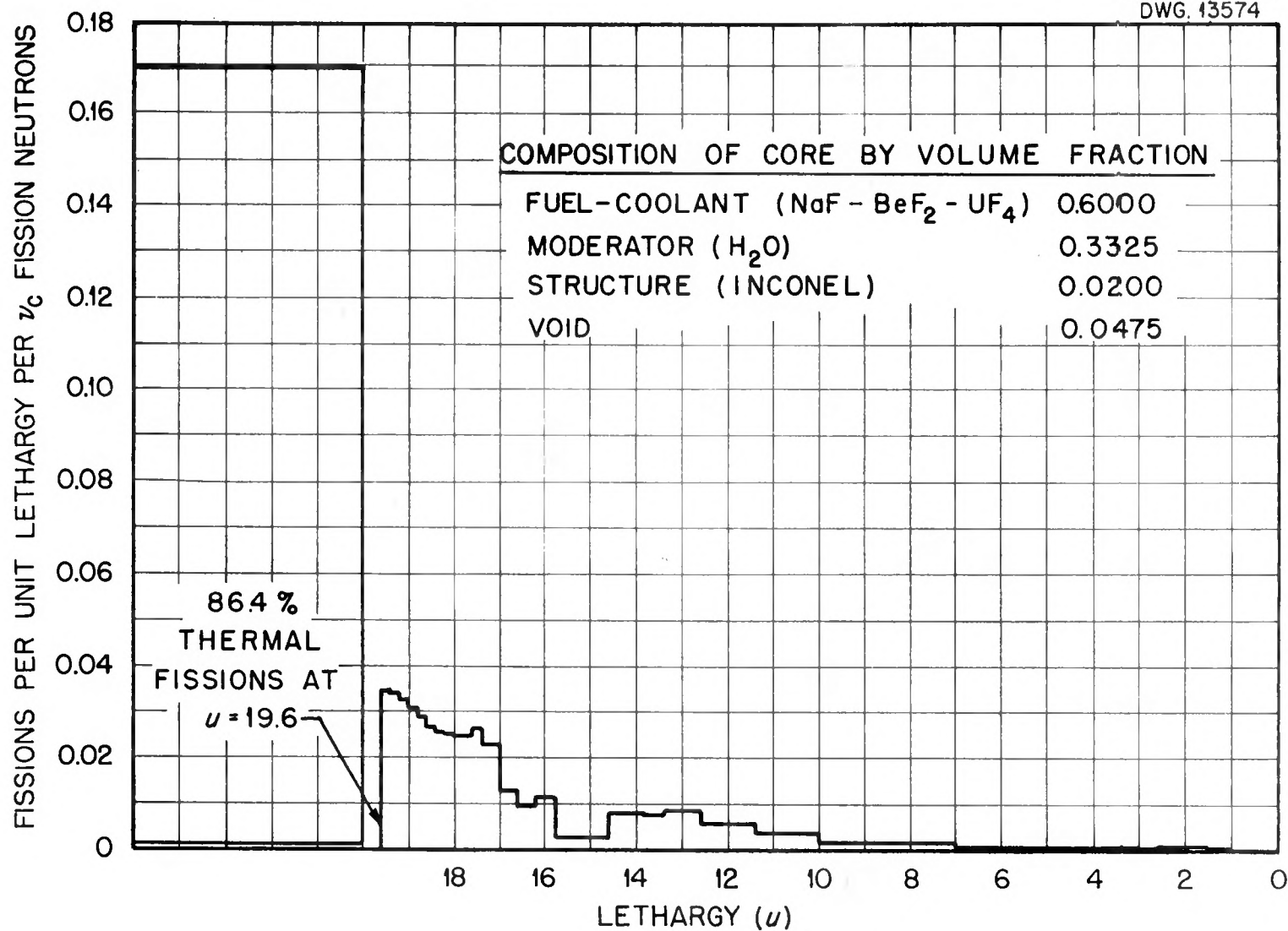
Fig. 3.10. Fission Spectrum vs. Lethargy for the H 2 O-Moderated Circulating-Fuel Reactor with 3-ft-Diameter Core.
