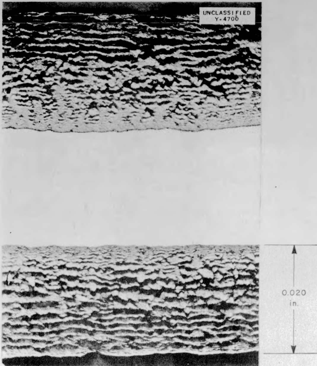
Fig. 11.3. Surface of Inconel Specimen after 100 hr of Exposure to Barium Hydroxide at 816°C.
