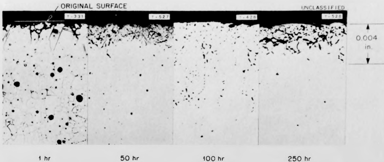
Fig. 11.9. Effect of Exposure Time on the Corrosion of Inconel by Potassium Hydroxide at 800°C.
