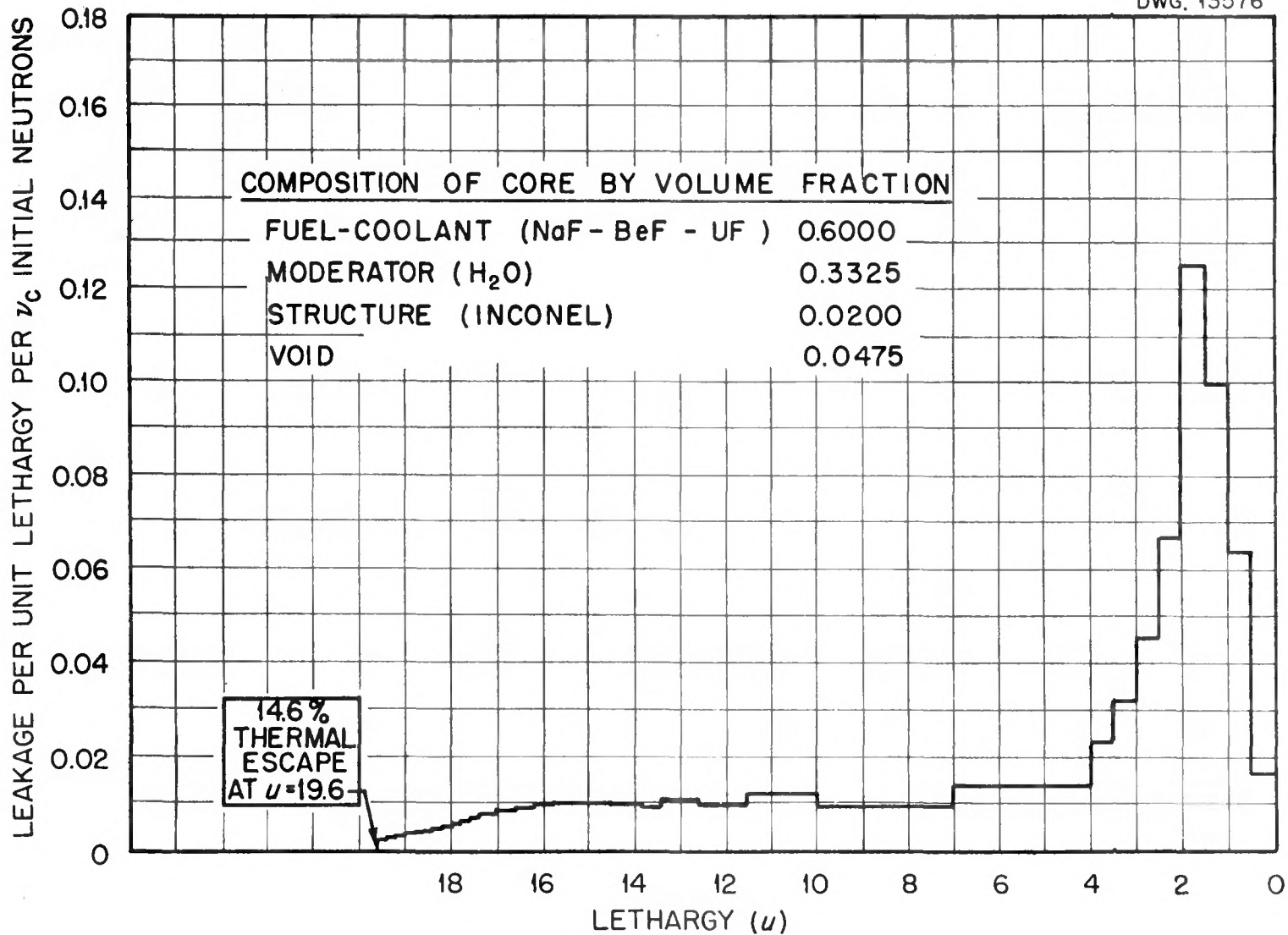
Fig. 3.12. Leakage Spectrum vs. Lethargy for the H 2 O-Moderated Circulating-Fuel Reactor with 3-ft-Diameter Core.
