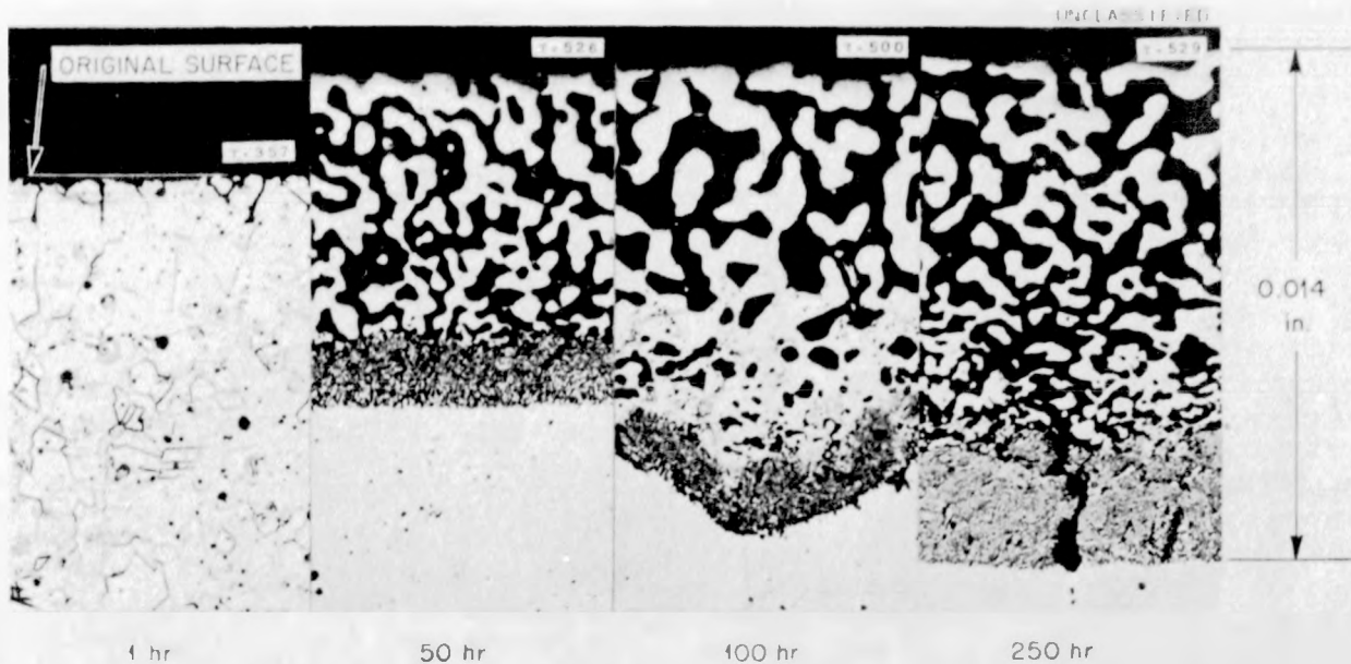
Fig. 11.8. Effect of Exposure Time on the Corrosion of Inconel by Sodium Hydroxide at 800°C.
