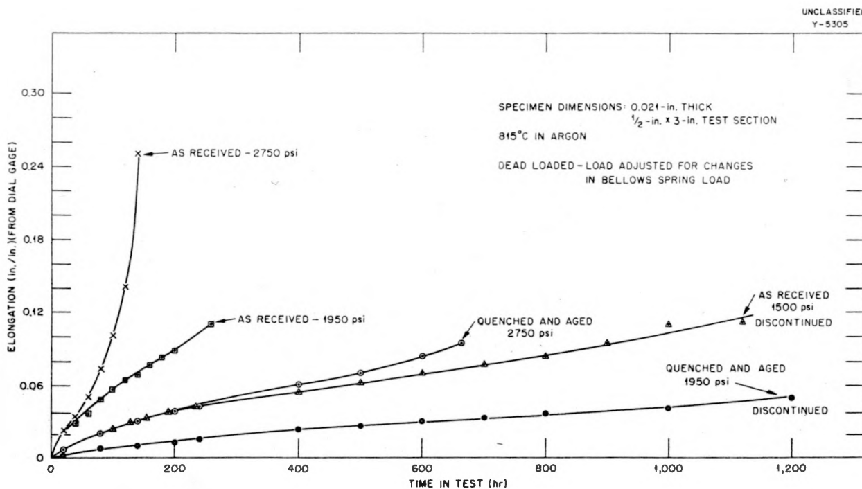
Fig. 13.11. Time-Elongation Curve for Nickel Z.
