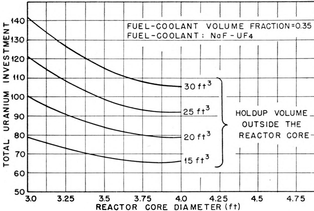
Fig. 3.2. Total Uranium Investment in BeO-Moderated Circulating-Fuel Reactor as a Function of Reactor Core Diameter for Several Assumed Holdup Volumes External to Core.
