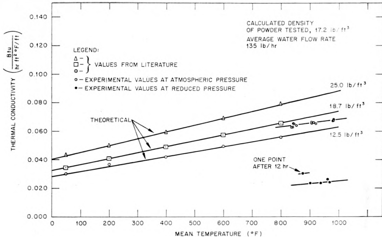
Fig. 12.3. Thermal Conductivity of Diatomaceous Earth.
