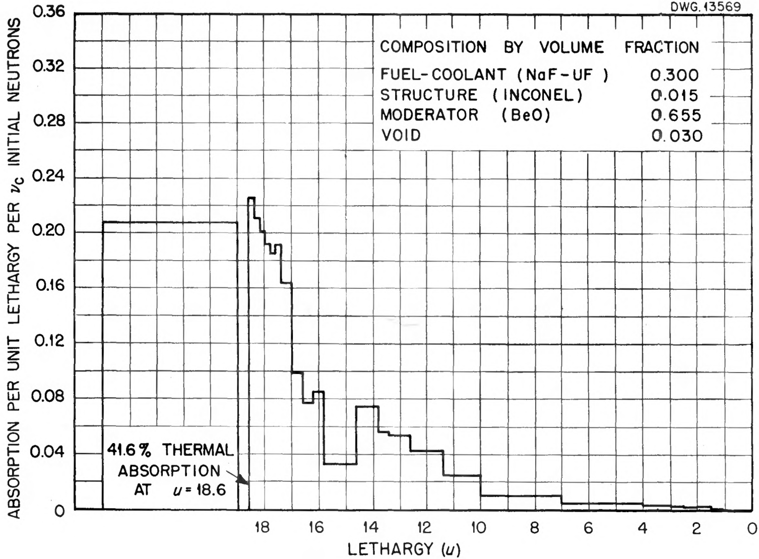
Fig. 3.5. Absorption Spectrum vs. Lethargy for the BeO-Moderated Circulating-Fuel Reactor with a 3½-ft-Diameter Core.
