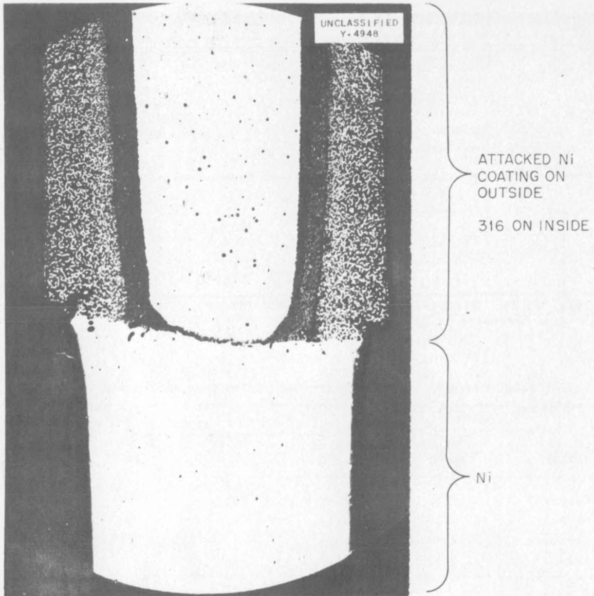
Fig. 11.13. Nickel-Clad Inconel (Nickel Sheet) after 100 hr of Exposure to Sodium Hydroxide at 816°C. 50X
