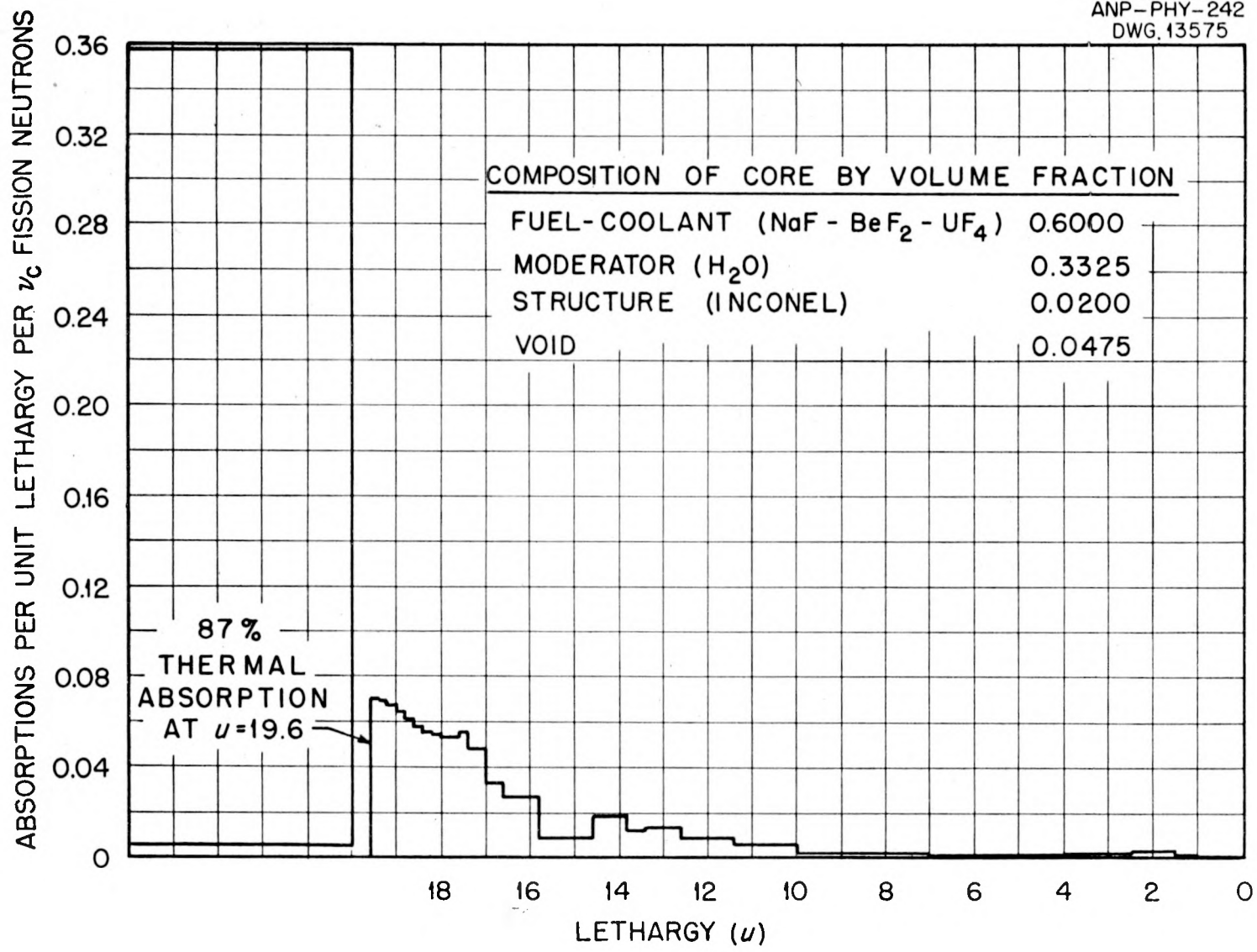
Fig. 3.11. Absorption Spectrum vs. Lethargy for the H 2 O-Moderated Circulating-Fuel Reactor with 3-ft-Diameter Core.
