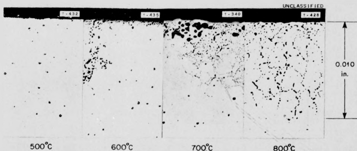
Fig. 11.10. Effect of Temperature on the Corrosion of Inconel by Potassium Hydroxide in 100 hr.
