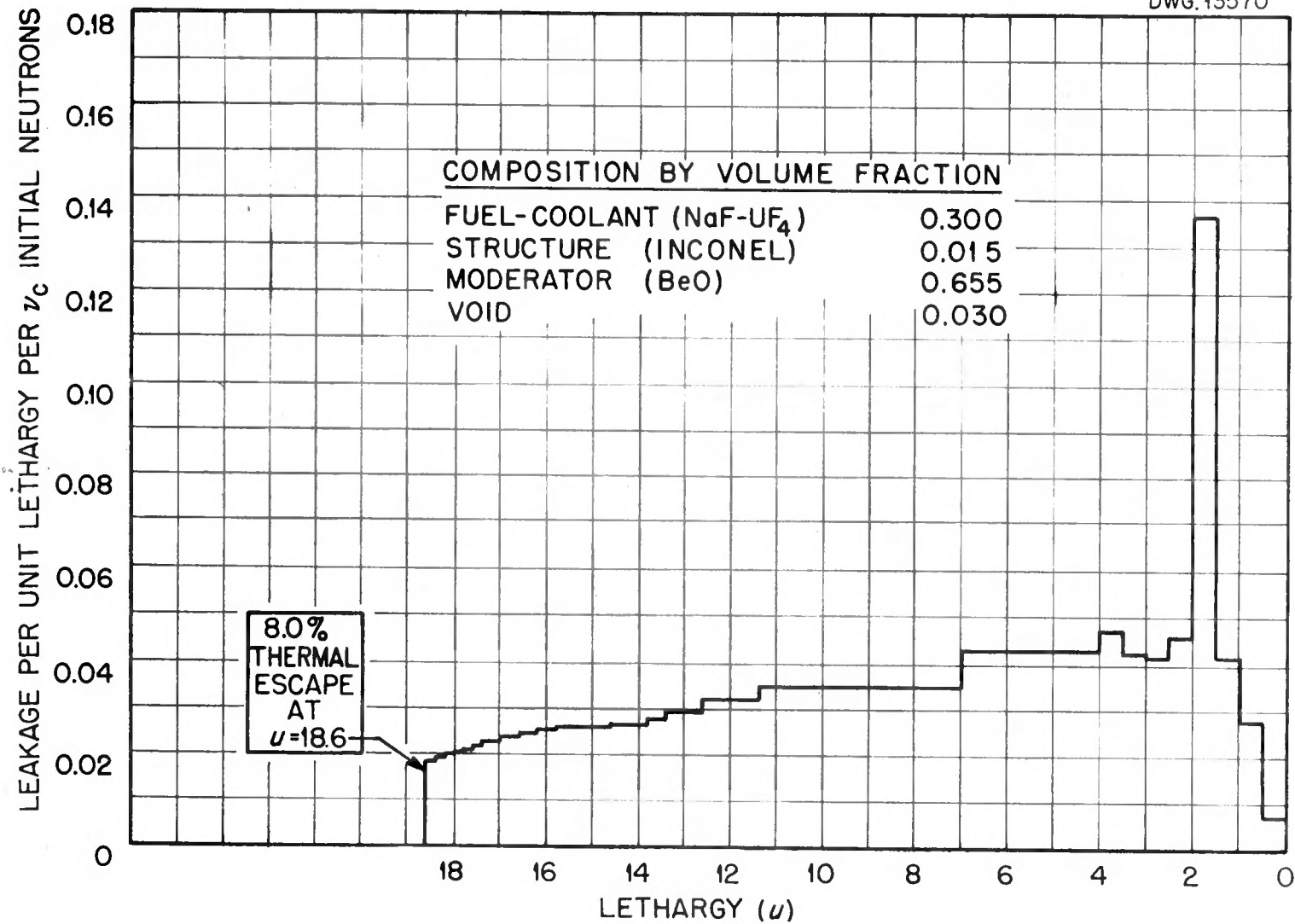
Fig. 3.6. Leakage Spectrum vs. Lethargy for the BeO-Moderated Circulating-Fuel Reactor with a 3½-ft-Diameter Core.
