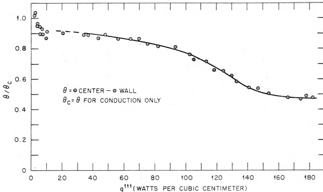
Fig. 12.1. Temperature Ratio in a 3-mm Tube Filled with Brine in which Heat is Generated Uniformly.
