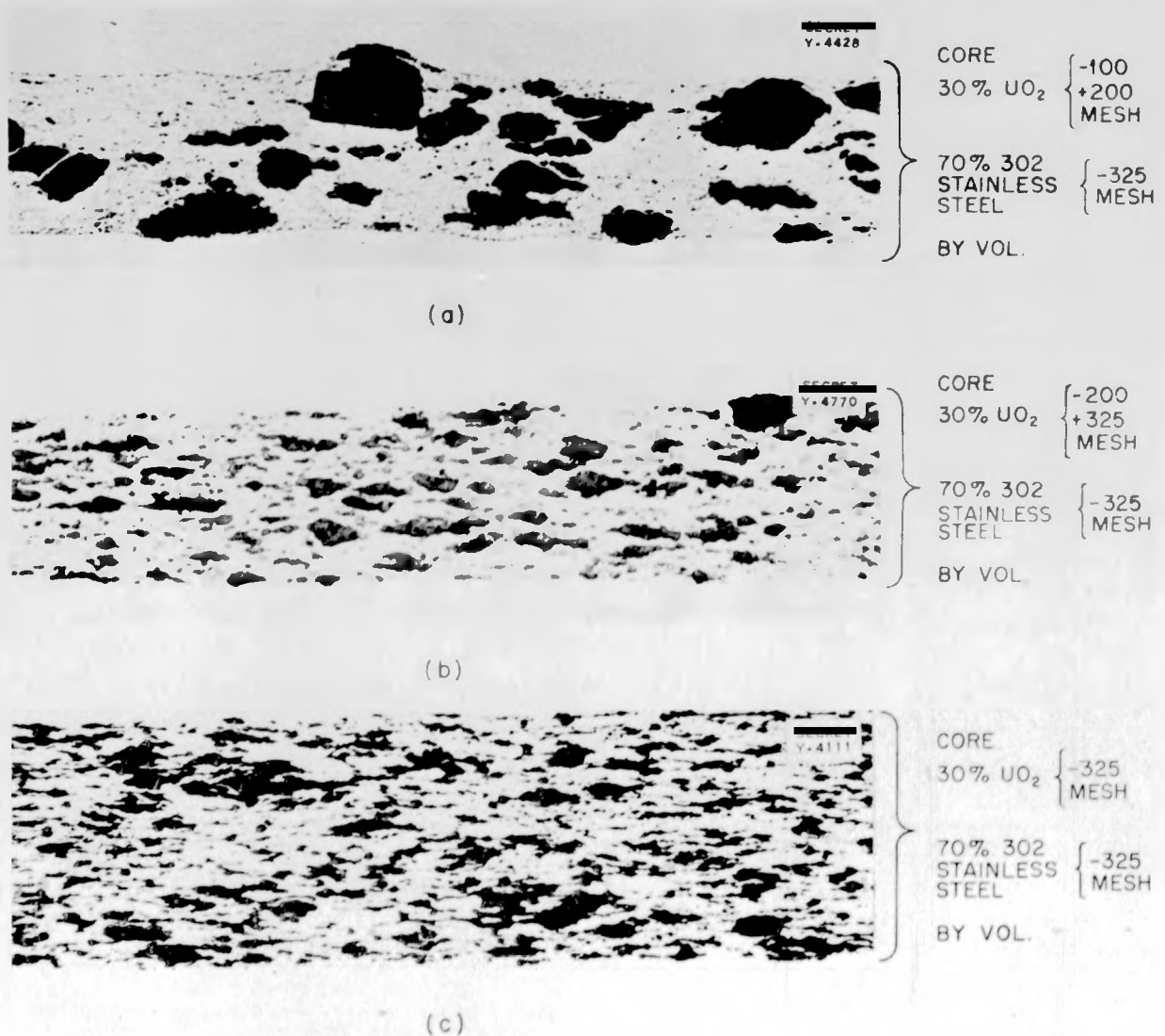
Fig. 13.1 a, b, c. Effect of UO_2 Particle Size on UO_2 Distribution. 175X.
