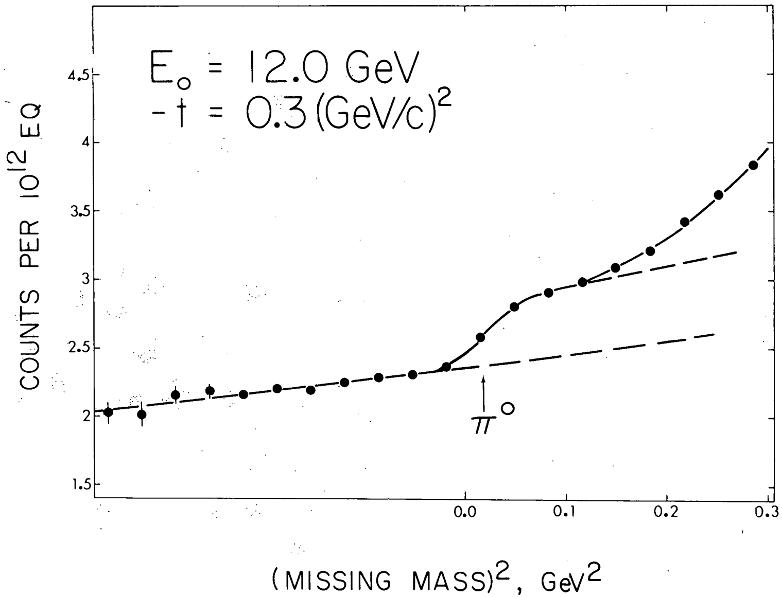
FIG. 13b--Sample \pi^0 fits.
