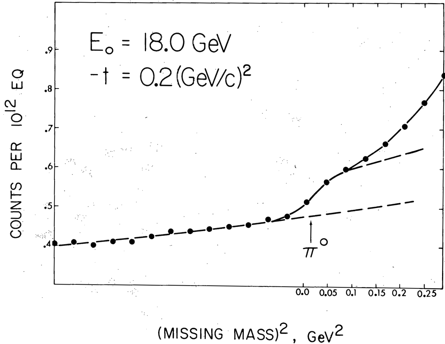
FIG. 13h--Sample \pi^0 fits.
