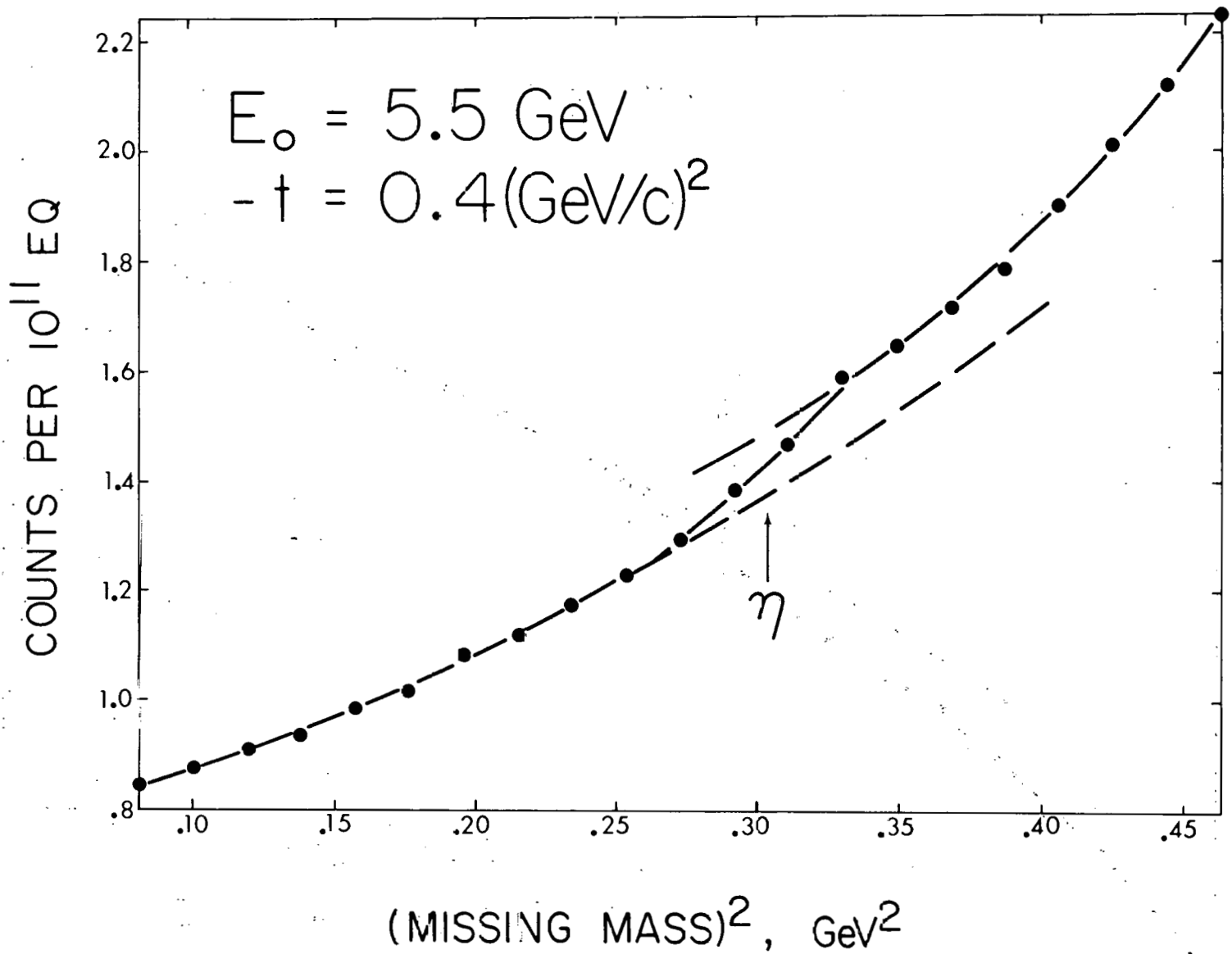
FIG. 14b--Sample \eta fits.
