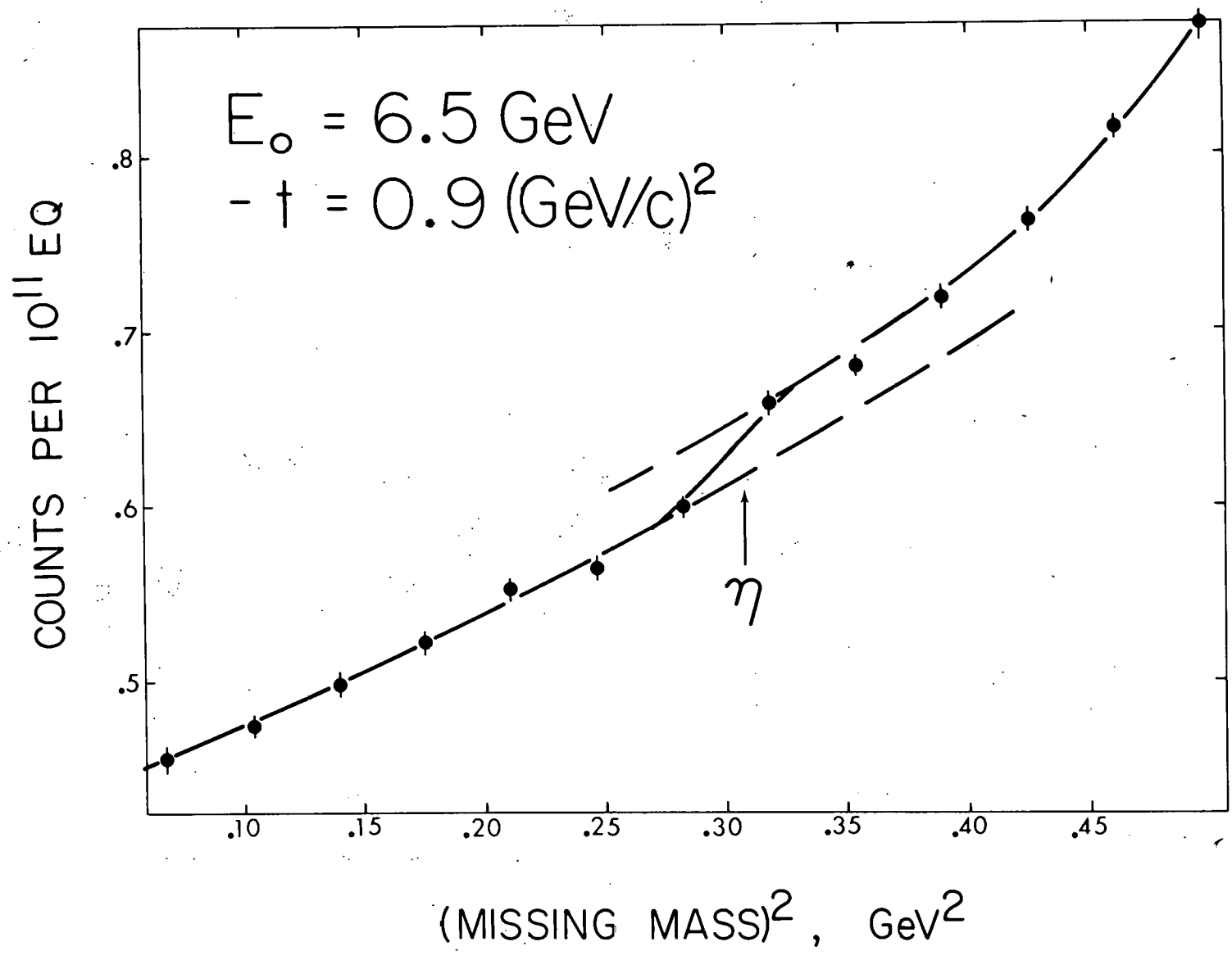
FIG. 14e--Sample \eta fits.
