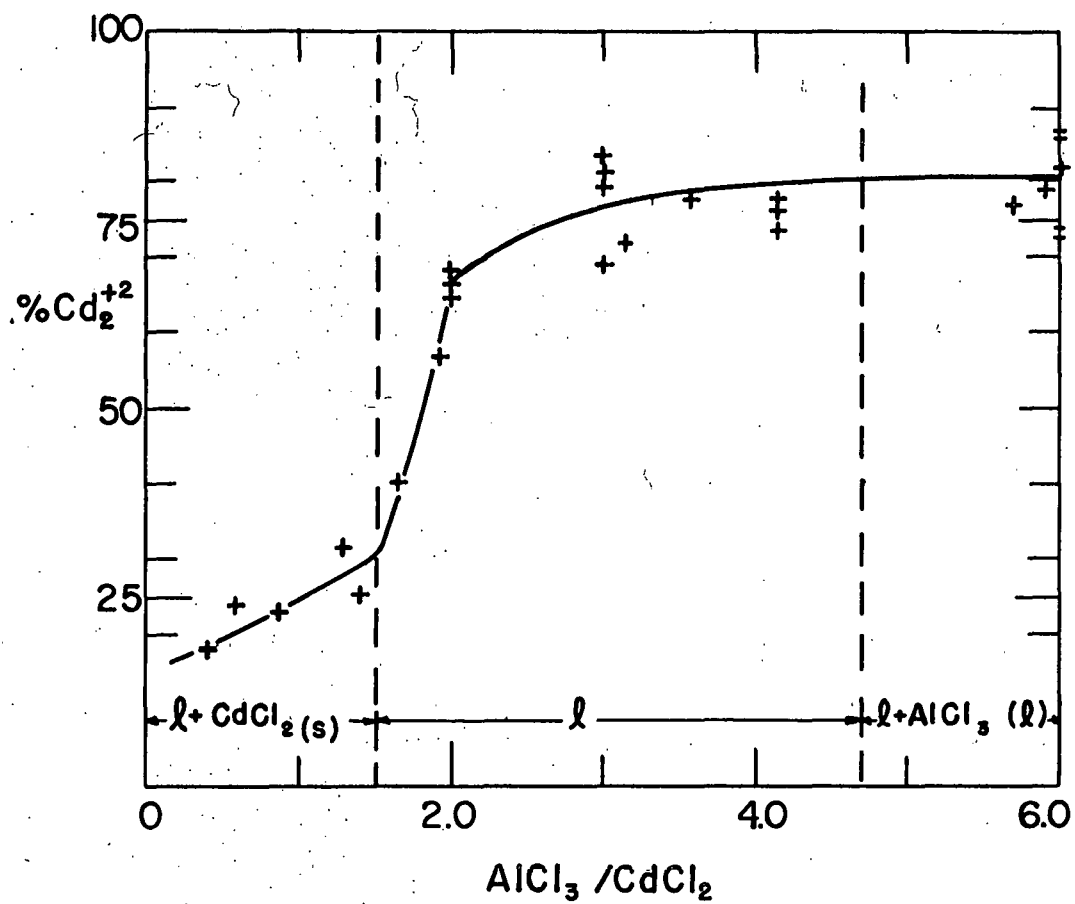
Fig. 2. The percent reduction of \text{Cd}^{+2} to \text{Cd}_2^{+2} at 335^\circ as a function of the ratio of \text{AlCl}_3 to \text{CdCl}_2 in the initial salt.
