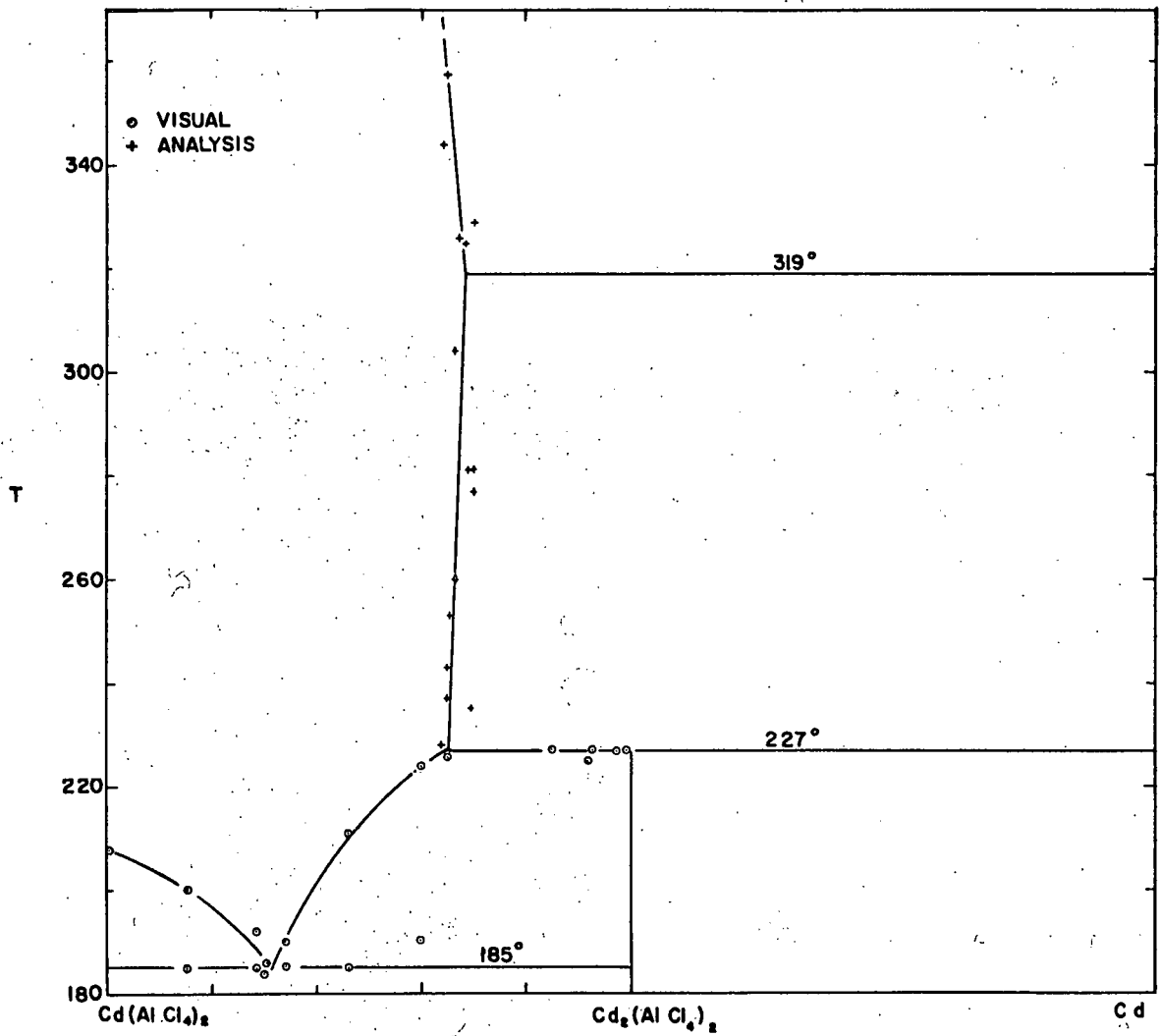
Fig. 1. The system \text{Cd}(\text{AlCl}_4)_2 - \text{Cd}_2(\text{AlCl}_4)_2 - \text{Cd} .
