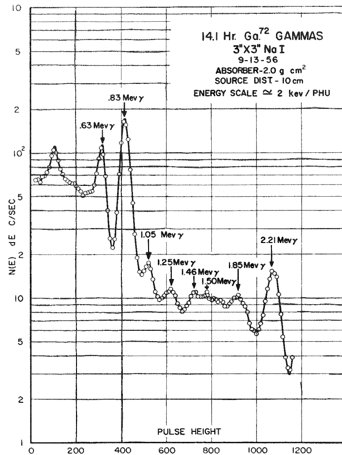
Fig.16. Gamma-ray spectrum of Ga^{72}
