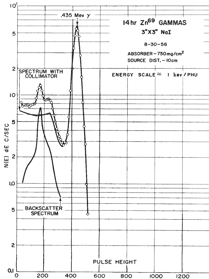
Fig.15. Gamma-ray spectrum of Zn^{69}
