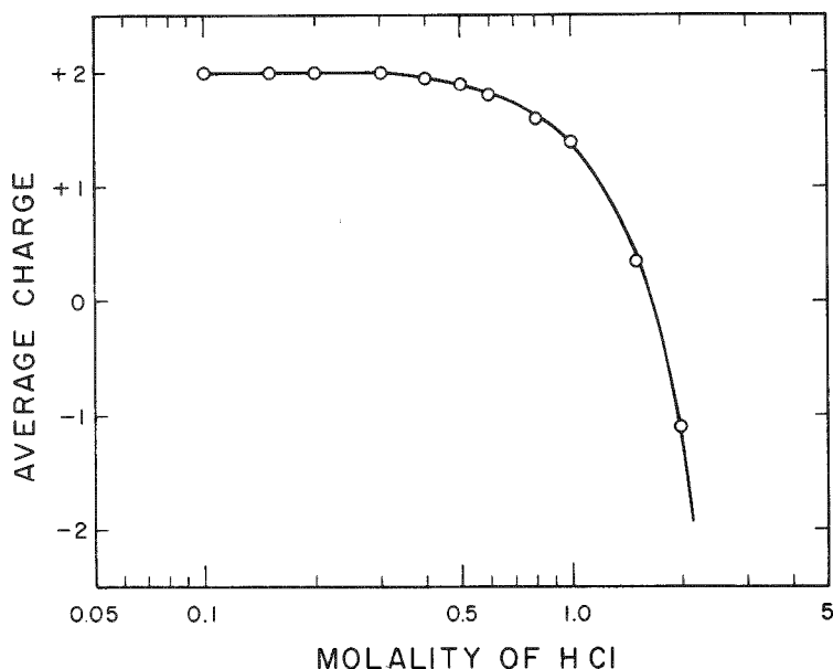
Fig. 4. Average charge of \text{Zn}(\text{II}) in \text{HCl} (anion exchange slope method).
