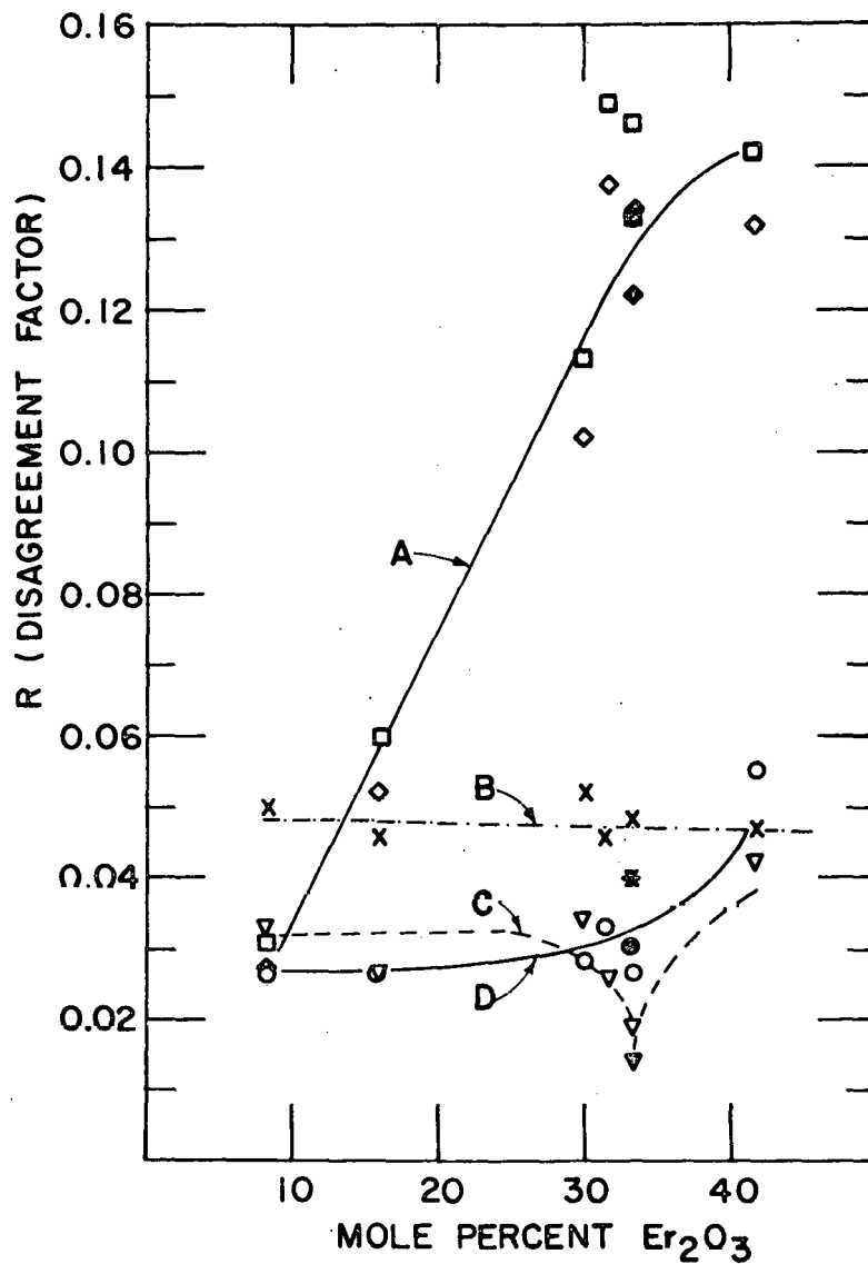
Figure 15. Crystallographic R factors for various structural models
