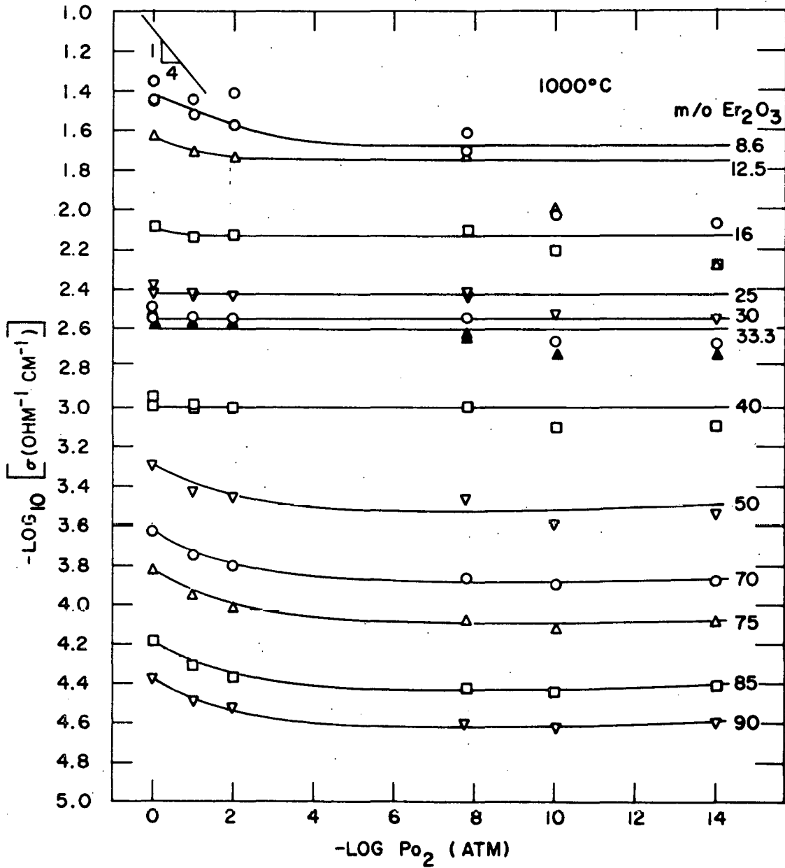
Figure 22. Total conductivity as a function of oxygen partial pressure for fluorite and erbia solid solutions
