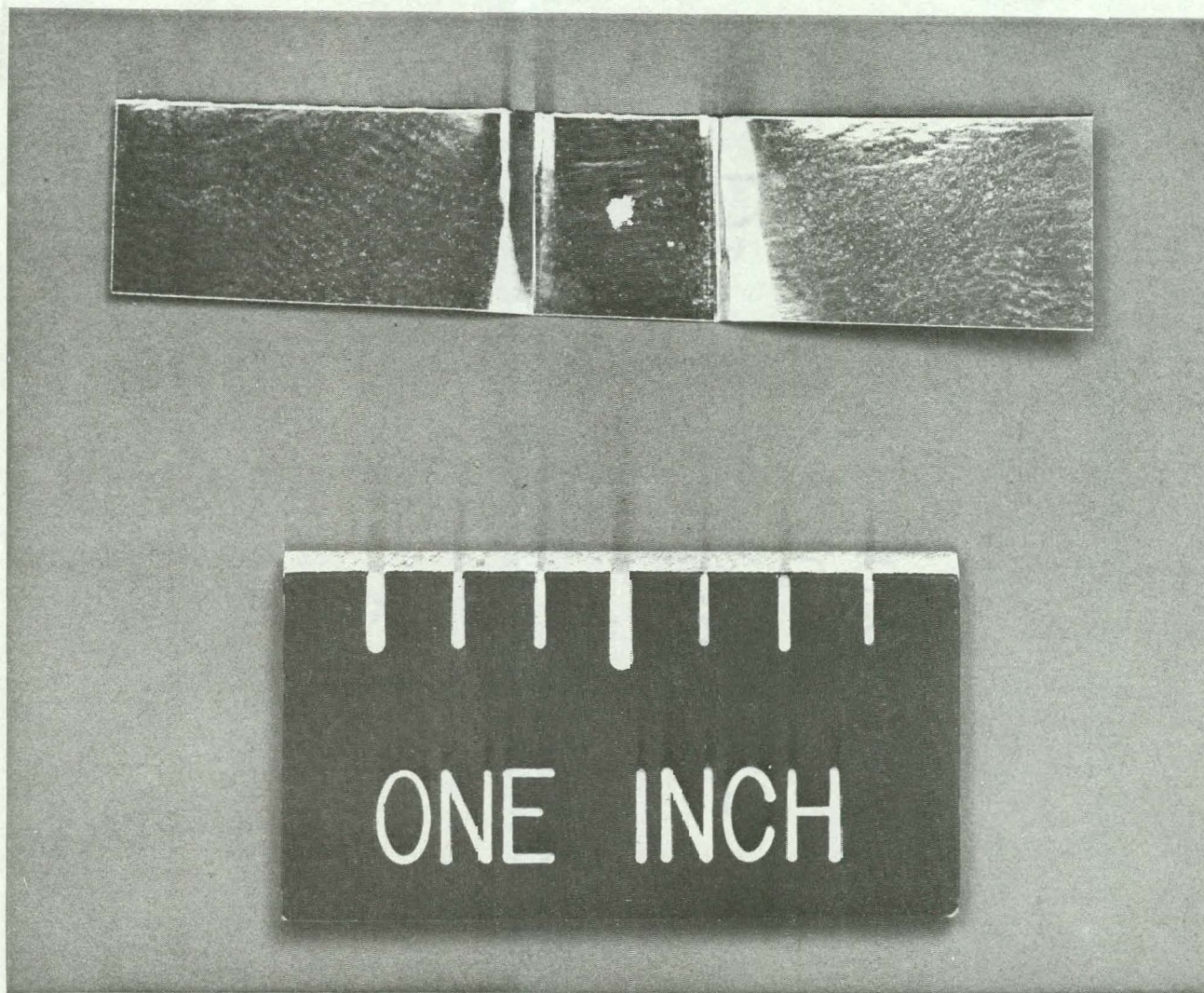
Figure 7. Photograph of a tungsten ribbon used in the melting point furnace. Note the sample in the depression
