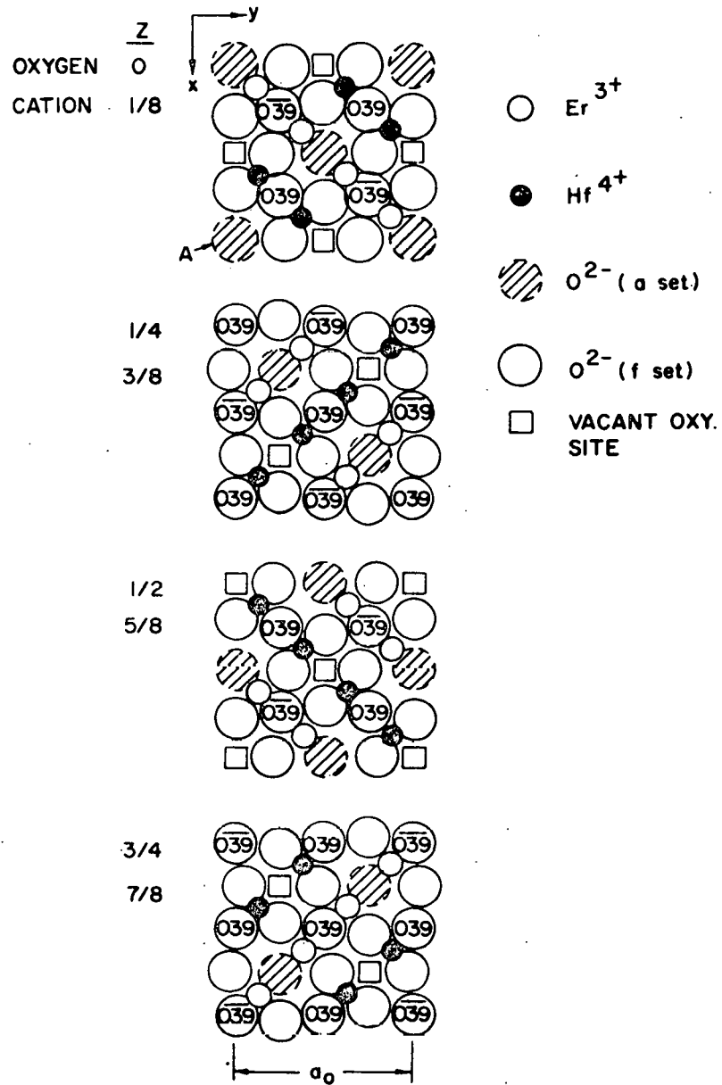
Figure 16. Pyrochlore structure for x(f) = 0.289
