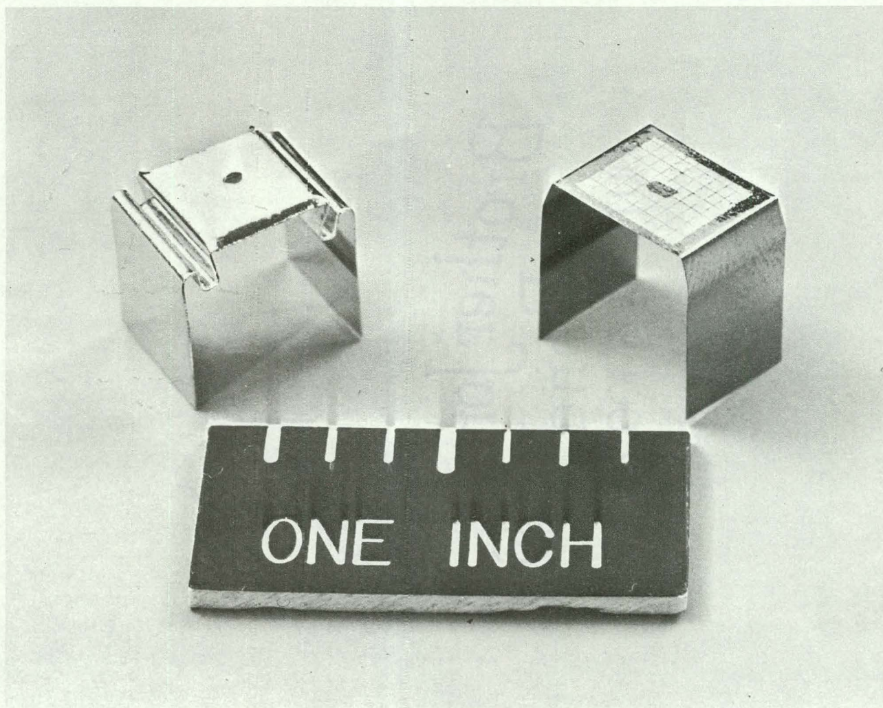
Figure 5. Photograph of the heater/sample configurations used in the high temperature X-ray furnace. Left side: Pt-40% ribbon; Right side: Tungsten ribbon
