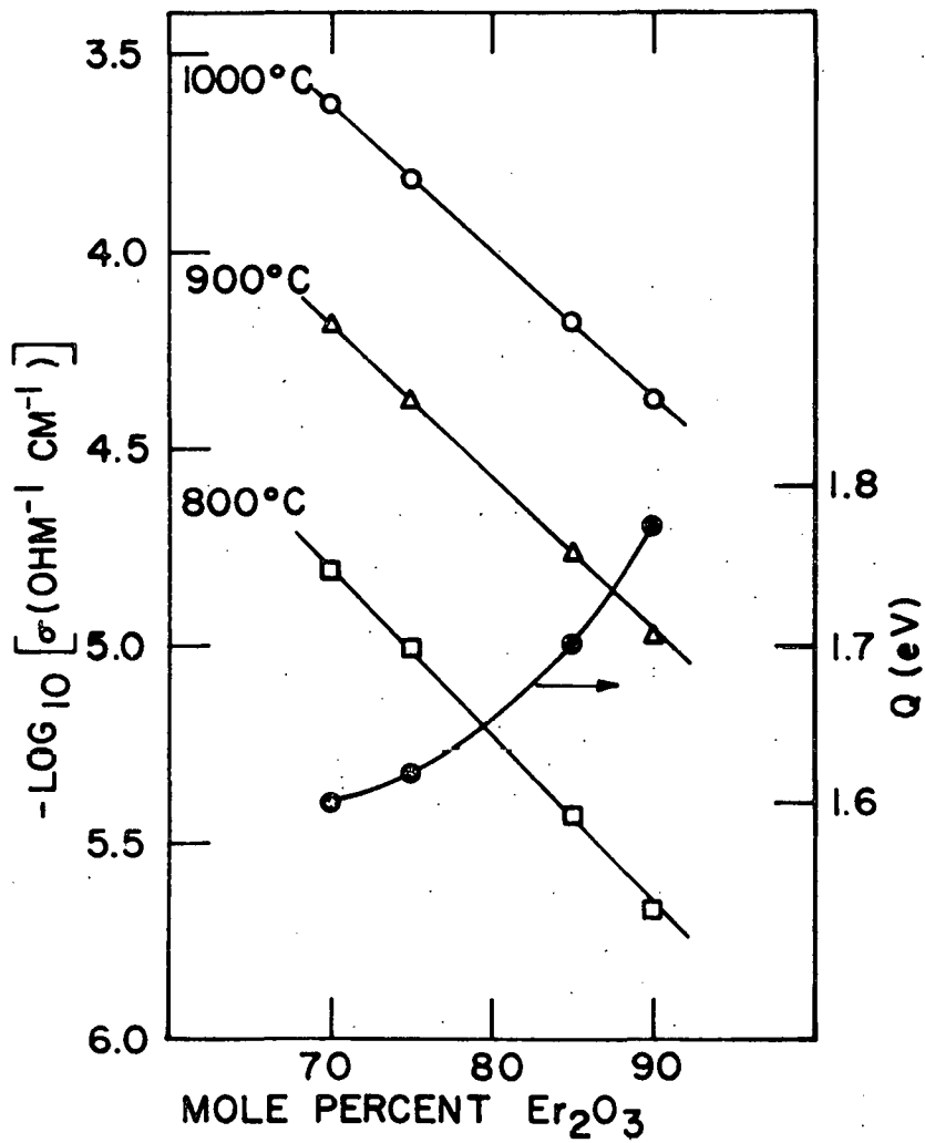
Figure 21. Total conductivity and activation energy for conduction as a function of composition in the erbia solid solution domain
