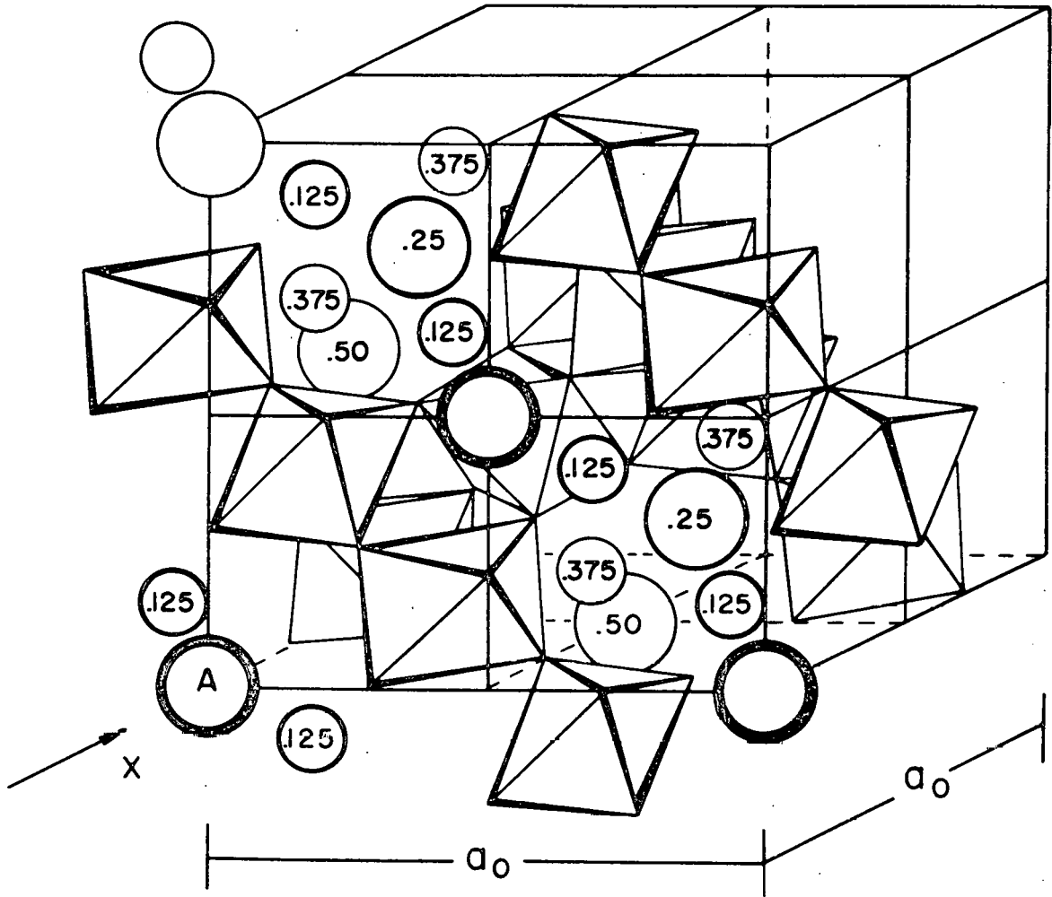
Figure 17. Clinographic projection of the pyrochlore structure in Figure 16, showing the \text{Er}^{3+} cations and the (a) set oxygen ions located in the holes between the framework octahedra. The oxygen ion labeled A in the lower left hand corner is common to both figures
