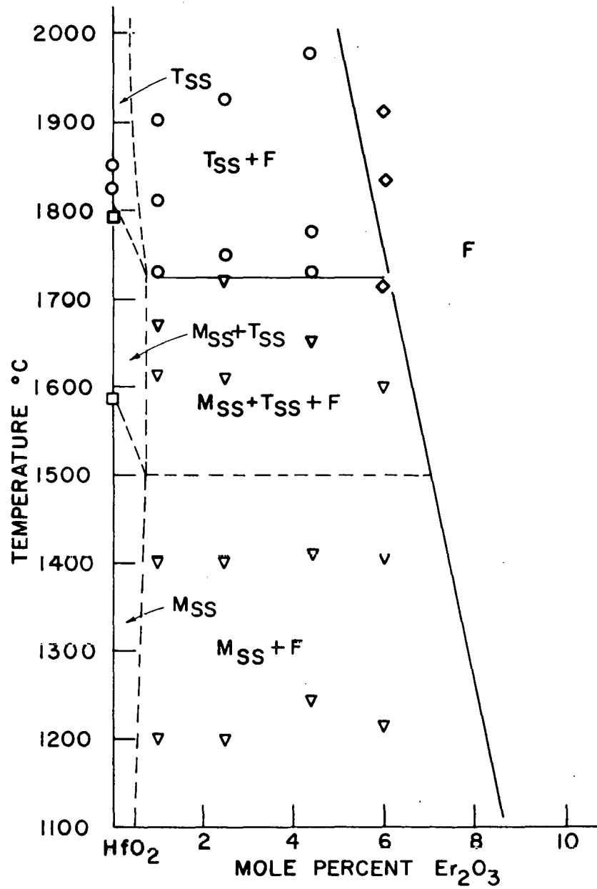
Figure 12. Phase relations in the hafnia-rich region of the hafnia-erbia system
