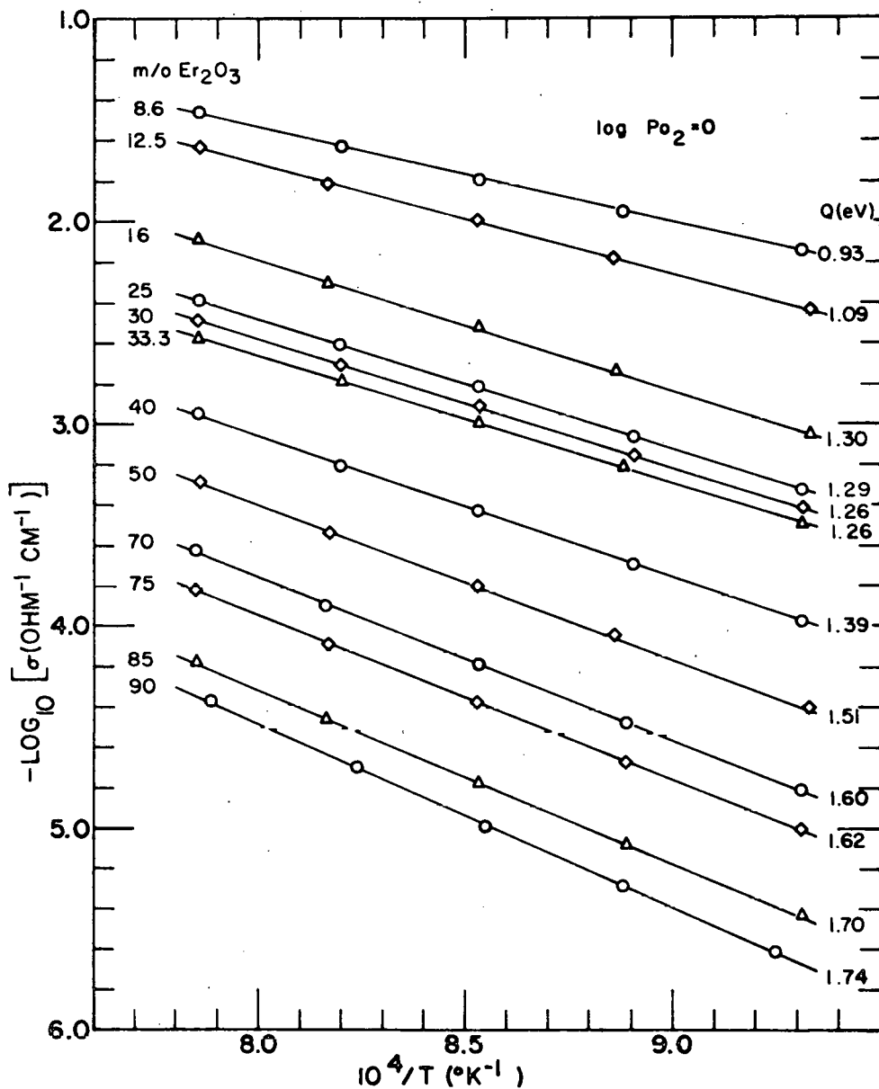
Figure 18. Total conductivity in pure oxygen as a function of temperature for selected compositions in the hafnia-erbia system
