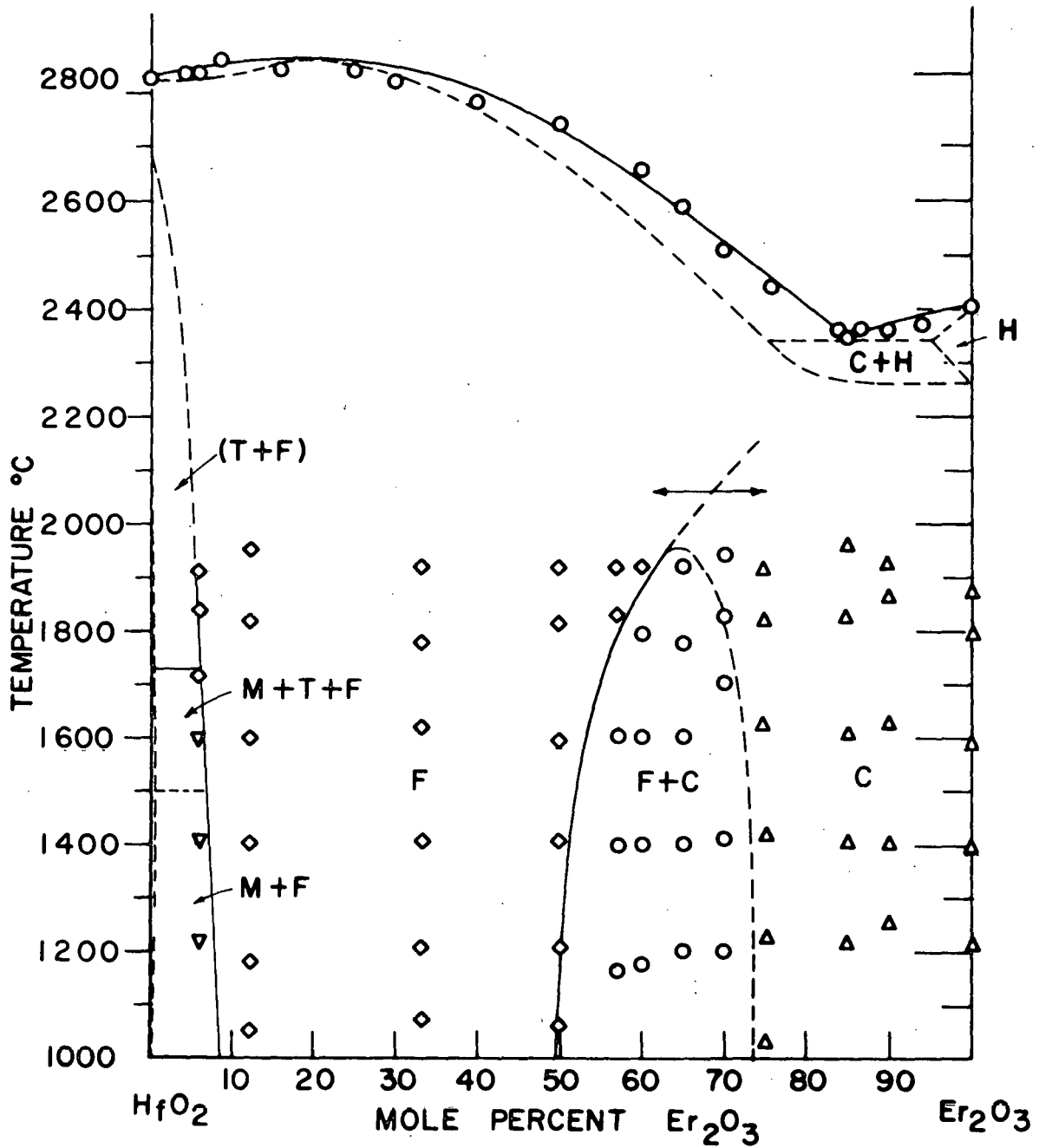
Figure 13. Proposed phase diagram for the hafnia-erbium system
