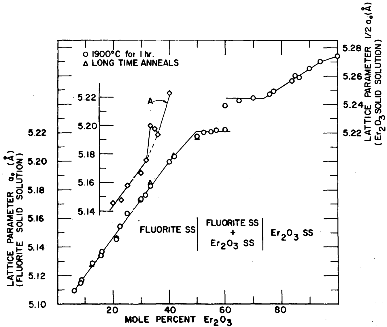
Figure 8. Relation between lattice parameter and composition A. HfO_2 - Y_2O_3 system
