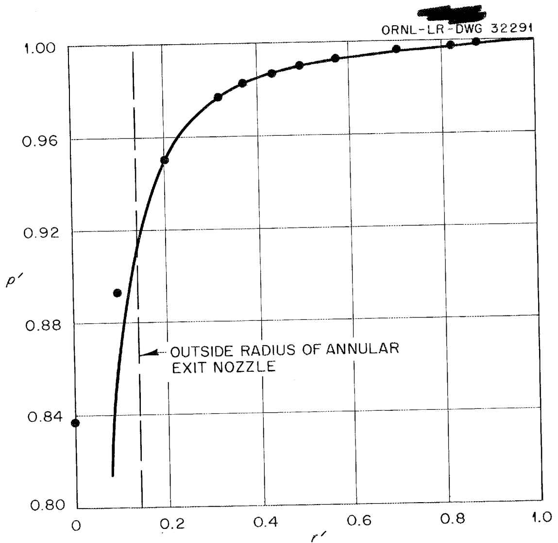
Fig. 7. Typical Correlation of Ratio of Pressure to Wall Pressure with Eq. (6)
