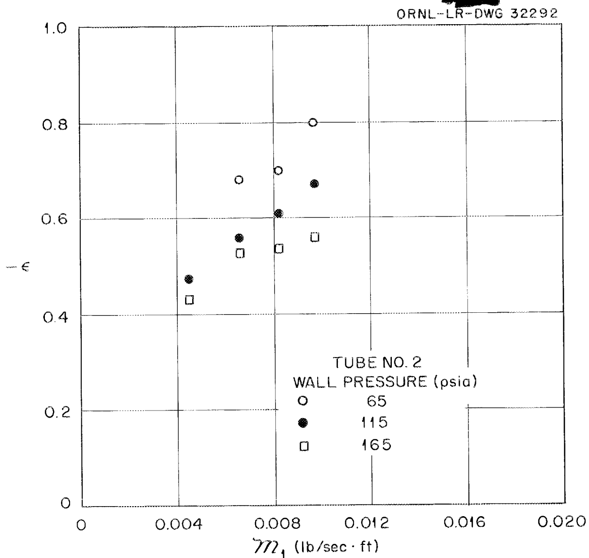
Fig. 8. Variation of \epsilon in \nu \propto r^{+\epsilon} with Mass Flow Rate per Unit of Tube Length, and Tube Pressure, for Tube No. 2.
