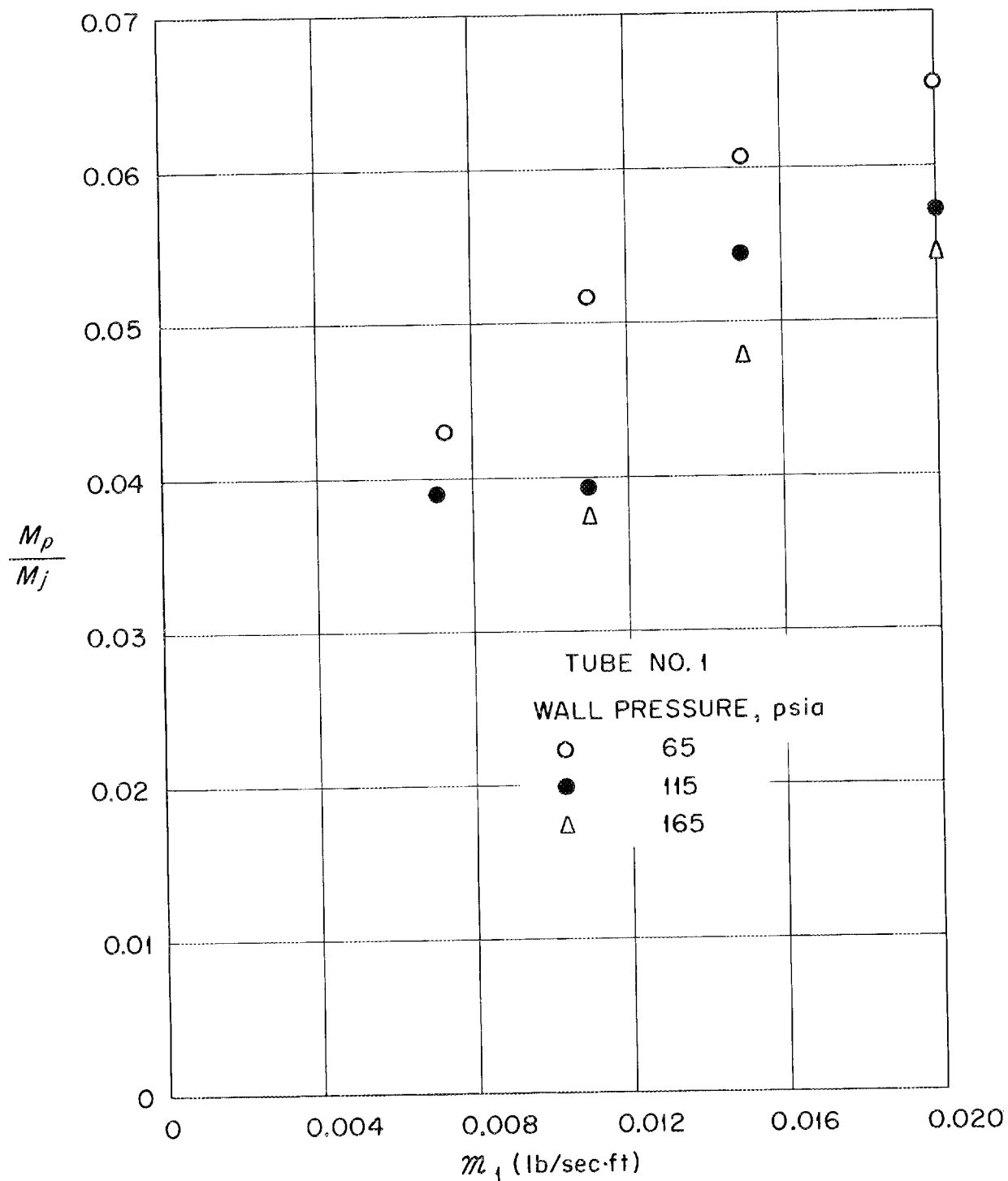
Fig. 11. Variation of Ratio of Vortex Tangential Mach Number and Jet Exit Mach Number With Mass Flow Rate per Unit of Tube Length, and Tube Pressure, for Tube No. 1.
