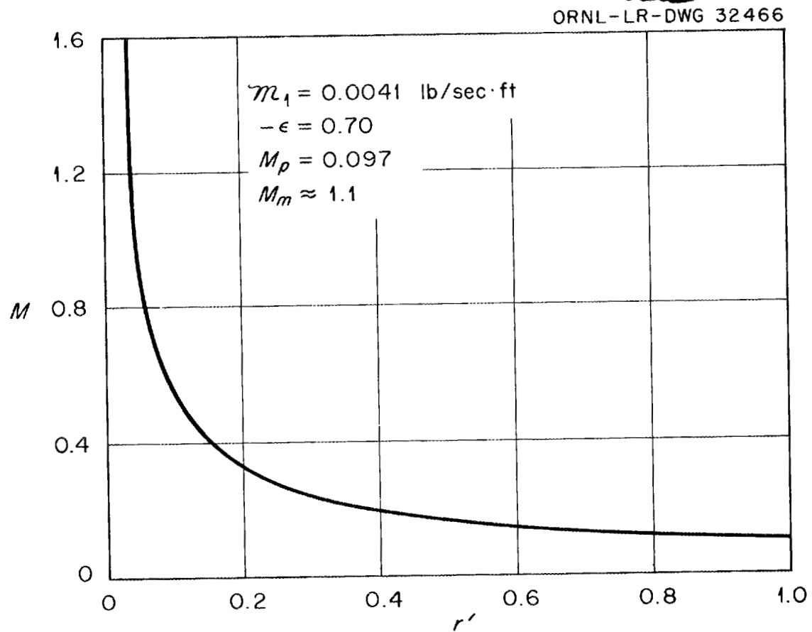
Fig. 23. Mach Number Profile Corresponding to Fig. 21.
