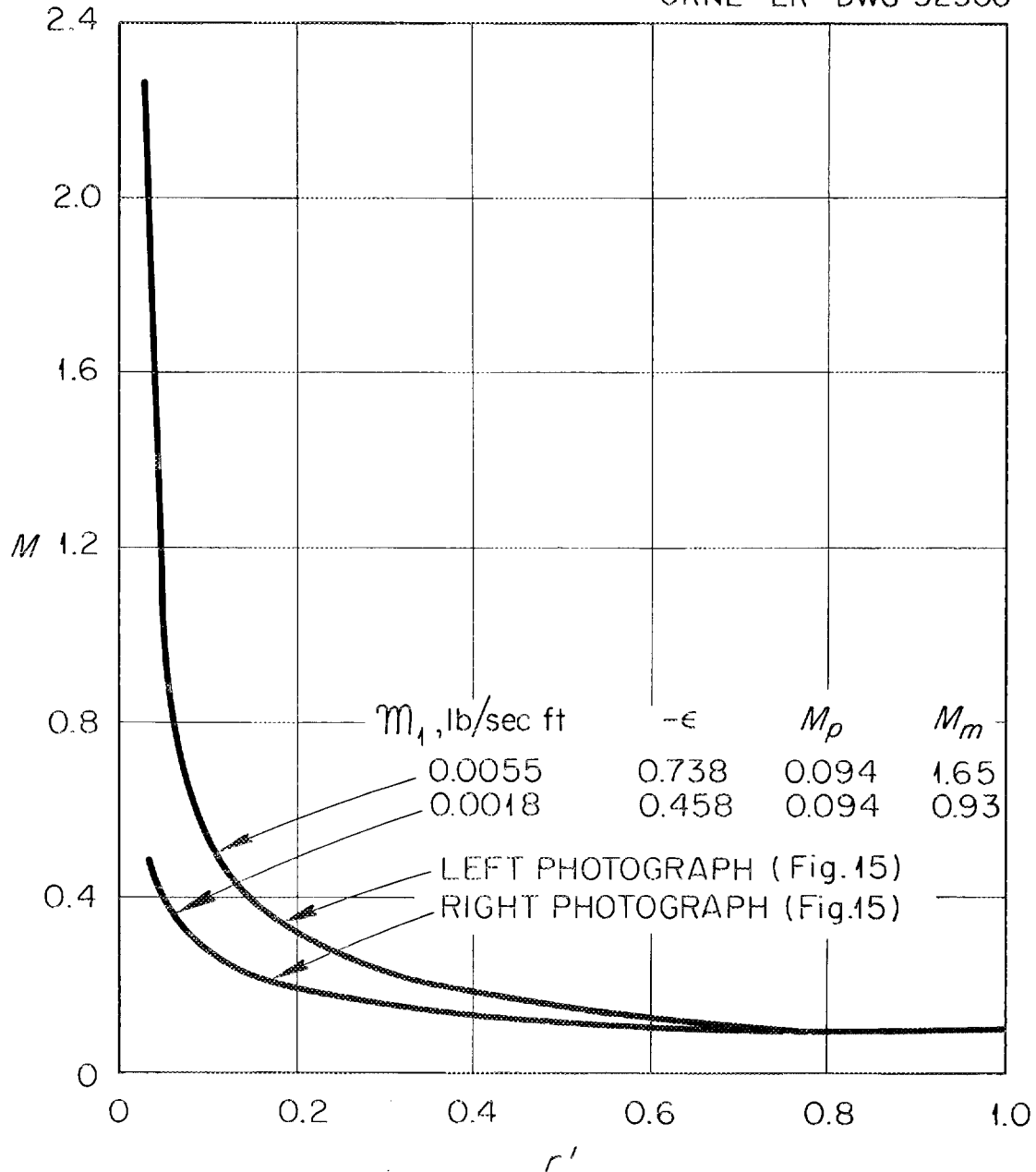
Fig. 17. Mach Number Distributions Corresponding to the Photographs of Fig. 15, with Values of Mach Number Required for Separation, M_m .
