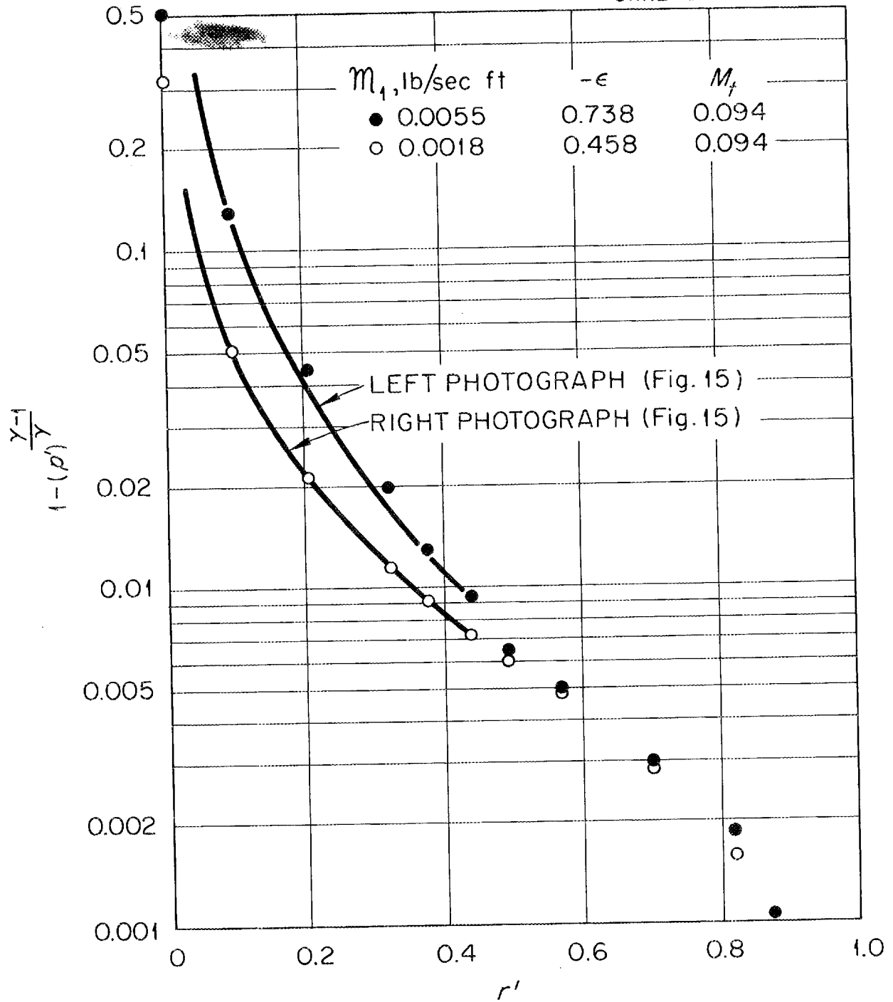
Fig. 16. Pressure Distributions Corresponding to the Photographs of Fig. 15.
