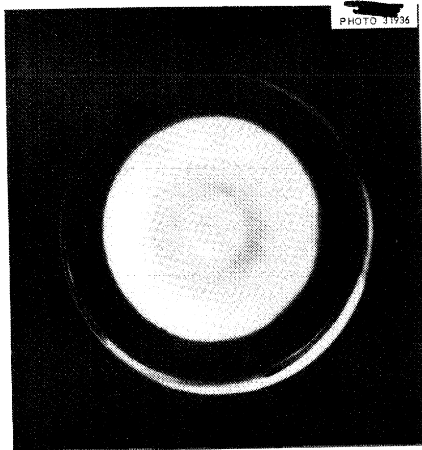
Fig. 15. Photographs Taken Axially Through Vortex Tube Operating With He and \text{Br}_2 , Showing at The Left a Large Ring of Condensed \text{Br}_2 , and at The Right Only The Condensed \text{Br}_2 .
