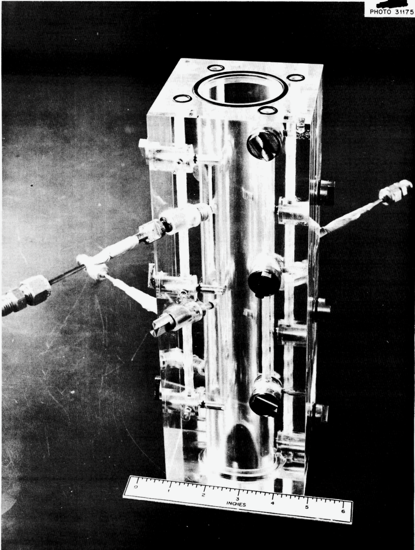
Fig. 3. Plastic Test Block - Vortex Tube No.1.
