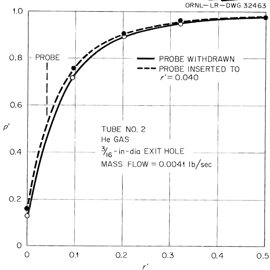
Fig. 19. Effect of Sampling Probe on Pressure Distribution.
