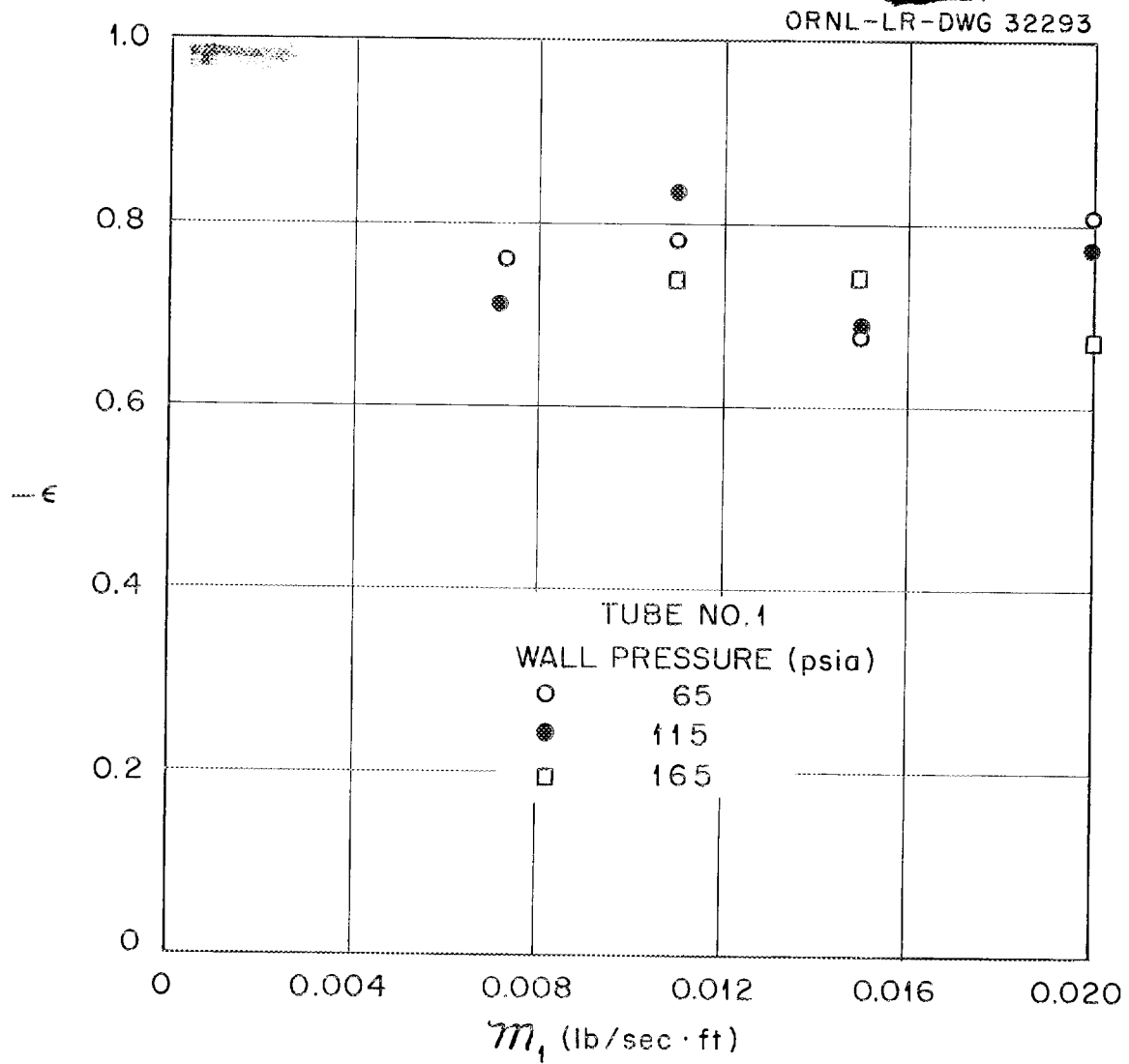
Fig. 9. Variation of \epsilon in \nu \propto r^{+\epsilon} with Mass Flow Rate per Unit of Tube Length, and Tube Pressure, for Tube No. 1.
