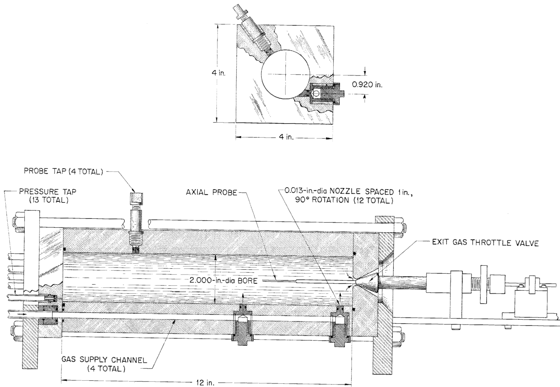
Fig. 2. Sketch of Experimental Vortex Tube.
