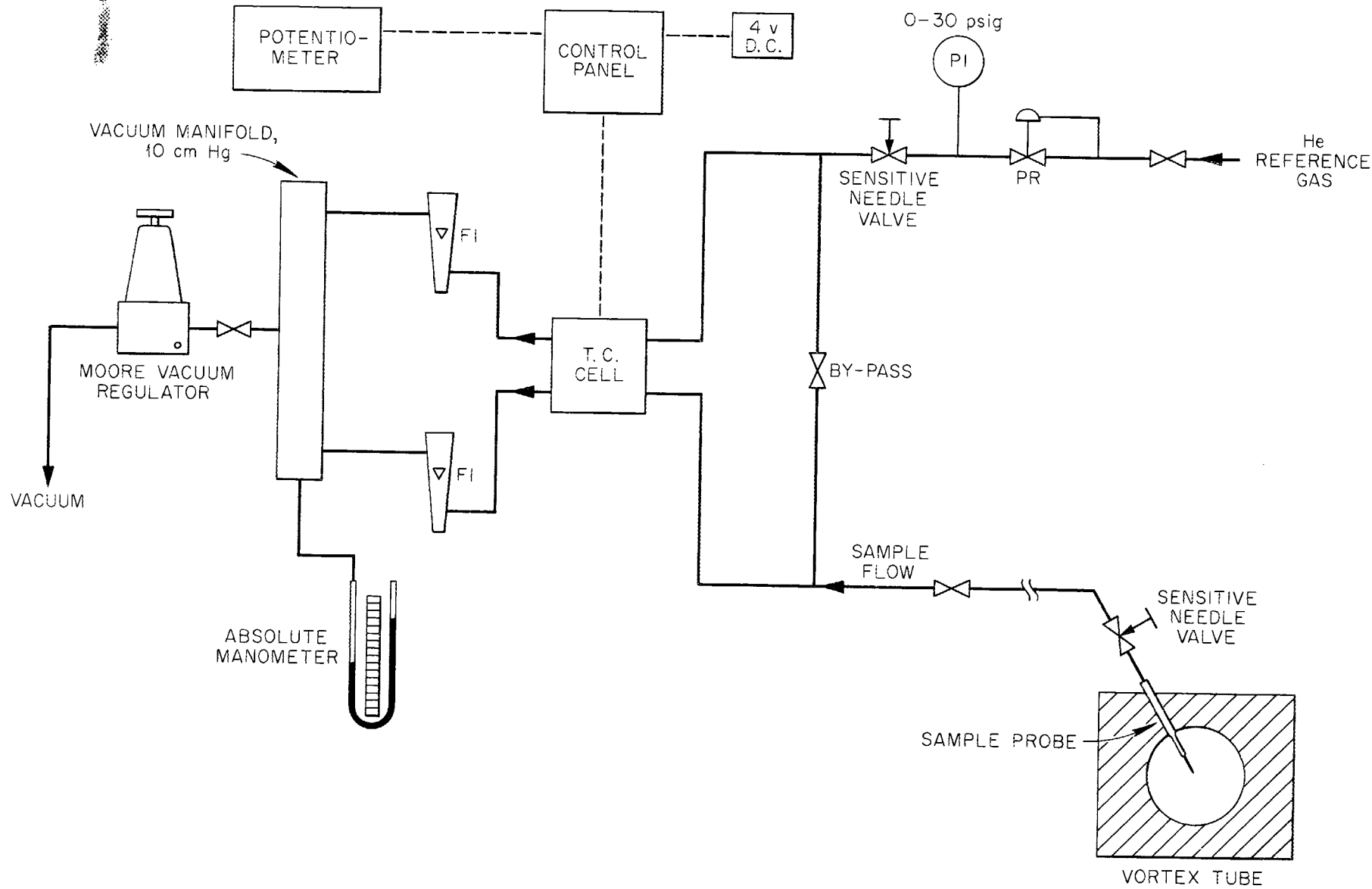
Fig. 20. Gas Analysis Apparatus.
