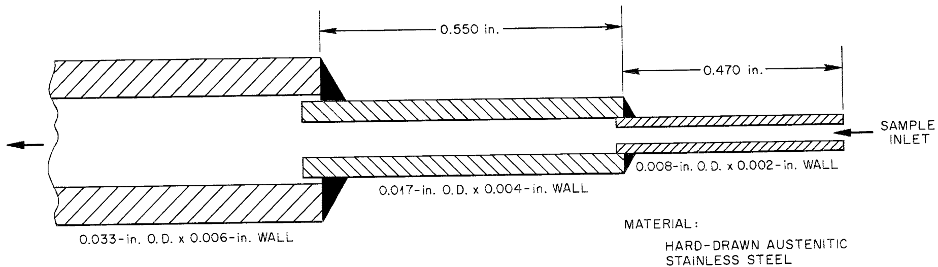
Fig. 18. Sample Probe Detail.
