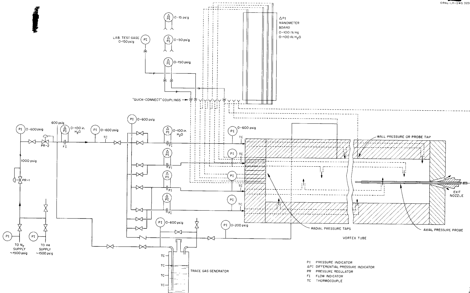
Fig. 5. Over-all Flow and Instrumentation Diagram.
