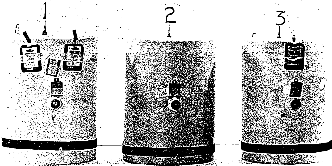
Fig. 1. Typical Placement of Dosimeters on Phantom Section
