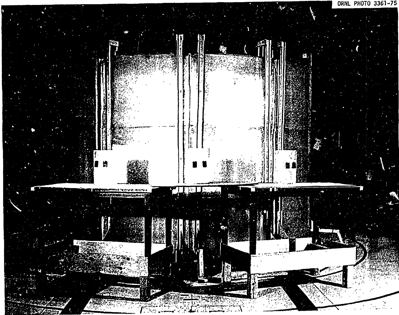
Fig. 2. Typical Experimental Arrangement for Reactor Exposures
