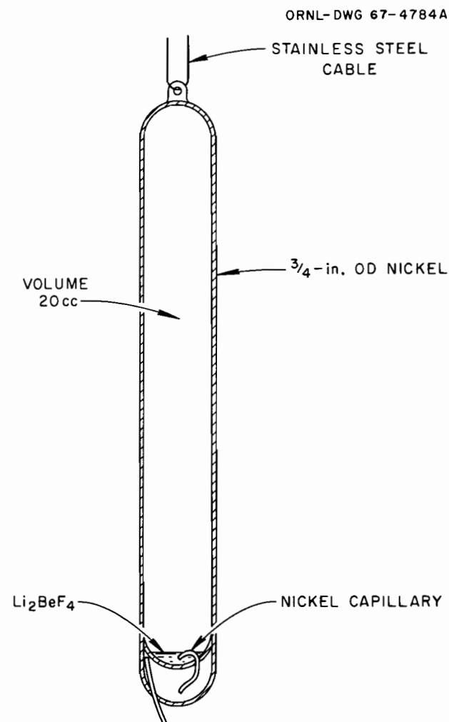
Fig. 8.1. Freeze valve capsule.
