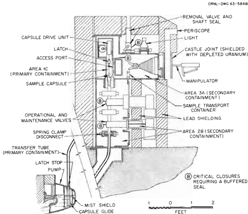
Fig. 6.1. Sampler-enricher schematic.
