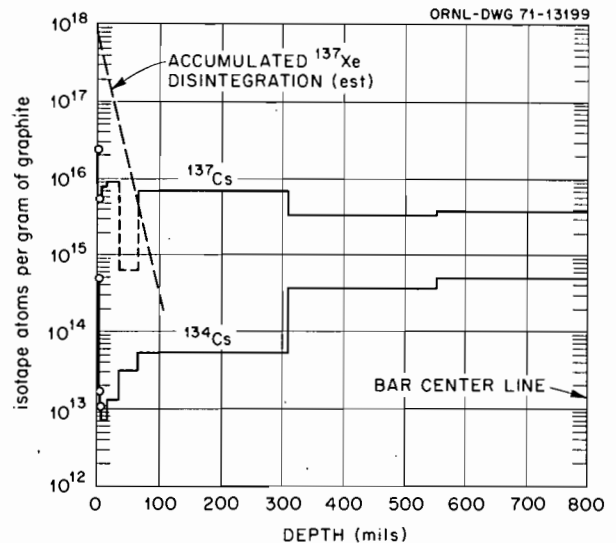
Fig. 11.6. Concentration of cesium isotopes in MSRE core graphite at given distances from fuel channel surface.
