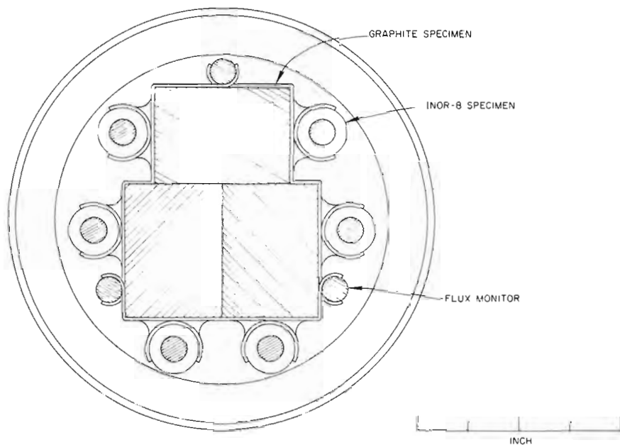
Fig. 9.4. Stringer assembly.
