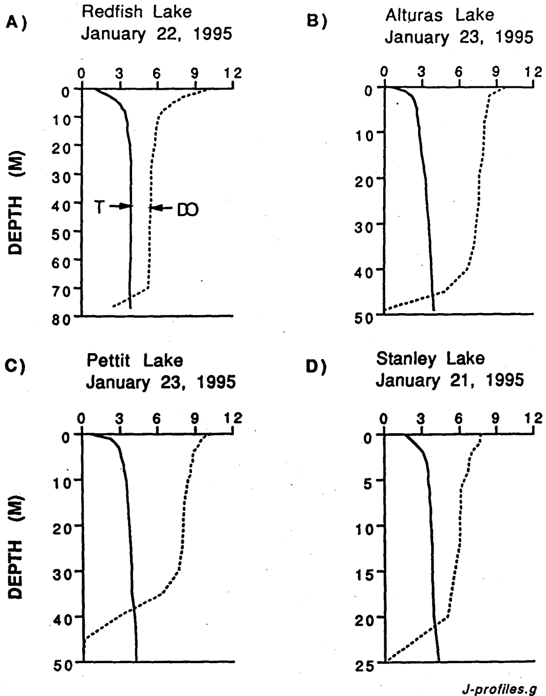
Figure 2. Temperature (T) and oxygen concentration (DO) vertical profiles of four Sawtooth Valley Lakes: A) Redfish, B) Alturas, C) Pettit, and D) Stanley Lakes. Data were collected through the ice in January 1995.
