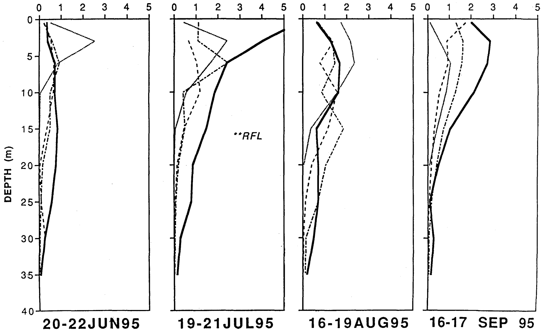
Figure 8. Rates of primary production as measured with the 14 C method in four Sawtooth Valley Lakes on four dates in 1995.
