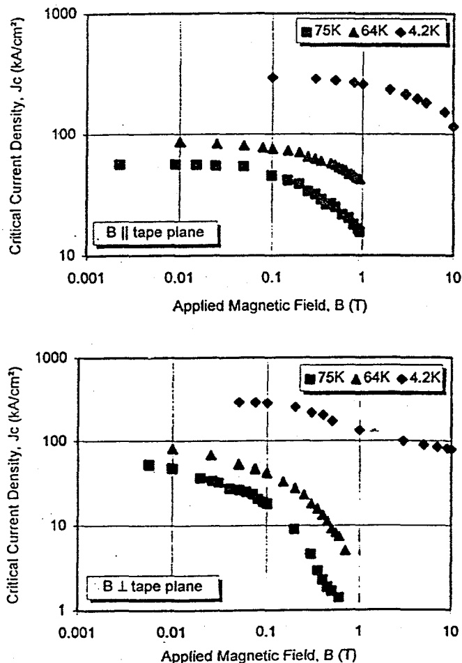
Fig. 2. The magnetic field dependence of J_c (a) for B \parallel tape plane and (b) for B \perp tape plane at temperature range from 4.2 to 75 K for the rolled 85 filament conductors.
