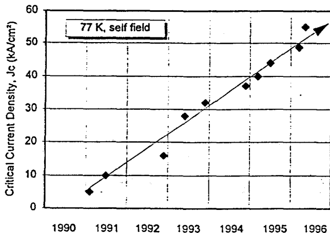
Fig. 1. Plot of J_c performance vs. time for rolled multifilamentary Bi-2223 conductors at American Superconductor Corporation.
