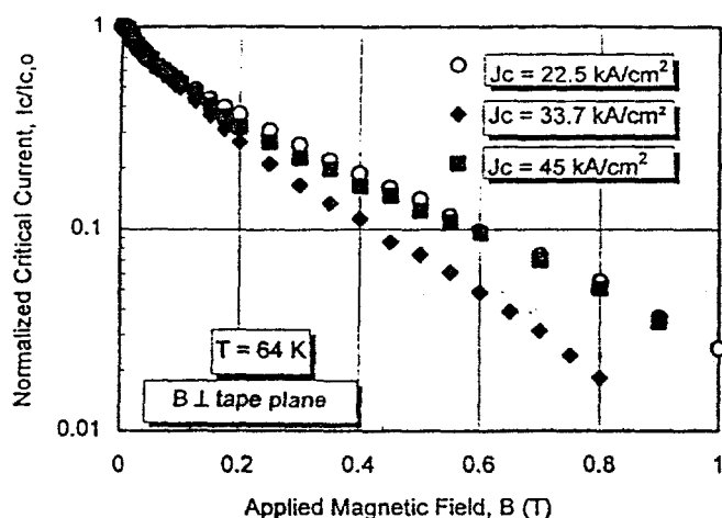
Fig. 5. The retention of critical current relative to the self field value at 64 K for three rolled 85 filamentary conductors with J_c values of 22.5, 33.7, and 45 kA/cm 2 , showing independence of connectivity and flux pinning.
